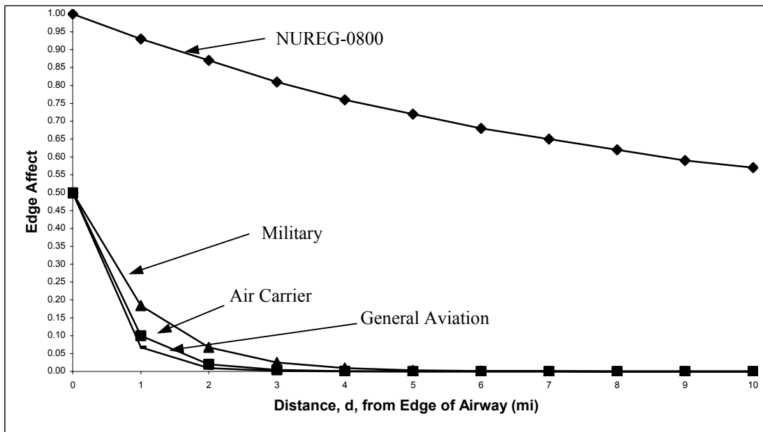
Figure 4. Illustration of Airway Models
