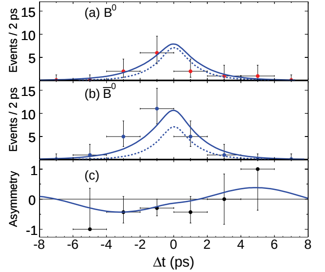
FIG. 2: Plots (a) and (b) show the \Delta t distributions of B^0 - and \bar{B}^0 -tagged B^0 \rightarrow K_S^0 \pi^0 \pi^0 candidates. The solid lines refer to the fit for all events; the dashed lines correspond to the total background. Plot (c) shows the raw asymmetry (see text). A requirement is applied on the event likelihood to suppress background.
