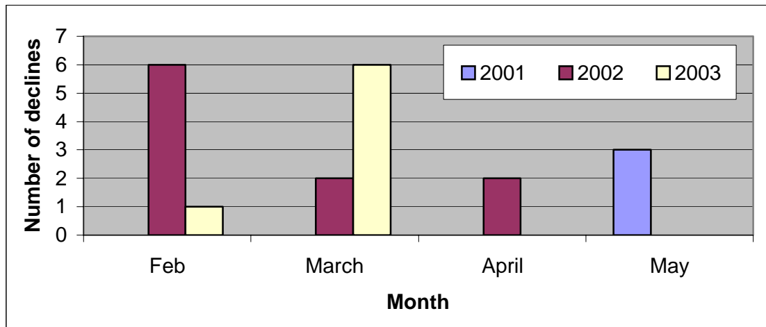
Figure 26: Frequency of tailwater declines of at least 1 foot that began at levels less than or equal to 16ft and ended at levels greater than or equal to 13 ft
