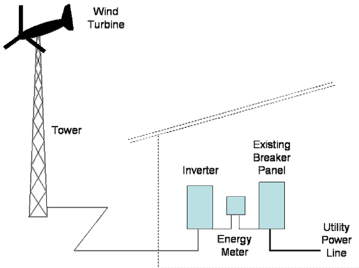
Figure 3-3. Small-scale Wind Turbine Interconnection Diagram
