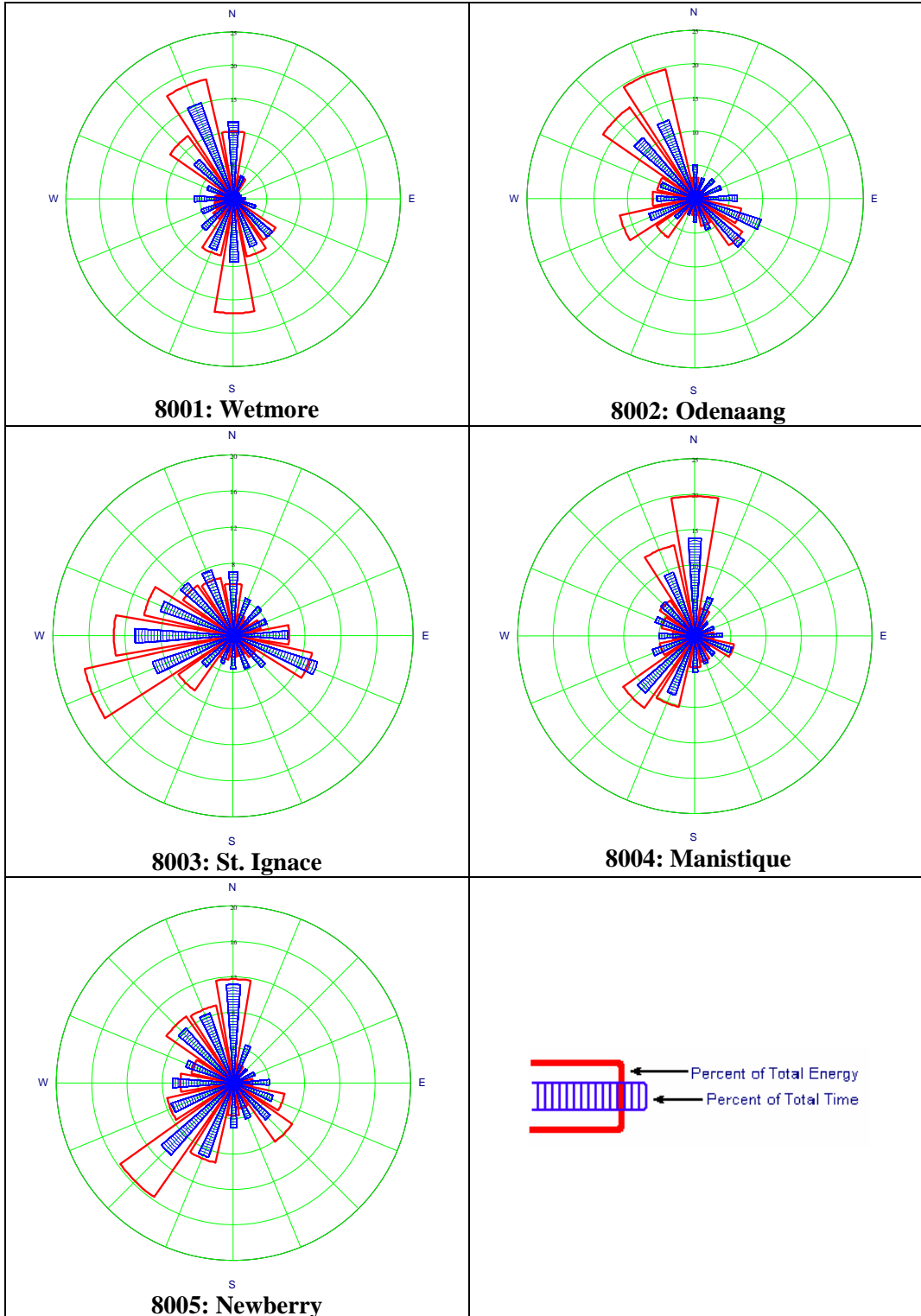
Figure 2-10. Annual Wind Roses for the Five Sites
