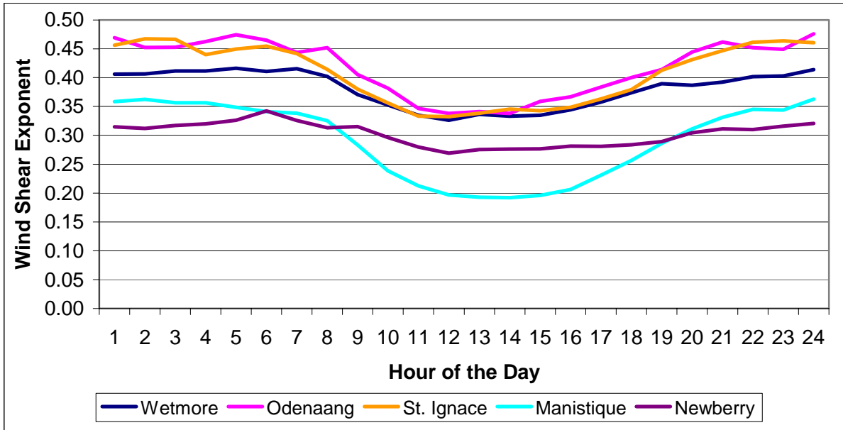
Figure 2-12. Annual Diurnal Wind Shear
