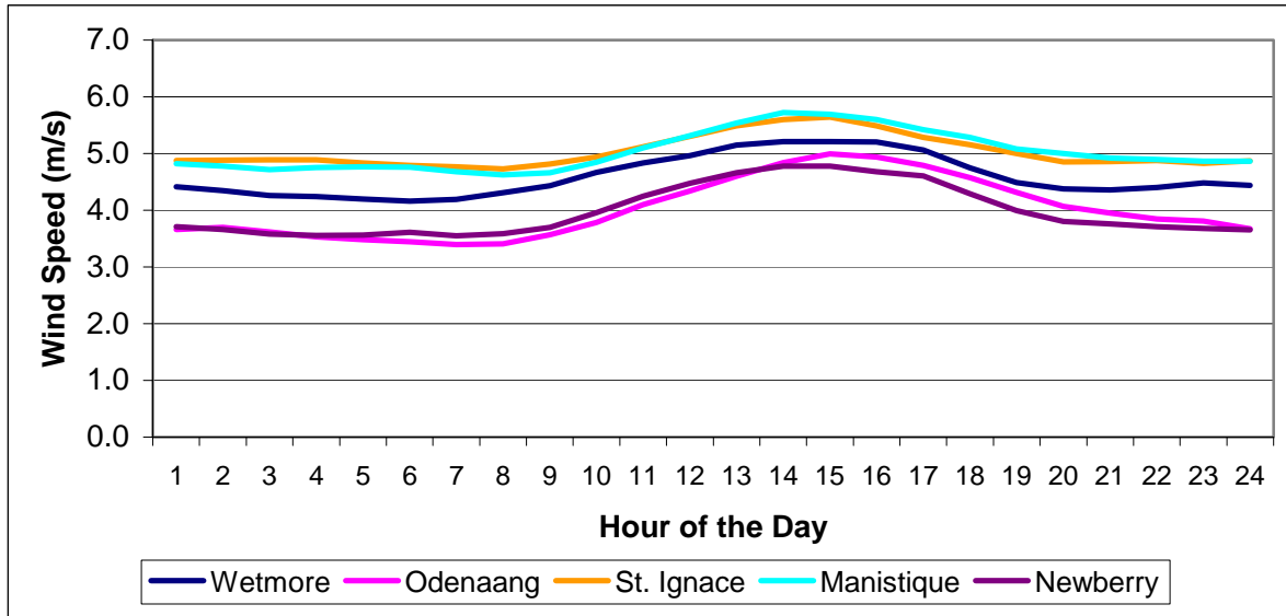
Figure 2-11. Annual Diurnal Wind Speeds
