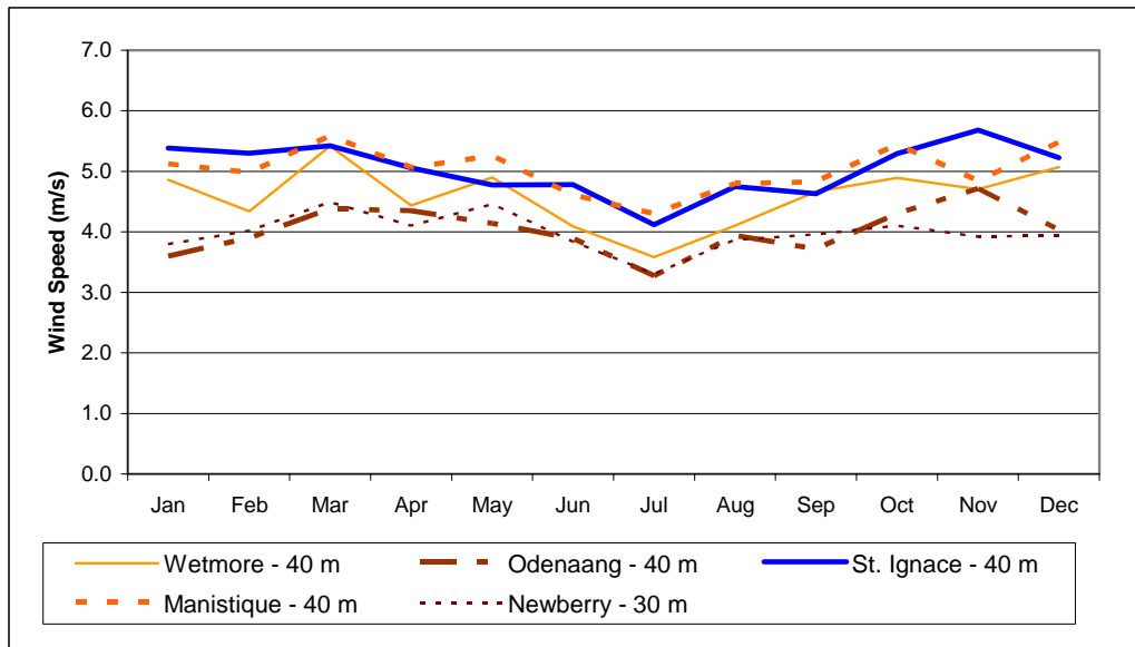
Figure 2-8. Monthly Wind Speeds
