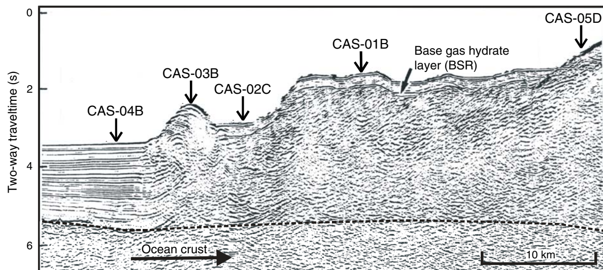
Figure F4. Seismic section (line 89-08) showing proposed Expedition 311 sites. BSR = bottom-simulating reflector.
