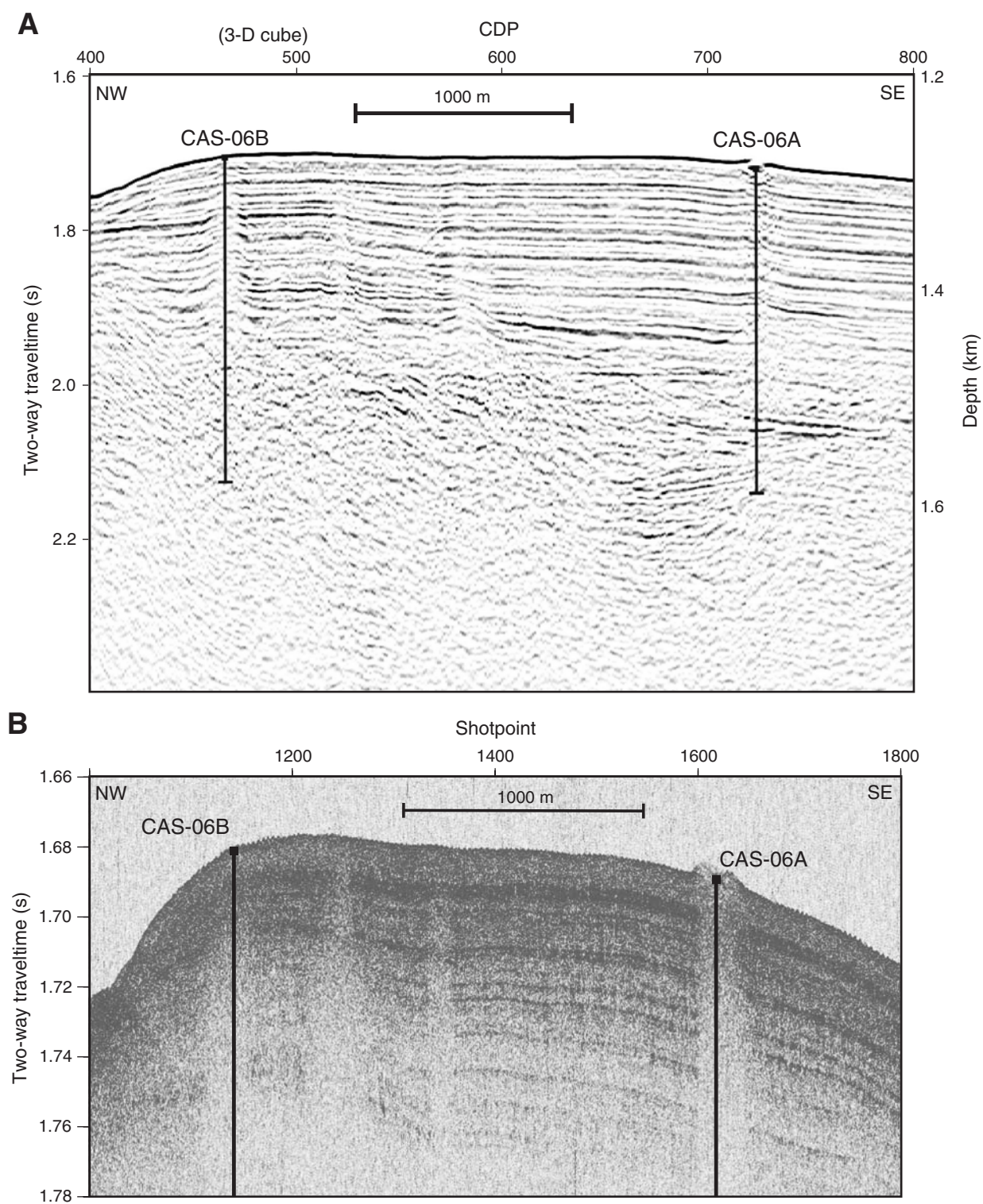
Figure F14. Site survey data for proposed Site CAS-06A. Inline 27 from 1999 3-D MCS data cube. A. MCS data (stacked). B. 3.5 kHz subbottom profiler data.
