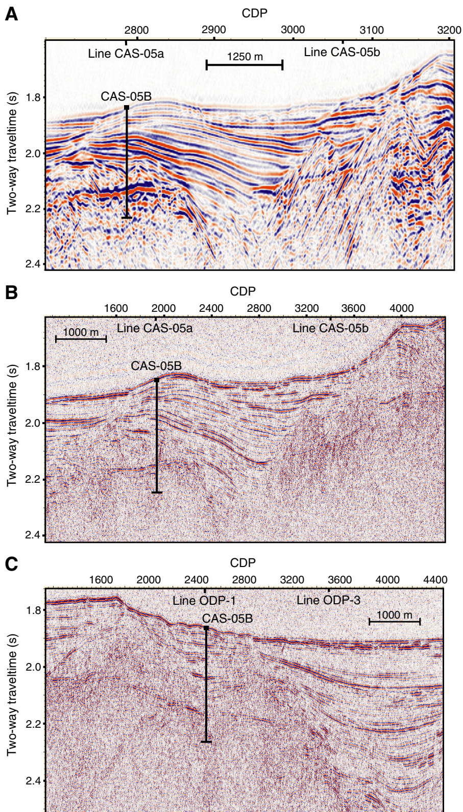
Figure F12. Site survey data for proposed Site CAS-05B. A. Conventional MCS data of Line 89-08. B. MCS data of Line PGC9902_ODP7. C. MCS data of Line PGC9902_CAS05a.
