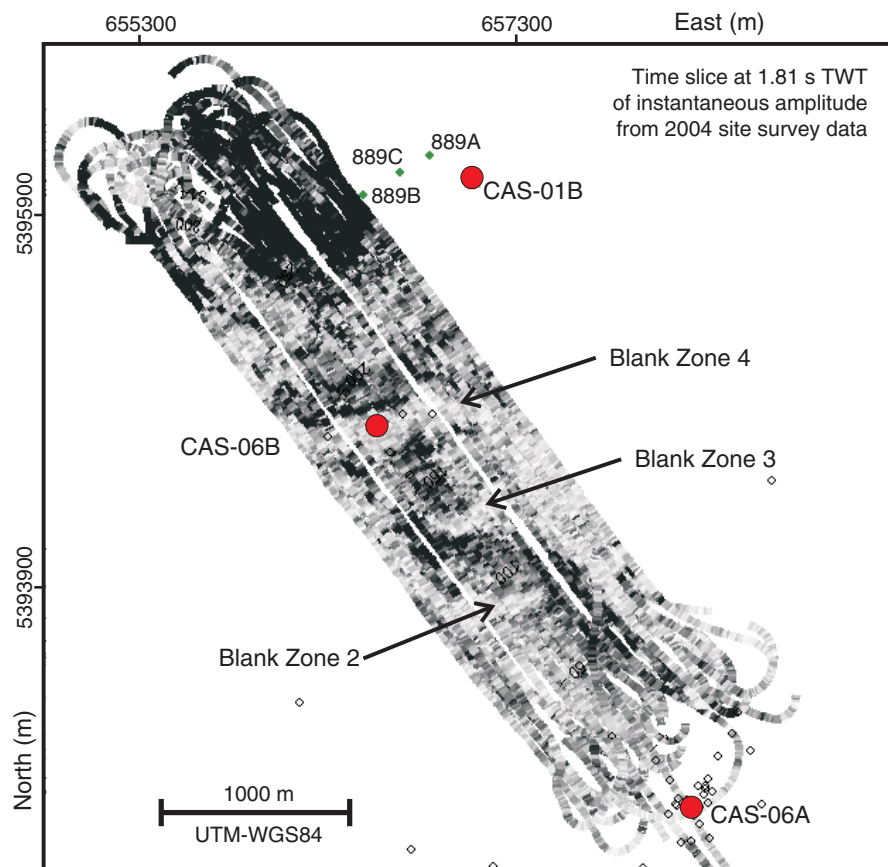
Figure F20. Site survey data for proposed Site CAS-06B. Time slice of instantaneous amplitude calculated from 2004 SCS data at 1.81 s two-way traveltime (TWT) showing extent of blank Zone 4 (CAS-06B).
