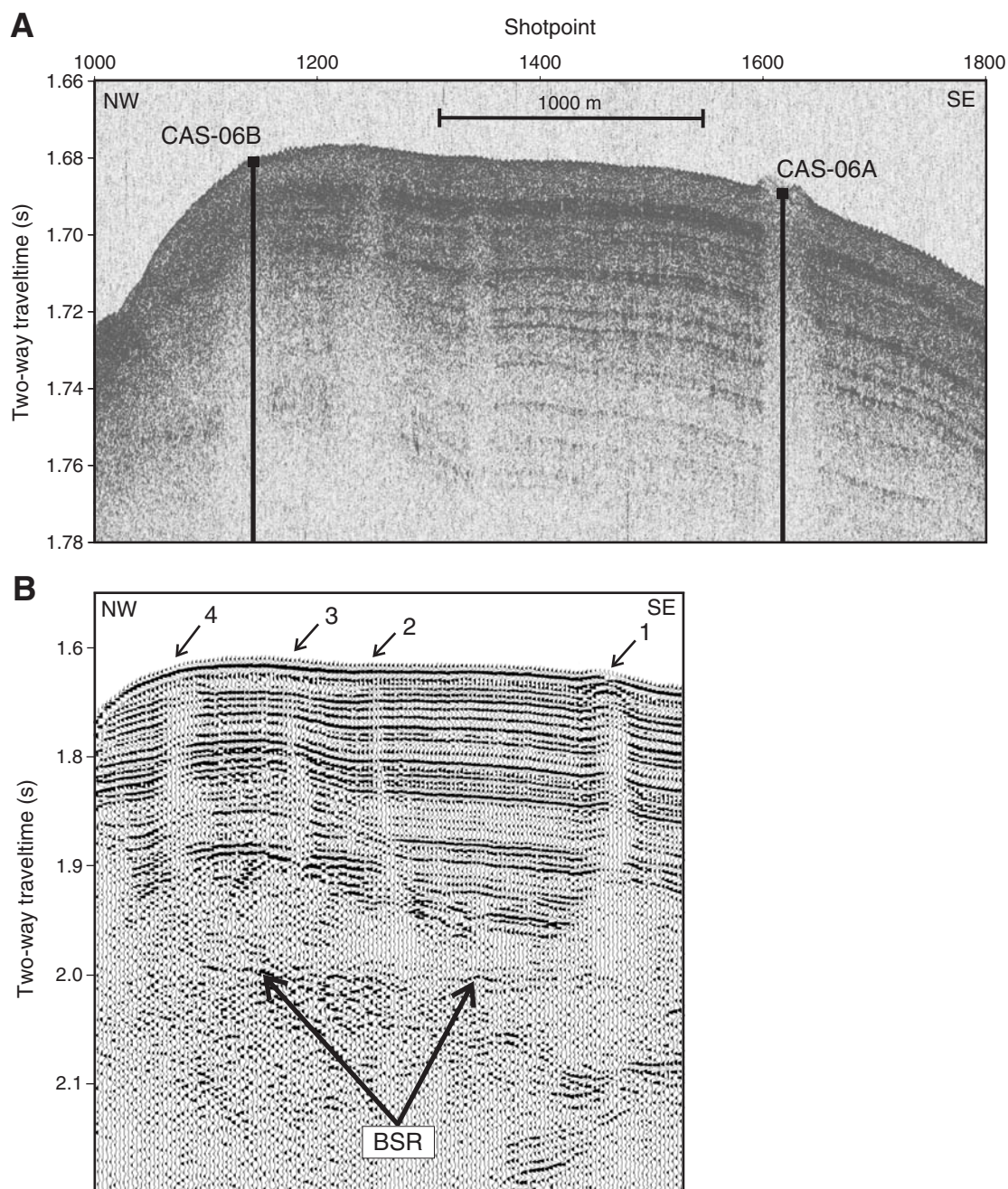
Figure F6. Seismic signature of the cold vents (blank zones) from (A) 3.5 kHz subbottom profiler (vertical exaggeration = 20) and (B) single-channel seismic data. Blank Zone 1 (proposed Site CAS-06A) is active; Zones 2–4 are inactive. Alternate Site CAS-06B is at blank Zone 4. BSR = bottom-simulating reflector.
