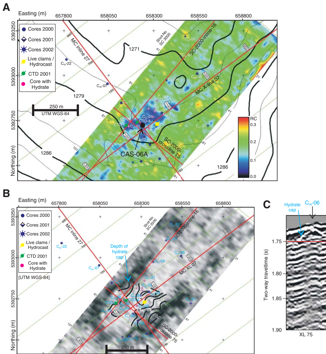
Figure F18. Site survey data for proposed Site CAS-06A. A. Map showing seafloor reflection coefficient from 2000 SCS data with location of piston cores near CAS06A. B. Map showing time slice of instantaneous amplitude from 2000 SCS 3-D data and depth of massive gas hydrate cap reflector. C. Crossline 75 through 2000 SCS 3-D data cube showing gas hydrate cap reflector. Open circles are location of piston cores taken in 2000.
