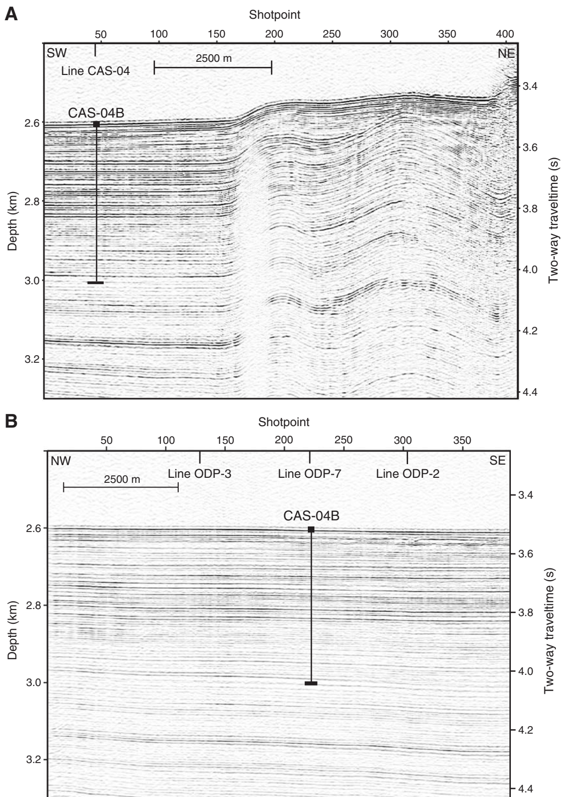
Figure F11. Site survey data for proposed Site CAS-04B. A. SCS data of Line PGC9902_ODP07. B. SCS data of Line PGC9902_CAS04.
