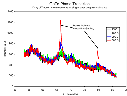
Figure 16: GaTe exhibits a phase change at 290°C.
