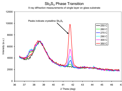
Figure 15: \text{Sb}_2\text{S}_3 exhibits a phase change at 260°C.
