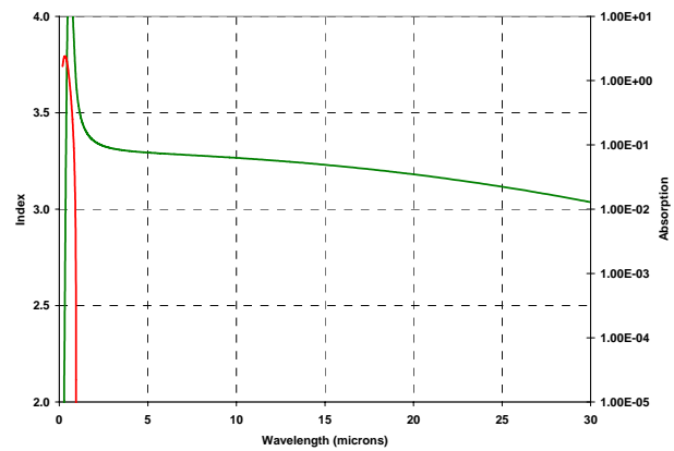
Figure 6: The real ( n ) and imaginary ( k ) components of the refractive index of \text{Sb}_2\text{Se}_3 are presented. The measurements were made from single layer samples of \text{Sb}_2\text{Se}_3 on silicon and glass using VASE ellipsometry.
