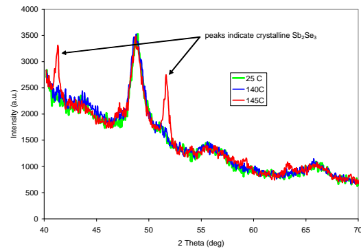
Figure 10: The absorption seems to be related to a phase change which occurs rapidly at or about 145^\circ\text{C} .
