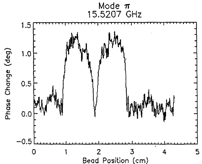
Figure 5: Perturbation measurement result for \pi -mode
