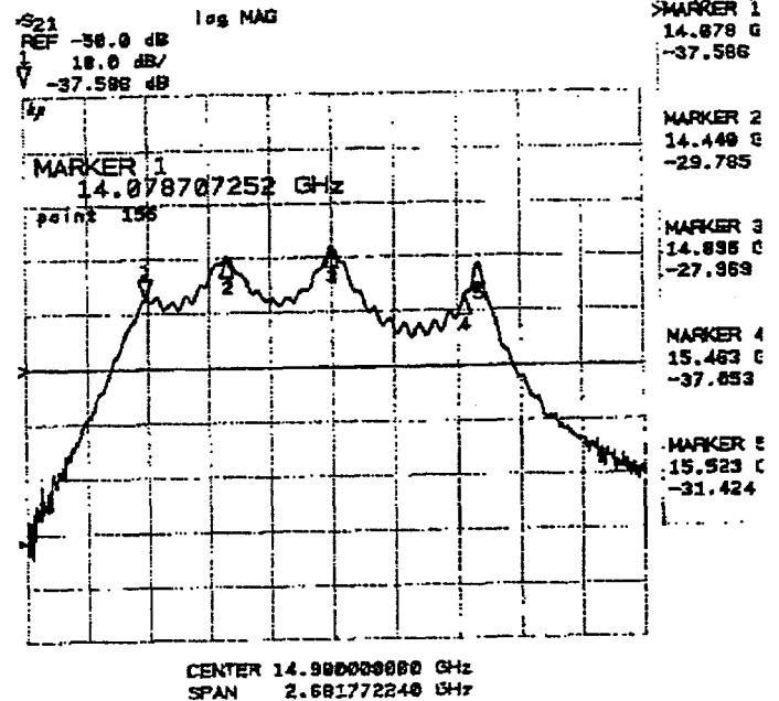
Figure 4: Frequency spectrum of the excited modes
