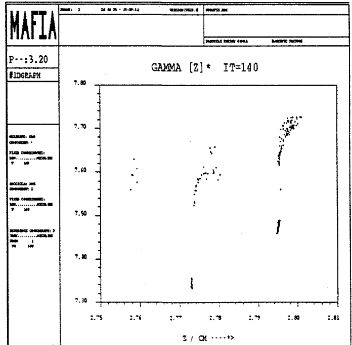
Figure 2: Particle beam energy distribution
