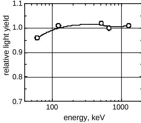
Fig. 5. Proportionality in light yield as a function of \gamma -ray energy measured for \text{LaBr}_3\text{:Ce} at room temperature.
