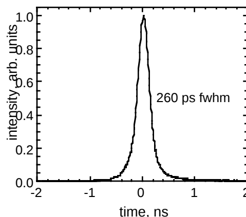
Fig. 4. Timing resolution spectrum measured for a \text{LaBr}_3:\text{Ce} (5% \text{Ce}^{3+} ) crystal in coincidence with a \text{BaF}_2 crystal.
