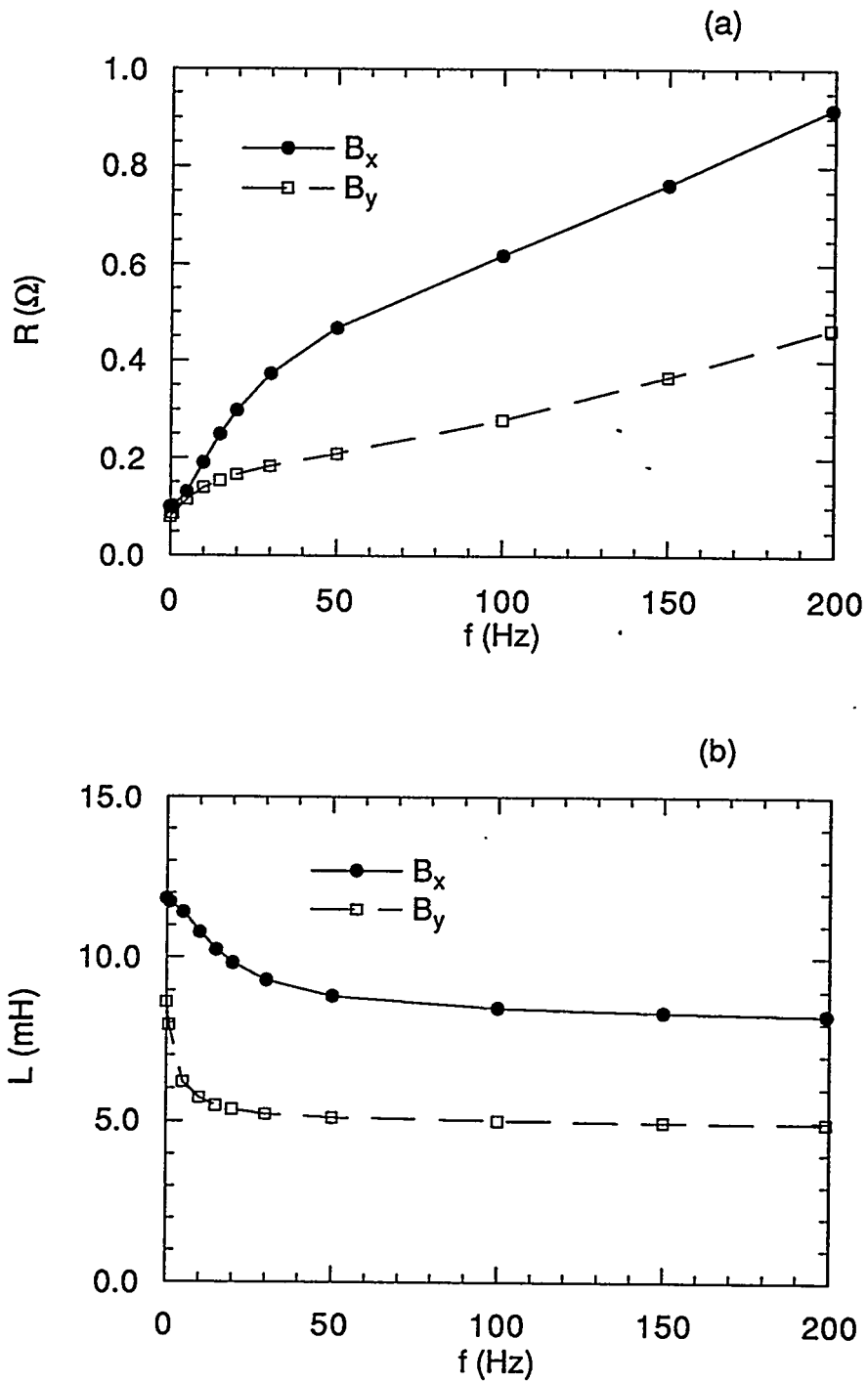
Fig. 3.1: Change of magnet impedance due to the vacuum chamber eddy current as a function of frequency: (a) resistance R in units of \Omega and (b) inductance L in units of mH.
