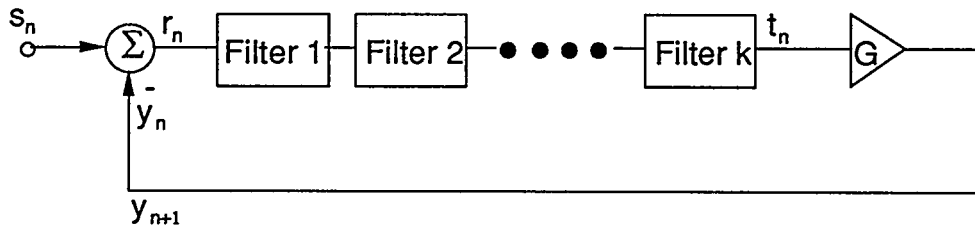
Fig. 5.3: Closed loop feedback with multiple filtering elements.
