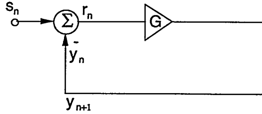
Fig. 5.1: A simple digital closed loop feedback system with open loop gain G > 0 .
