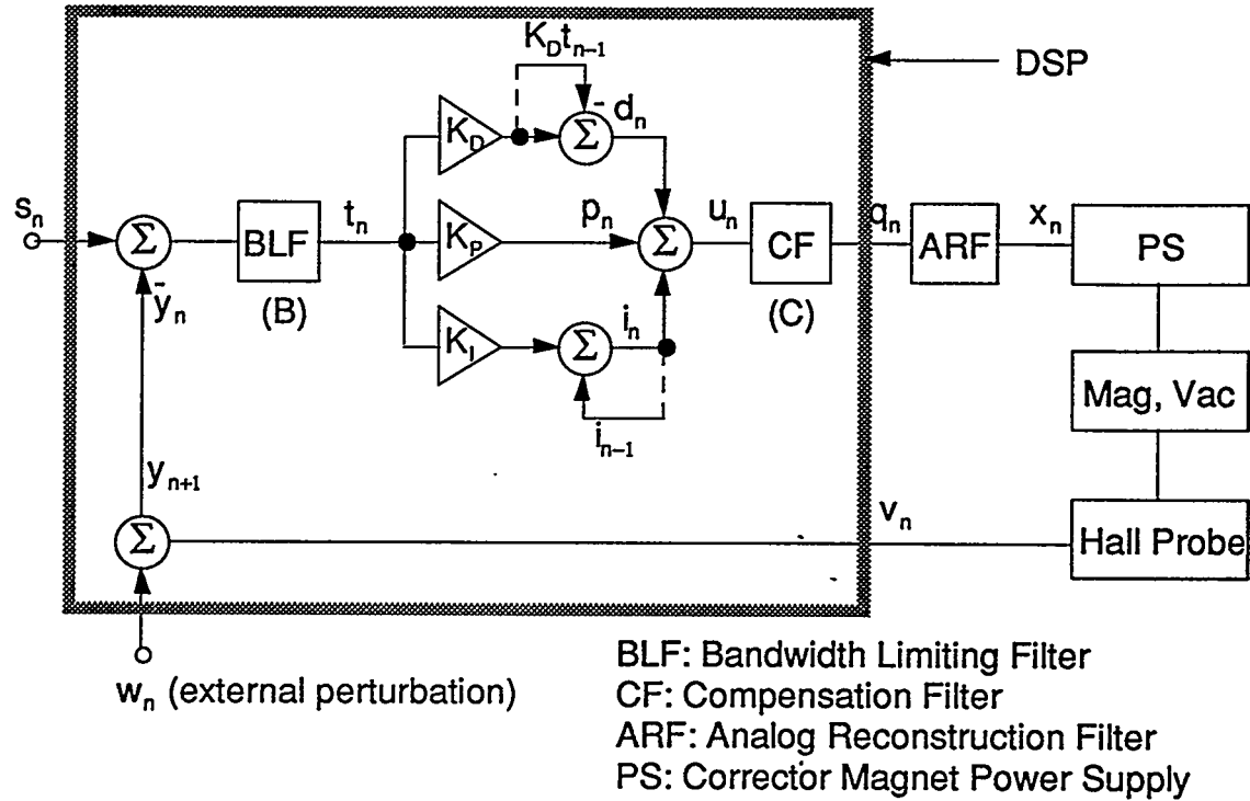
Fig. 6.1: Schematic diagram for the closed loop feedback with PID control.
