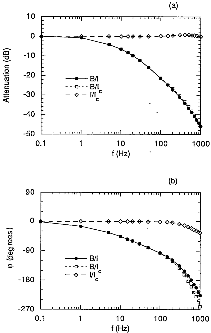
Fig. 6.3: Results of the open loop measurements on (a) the amplitude ratios and (b) the relative phases of current control signal I_c , magnet current I , and the magnetic field B in the vacuum chamber.
