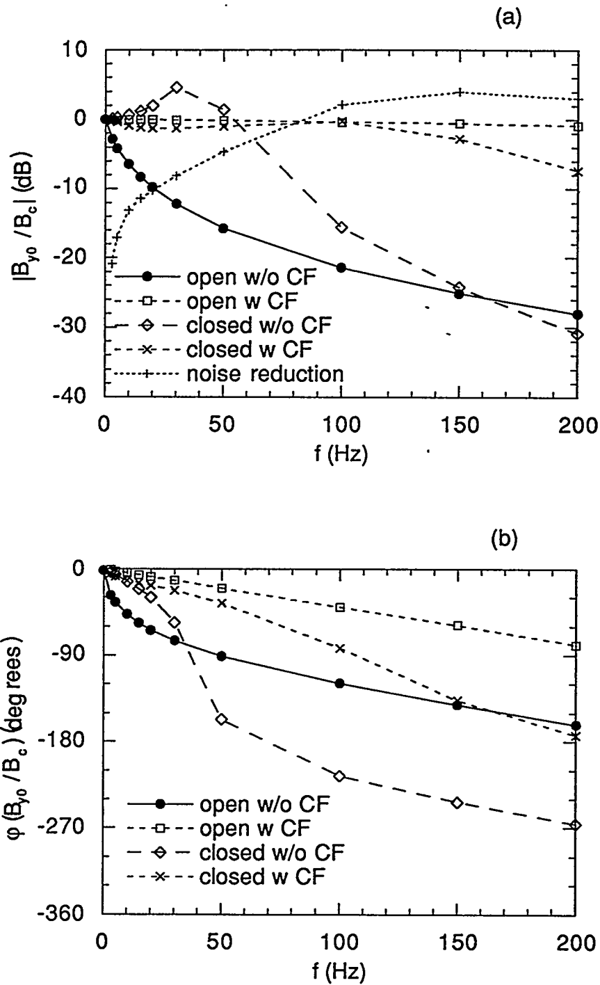
Fig. 6.4: Results of measurement on the closed loop feedback for corrector magnet field: (a) amplitude attenuation and (b) phase shift. For closed loop measurements, an analog reconstruction filter of 200 Hz bandwidth was inserted in front of the power supply to suppress ringing. The parameters used were: F_s = 4 kHz, f_b = 30 Hz, K_P = 3 , K_I = 0.05 , and K_D = 0.5 .
