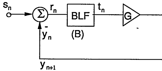
Fig. 5.2: A simple P-control closed loop feedback system.
