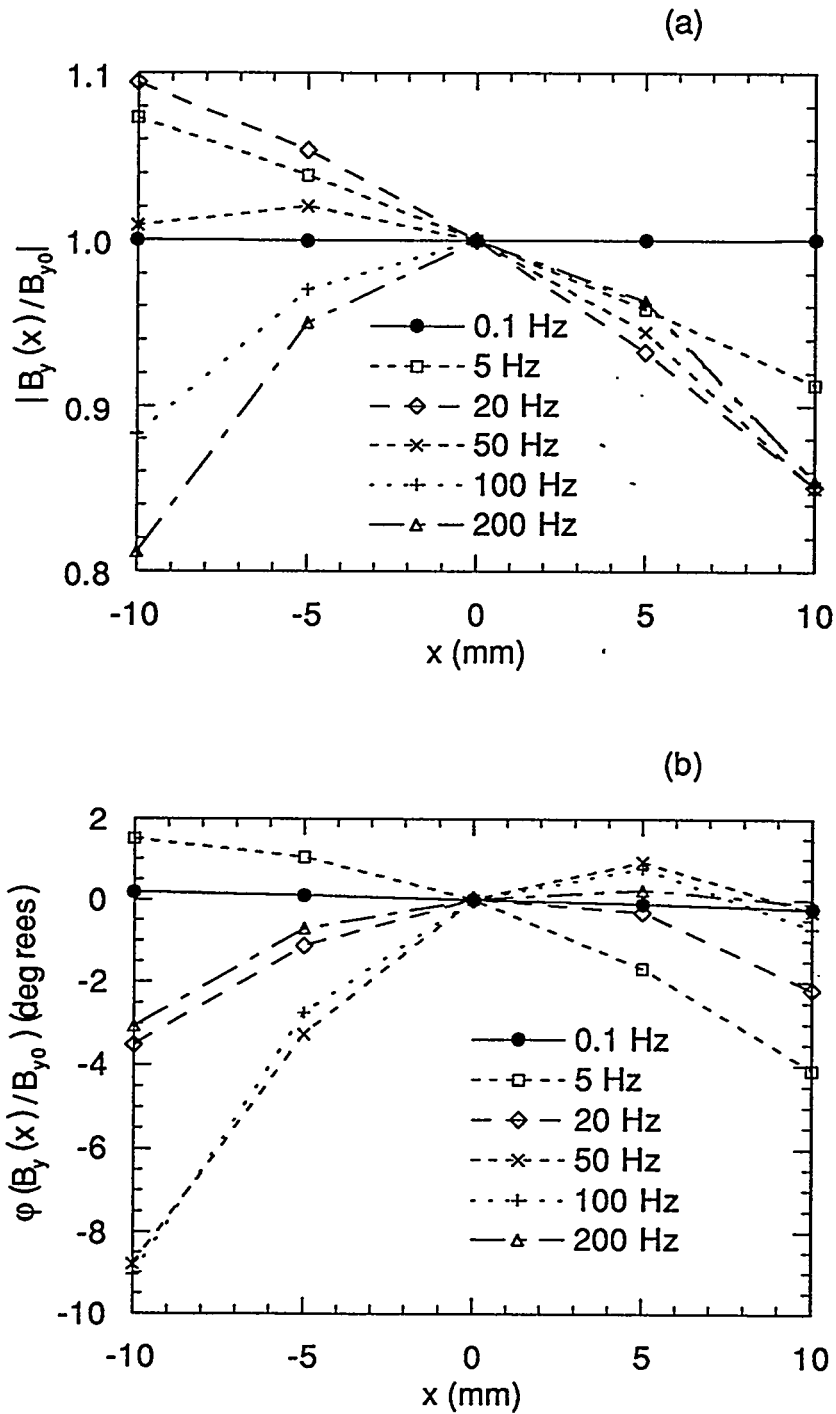
Fig. 4.2: Dependence of the magnetic field in the vacuum chamber on the position and the frequency. x is the horizontal distance from the center where the field was measured. The antechamber side is the positive direction. (a) Amplitude attenuation and (b) phase delay relative to the center ( x = 0 ).
