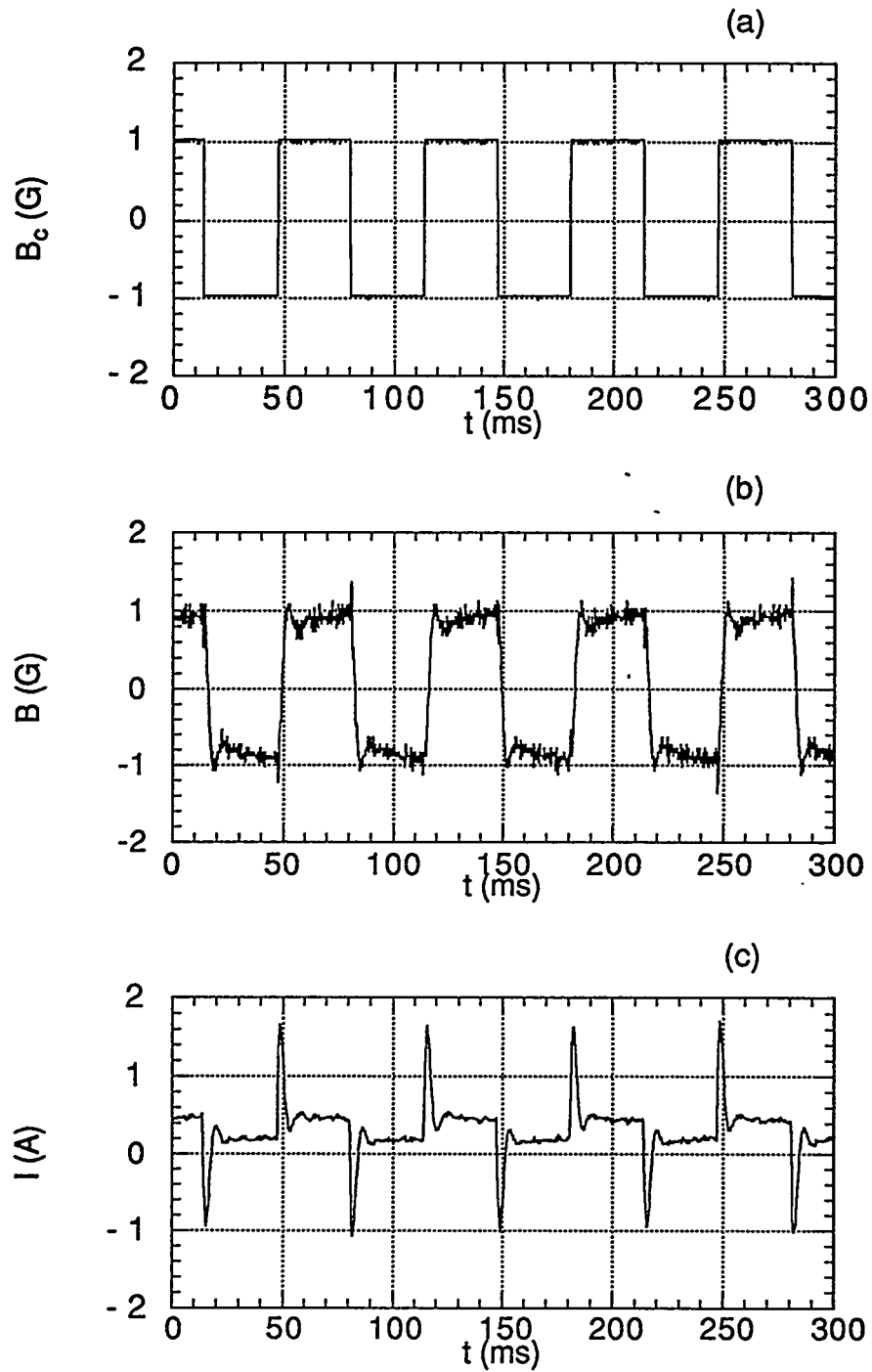
Fig. 6.6: Feedback system response in the time domain with eddy current compensation: (a) magnetic field control signal B_c ( s_n , 15 Hz square wave), (b) magnetic field in the vacuum chamber ( y_n ), and (c) magnet current I . The parameters used were: F_s = 4 kHz, f_b = 30 Hz, K_p = 3 , K_I = 0.05 , and K_D = 0.5 .
