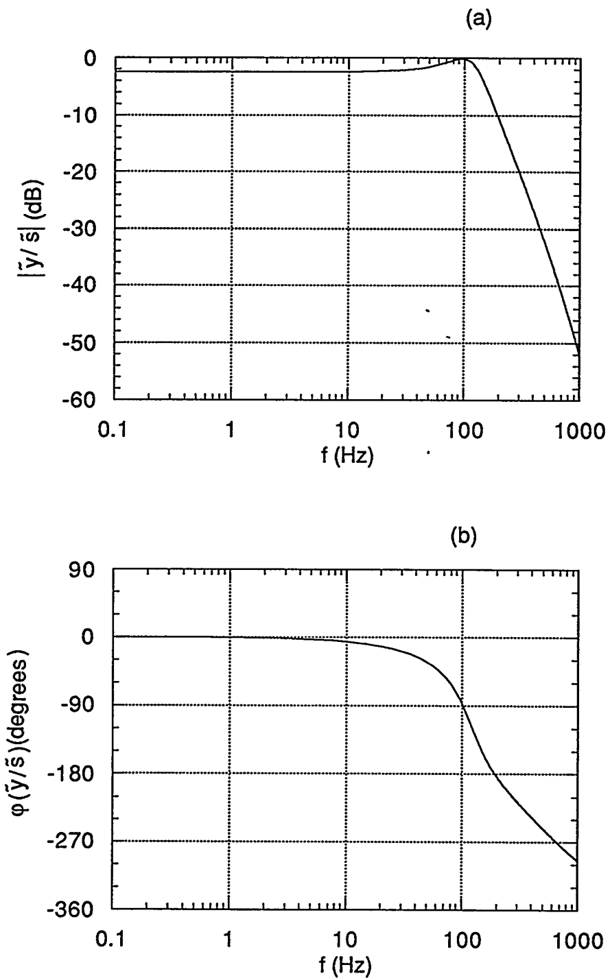
Fig. 5.4: Frequency response of the closed loop feedback system with parameters in Eq. (5.25), (a) magnitude and (b) phase. Note that there is a resonance at f \approx 100 Hz.
