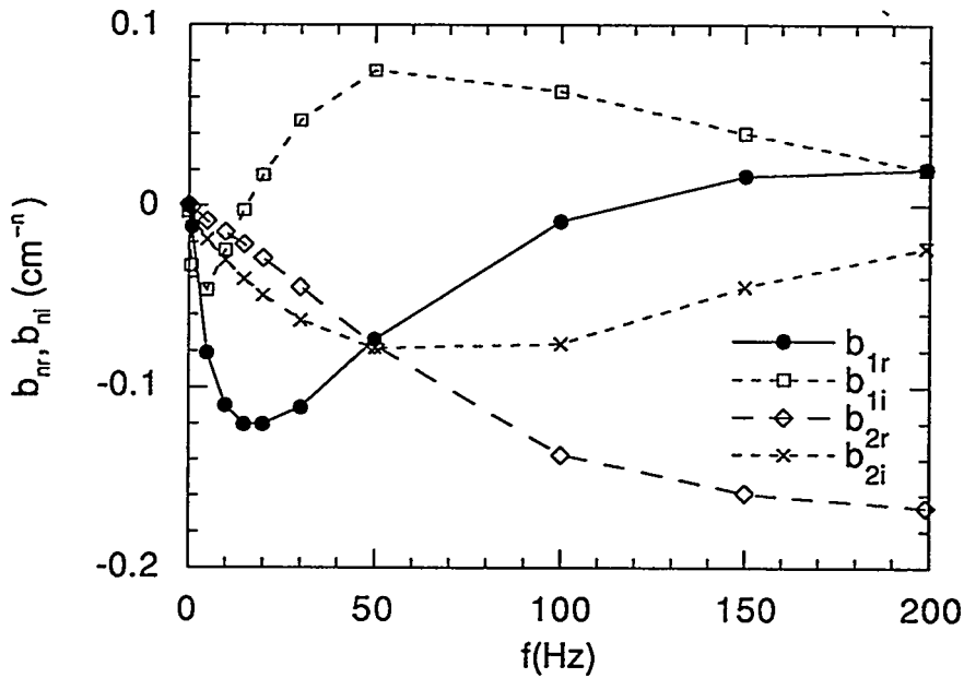
Fig. 4.3: Plotting of the multipole coefficients b_{1r} , b_{1i} , b_{2r} , and b_{2i} as functions of frequency.
