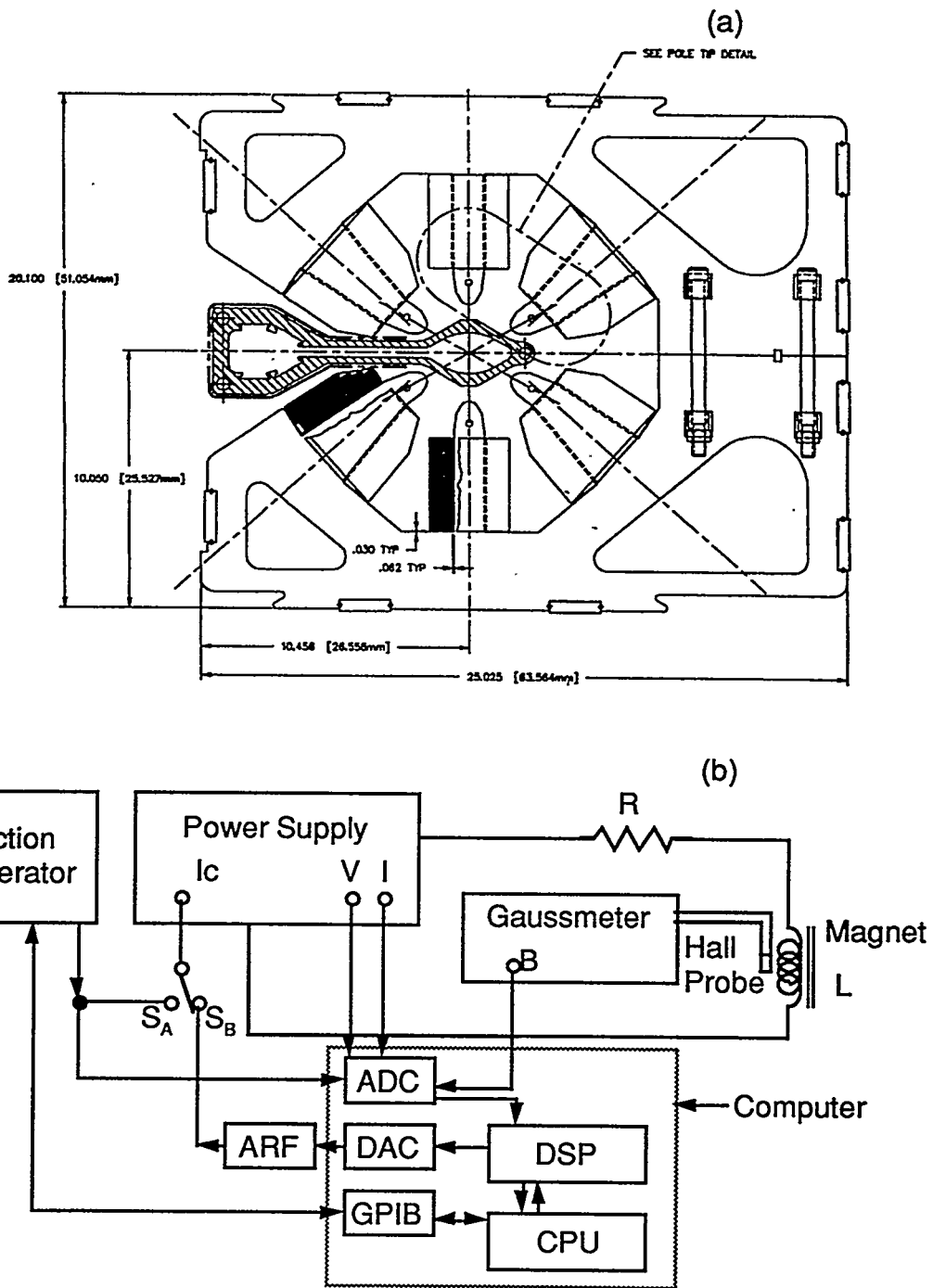
Fig. 2.1: (a) Vacuum chamber cross section in the storage ring H/V corrector magnet, similar to the sextupole magnet used in this work. (b) Schematic diagram of measurement setup for the eddy current effect on the magnet field. The voltage ( V ) and the current ( I ) signals were provided by the power supply and the magnet field ( B ) was measured by a gaussmeter with a Hall probe. The ADC and DAC are on the ATMIO-16 board. ARF is an analog reconstruction filter with 200 Hz bandwidth.
