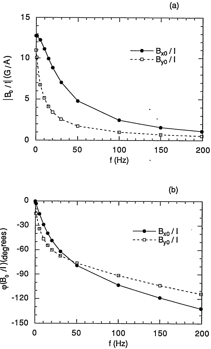
Fig. 4.1: (a) Attenuation of the field efficiency |B_{x,y0}/I| and (b) phase shift \phi between the field and the current as functions of frequency at the center of the vacuum chamber ( x = 0 ).
