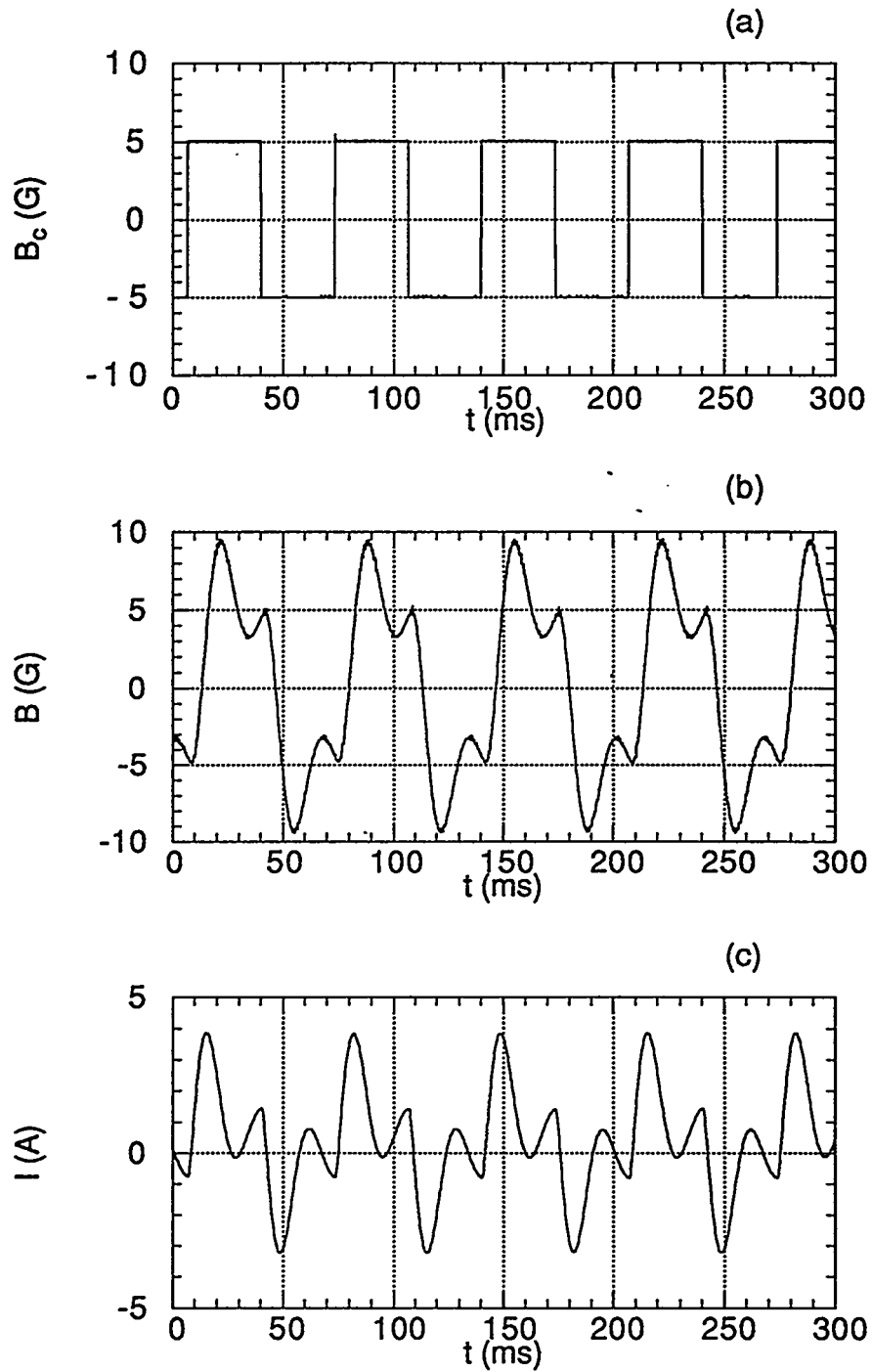
Fig. 6.5: Feedback system response in the time domain without eddy current compensation: (a) magnetic field control signal B_c ( s_n , 15 Hz square wave), (b) magnetic field in the vacuum chamber ( y_n ), and (c) magnet current I . The parameters used were: F_s = 4 kHz, f_b = 30 Hz, K_P = 3 , K_I = 0.05 , and K_D = 0.5 .
