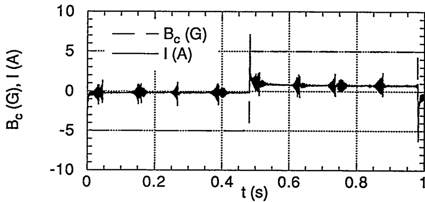
Fig. 6.2: Ringing in the magnet current with the feedback loop closed (solid line). The dotted line is the field control signal of 1 Hz square pulse. The ARF was turned off and the parameters used were: F_s = 2 kHz, f_b = 20 Hz, K_P = 3 , K_I = 0.1 , and K_D = 1 .
