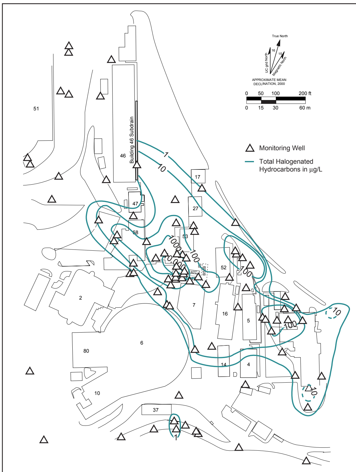
Figure 6-4 Groundwater Contamination (Total Halogenated Hydrocarbons in µg/L) in Old Town Area (September 2001)
