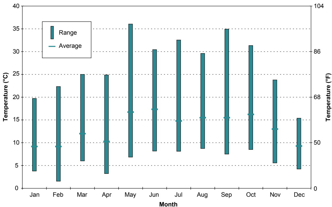
Figure 2-5 Temperature Summary by Month
