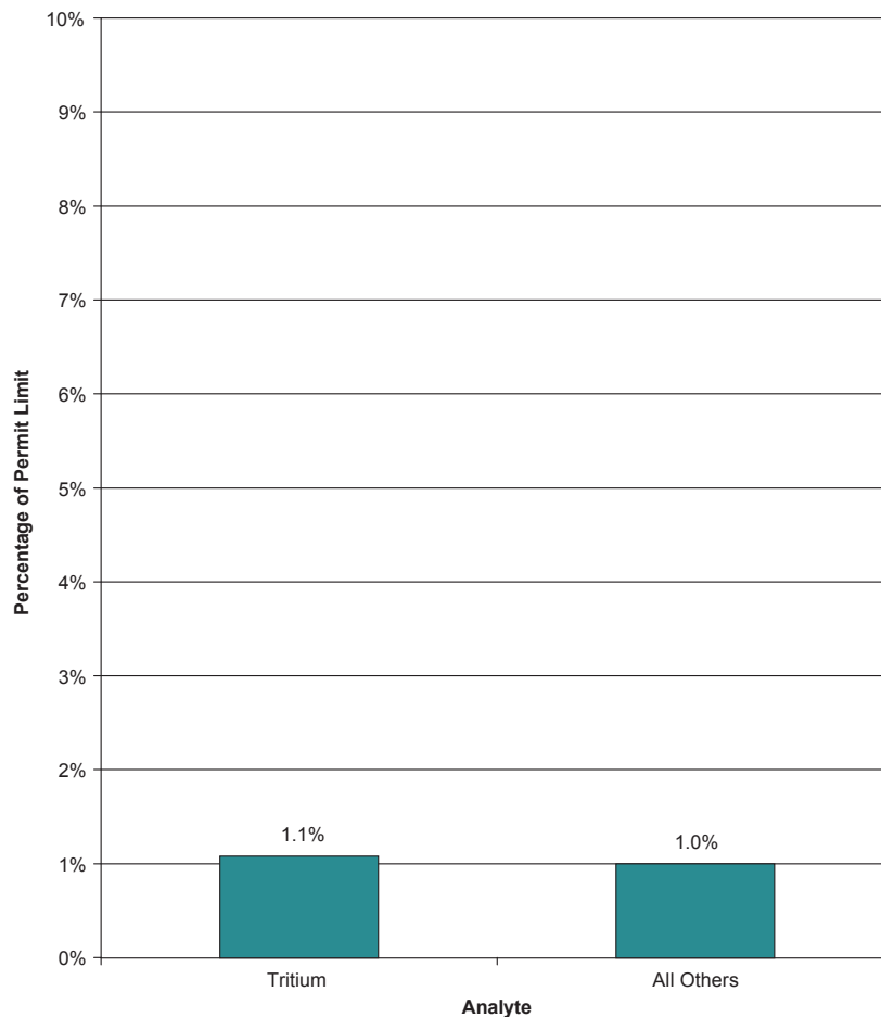
Figure 5-9 Radioisotopes Discharged to Sewers in 2001 as a Percentage of Permit Limit
