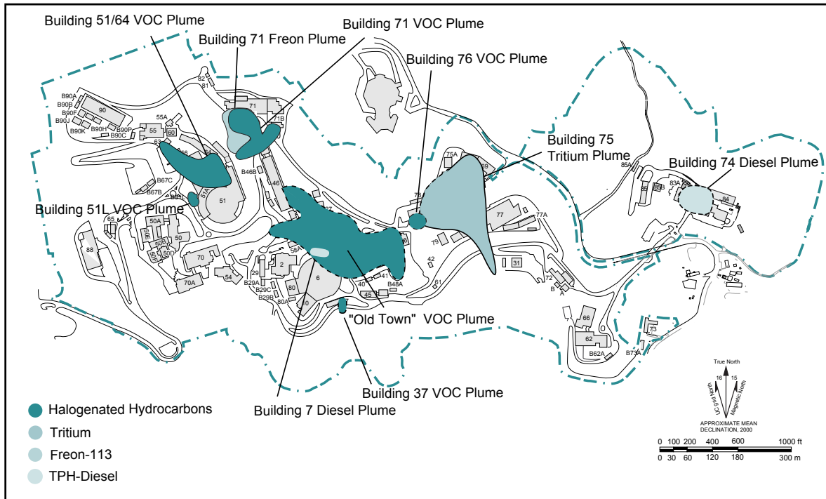
Figure 6-3 Groundwater Contamination Plumes (September 2001)
