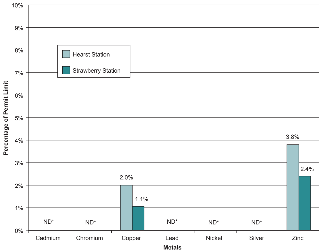
Figure 5-8 Concentration of Metals in Sewer Water Samples as a Percentage of Permit Limit
