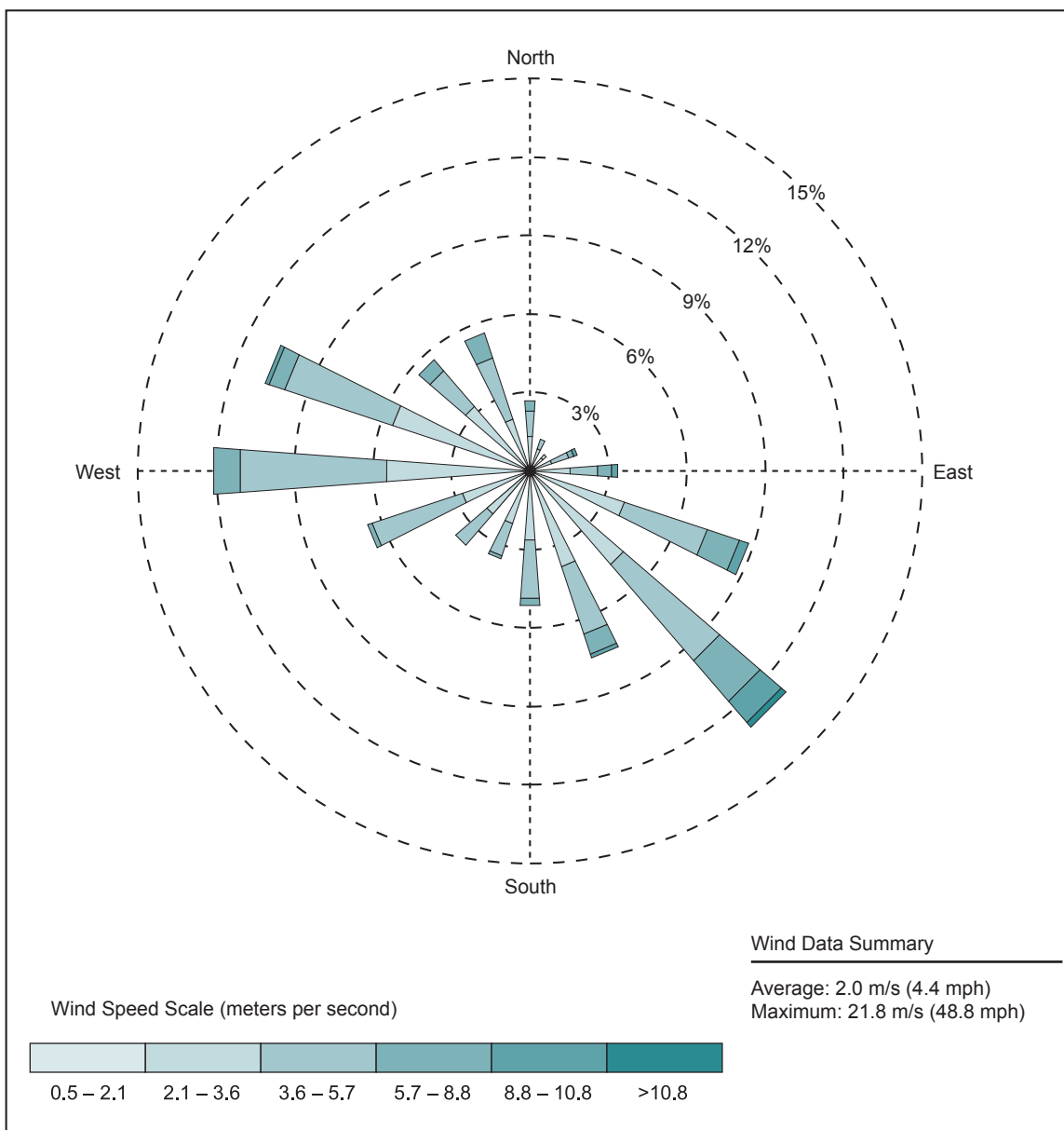
Figure 2-6 Annual Wind Patterns
