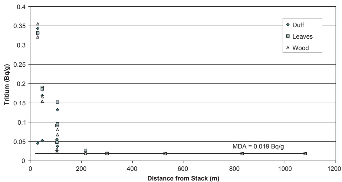
Figure 10-8 Tissue-Free Water Tritium Results with Distance from the NTLF Hillside Stack
