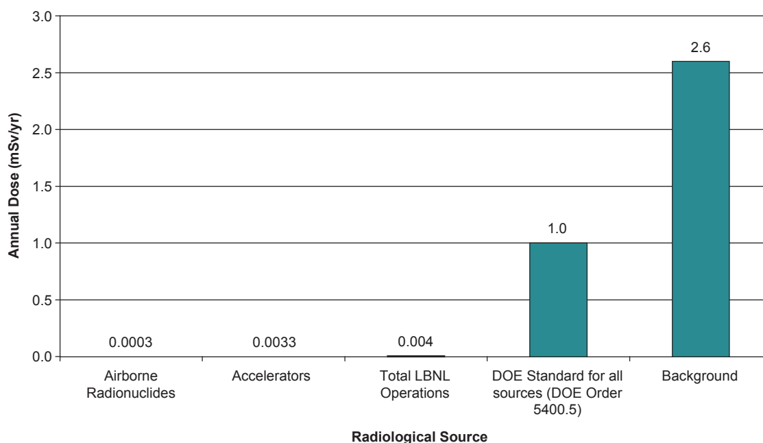
Figure 9-2 Comparison of Radiological Dose Impacts
