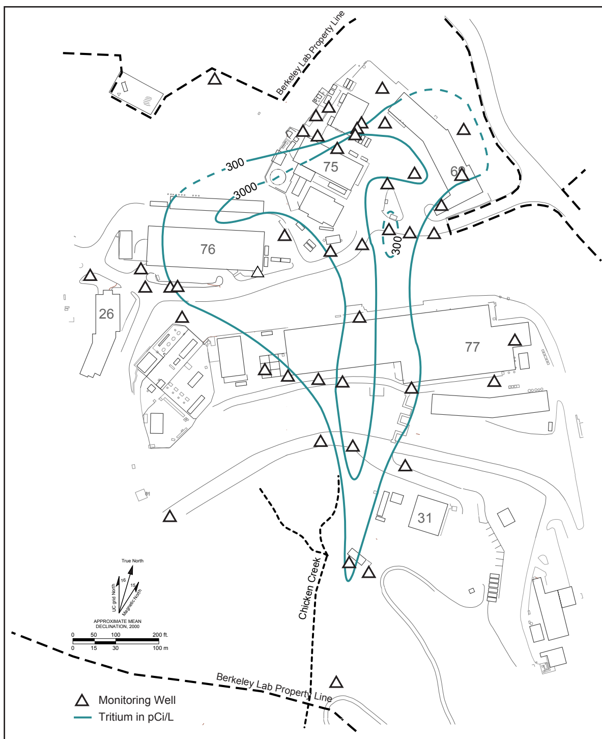
Figure 6-6 Groundwater Contamination (Tritium in pCi/L), October to December 2001
