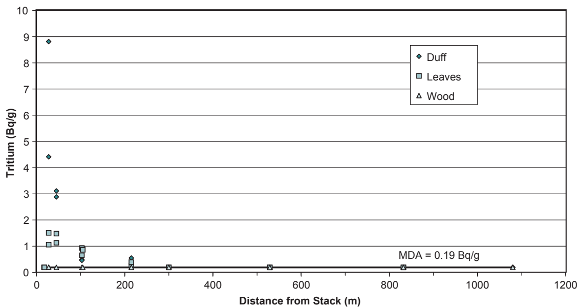
Figure 10-9 Organically Bound Tritium Results with Distance from the NTLF Hillside Stack
