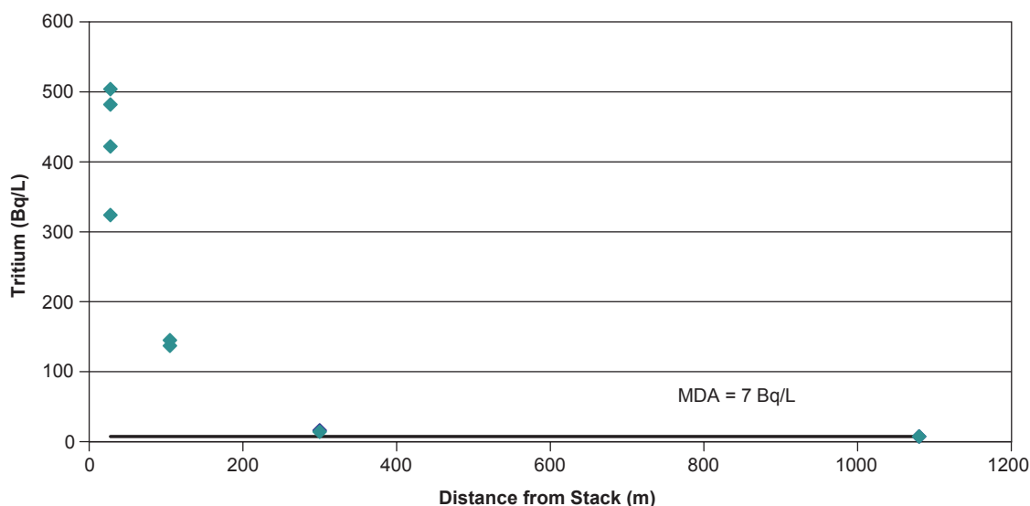
Figure 10-10 Tritium in Transpired Water with Distance from the NTLF Hillside Stack
