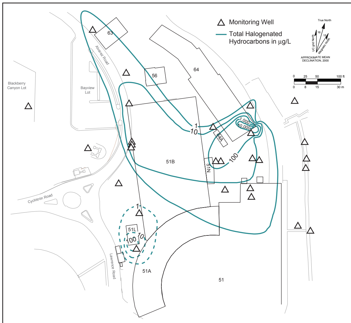
Figure 6-5 Groundwater Contamination (Total Halogenated Hydrocarbons in µg/L) at Building 51/64 VOC Plume (September 2001)
