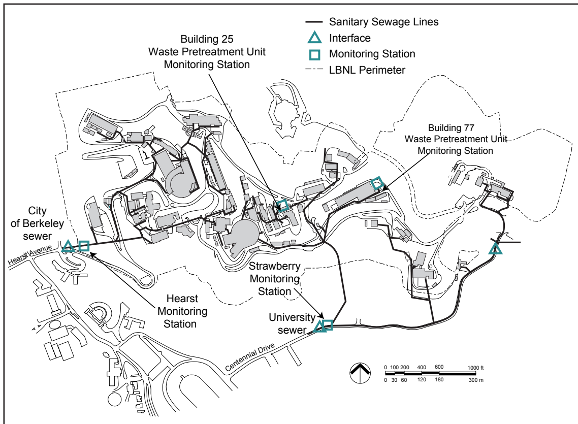
Figure 5-7 Sanitary Sewer System
