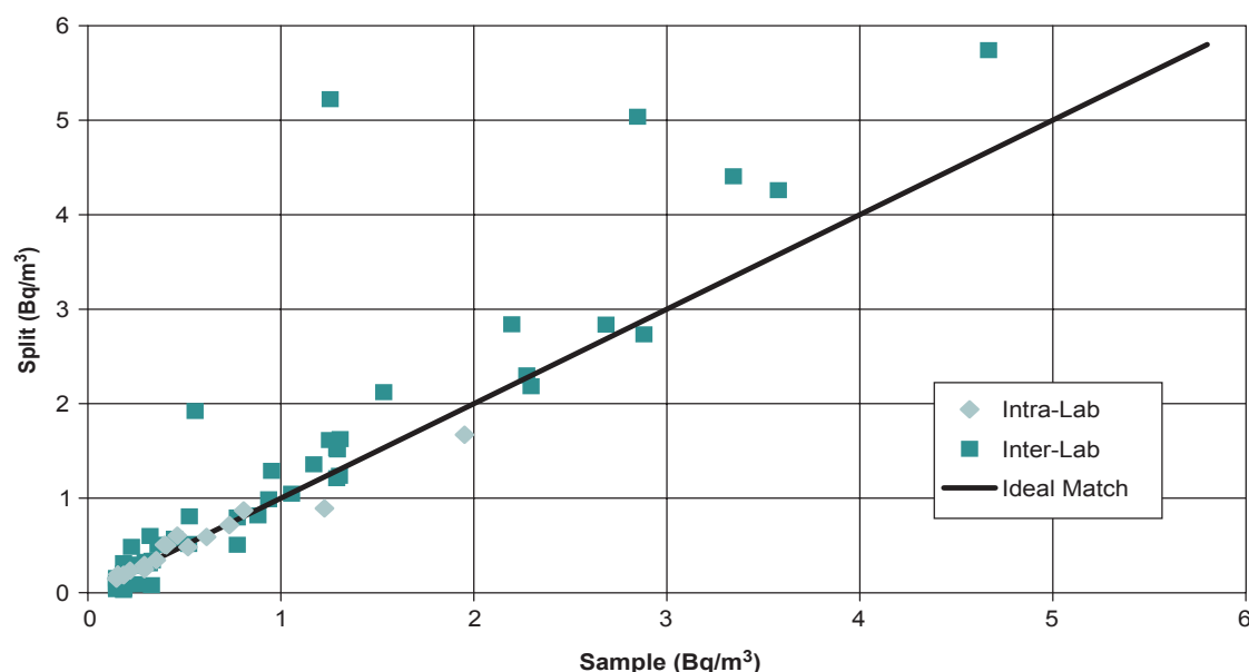
Figure 11-1 Comparison of Split Results for Tritiated Water in Ambient Air
