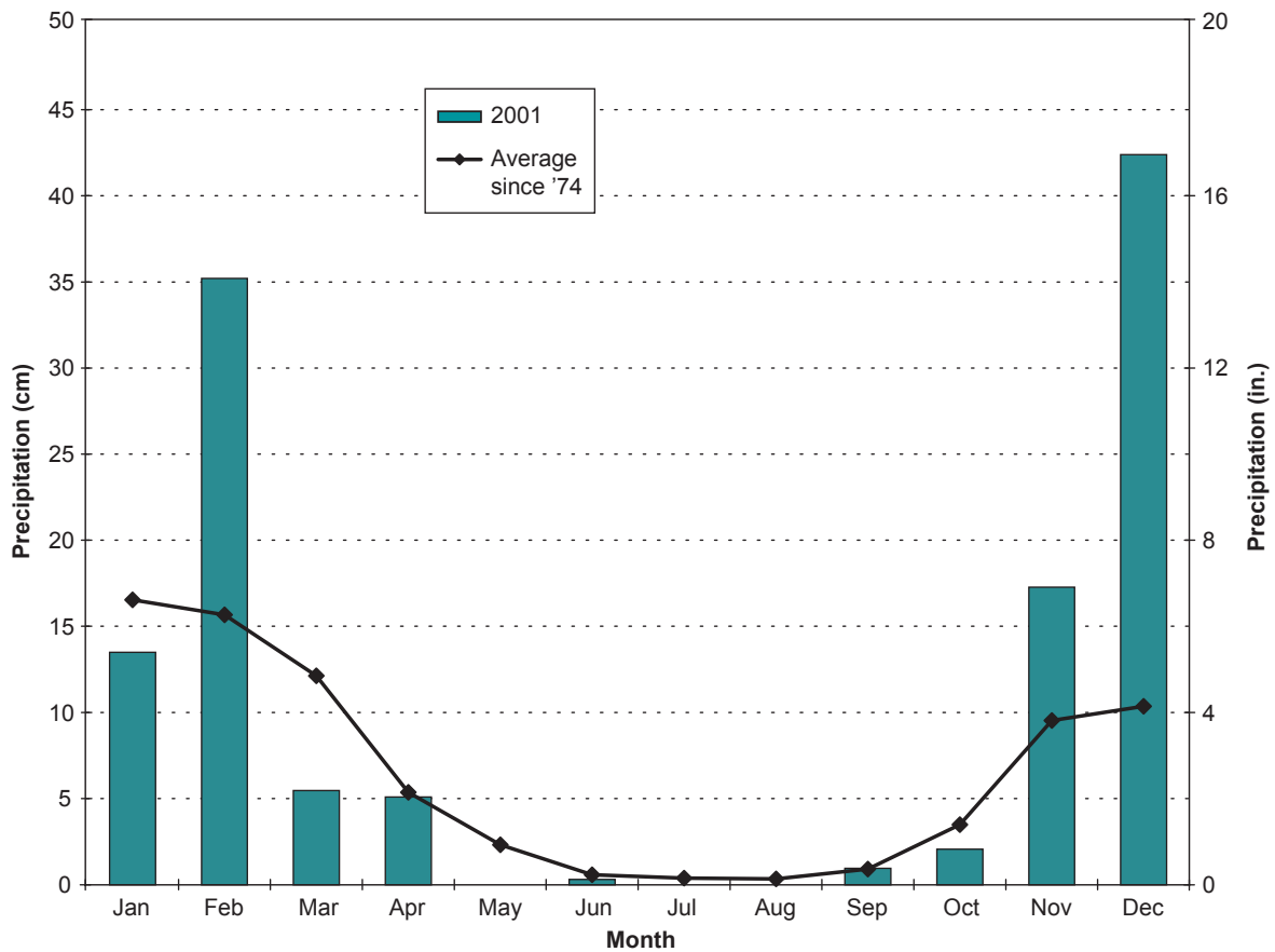
Figure 2-7 Precipitation Summary by Month
