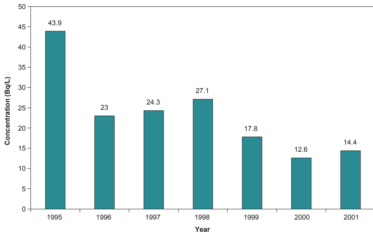
Figure 5-5 Annual Averages for Tritium in Chicken Creek (1995–2001)
