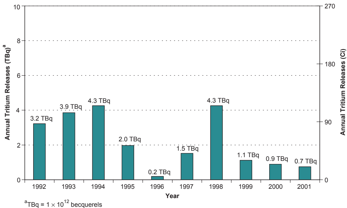
Figure 4-1 Trends in Annual Tritium Releases from NTLF
