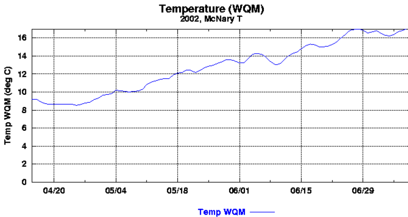
Figure 4. Temperature profile of McNary Forebay, the water source at the McNary Satellite Spawning Facility.
