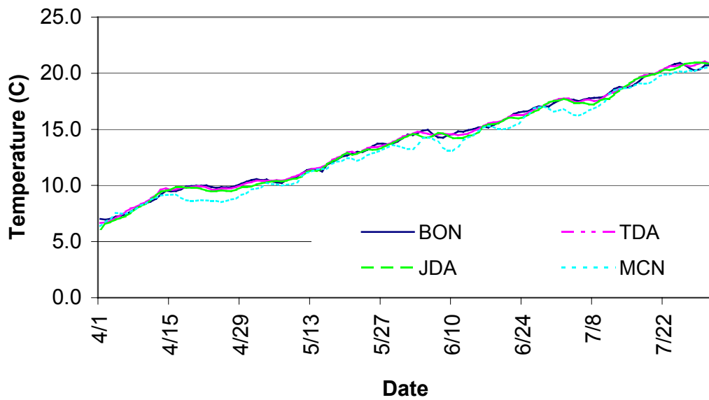
Figure 2. Water temperatures at Bonneville (BON), The Dalles (TDA), John Day (JDA), and McNary (MCN) dams during 2002. Data were obtained from the DART website ( http://www.cqs.washington.edu/dart/ ).
