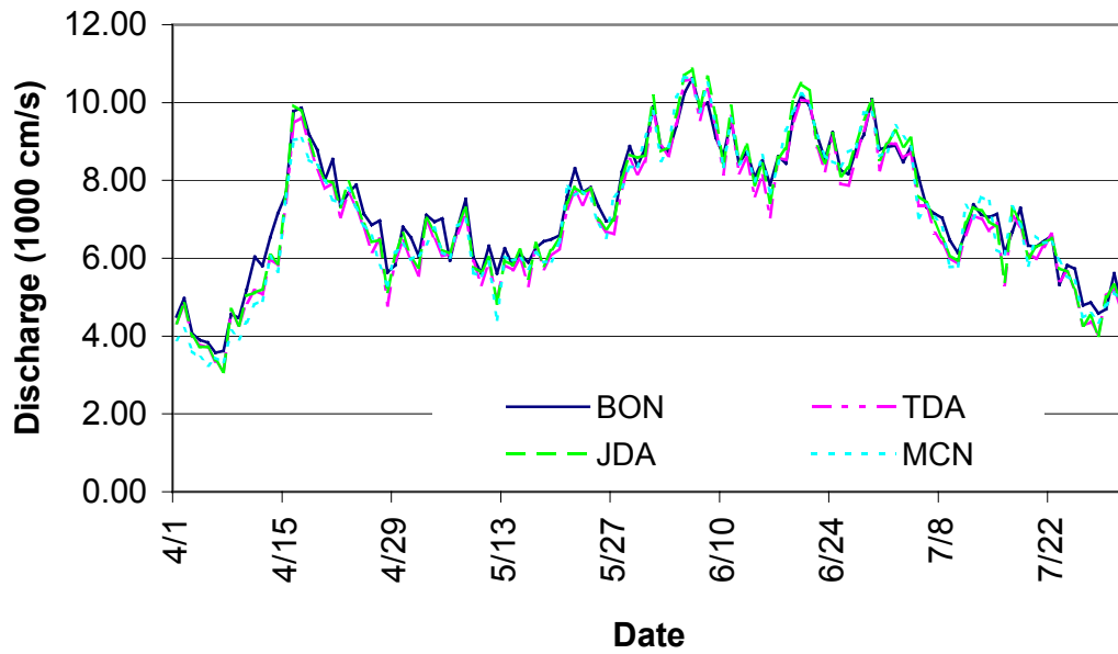
Figure 1. River discharges at Bonneville (BON), The Dalles (TDA), John Day (JDA), and McNary (MCN) dams during 2002. Data were obtained from the DART website ( http://www.cqs.washington.edu/dart/ ).
