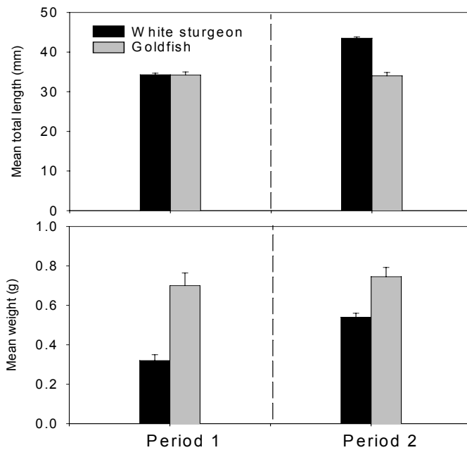
Figure 13. Mean total lengths and weights of white sturgeon and goldfish used in prickly sculpin predation trials during two periods. Each vertical bar equals one standard error. N = 18-20 for each prey type and period.
