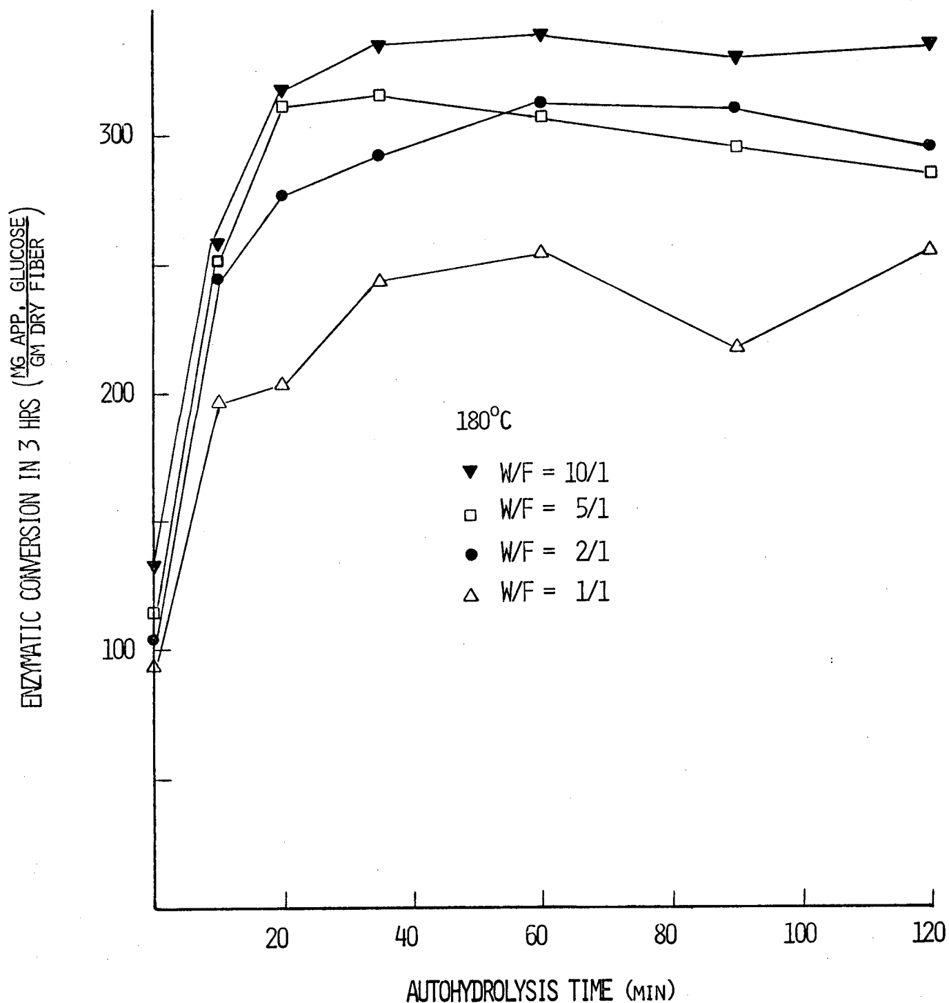
Figure 3. Production of reducing sugar during a standardized 3 hr enzymatic hydrolysis of autohydrolyzed wheat straw as a function of autohydrolysis time for materials treated at 180°C and various water/fiber (W/F) weight ratios. Yield is based on the dry weight of the autohydrolyzed straw.
