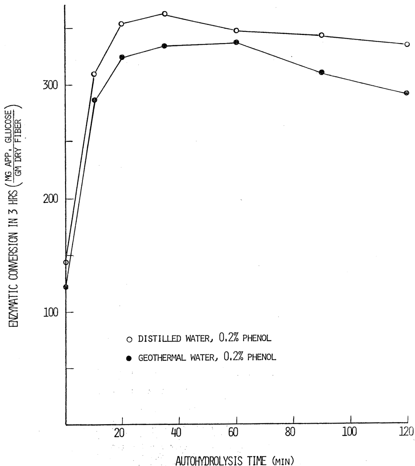
Figure 16. Effect of direct use of geothermal water in autohydrolysis of wheat straw at 180°C on the subsequent yield of reducing sugar during a standardized 3 hr enzymatic hydrolysis. The water/straw weight ratio during autohydrolysis was 5/1. Phenol addition is based on the original dry weight of the straw. Sugar yield is based on dry weight of autohydrolyzed straw.
