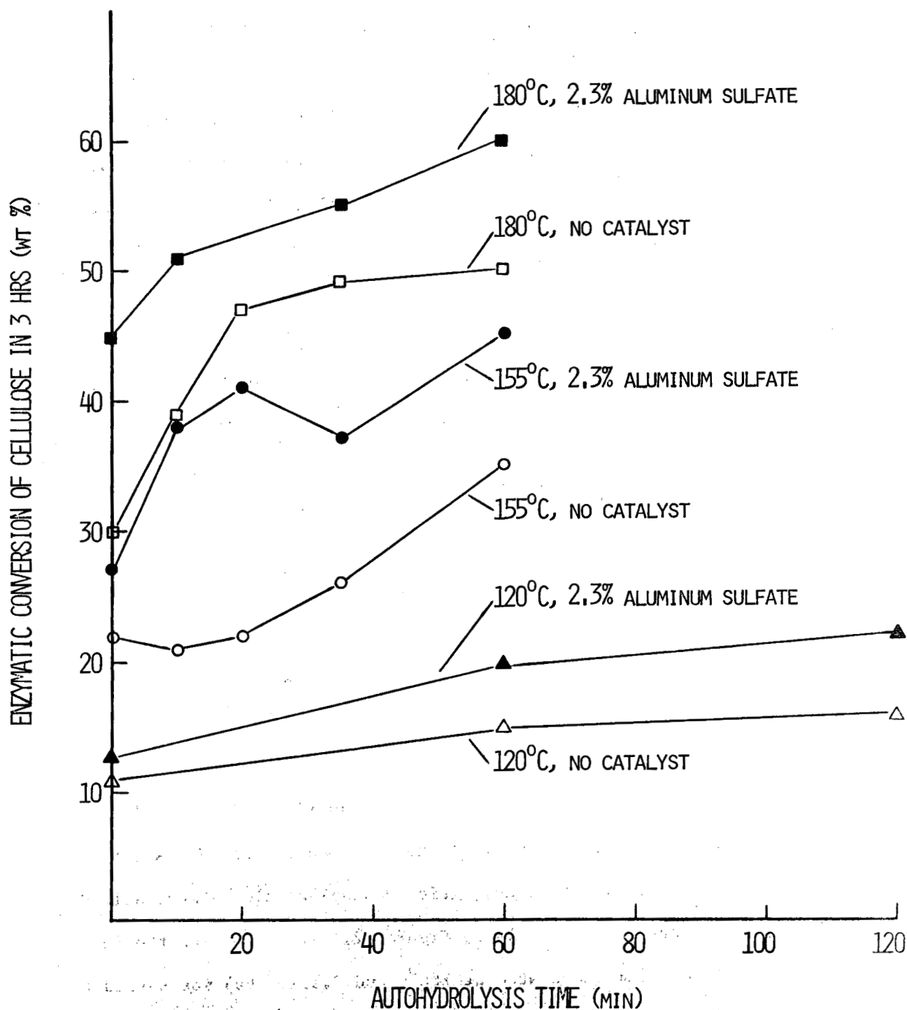
Figure 11: Fractional conversion of cellulose during standard 3 hr enzymatic hydrolysis of autohydrolyzed wheat straw as a function of autohydrolysis conditions. All autohydrolysis operations were carried out at a water/fiber weight ratio of 5/1. Fractional conversion was computed as 0.9(S/C) where S is the yield of reducing sugar as given in Figure 10 and C is the cellulose percentage at the start of enzymatic hydrolysis as given in Table 7. The factor 0.9 accounts for the water molecule added during hydrolysis.
