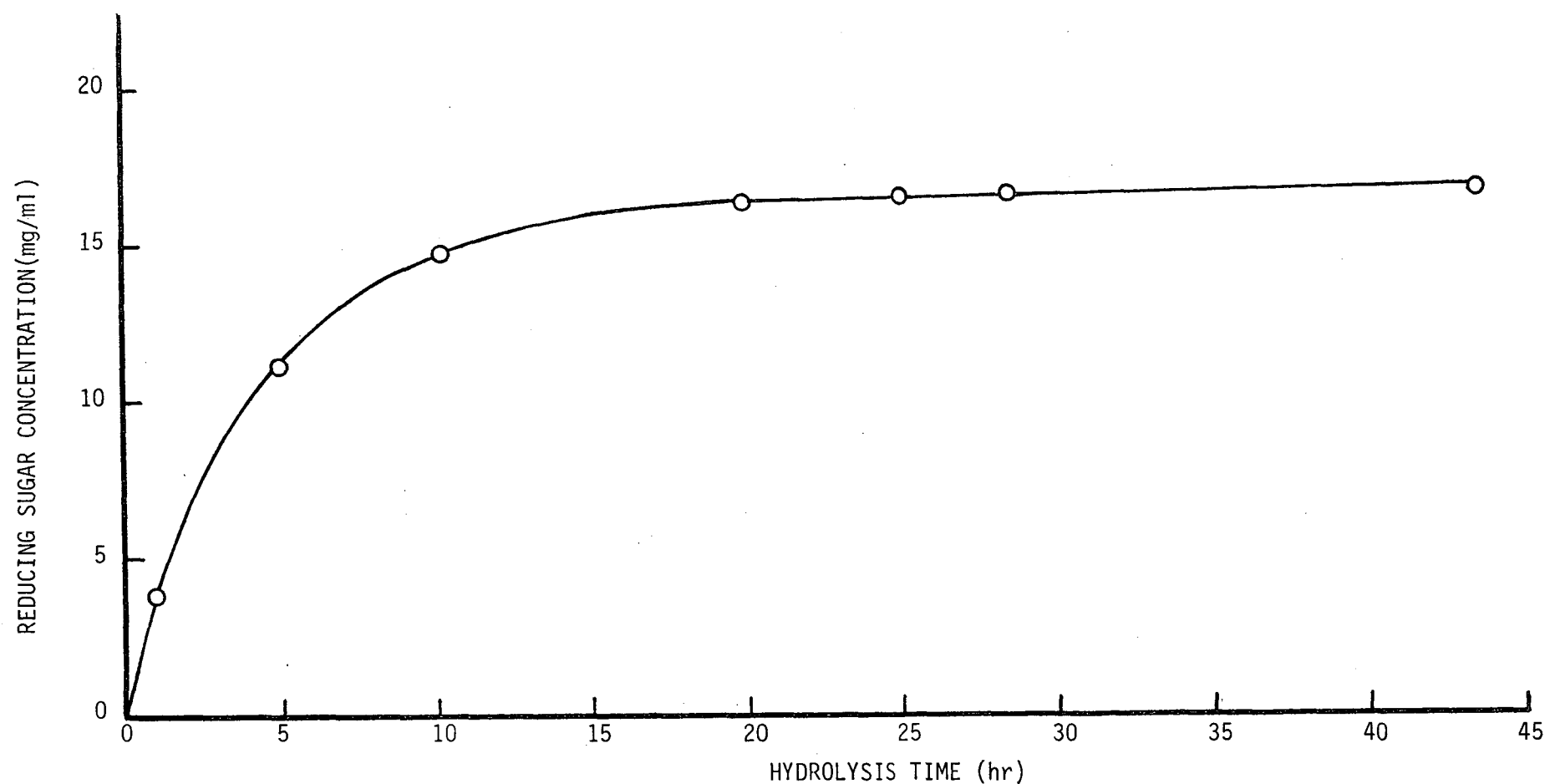
Figure 13. Reducing sugar concentration vs time for large-scale enzymatic hydrolysis of autohydrolyzed wheat straw. Autohydrolysis was carried out at 180^{\circ}\text{C} for 20 min with a water/straw weight ratio of 5/1 and 2.3% (based on dry weight of straw) aluminum sulfate added. Initial substrate concentration and enzyme/substrate ratio were 33 gm/liter and 43 IU/gm. Reducing sugar was determined by reaction with 3,5-dinitrosalicylic acid reagent. Values are given as glucose equivalents and are corrected for lactose present in enzyme preparation.
