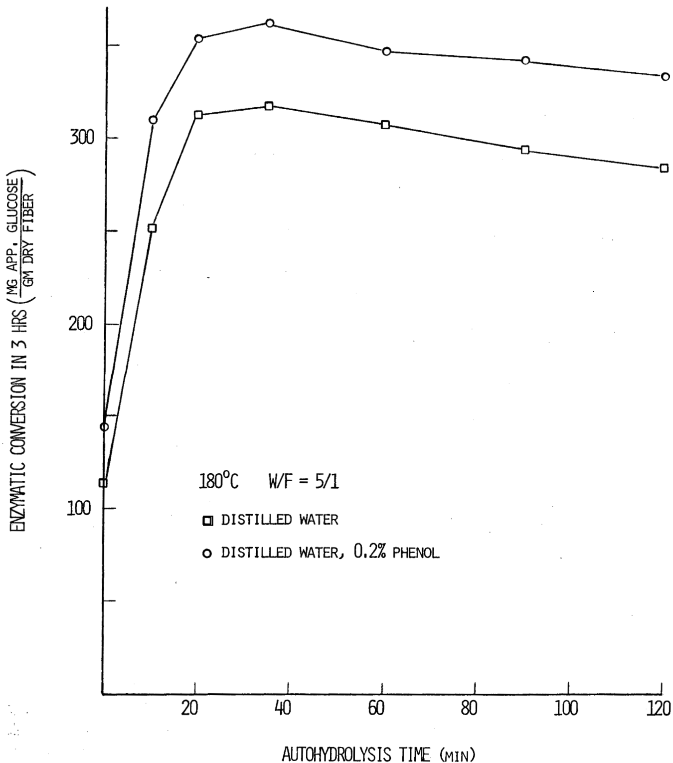
Figure 6. Production of reducing sugar during a standardized 3 hr enzymatic hydrolysis of autohydrolyzed wheat straw as a function of autohydrolysis time for materials treated in the presence of phenol. Autohydrolysis was conducted at 180°C and a water/fiber (W/F) weight ratio of 5/1. Phenol addition is based on the original dry weight of the straw. Sugar yield is based on the dry weight of the autohydrolyzed straw.
