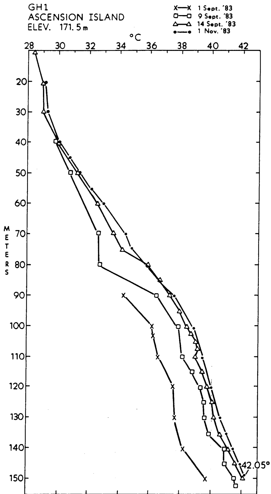
Figure 12. Temperature logs for GH-1. See Figure 3 for explanation of lithology symbols.
