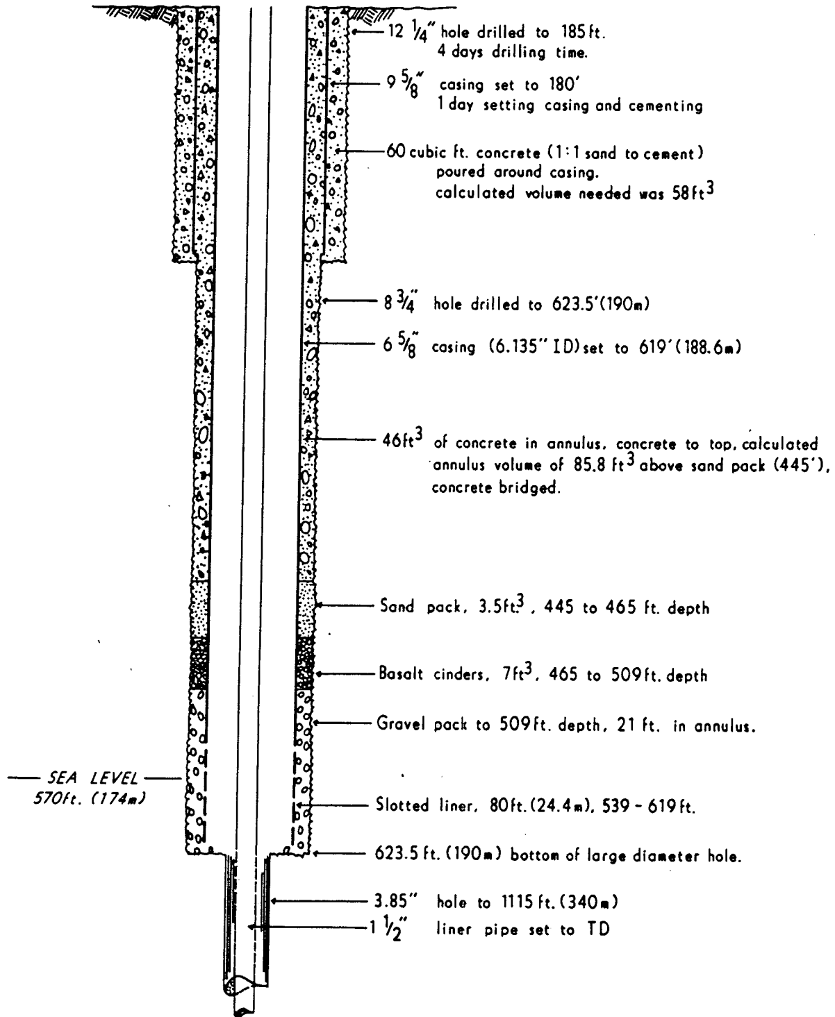
Figure 2. Completion diagram of LDTGH.
