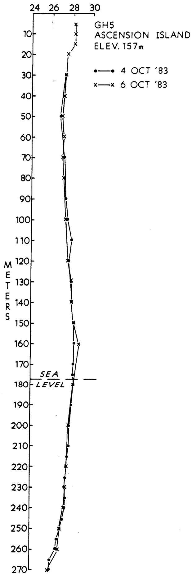
Figure 16. Temperature logs for GH-5.
