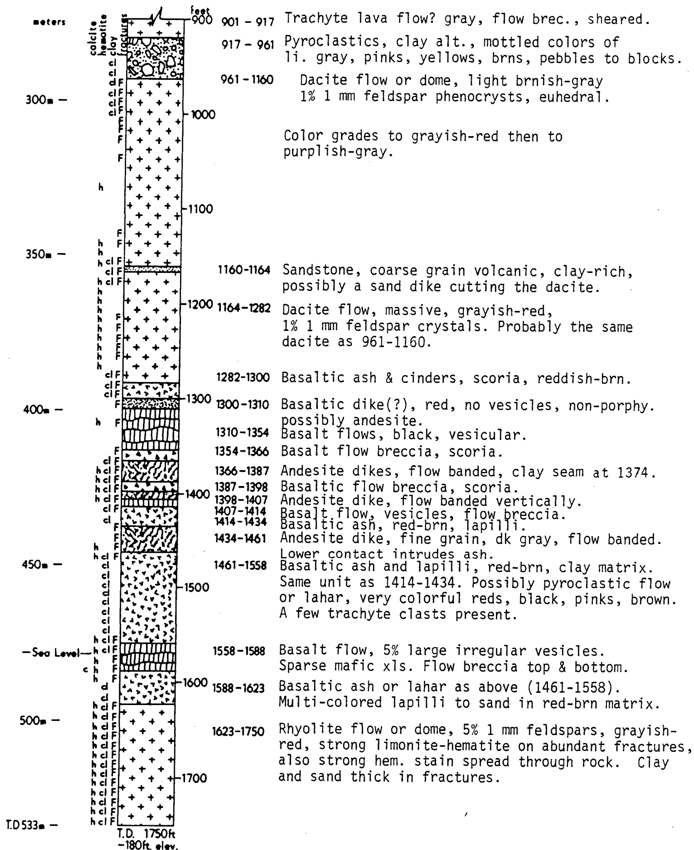
Figure 4 (continued). Lithologic log of GH2.
