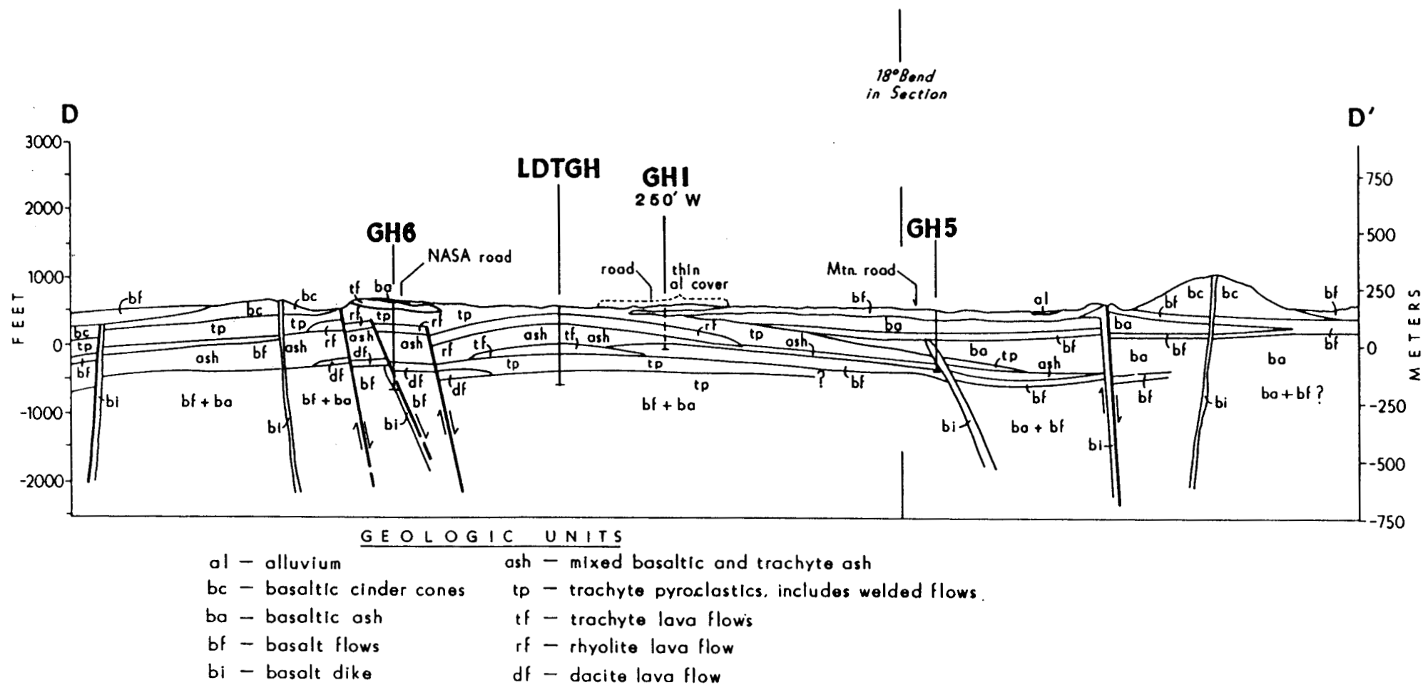
Figure 10. Cross section D-D' through holes GH5, GH6, and LDTGH, central part of the island.
