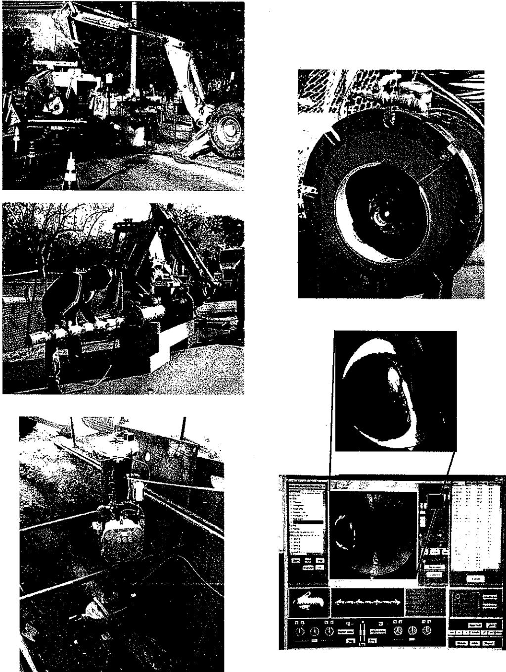
Figure 34: Live high-pressure steel main deployment images
