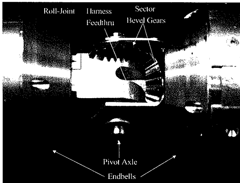
Figure 14: Explorer steering joint module design
