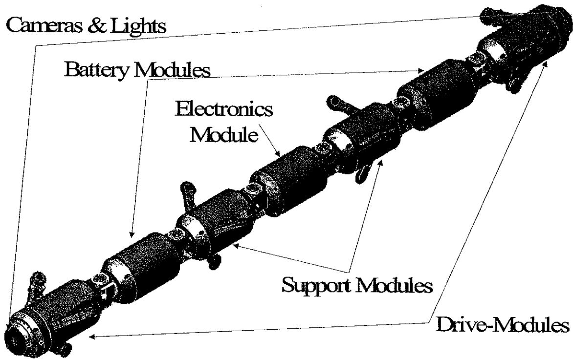
Figure 6 : Explorer Architecture CAD Design
