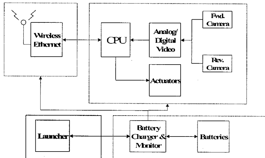
Figure 8 : Explorer overall electronics architecture
