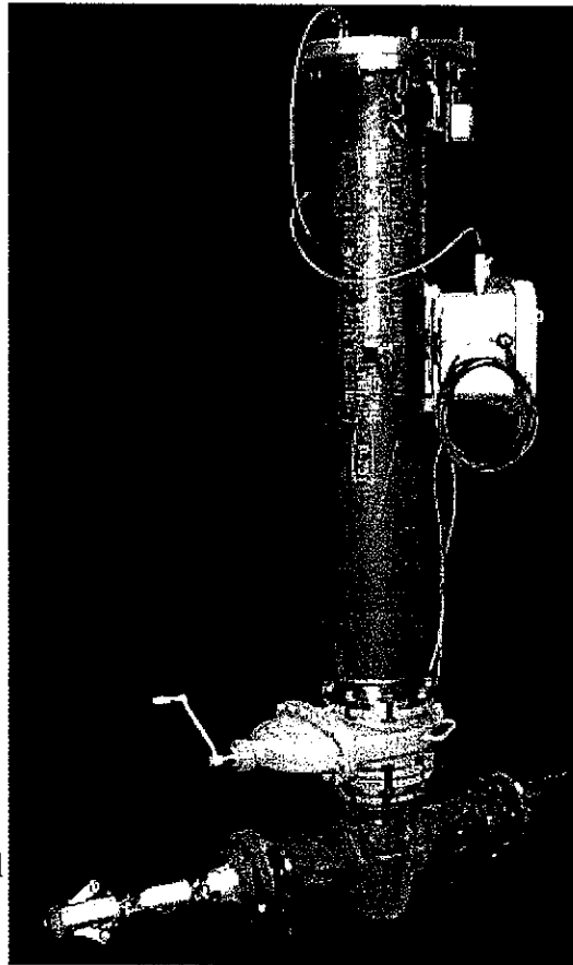
Figure 23 : Live-access launching hardware systems: Low-pressure CI and high-pressure steel
