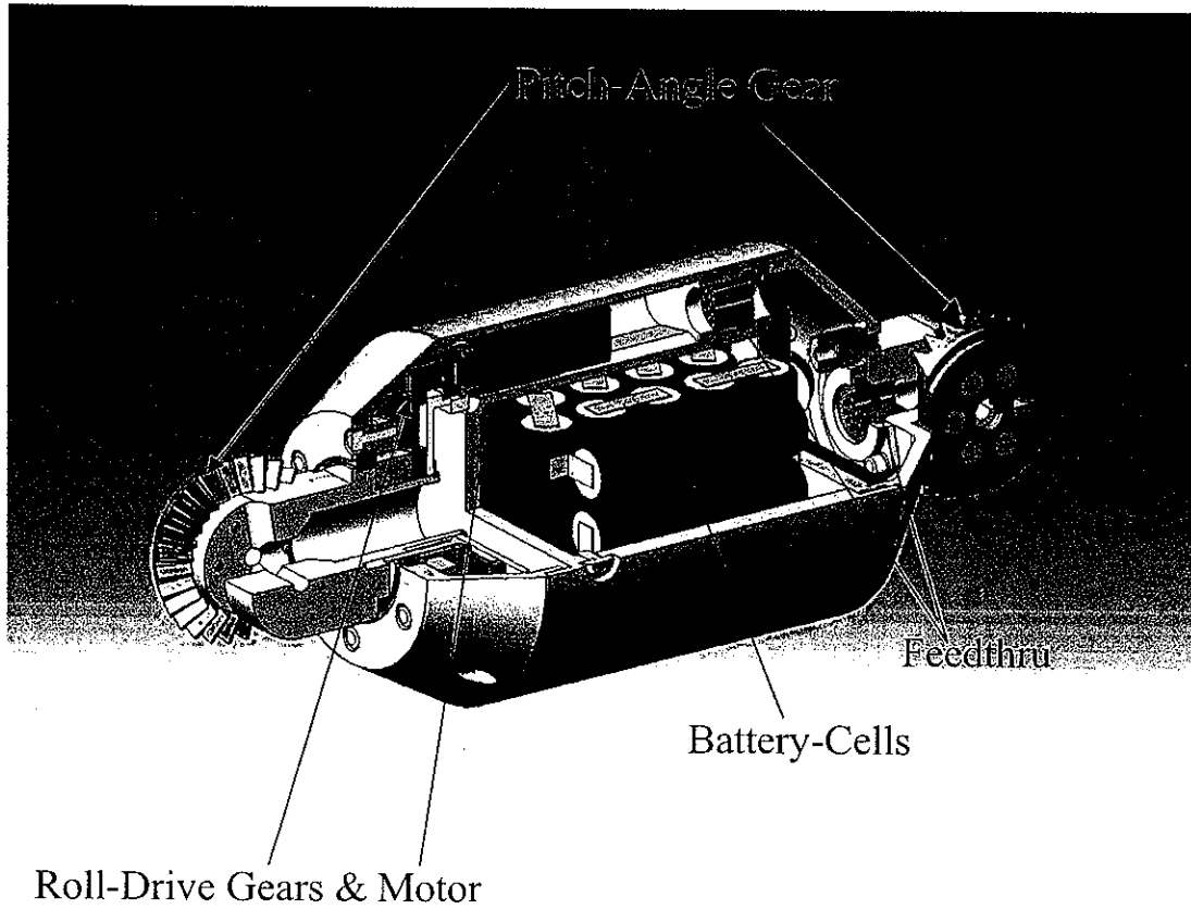
Figure 21: Cut-away CAD rendering of the battery-module
