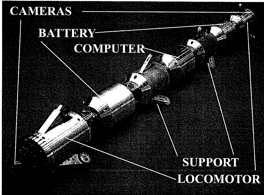
Figure 7 : Overall view of Explorer
