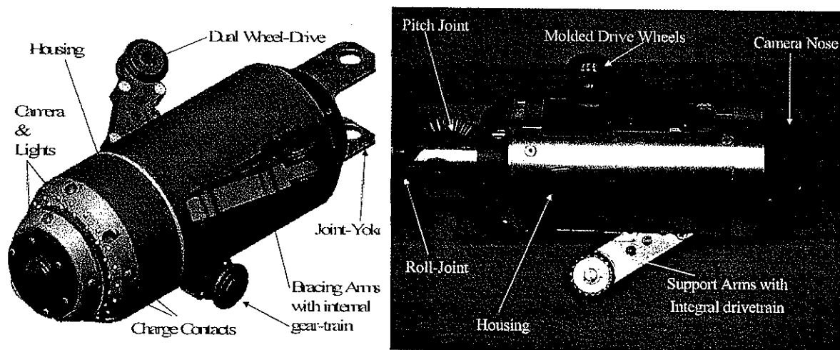
Figure 12: Explorer locomotor module design
