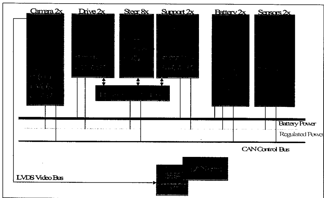
Figure 9 : On-board robot distributed electronics & functional architecture
