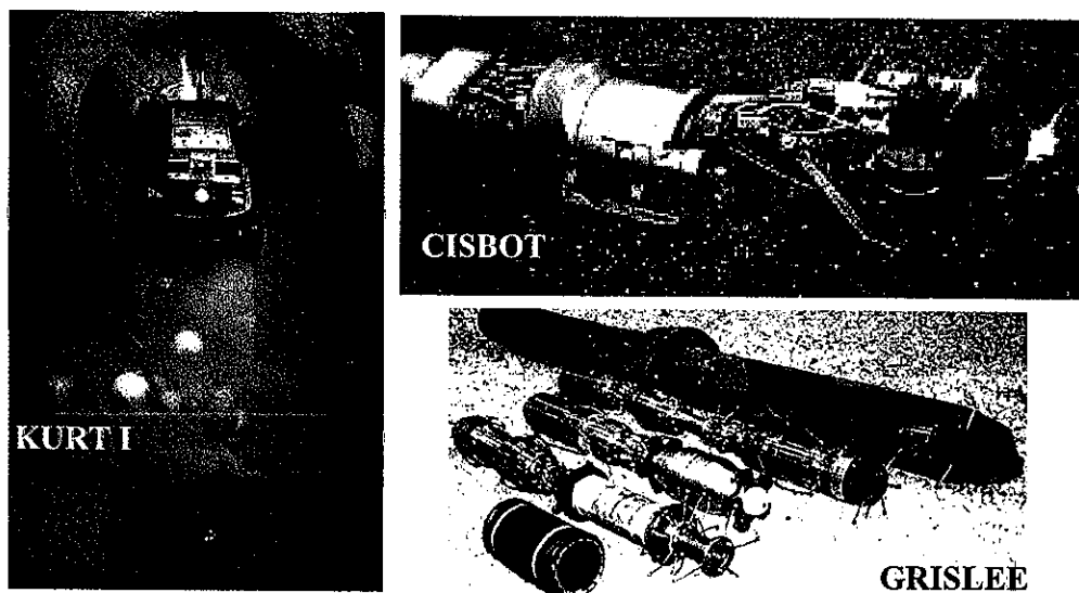
Figure 2: Tethered gasmain (CISBOT; GRISLEE) and untethered (Kurt I) robots
