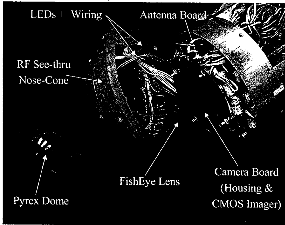
Figure 19: Explorer Camera-Nose internal assembly detail
