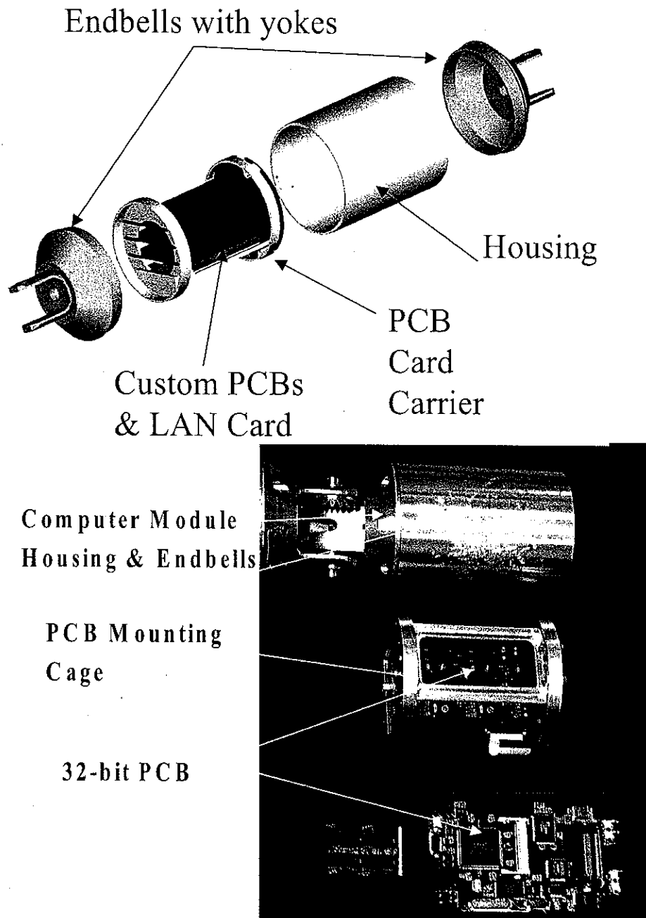
Figure 17: Explorer Electronics Module
