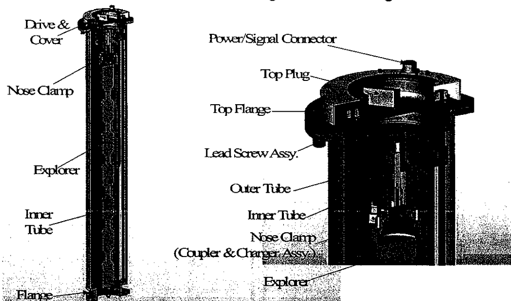
Figure 24 : CAD views of the high-pressure steel launcher
