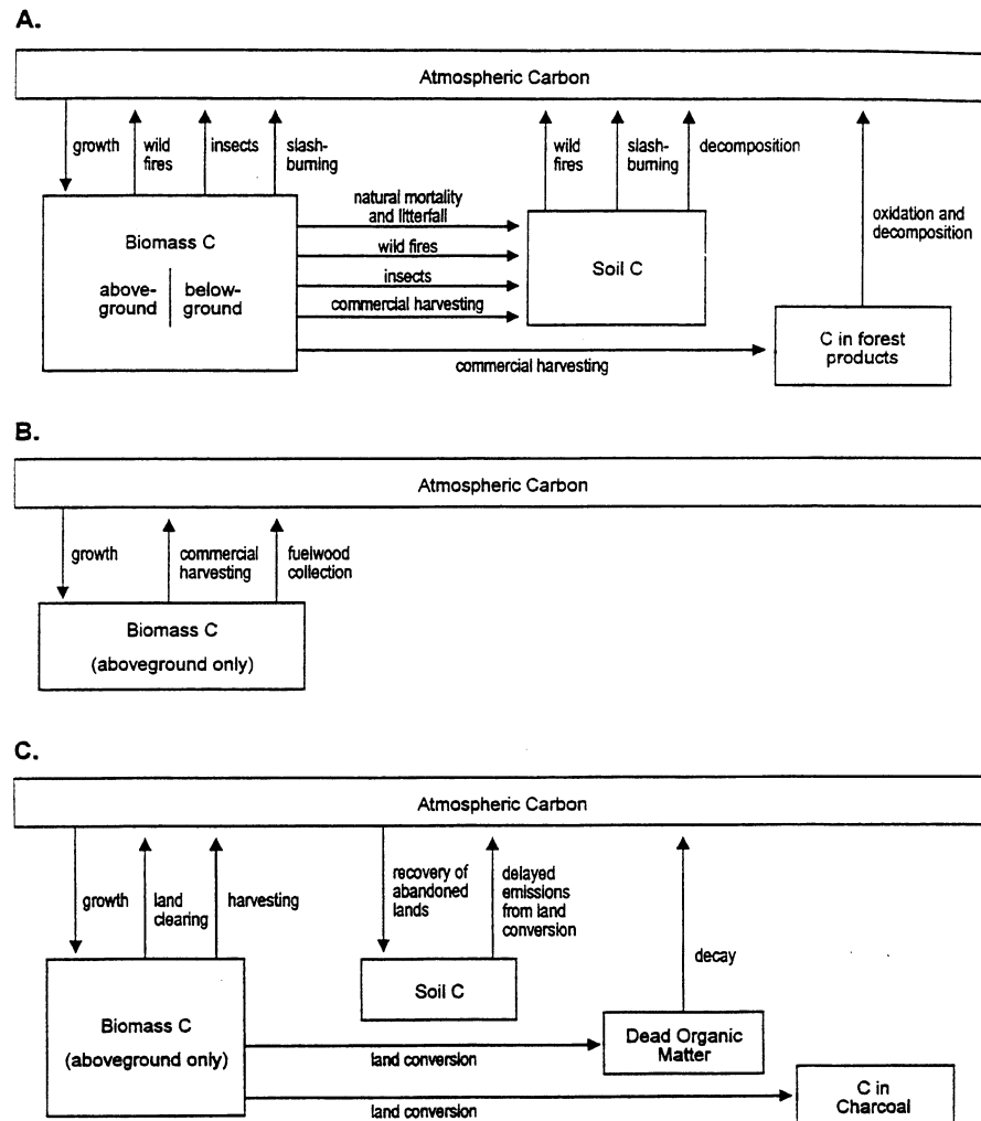
Figure 1. The carbon pools and carbon fluxes considered in each inventory methodology. In this figure, boxes represent “pools” of carbon, and arrows indicate possible carbon fluxes—the transfer of carbon between pools. The figure shows the pools and fluxes that are considered a) in the Carbon Budget Model of the Canadian Forest Sector; b) in the IPCC assessment of changes in “forest and other woody biomass stocks”; and c) in the IPCC assessment of the effects of land-use change. See text for further discussion.
