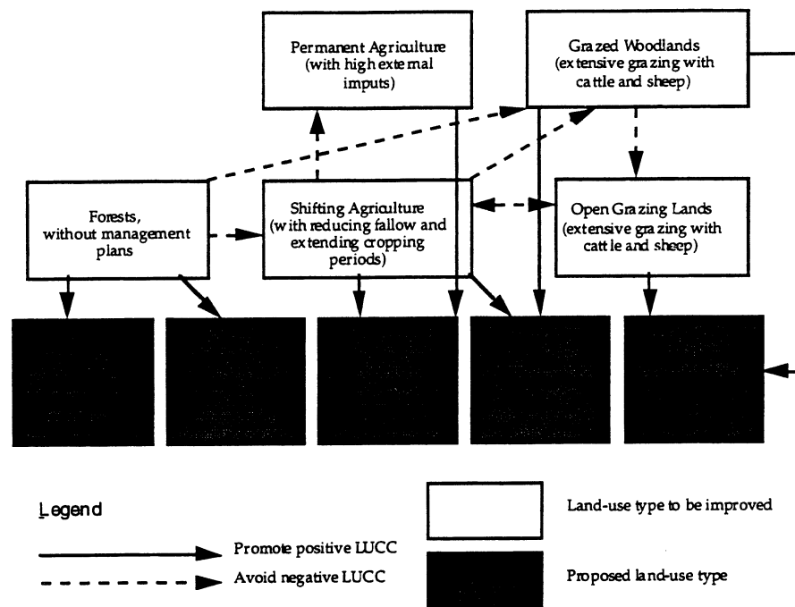
Figure 3. Current and proposed land-use change strategies, based on De Jong and Montoya (1994)
