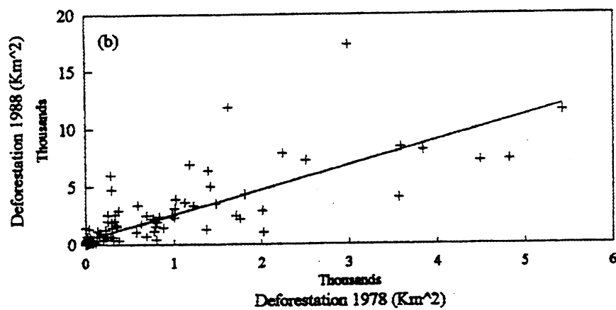
Figure 4. Persistence at the Amazon Basin wall-to-wall remote sensing derived data set. A reduction in the correlation coefficient ( r^2 ) is a measure of a regional deforestation trend.
