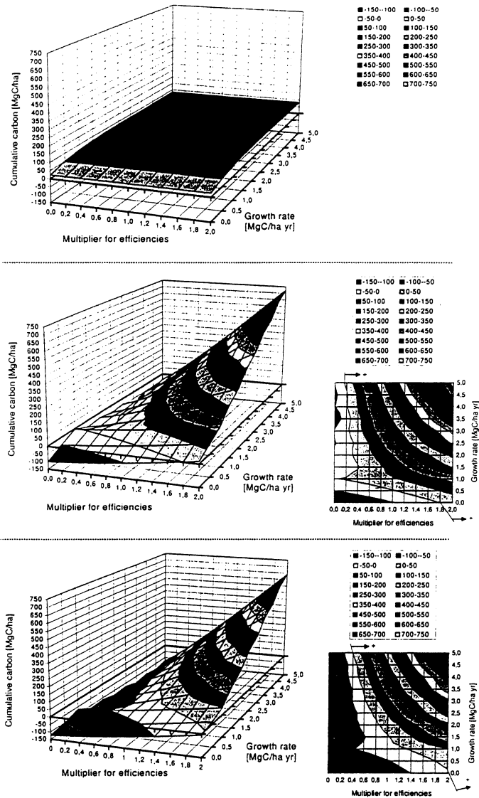
Figure 3. Sensitivity of the results to changes in growth rate and efficiencies. Figure 3a (upper diagram) shows the net cumulative C mitigation after 100 years for the forest protection scenarios. Values of net cumulative C mitigation are shown as a function of the forest growth rate and the “efficiency” with which forest products are harvested and used, as defined in the text. The accumulation of C in soil and litter is taken from the base-case scenario and is not dependent on the forest growth rate. Figure 3b (middle diagram) shows the net cumulative C mitigation after 100 years for a sustainable, forest-harvest scenario. The insert shows a contoured, two-dimensional representation of net cumulative carbon mitigation to make it easier to see the location of the zero contour. Figure 3c (lower diagram) shows the difference between the scenarios of Figure 3a and 3b. Values for net cumulative C mitigation for scenario 1 (Figure 3a) are subtracted from corresponding values for scenario 2 (Figure 3b). As in Figure 3b, an insert is provided to help characterize the location of the zero intercept. The zero contour line separates regions where mitigation is greater for the forest protection scenario (negative values in the figure) from those in which sustainable harvest yields greater mitigation (positive values of cumulative C).
