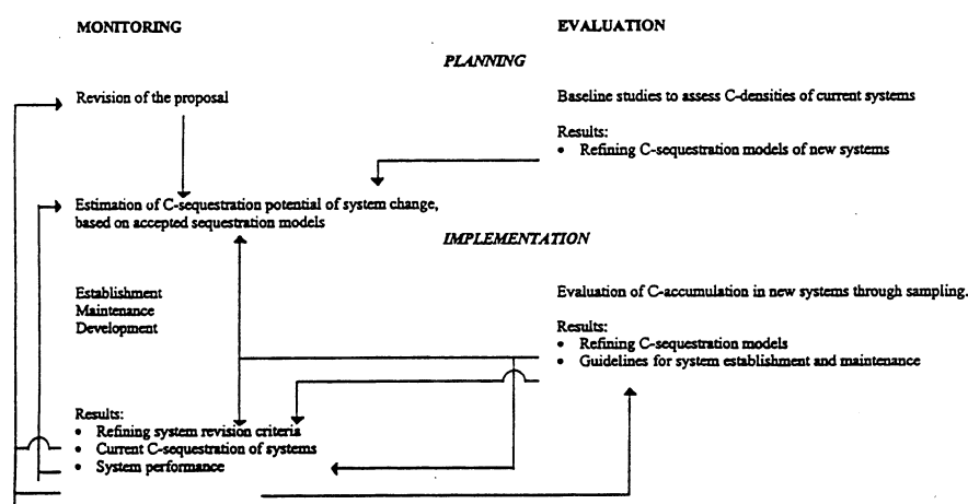
Figure 4. Information flows between monitoring and evaluation results for carbon sequestration estimation.
