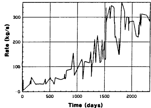
Figure 2. Rate of production with time.
