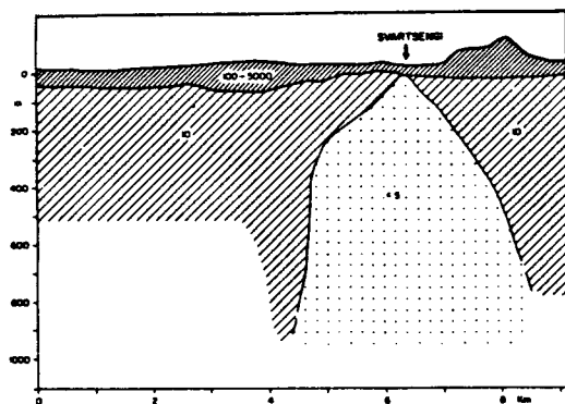
Figure 4. Resistivity cross-section.
