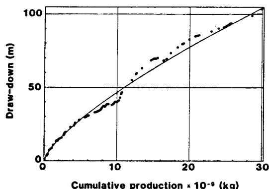
Figure 7. Empirical match to production data.
