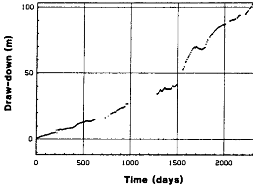
Figure 3. Draw-down with time.
