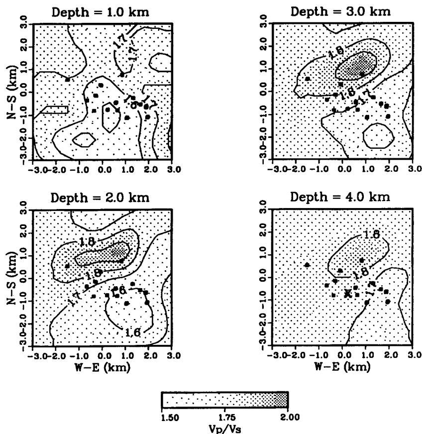
Figure 6. NW Geysers, 3-D V_p/V_s structure at several depths; datum: 700 masl. Solid circles correspond to wellhead locations. Well PRATI-8 is indicated by the X in the lower right figure. Note the anomalously low V_p/V_s within the producing horizon and the high V_p/V_s anomaly north of the CCOC area (from Romero et al., 1992).
