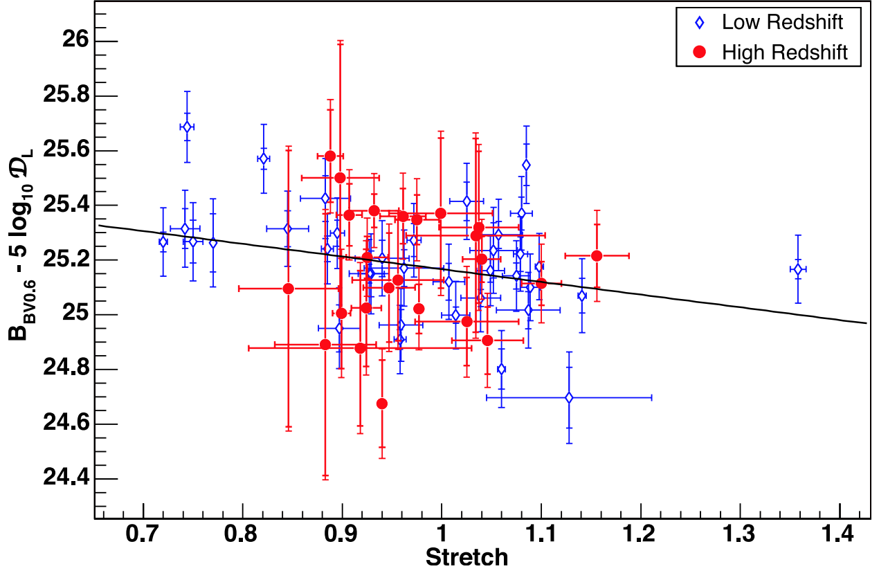
Fig. 9.— Stretch-luminosity relationship for the low redshift SNe (open diamonds) and high redshift SNe (filled circles). Each point is B_{BV0.6} minus the c/H_0 free luminosity distance of equation 3, plotted against the stretch of the SN. The line represents the fit estimates for \alpha and \mathcal{M} from the primary fit ( \alpha = 0.52 , \mathcal{M} = 25.17 ). The outer error bars include 0.12 magnitudes of intrinsic scatter.
