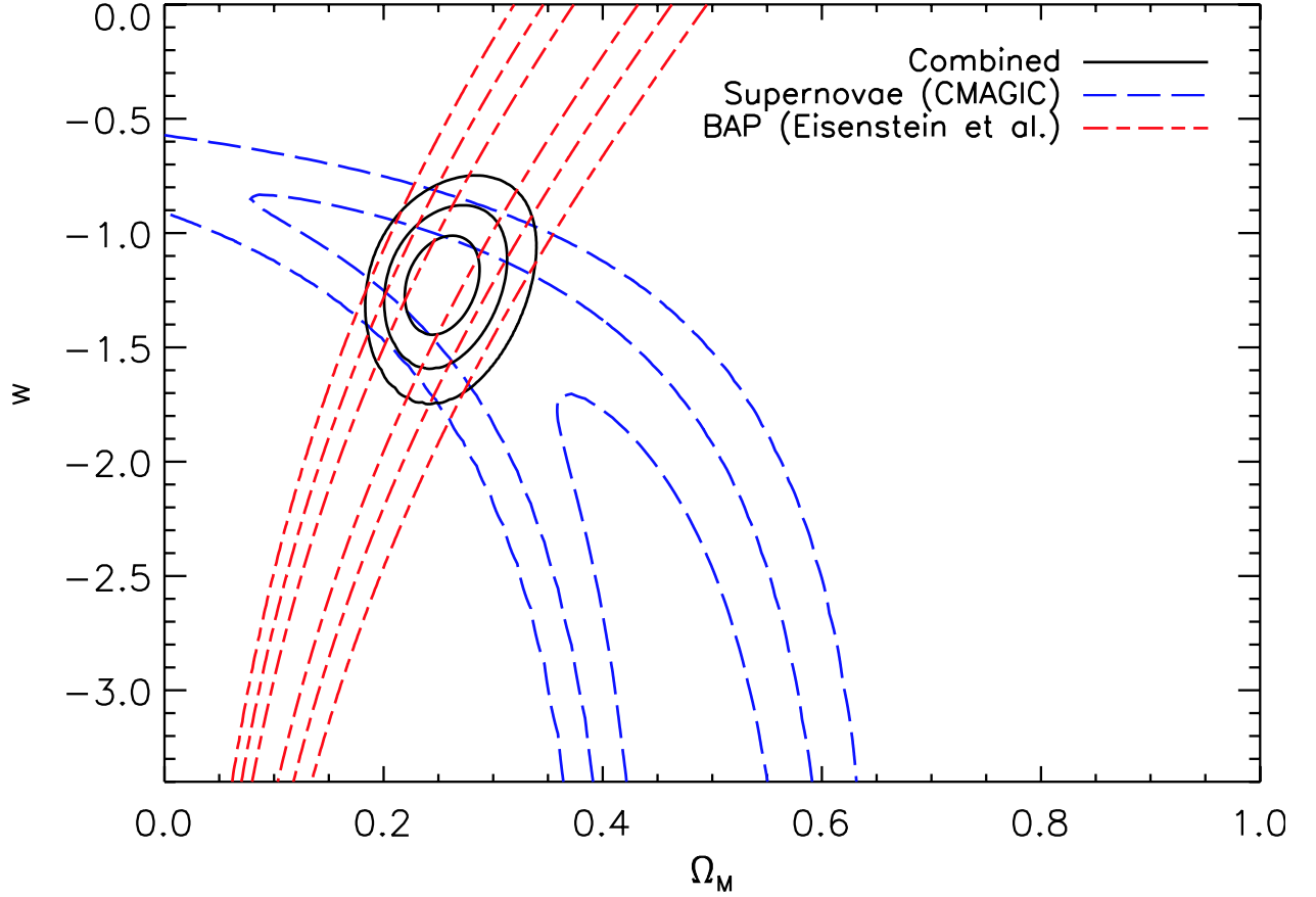
Fig. 10.— Confidence regions for w , \Omega_m assuming a flat universe. The contours represent 68.3%, 95.4%, and 99.7% of the total probability. Both the constraints from the CMAGIC analysis of supernovae and the baryon acoustic peak (BAP) of Eisenstein et al. (2005) are shown, as are the contours that result from combining the two measurements. A cosmological constant corresponds to w = -1 .
