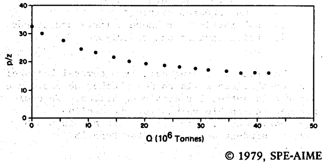
FIG. 15b. p/z vs Q—Larderello data (from Brigham & Neri, 1979).
