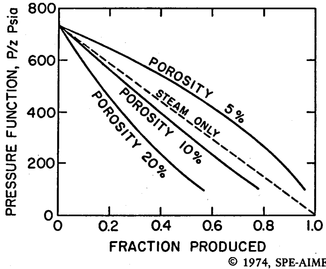
FIG. 11. Pressure depletion vs recovery, falling liquid level (from Brigham & Morrow, 1974).
