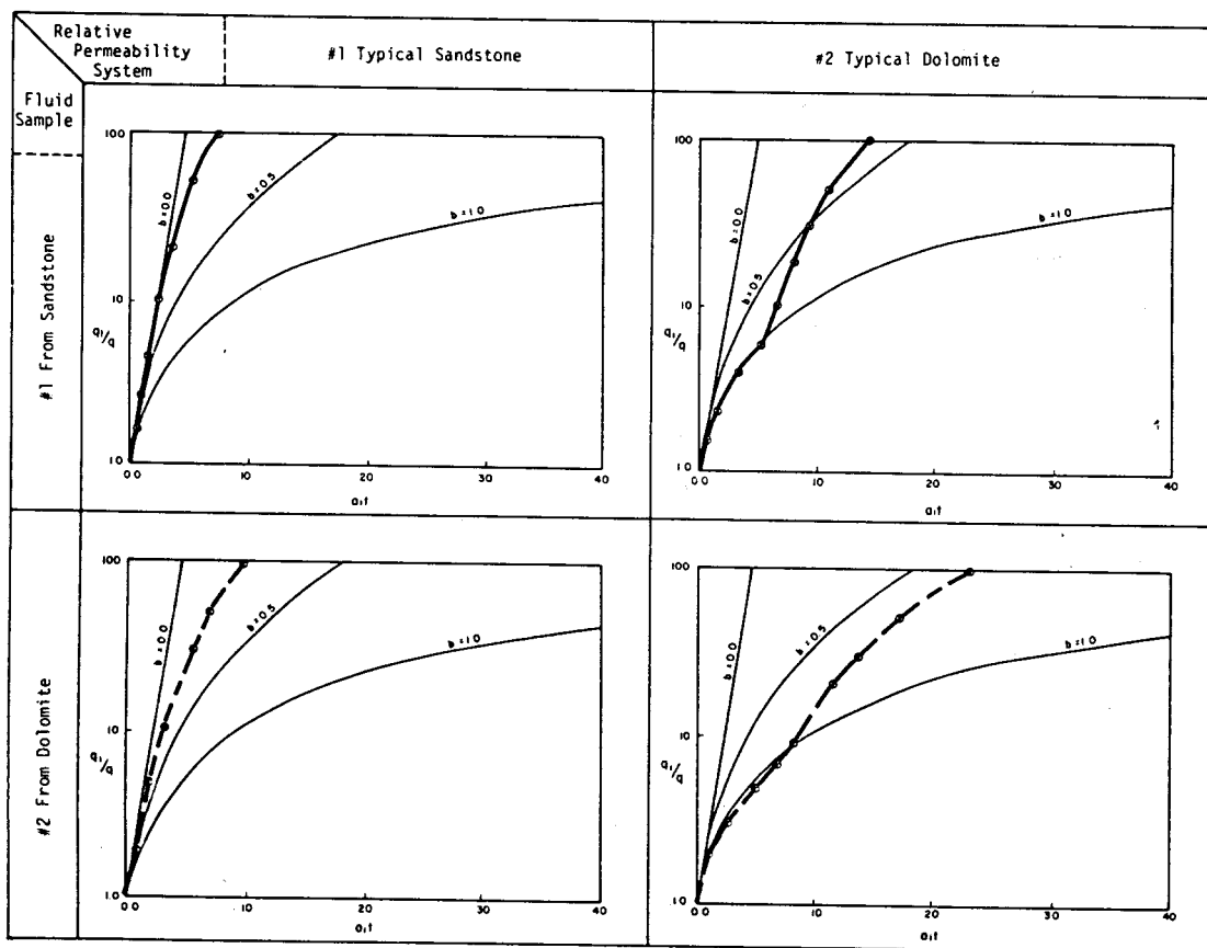
FIG. 9c. Dimensionless a_i t curve histories for four fluid-permeability systems (after Gentry & McCray, 1978). © 1978, SPE-AIME
