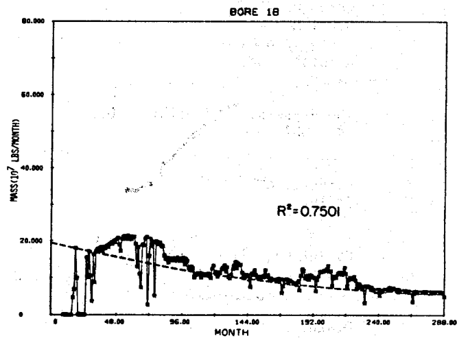
FIG. 17f. Bore 18, Wairakei, New Zealand.
