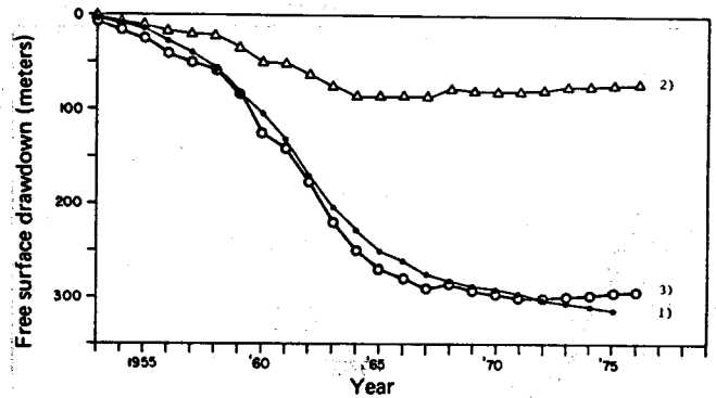
FIG. 21. Linearized free surface fits to Wairakei data. Curve 1, ●—●: observed pressure drawdown Curve 2, △—△: LFS fit, 1 term Curve 3, ○—○: LFS fit, 2 terms
