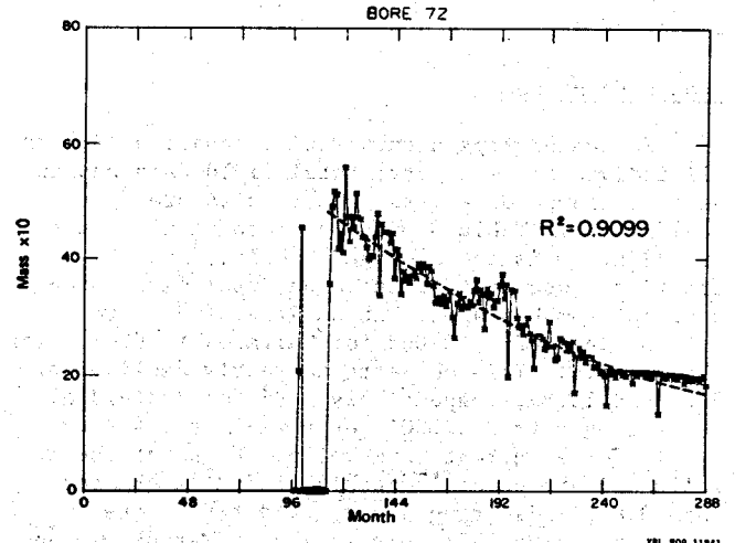
FIG. 17d. Bore 72, Wairakei, New Zealand.
