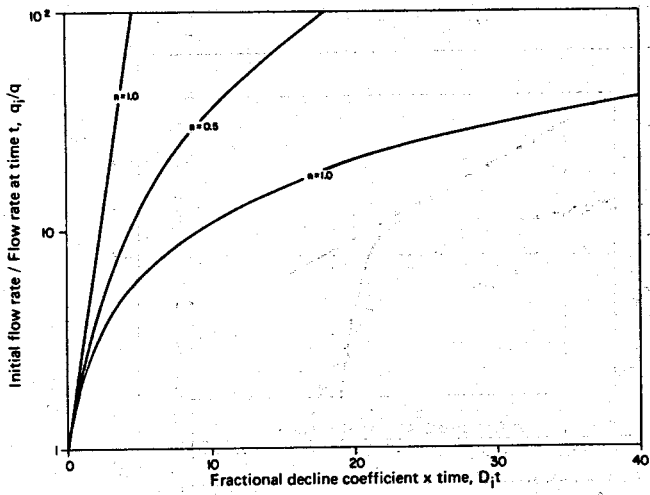
FIG. 8a. Decline curve analysis chart relating production rate to time (after Gentry, 1972).
