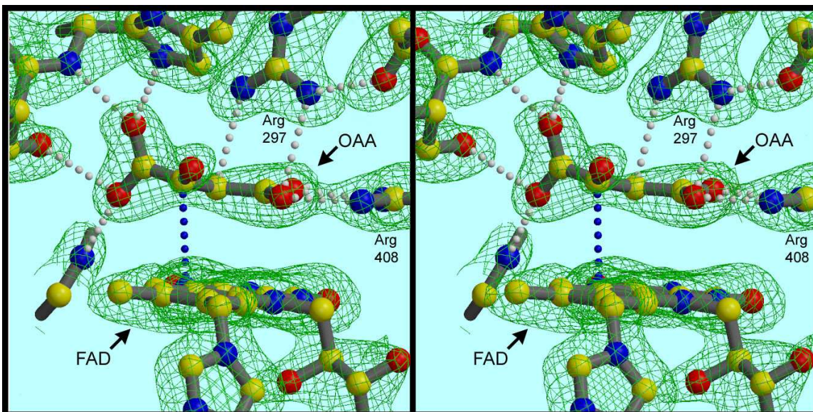
Figure 2. The dicarboxylate site and its ligand in the untreated enzyme. The occupant is nonplanar, suggesting that if oxaloacetate it is highly strained. Note the H-bond between C2 of the ligand and catalytic base Arg297, and the close approach of C3 to the flavin N5 atom (blue dotted line). Essentially the same arrangement was seen when crystallization was carried out in the presence of excess OAA. The density is a 2F_o - F_c map contoured at 1.7 \sigma .
