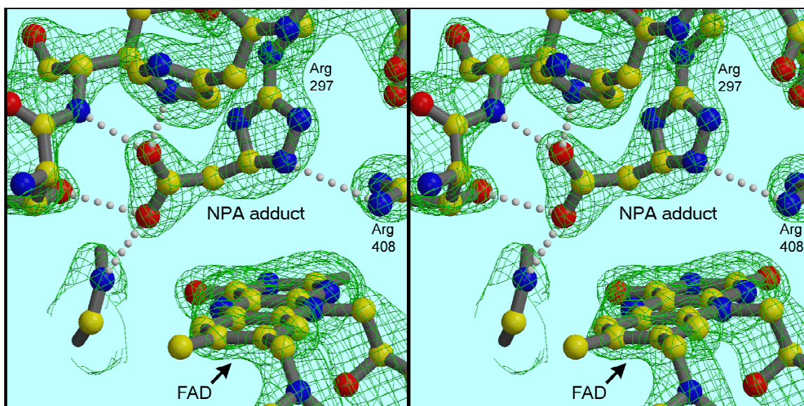
Figure 4. The dicarboxylate site in the 3-NP-treated enzyme. The density attributed to the ligand has shrunk and moved away from the flavin toward Arg297 and His253. It can be modeled by assuming two atoms from the backbone of 3-NP (C3 and N) fuse with the guanidino group to form a 5-membered ring, with loss of the two nitro oxygens. The carboxylate at the other end fits into the clearly forked density branching off the ring.
