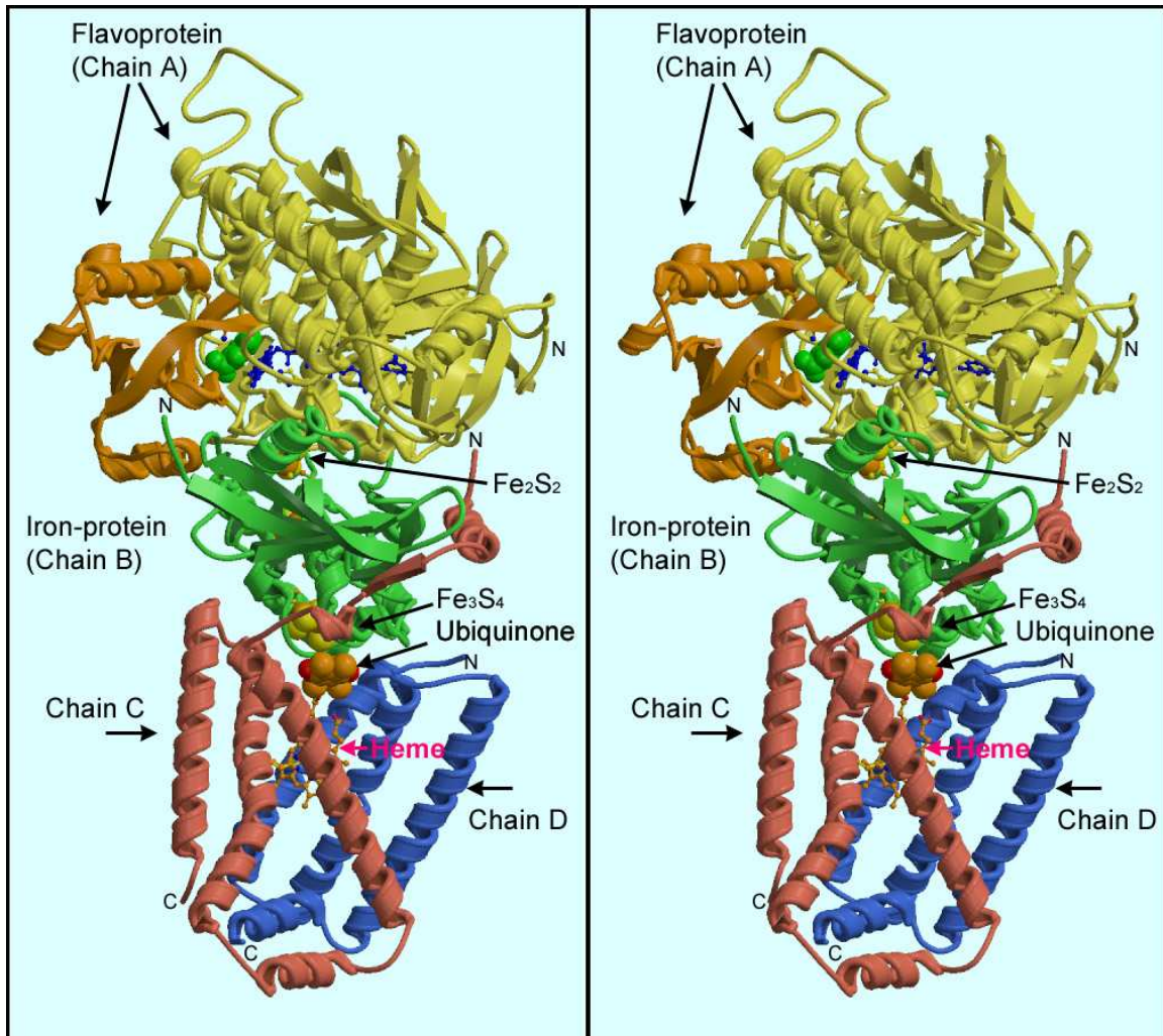
Figure 1. Overall structure of mitochondrial complex II. The stereo ribbon diagram is colored yellow & brown (flavoprotein), green (iron protein), pink (large anchor polypeptide, chain C), and blue (small anchor peptide, chain D). The CAP domain of the FP is colored brown. The green spacefilling model at the intersection between the CAP domain and the rest of the FP is the malate-like ligand, and the extended blue ball-and-stick model starting just to the right of that is the FAD cofactor. Note the first helix of anchor peptide (chain C) packs against a helix of the IP.
