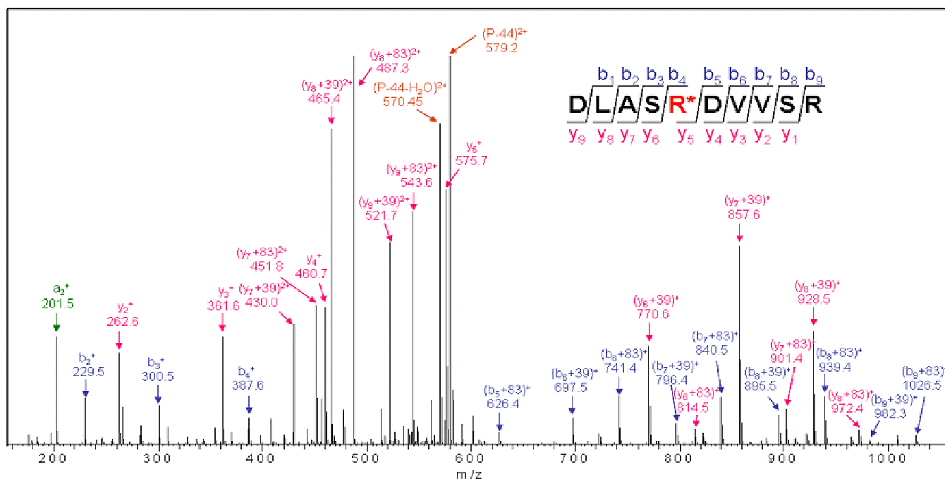
Figure 5. LTQ linear ion trap tandem mass spectrum obtained from fragmenting 3-NP modified peptide DLASR*DVVSR. The doubly charged precursor ion of m/z 600.9 corresponds to a mass increment of 83 Da. This peptide was present in the digest of the 3-NP-treated sample but not the control. The peaks can be assigned as "b" and "y" fragments of the indicated sequence (corresponding to D293 – R302 of the mature flavoprotein sequence, and including the modified catalytic base R297) if it is assumed that R297 has an additional mass of 83 Da or 39 Da, consistent with the proposed adduct (NCCCO 2 ) or its decarboxylation product (NCC). Peaks corresponding to the decarboxylation (P-44) and dehydrated decarboxylation (P-44-H 2 O) products of the parent peptide (P) are also indicated.
