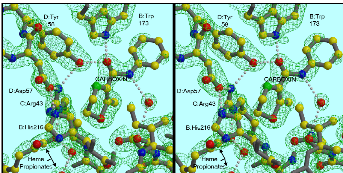
Figure 6. Binding mode of carboxin, and a H-bonded network involving heme propionate and residues from three subunits. The carbonyl oxygen of the inhibitor is H-bonded to Tyr58 of chain D and Trp173 of chain B. D:Tyr58 is also H-bonded to C:Arg43 which makes H-bonds with a heme propionate and with D:Asp57. The latter H-bonds B:His216. The density is a 2F_o - F_c map contoured at 1.8 \sigma .
