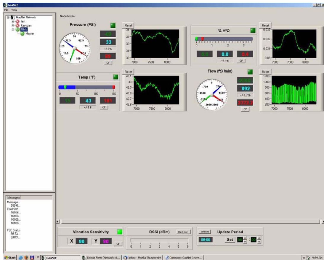
Figure II-20: GUI screen-capture layout showing real-time single-node data
