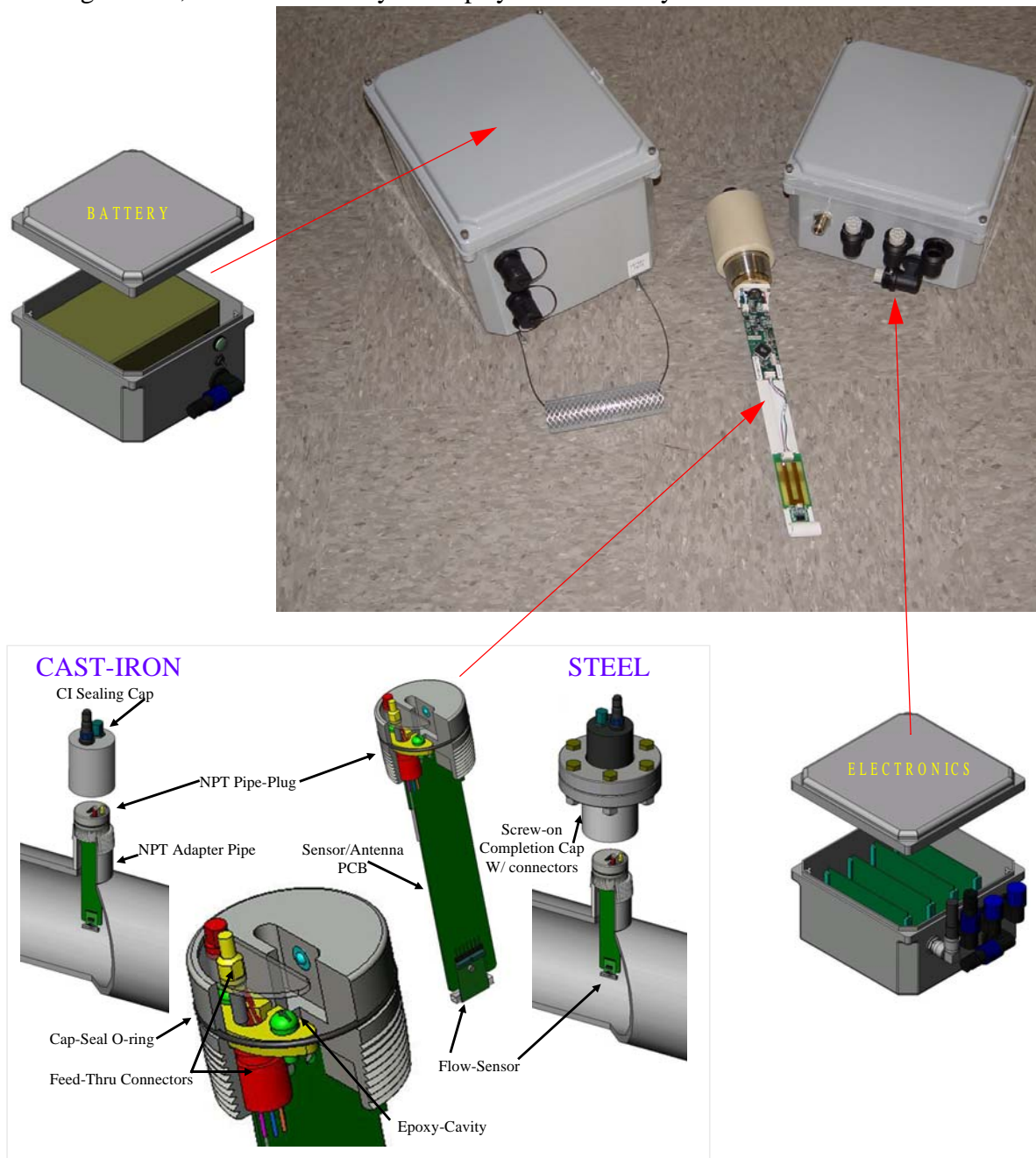
Figure II-5: GasNet™ System Overview and as-built ready-to-ship assembly
