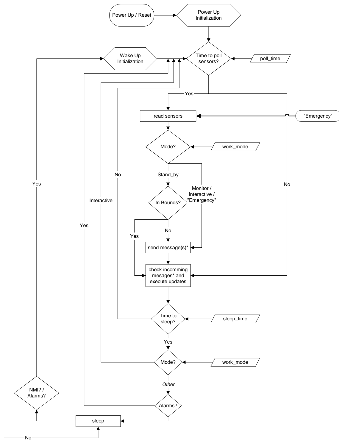
Figure II-22: Software mode flow chart diagram
