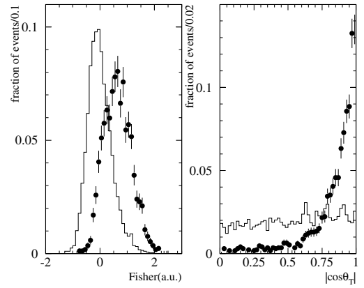
FIG. 2: Distribution of the discriminating variables |\cos\theta_T| and \mathcal{F} in the B^+ \rightarrow D^+ K_s^0 signal MC (histograms) and the off-resonance data (dots).
