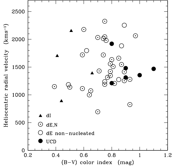
Fig. 12.— The velocities of Fornax Cluster galaxies plotted against their (B-V) color indices. The heliocentric radial velocity is taken from the NASA Extragalactic Database. The (B-V) color is taken from Karick, Drinkwater & Gregg (2003). Galaxies are distinguished according to their morphological types in the Fornax Cluster Catalog (Ferguson 1989). dI here includes galaxies classified as spirals in the FCC having M_B > -16 mag. The UCDs from this paper and from Phillipps et al. (2001) are shown as solid circles.
