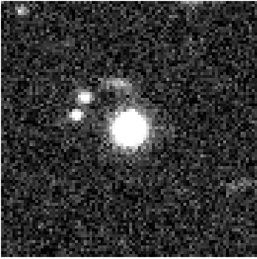
Fig. 13.— A CCD image of Virgo UCD 6. A 30'' \times 30'' region around UCD 6 is shown based on a 25 min B-band integration with the Isaac Newton Telescope in 1''.1 seeing.
