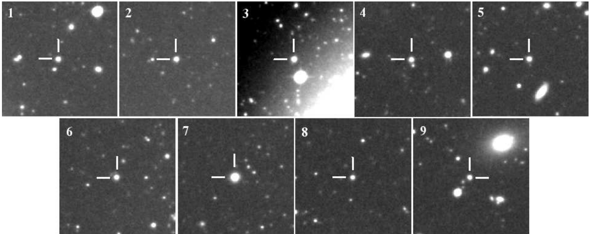
Fig. 6.— Images of the nine Virgo Cluster UCDs from the stack of 56 UKST red band films. Each frame is 2.0 arcmin wide and north is at the top. The UCD is centered in each frame.
