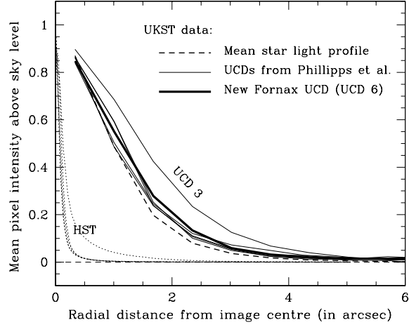
Fig. 10.— Radial light intensity profiles for Fornax Cluster UCD6 derived from a Super-COSMOS scan of a UKST red Tech Pan film. The profiles of the five UCDs of Drinkwater et al. (2000a) and a mean star point-spread function from the same UKST data are shown for comparison, taken from Phillipps et al. (2001). Resolved profiles from the Hubble Space Telescope STIS data of Drinkwater et al. (2003) are shown for the first 5 UCDs to illustrate the effects of seeing on the UKST images.
