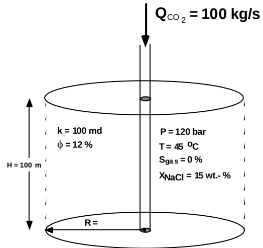
Figure 4. Schematic of radial flow problem.
