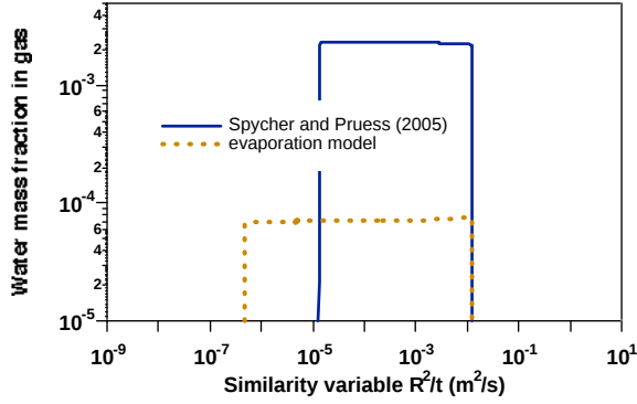
Figure 5. Simulated water mass fraction in \text{CO}_2 -rich phase.
