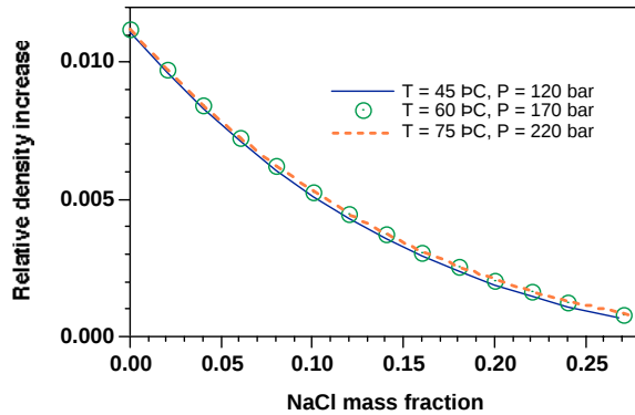
Figure3. Relative increase in aqueous phase density from CO 2 dissolution, as a function of salt concentration.
