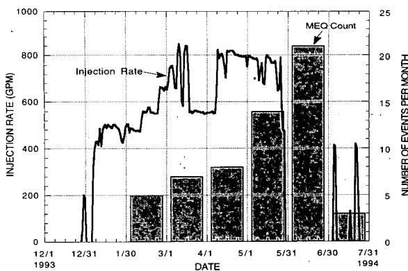
Figure 4. Comparison of DV-11 injection rate and seismicity in the surrounding 2400- \times 2400-ft (0.73- \times 0.73 km) area. MEQ count is based on U-N-T data, because of some down-time of the LBL network during the period shown.
