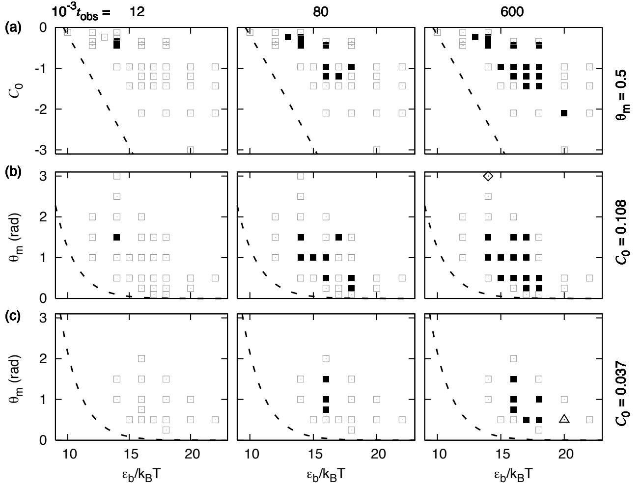
FIG. 6: Changing model parameters reveals the kinetic phase diagram for design B 3 . Filled points denote parameter values for which 30% of subunits are in complete capsids ( f_c \geq 30\% ) by the observation time, t_{\text{obs}} , open points indicate parameter values for which f_c < 30\% , and the dashed lines indicate the location of the thermodynamic critical surface, calculated with Eq. 16. The first, second, and third columns correspond to observation time t_{\text{obs}} = 1.2 \times 10^4 , 8 \times 10^4 , and 6 \times 10^5 , respectively. The top row (a) shows cross-sections through C_0 and \epsilon_b with \theta_m = 0.5 . The second and third row show cross-sections through \theta_m and \epsilon_b , with (b) C_0 = 0.11 and (c) C_0 = 0.037 . In each case the region covered by filled points roughly defines a cross-section of parameter space within which assembly is kinetically possible. Simulation snapshots corresponding to the \diamond in the right hand panel in row (b) and the \triangle in the right hand panel in row (c) are shown in Fig. 7.
