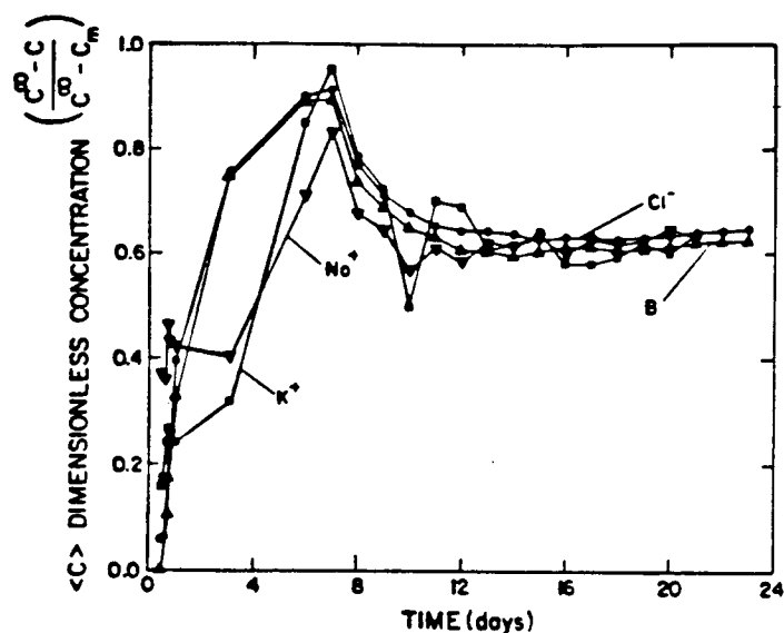
Figure 3 Nondimensional concentrations of Na + , K + , Cl - and B in the produced fluid from the Segment 4 test.
