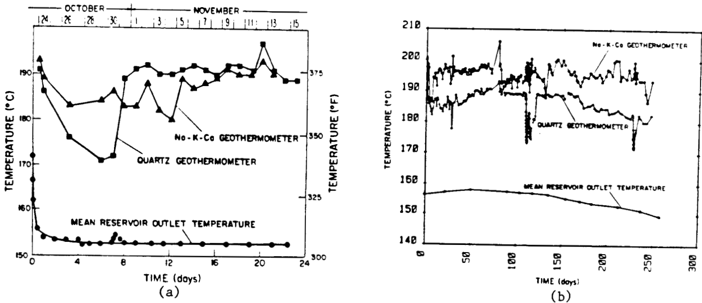
Figure 6 Comparison of the Na-K-Ca geothermometer and quartz geothermometer temperatures to the measured downhole reservoir outlet temperature for Segment 4 (a) and Segment 5 (b).
