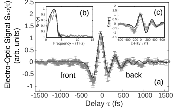
FIG. 3: The main plot (a) shows the measured EO signal S_{\text{EO}}(\tau) (grey dots), with the solid black line representing the modeled EO signal based on CTR from a skewed electron profile with a 50 fs rise and a 600 fs tail (HWHM). The EO signal S_{\text{EO}}(\nu) in the Fourier domain is shown in inset (b). The solid curve in inset (c) shows the same data as in (a) but superimposed with a modeled EO signal S_{\text{EO}}(\tau) based on a 50 fs (rms) Gaussian electron profile (no skew).
