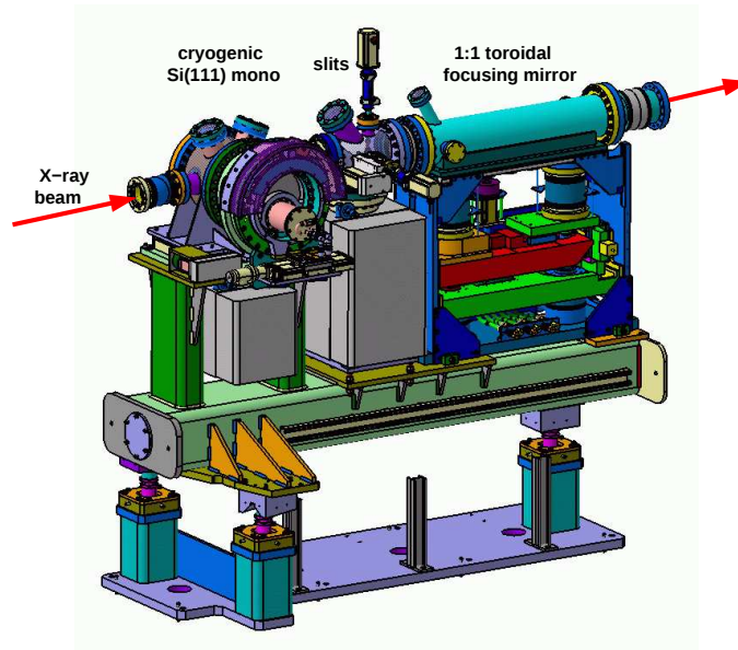
FIGURE 2. 3D model of the monochromator and focusing section of the X05DA beamline.
