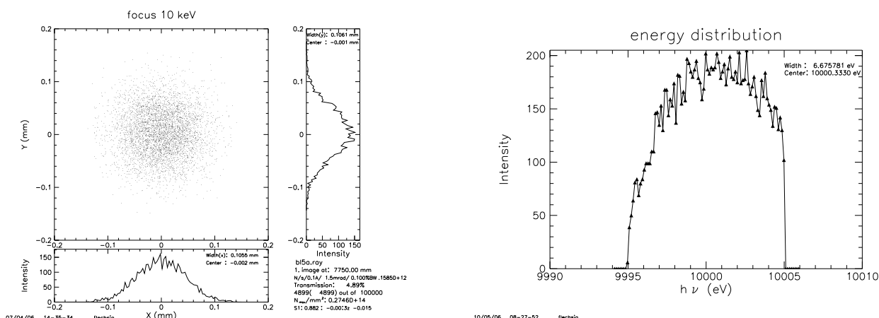
FIGURE 4. Ray tracing results for the focus at 10 keV. Left: spatial distribution, spot size: 100\text{ }\mu\text{m} FWHM, photon flux: 1.5 \cdot 10^{11} photons/(s 100 mA 0.001 BW). Right: calculated spectral distribution, resolving power E/\Delta E = 1300 .
