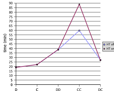
Figure 4.10 Concurrent jobs: single CPU
