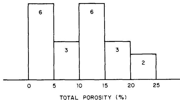
Fig. 7 Distribution of total porosity.
