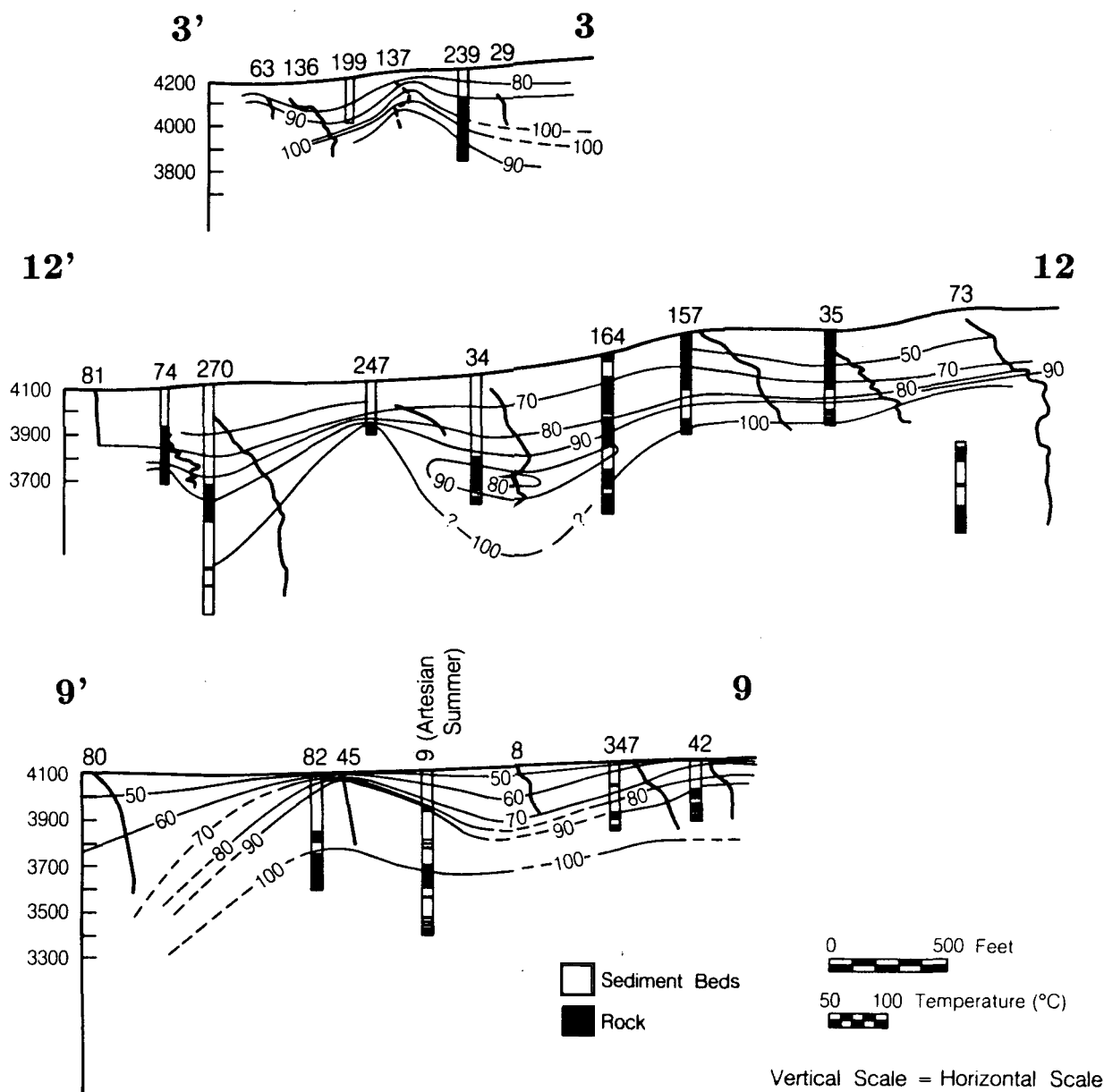
Figure 5. Cross-sectional temperature profiles drawn perpendicular to the main normal fault. Well numbers appear above the isotherms.
