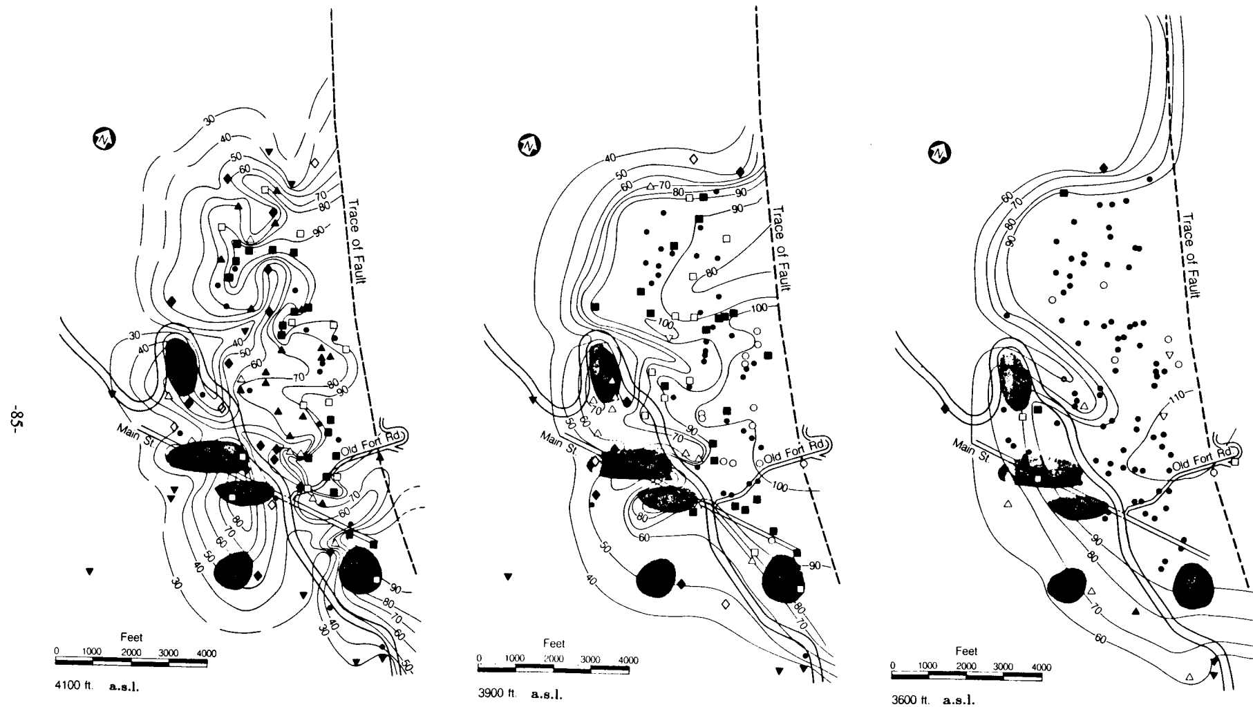
Figure 7. Temperature contour maps drawn at 4100 ft, 3900 ft and 3600 ft.
