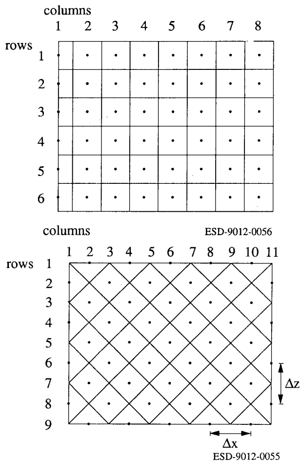
Figure 5. Schematic of parallel and diagonal grids used for modeling injection in 2-D vertical section.
