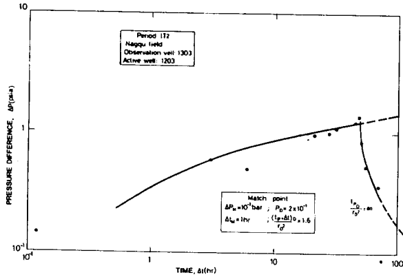
Fig. 9 Type curve match of data from period IT2 by means of a homogeneous model
