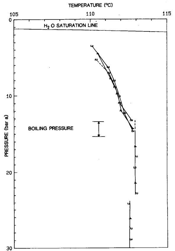
Fig. 6 Pressure-temperature data measured at well ZK 1203 compared with the H_2O saturation line
