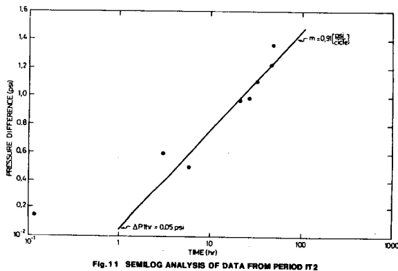
Fig. 11 SEMILOG ANALYSIS OF DATA FROM PERIOD IT2
