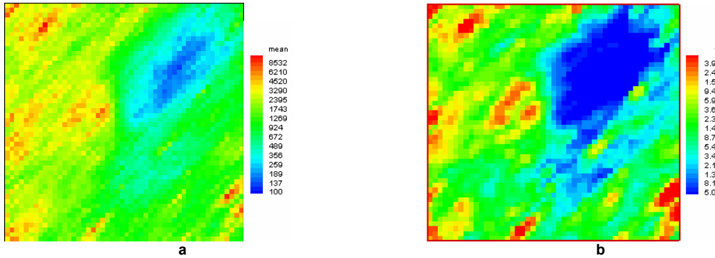
Fig. 13 – (a) Ensemble mean of the 100 final estimated permeability fields and (b) uncertainty in terms of the variance.
