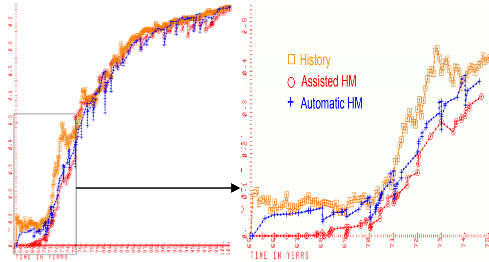
Fig. 18 – Field-wide water-cut performance for Example 1. Orange-square is history, red-circle is assisted history matching result, and blue-plus is the final automatic history matching result.
