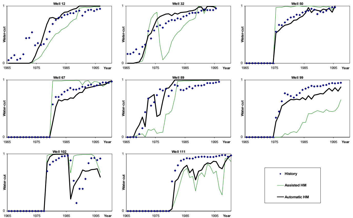
Fig. 19 – Automatic history matching improved water-cut match upon assisted history matching for most of 130 wells. Eight typical wells are shown. 'Diamond' is history, 'green line' is assisted-history-matching result, and 'black bold line' is final result by automatic history matching.
