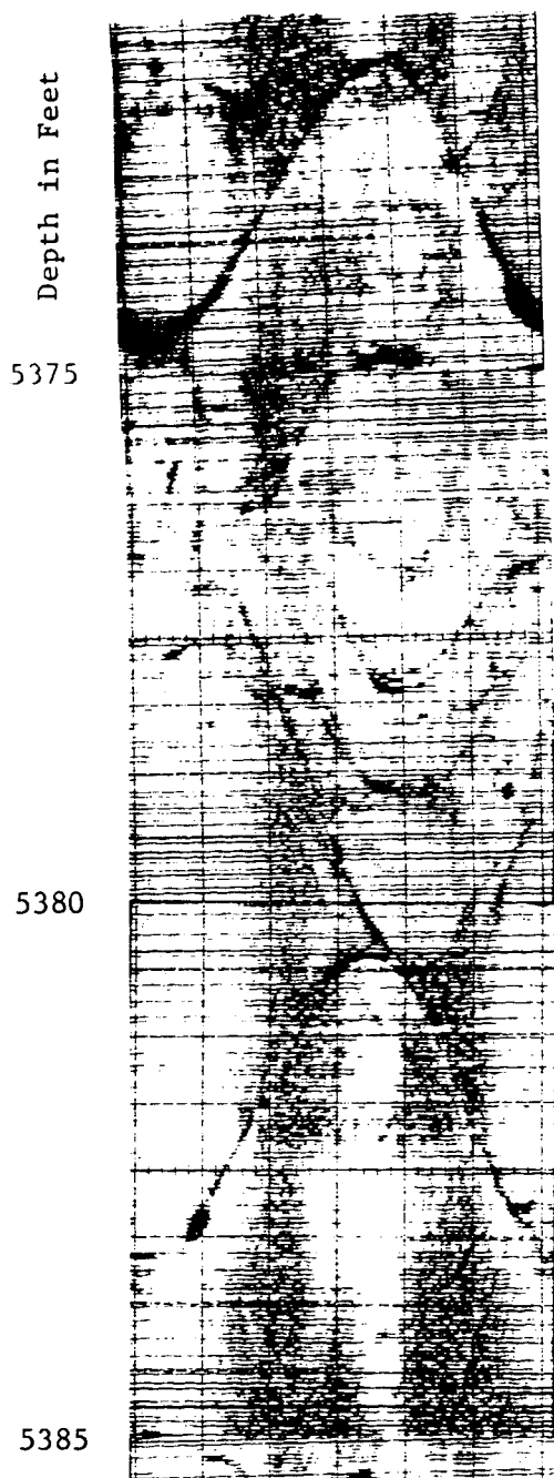
Log A--Long Valley, California
