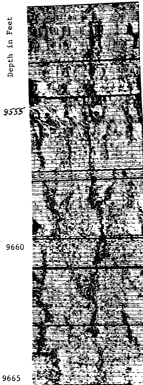
Log B--Los Alamos, New Mexico
