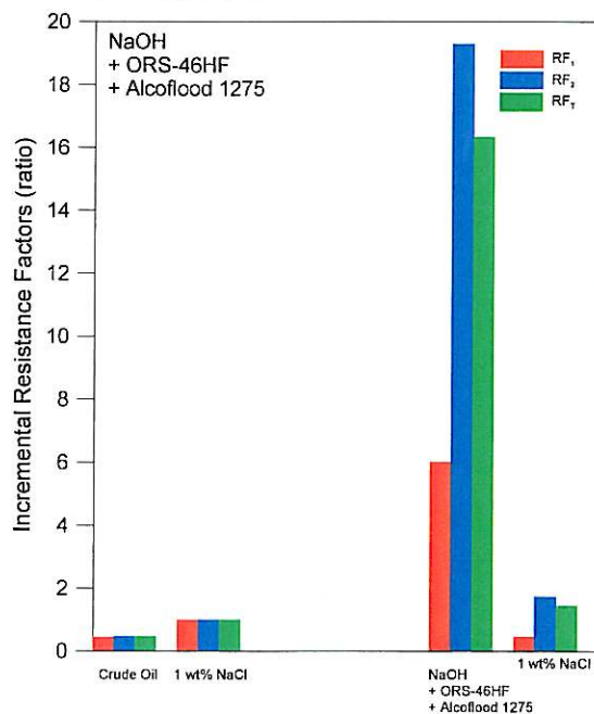
Figure 1 Ending Resistance Factors for the NaOH+ORS-46HF+Alcoflood 1275A Linear Coreflood, from left to right each set of histograms is RF 1 (red), RF 2 (blue), RF T (green)
