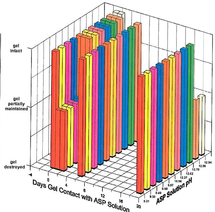
Chromium-Polyacrylamide Gel Stability In Contact with ASP Solutions 7500 mg/L Watercut 204 + 1500 mg/l WaterCut 684 0.1 wt% Na 2 SO 4
