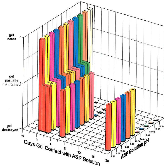
Chromium-Polyacrylamide Gel Stability In Contact with ASP Solutions 7500 mg/L Watercut 204 + 300 mg/l WaterCut 684 0.1 wt% Na 2 SO 4
