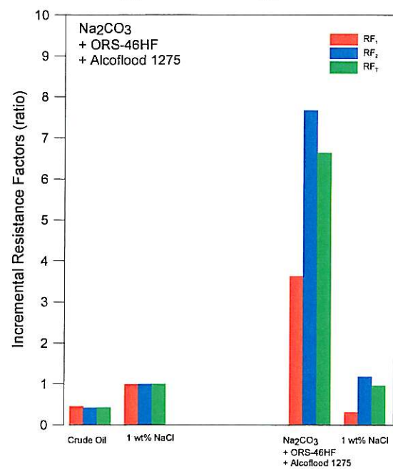
Figure 2 Ending Resistance Factors for the Na 2 CO 3 -OFS46HF+Alcoflood 1275A Linear Coreflood, from the left to right each set of histograms is RF 1 (red), RF 2 (blue), RF T (green)
