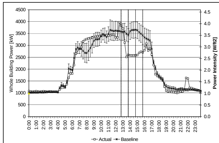
Figure B: Whole-Building Baseline Time-Series Chart Example
