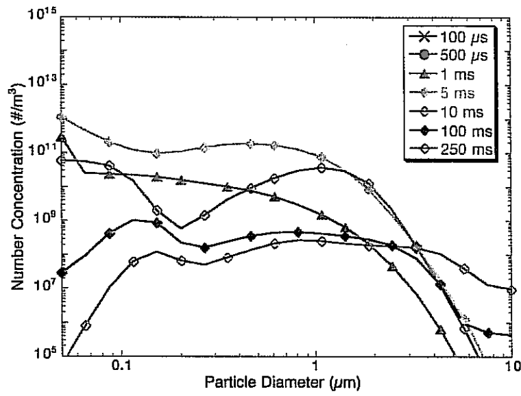
Figure 17. TOPGUN simulation results for aerosol production in a 6.5 m spherical chamber with a liquid lead wall indicate a significant population of moderately sized aerosol particles existing in the central region of the IFE chamber.
