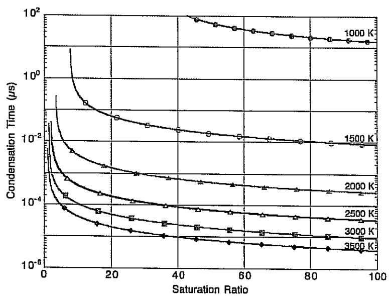
Figure 11. Time periods for condensation growth of a 1\text{ }\mu\text{m} Pb particle as a function of saturation ratio is less than 1 ms.
