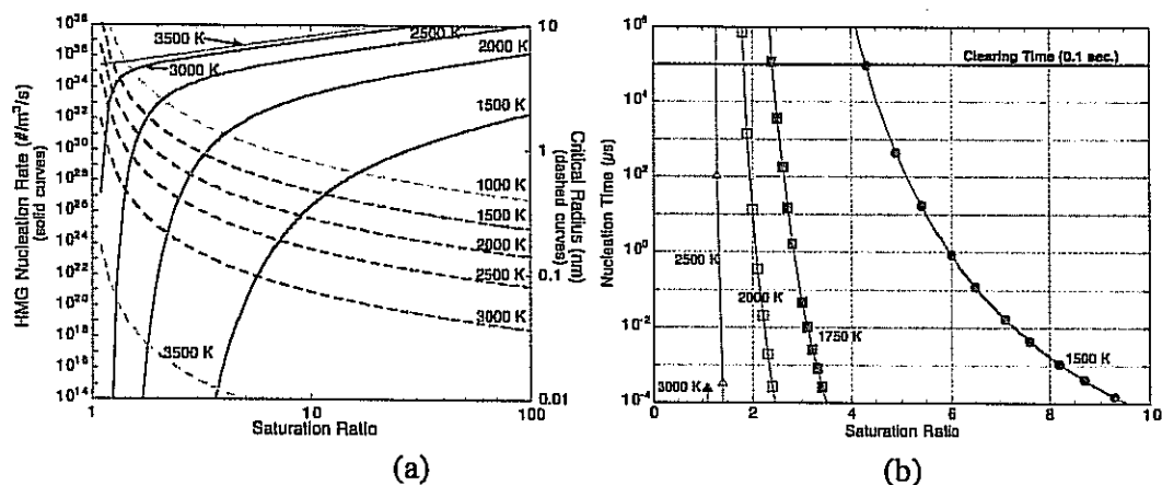
Figure 10. (a) Homogeneous nucleation rate (solid lines) and critical particle radii (dashed-lines) for nucleation of Pb aerosol particles. Note the highly non-linear behavior at moderate saturation ratios. (b) Illustration of the time required to nucleate 10^{15} particles/m 3 .
