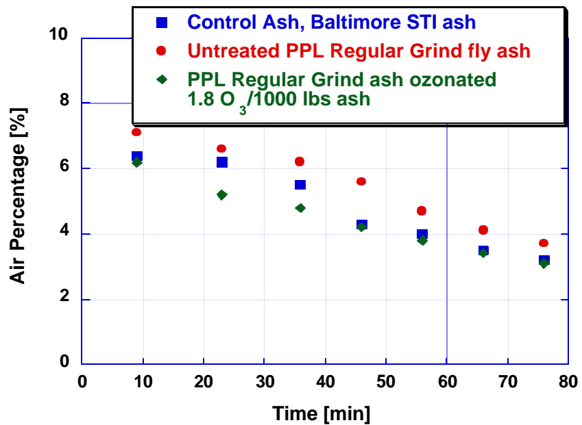
Figure 6.7. PPL regular grind ash concrete test results – test #11
