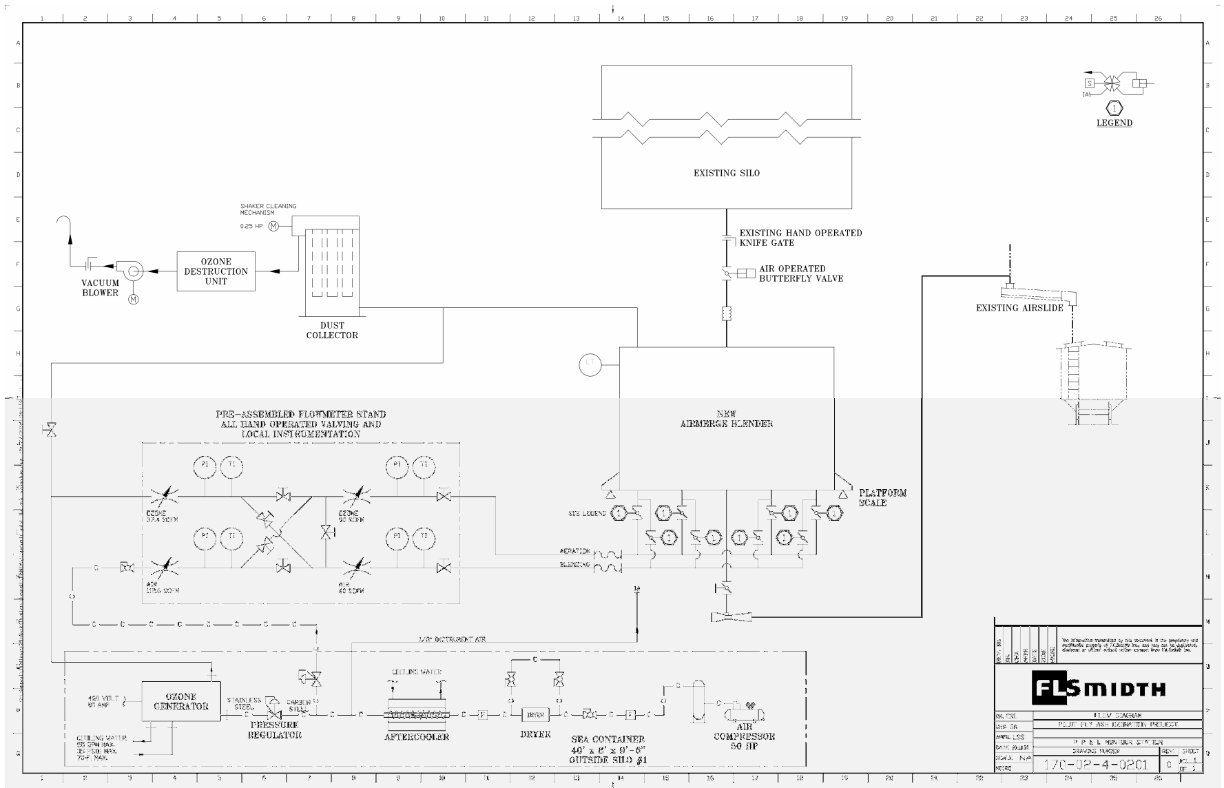
Figure 4.4 - Task 1. Semi-commercial scale installation of fluidization/ozonation technology at Montour
