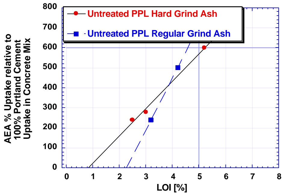
Figure 6.5. %AEA versus LOI for two PPL Class F ashes.
