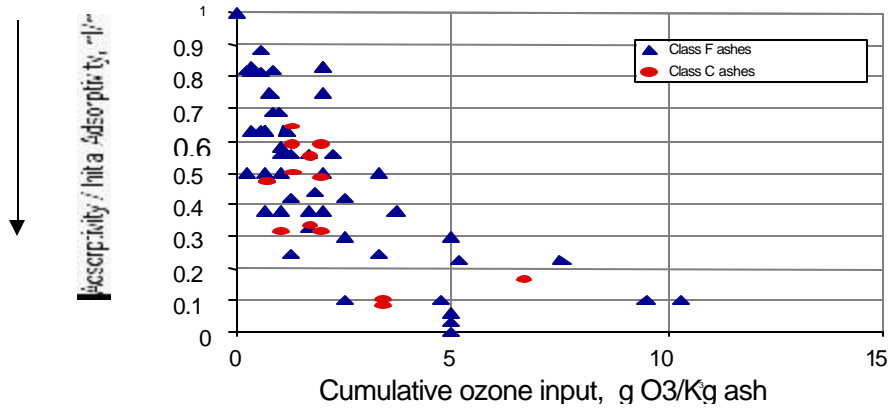
Figure 3.1. The effect of ozone treatment on surfactant adsorptivity of commercial fly ash samples. Data points represent a range of ash types, bed masses (50 - 400 gm), ozone concentrations (500 ppm - 2 vol-%), and contact times (10 - 800 min). All data are for fixed bed treatment at ambient temperature and pressure.
