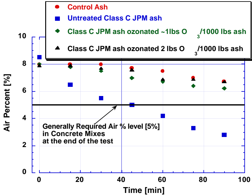
Figure 6.10. Dairyland JPM class C ash concrete test results – test #12
