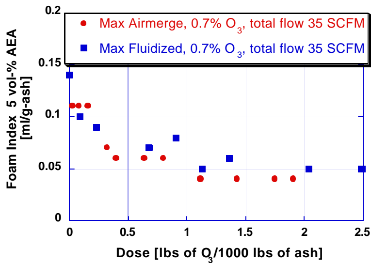
Figure 6.3. Parametric ozonation tests – effect of different fluidization modes (airmerge vs. simple fluidization)
