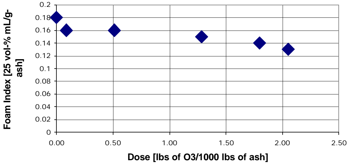
Test #17 - March 18 5% AC blended in STI ash, MaxFluidized 2% O3, Flow = 12 SCFM
