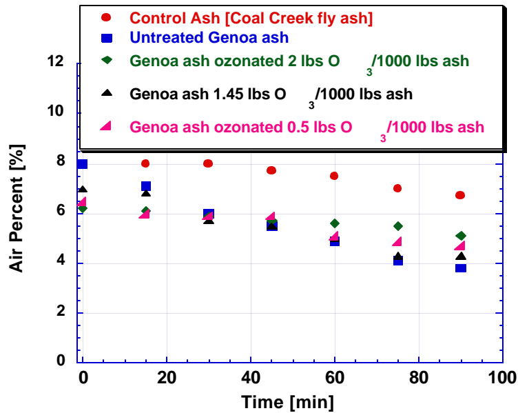
Figure 6.11. Dairyland Genoa Class C/F blend ash concrete test results – test #14
