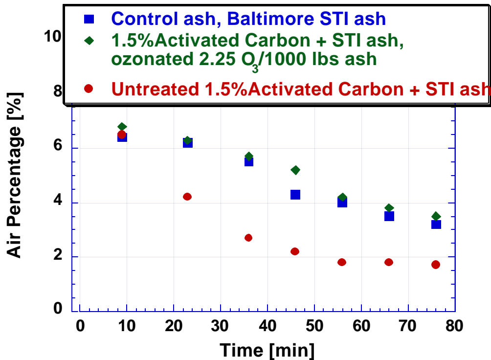
Figure 6.12. Class F (STI Baltimore) mixed with 1.5% Activated Carbon concrete test results – test#18
