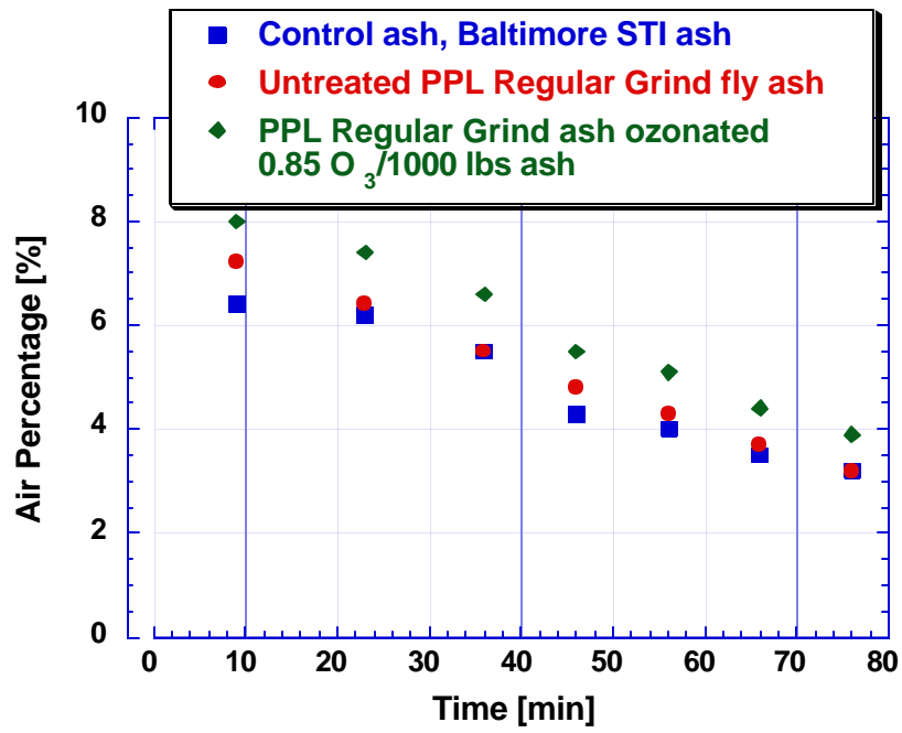
Figure 6.6. PPL regular grind ash concrete test results – test #9
