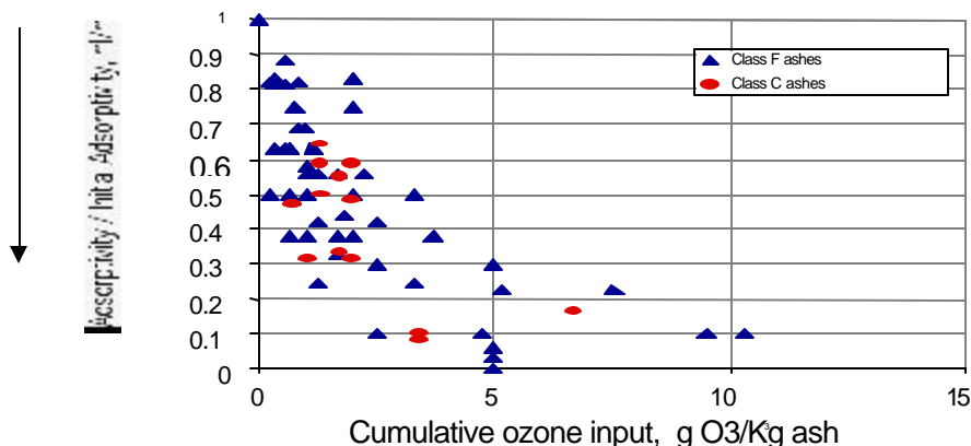
Figure 1.1. The effect of ozone treatment on surfactant adsorptivity of commercial fly ash samples. Data points represent a range of ash types, bed masses (50 - 400 gm), ozone concentrations (500 ppm - 2 vol-%), and contact times (10 - 800 min). All data are for fixed bed treatment at ambient temperature and pressure.
