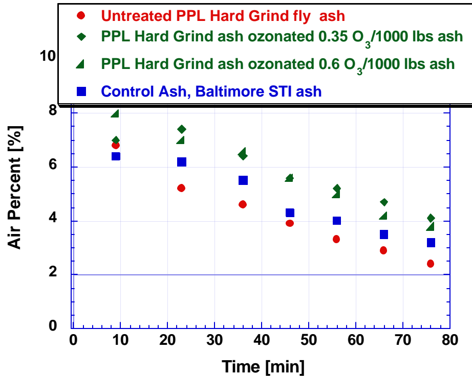
Figure 6.8. PPL hard grind ash concrete test results – test #8
