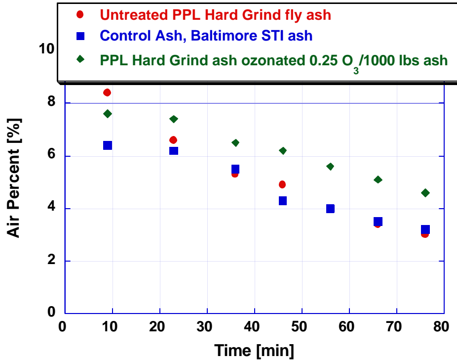
Figure 6.9. PPL hard grind ash concrete test results – test #7
