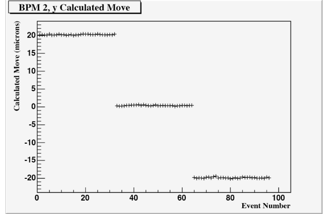
FIG. 18: Once x_2 and s_n had been determined, the amount by which any BPM had been moved could be calculated as a means of verifying the calibration. This plot shows the calculated move for the 96 events over which BPM 2, y was being moved, and clearly shows the pattern used: Nominal location plus 20 \mu\text{m} , nominal location, and nominal location minus 20 \mu\text{m} .
