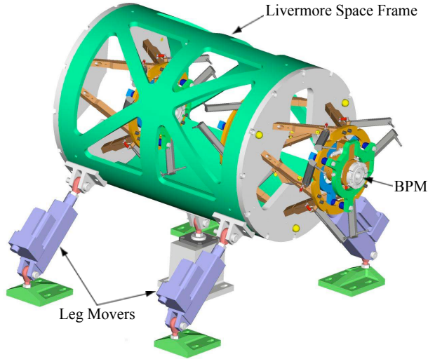
FIG. 6: The Livermore space frame served as the mounting platform for the three BINP BPMs.
