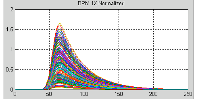
FIG. 14: Demodulated waveforms from BPM 1, x for a data set. Each colored line represents a separate ATF extraction and has been normalized by the corresponding amplitude of the reference cavity. In the plot, the x axis refers to the sample number.
