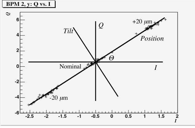
FIG. 13: Q plotted against I (in this case for BPM 2, y ). The three clusters of points each contain 32 beam pulses corresponding to three different y positions for BPM 2: The nominal position, and \pm 20 \mu\text{m} . The IQ -phase \Theta is the angle between the the I - Q basis and the Position - Tilt basis. The point spread in each cluster is due to beam jitter. The center cluster, which corresponds to the nominal y position of BPM 2, is not located at (0,0) owing to a small amount of residual y tilt and y offset for BPM 2.
