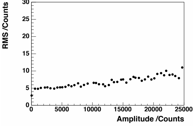
FIG. 42: Plot showing the variation with amplitude of the amplitude RMS.
