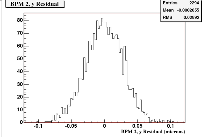
FIG. 30: The residuals \delta y_2 for 2300 ATF extractions from a period spanning approximately half an hour on the evening of 11 March 2005. Four events were removed on account of low reference cavity amplitude, which usually signifies either a missing bunch or at least a very low current bunch, and a further two flier events were removed for a total of 2294 events. The coefficients used to calculate the residuals were determined from the entire data set less the low reference cavity amplitude events.
