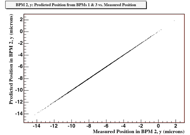
FIG. 31: The beam position at BPM 2 as predicted by BPMs 1 and 3 vs. the measured position in BPM 2 for 2300 ATF extractions from the evening of 11 March 2005. Four events were removed on account of low reference cavity amplitude, which usually signifies either a missing bunch or at least a very low current bunch, and a further two flier events were removed for a total of 2294 events. The coefficients used to calculate the position at BPM 2 from the positions in BPMs 1 and 3 were determined from the entire data set.
