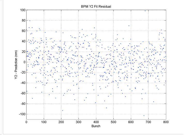
FIG. 28: The residual for BPM 2 vs. the event number (equivalent to time) for 800 ATF extractions from 27 May 2005. This data was analyzed using the digital down-conversion (DDC) algorithm, and the calculation of the predicted position included terms for x'_1 , y'_1 , x'_3 , and y'_3 . The lack of structure here demonstrates the stability of the experiment.
