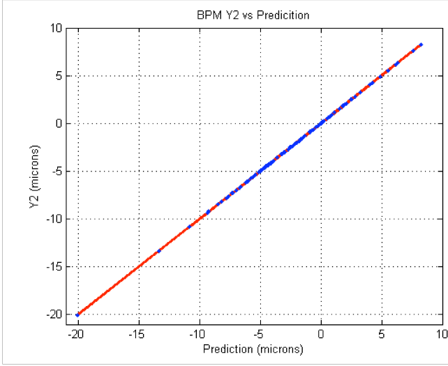
FIG. 26: The measured position vs. the predicted position for BPM 2 for 100 ATF extractions from 27 May 2005. This data was analyzed using the digital down-conversion (DDC) algorithm, and the calculation of the predicted position included terms for x'_1 , y'_1 , x'_3 , and y'_3 .
