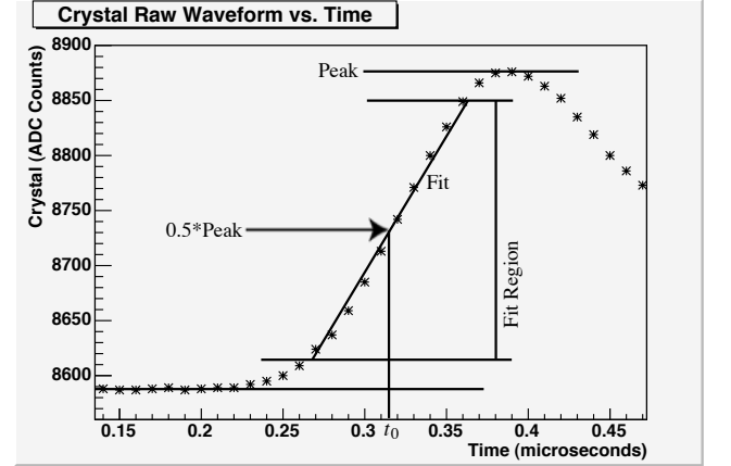
FIG. 12: The value for t_0 was determined on an event by event basis by fitting the rise of the signal from the crystal detector, and defining t_0 to be at the midpoint of the rise, i.e. the time corresponding to when the signal is 0.5 times the value at the peak. So that only the linear portion of the waveform is used, the top and bottom of the rise are excluded from the fit.
