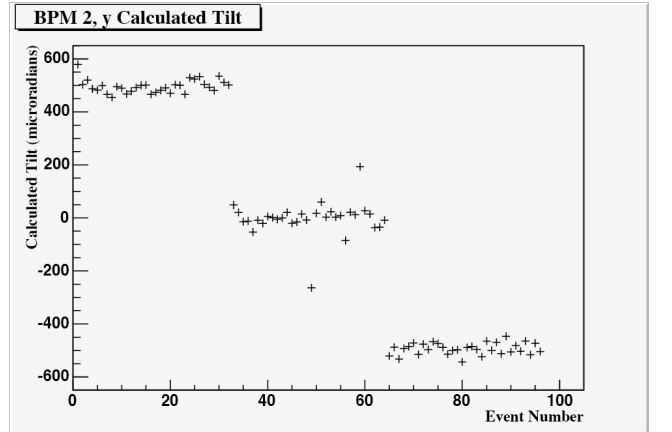
FIG. 20: Once \theta_{0i} and s'_i have been determined, the amount by which the BPM has been tilted may be calculated as a means of verifying the calibration. This plot shows the calculated tilts for the 96 events over which BPM 2, y was being tilted, and clearly shows the pattern used: Nominal orientation plus 500 \mu radians, nominal orientation, and nominal orientation minus 500 \mu radians. Deviations from the applied tilts may be attributed to jitter in the bunch's angle of attack.
