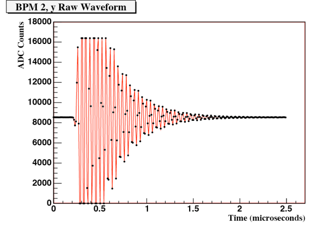
FIG. 11: An example of a raw waveform – this one happens to be from BPM 2, y . Note that in this case the samples between 0.3 \mu\text{s} and 0.6 \mu\text{s} are saturated.
