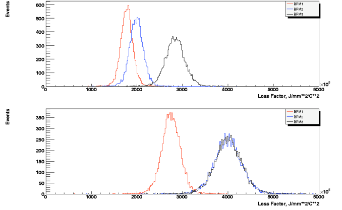
FIG. 38: Measured loss factors in the x (top) and y (bottom) directions from the data measured on 27/05/05. See Table II for explicit values.
