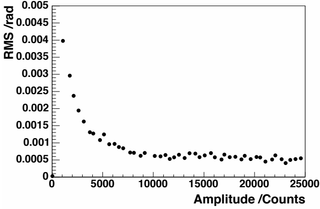
FIG. 43: Plot showing the variation with amplitude of the phase RMS.
