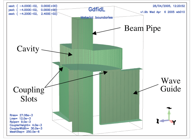
FIG. 5: A quarter view of the inside surface of a BINP BPM.
