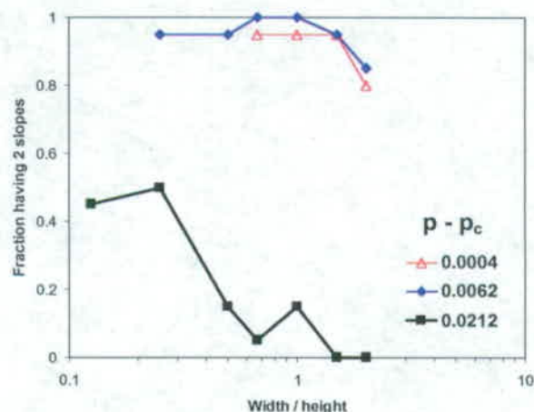
Figure 8. Fraction of realizations having two distinct slopes in their simulated imbibition curve.
