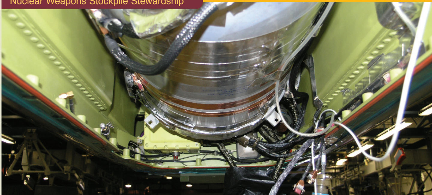
W80 Environmental Test Unit installed in an Advanced Cruise Missile in preparation for flight test FTU-1, flown in September.
