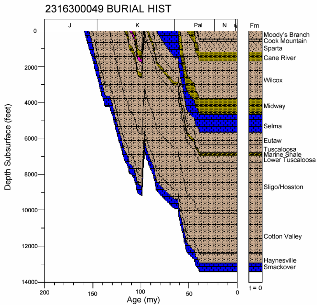
Figure 194. Burial history for well 2316300049, Mississippi Interior Salt Basin.
