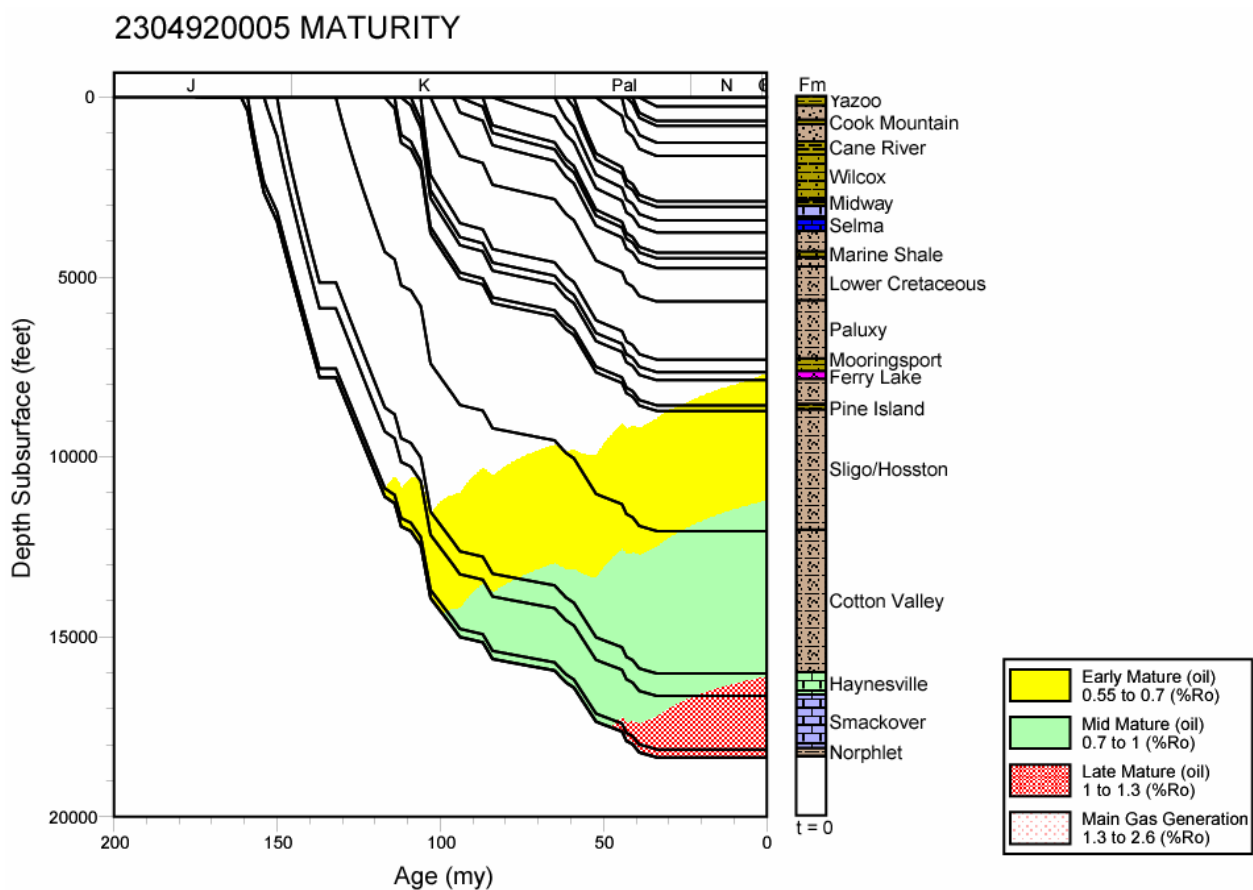
Figure 224. Thermal maturation profile for well 2304920005, Mississippi Interior Salt Basin.
