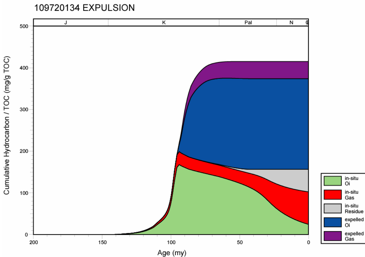
Figure 310. Hydrocarbon expulsion plot for well 109720134, Mississippi Interior Salt Basin.
