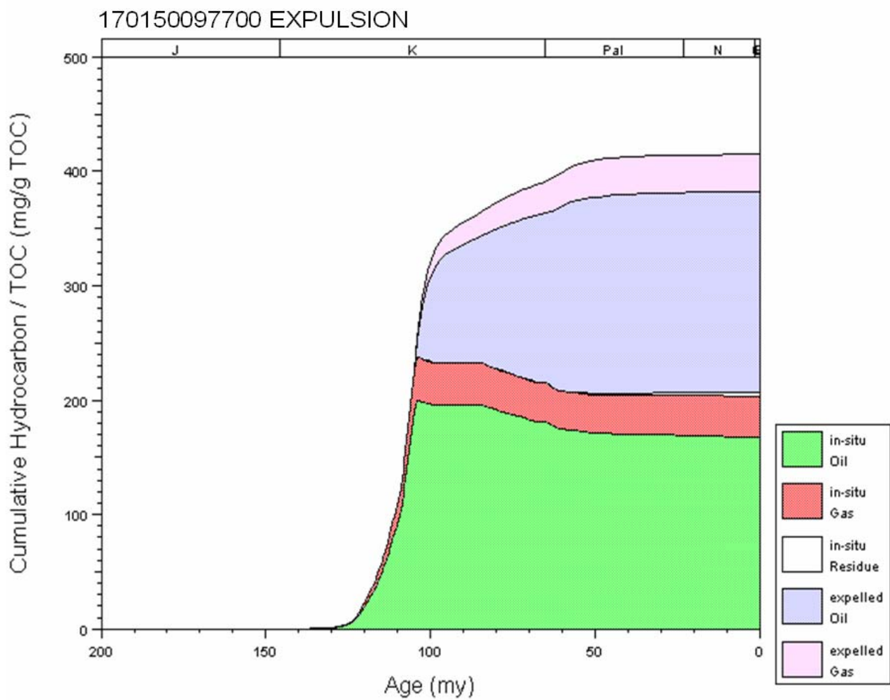
Figure 321. Hydrocarbon expulsion plot for well 170150097700. Sabina Uplift. Prepared by Roger Barnaby.
