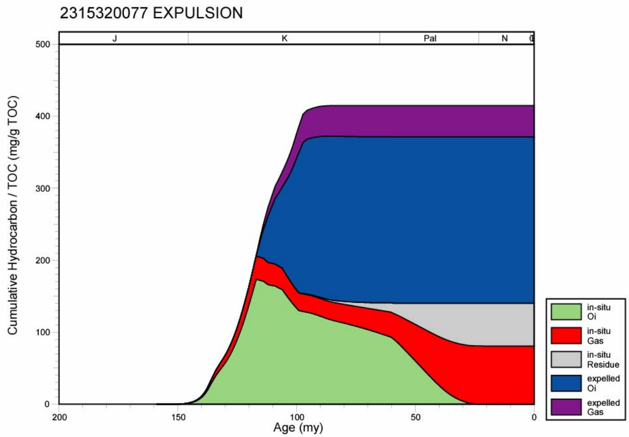
Figure 304. Hydrocarbon expulsion plot for well 2315320077, Mississippi Interior Salt Basin.
