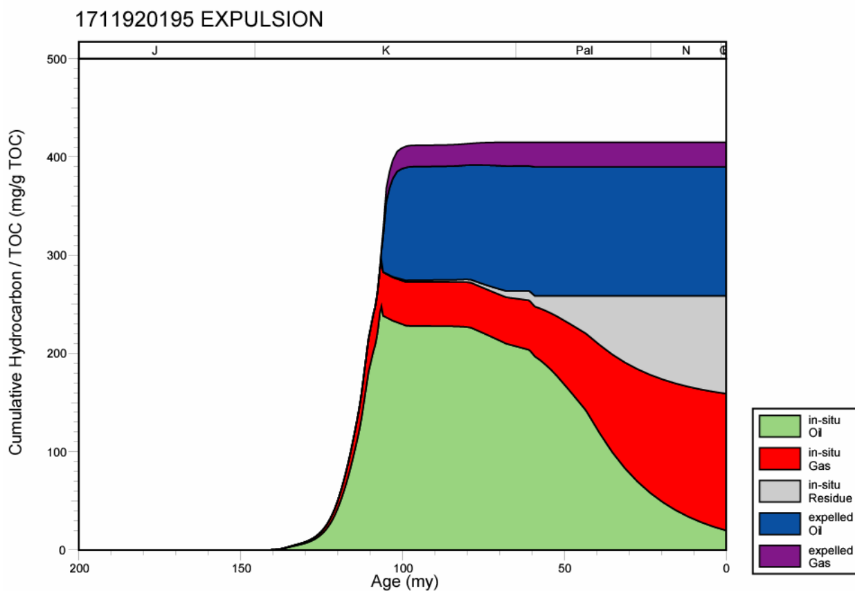
Figure 142. Hydrocarbon expulsion plot for well 1711920195, North Louisiana Salt Basin.
