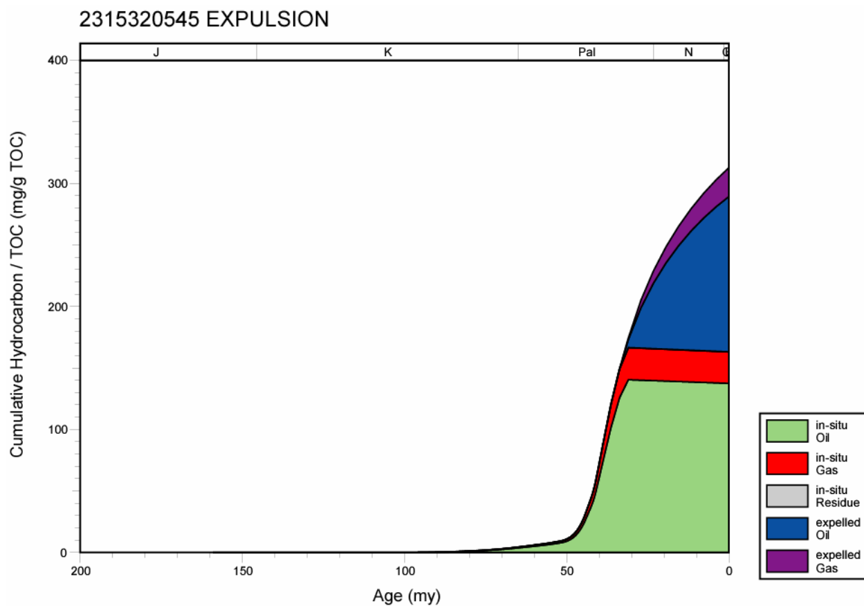
Figure 282. Hydrocarbon expulsion plot for well 2315320545, Mississippi Interior Salt Basin.
