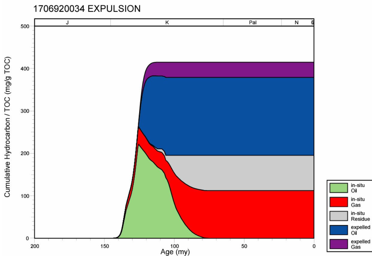
Figure 148. Hydrocarbon expulsion plot for well 1706920034, North Louisiana Salt Basin.
