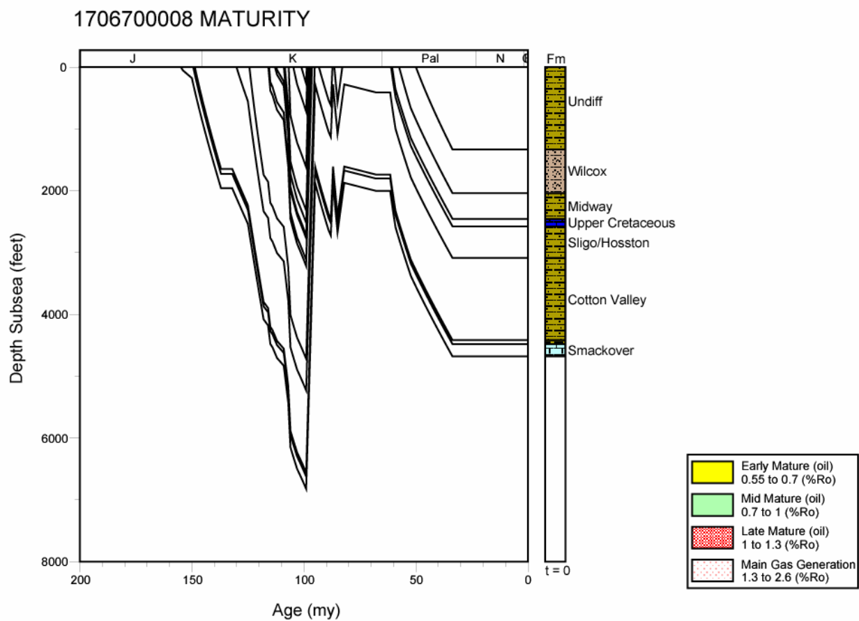
Figure 126. Thermal maturation profile for well 1706700008, North Louisiana Salt Basin.
