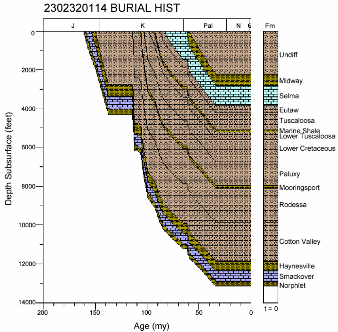
Figure 207. Burial history for well 2302320114, Mississippi Interior Salt Basin.
