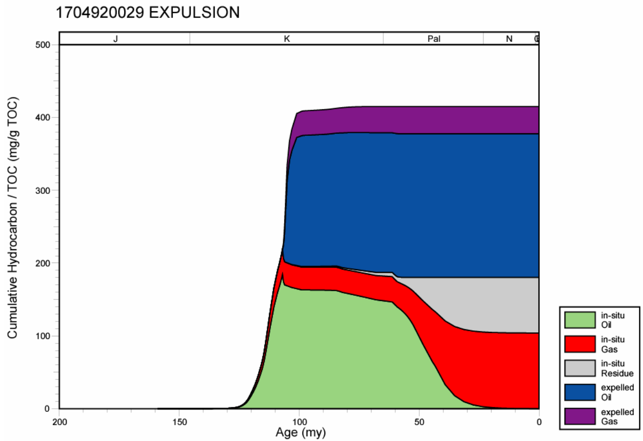
Figure 162. Hydrocarbon expulsion plot for well 1704920029, North Louisiana Salt Basin.
