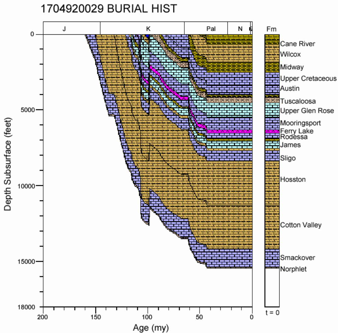
Figure 74. Burial history for well 1704920029, North Louisiana Salt Basin.
