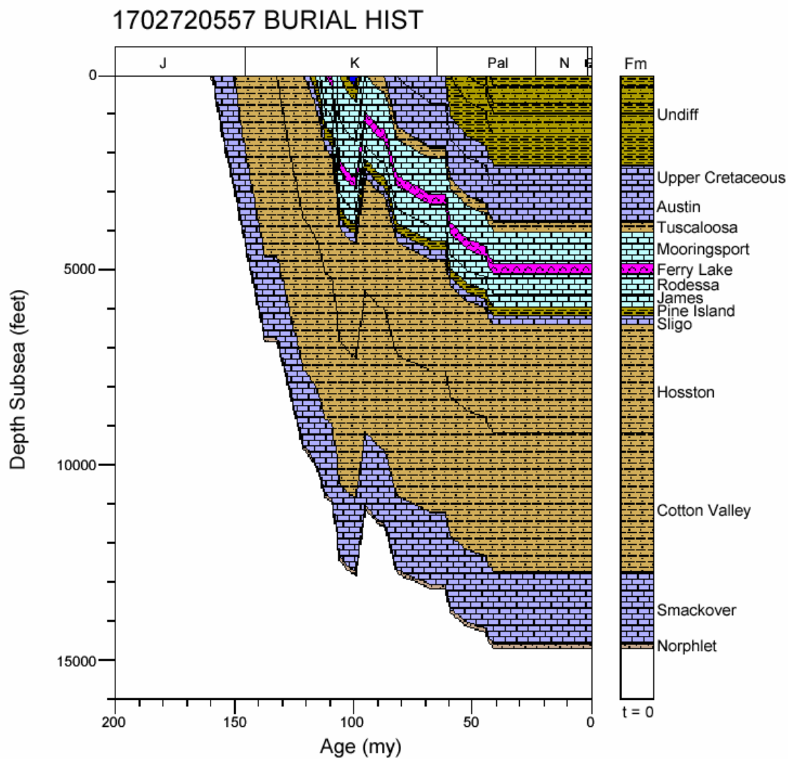
Figure 63. Burial history for well 1702720557, North Louisiana Salt Basin.
