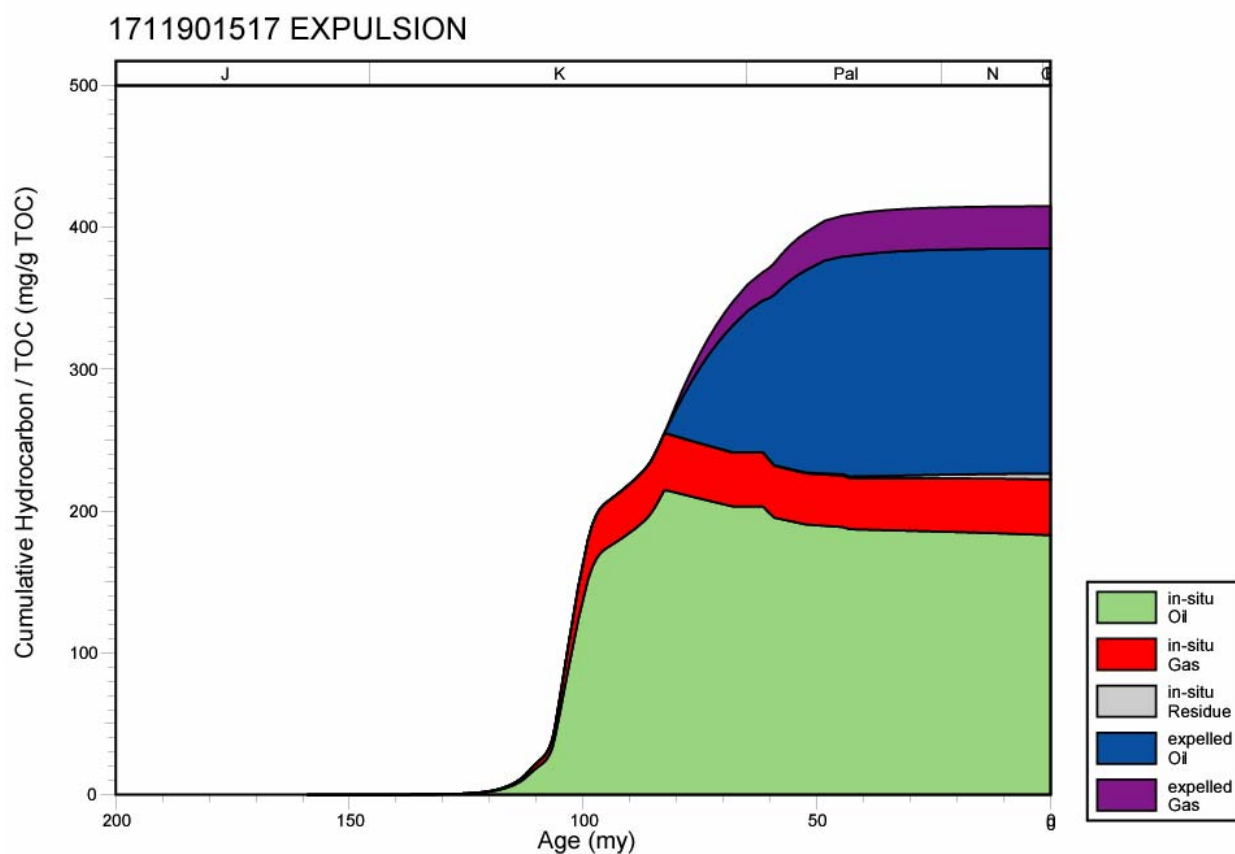
Figure 143. Hydrocarbon expulsion plot for well 1711901517, North Louisiana Salt Basin.
