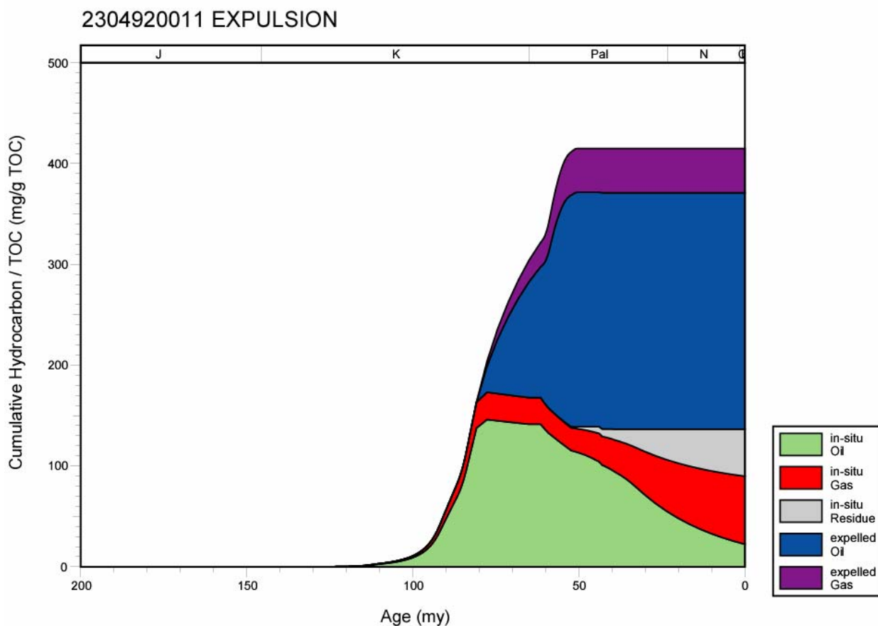
Figure 271. Hydrocarbon expulsion plot for well 2304920011, Mississippi Interior Salt Basin.
