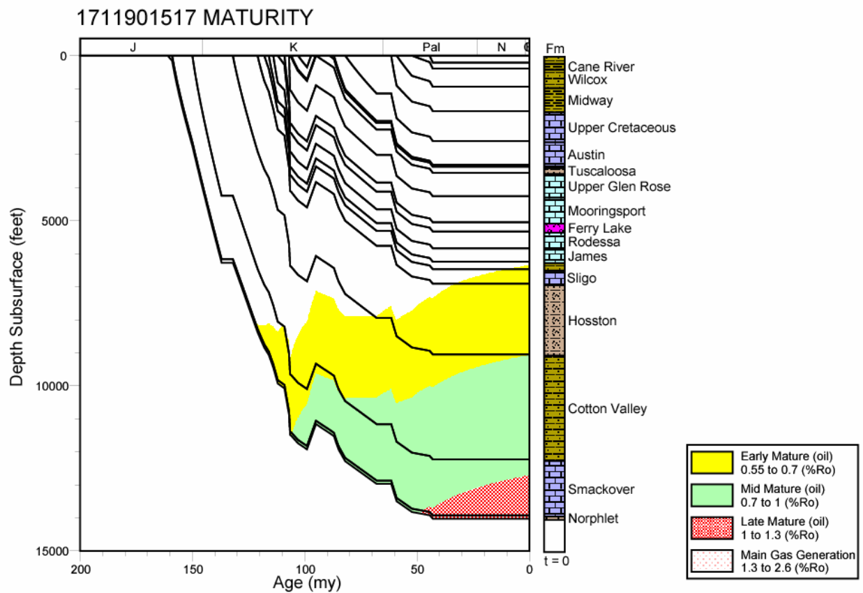
Figure 101. Thermal maturation profile for well 1711901517, North Louisiana Salt Basin.
