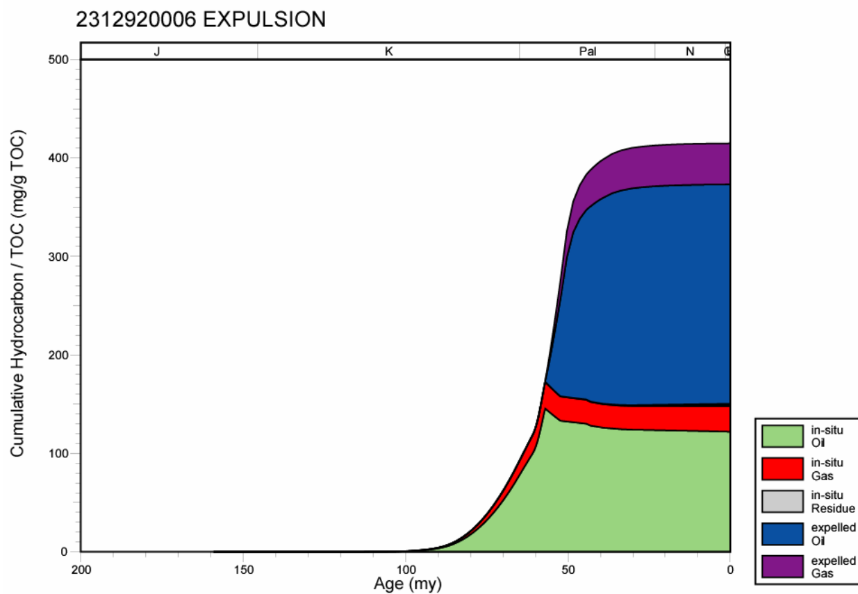
Figure 275. Hydrocarbon expulsion plot for well 2312920006, North Louisiana Salt Basin.
