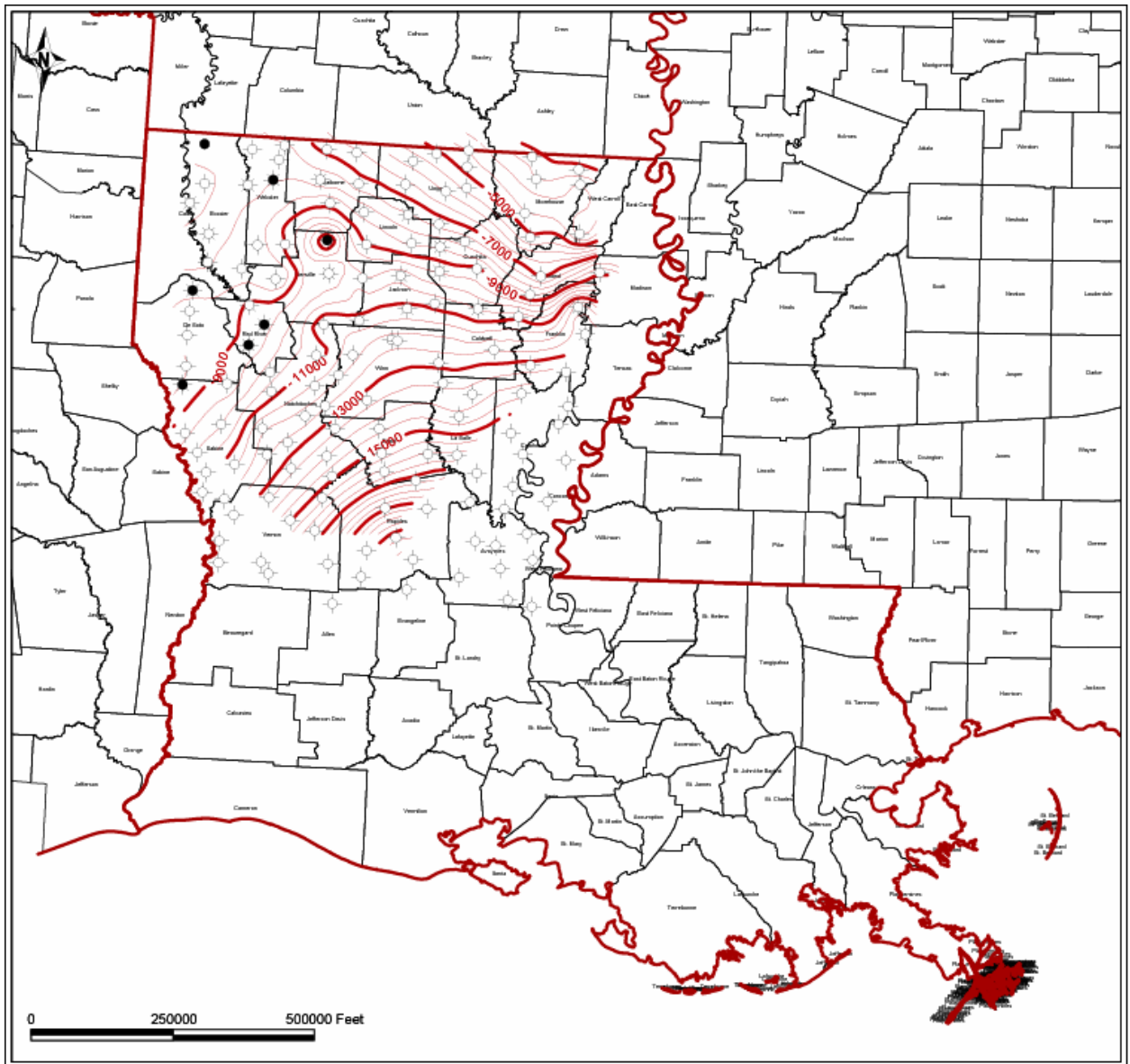
Figure 14. Structure map on the top of the Cotton Valley.
