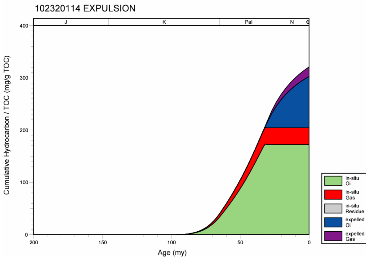
Figure 300. Hydrocarbon expulsion plot for well 102320114, Mississippi Interior Salt Basin.
