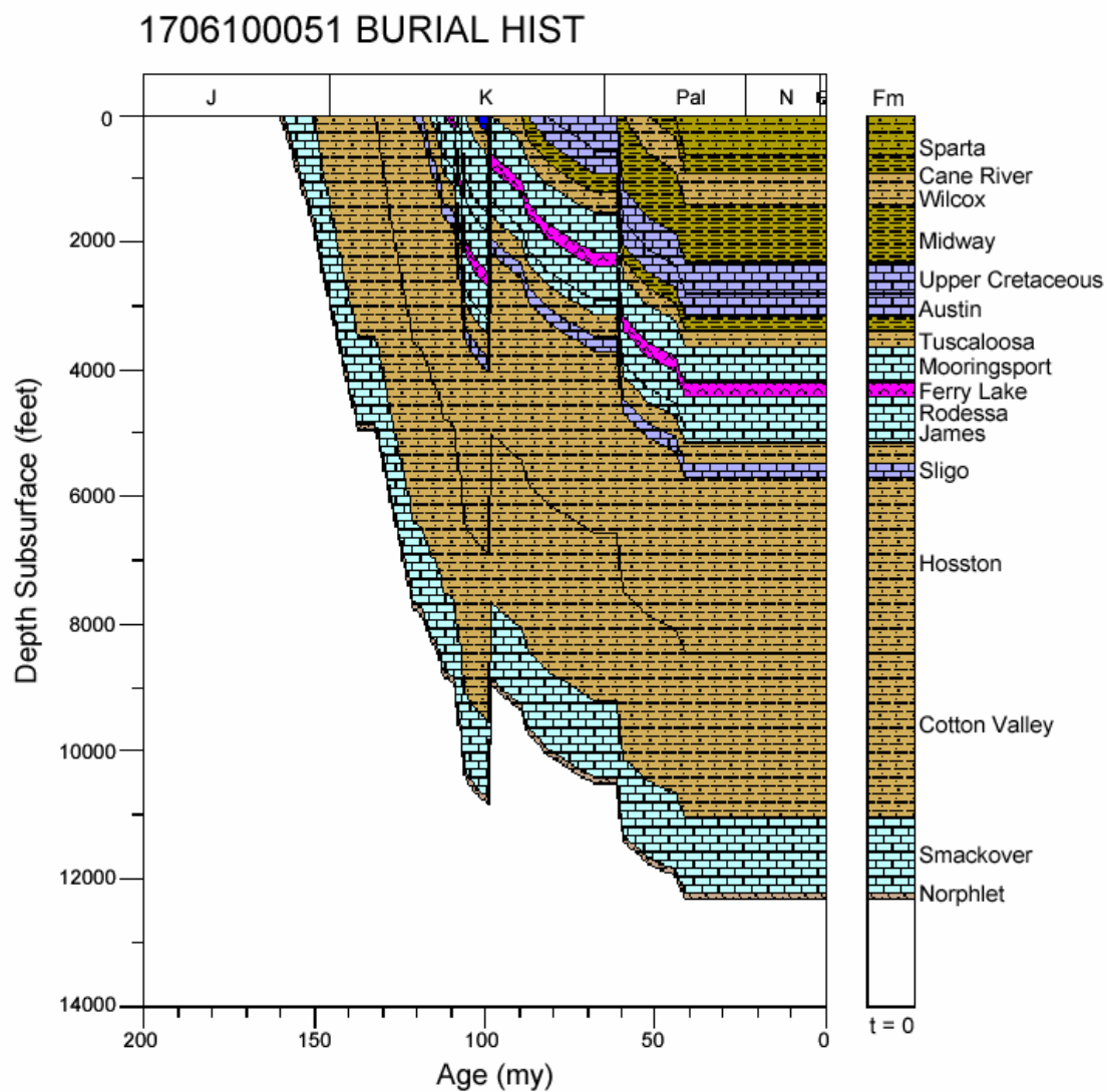
Figure 71. Burial history for well 1706100051, North Louisiana Salt Basin.
