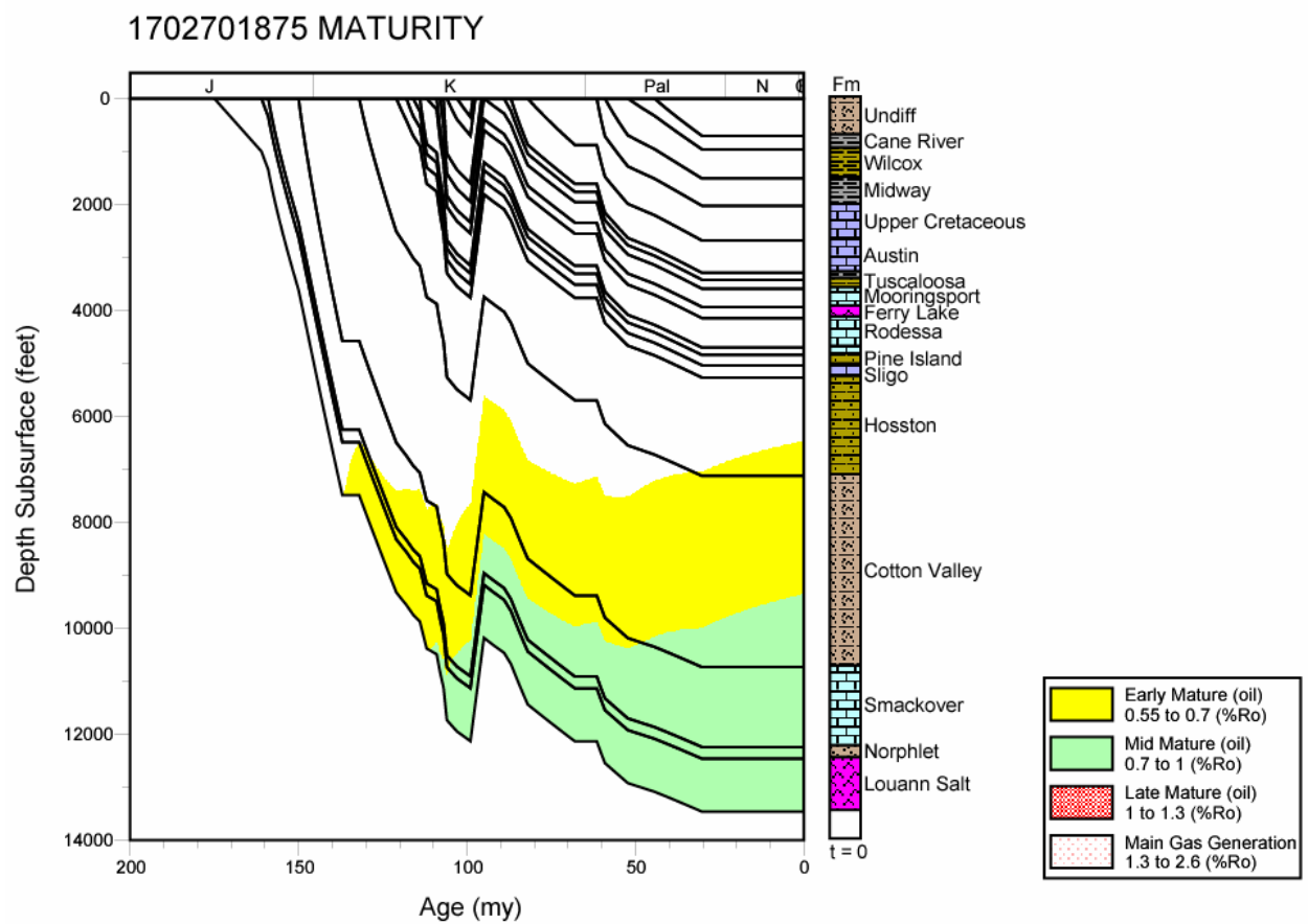
Figure 107. Thermal maturation profile for well 1702701875, North Louisiana Salt Basin.
