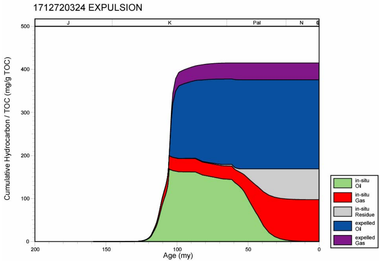
Figure 163. Hydrocarbon expulsion plot for well 1712720324, North Louisiana Salt Basin.
