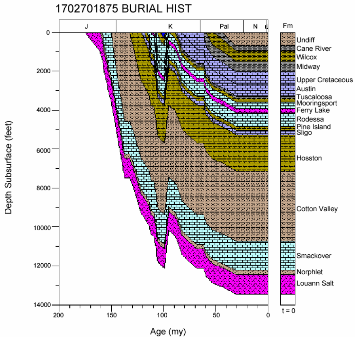
Figure 61. Burial history for well 1702701875, North Louisiana Salt Basin.
