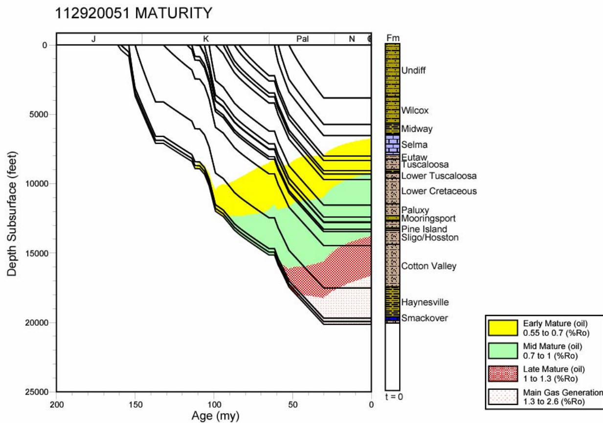
Figure 264. Thermal maturation profile for well 112920051, Mississippi Interior Salt Basin.
