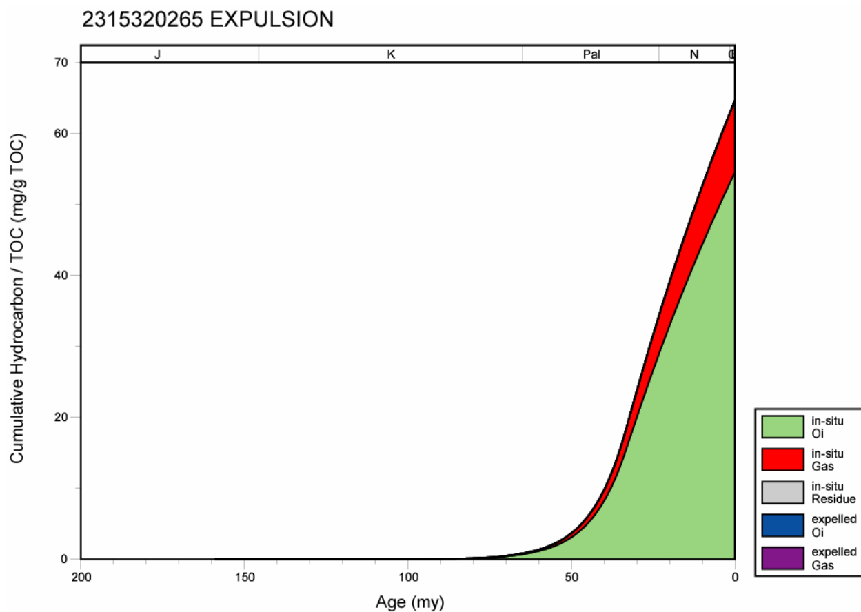
Figure 302. Hydrocarbon expulsion plot for well 2315320265, Mississippi Interior Salt Basin.
