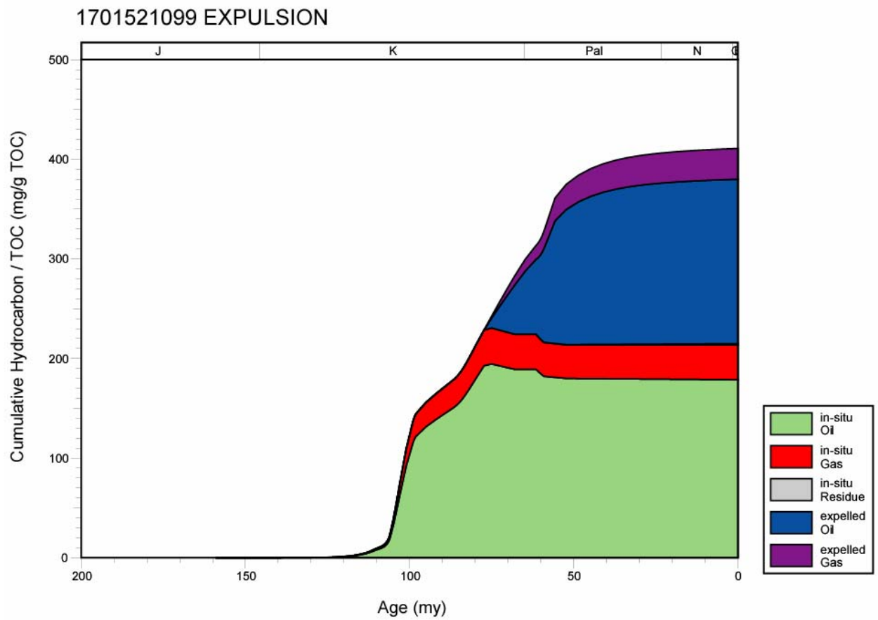
Figure 131. Hydrocarbon expulsion plot for well 1701521099, North Louisiana Salt Basin.
