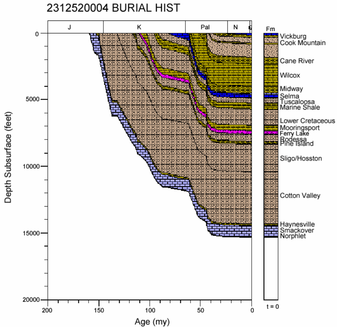
Figure 174. Burial history for well 2312520004, Mississippi Interior Salt Basin.
