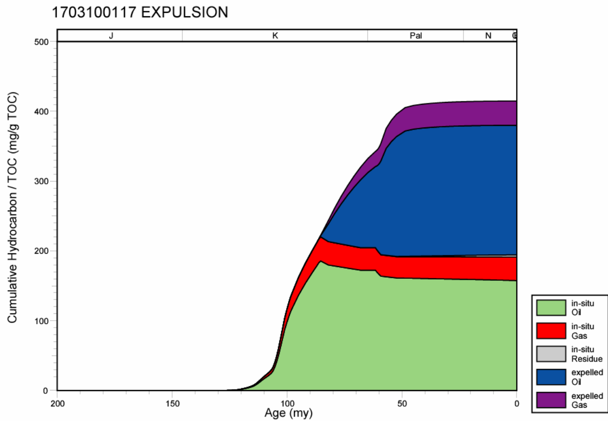
Figure 137. Hydrocarbon expulsion plot for well 1703100117, North Louisiana Salt Basin.
