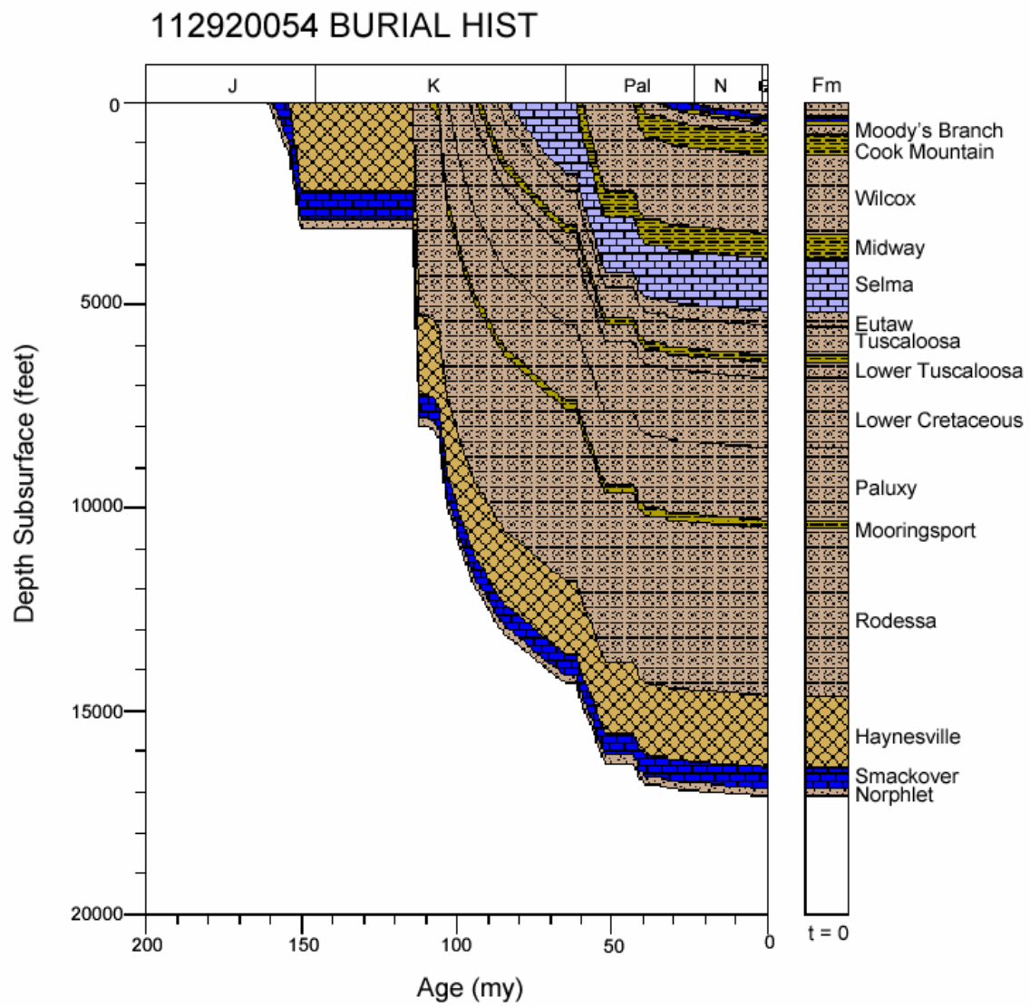
Figure 188. Burial history for well 112920054, Mississippi Interior Salt Basin.
