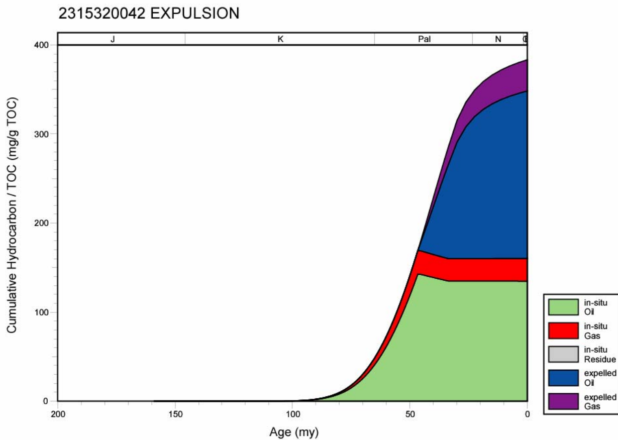
Figure 301. Hydrocarbon expulsion plot for well 2315320042, Mississippi Interior Salt Basin.
