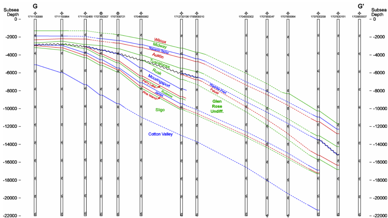
Figure 9. Cross section G-G' for the North Louisiana Salt Basin. See Figure 2 for location of cross section.
