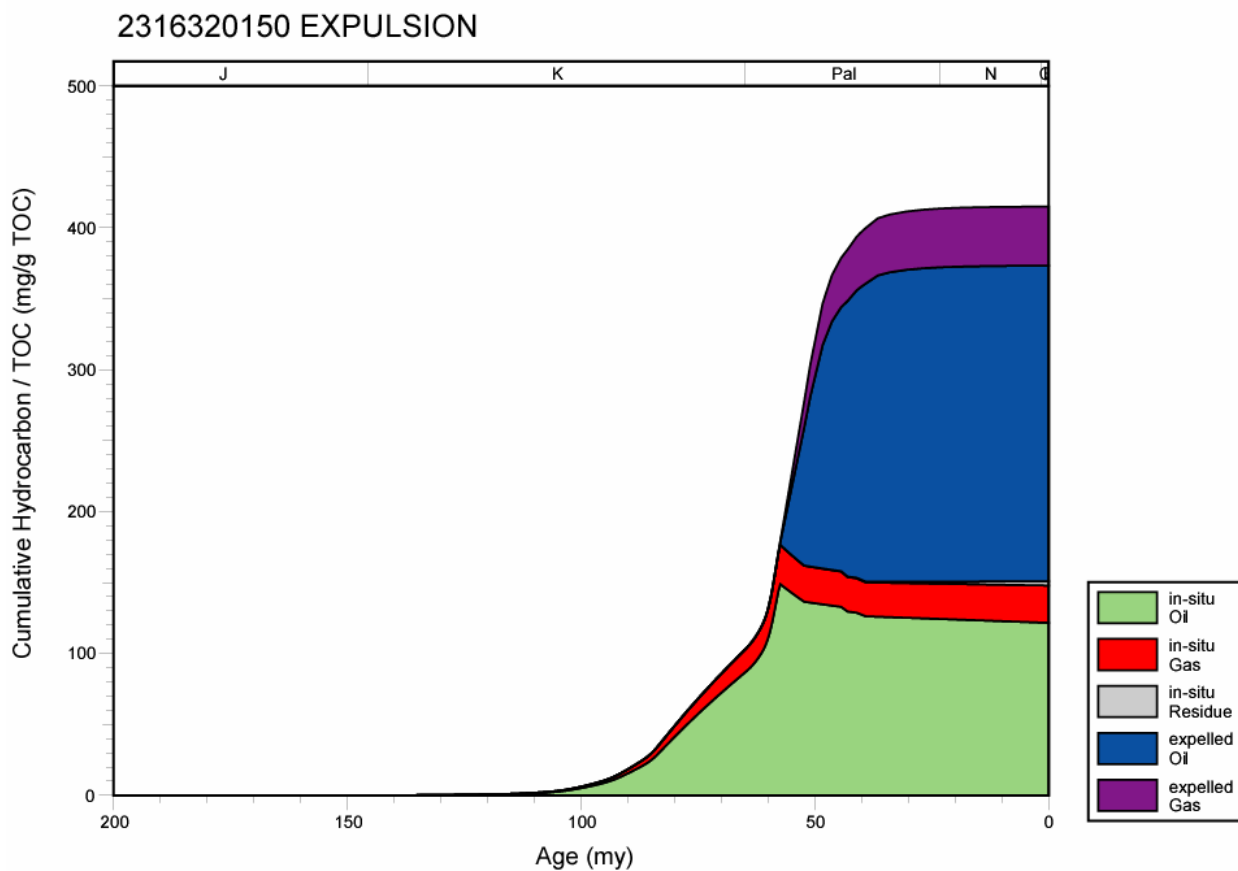
Figure 291. Hydrocarbon expulsion plot for well 2316320150, Mississippi Interior Salt Basin.
