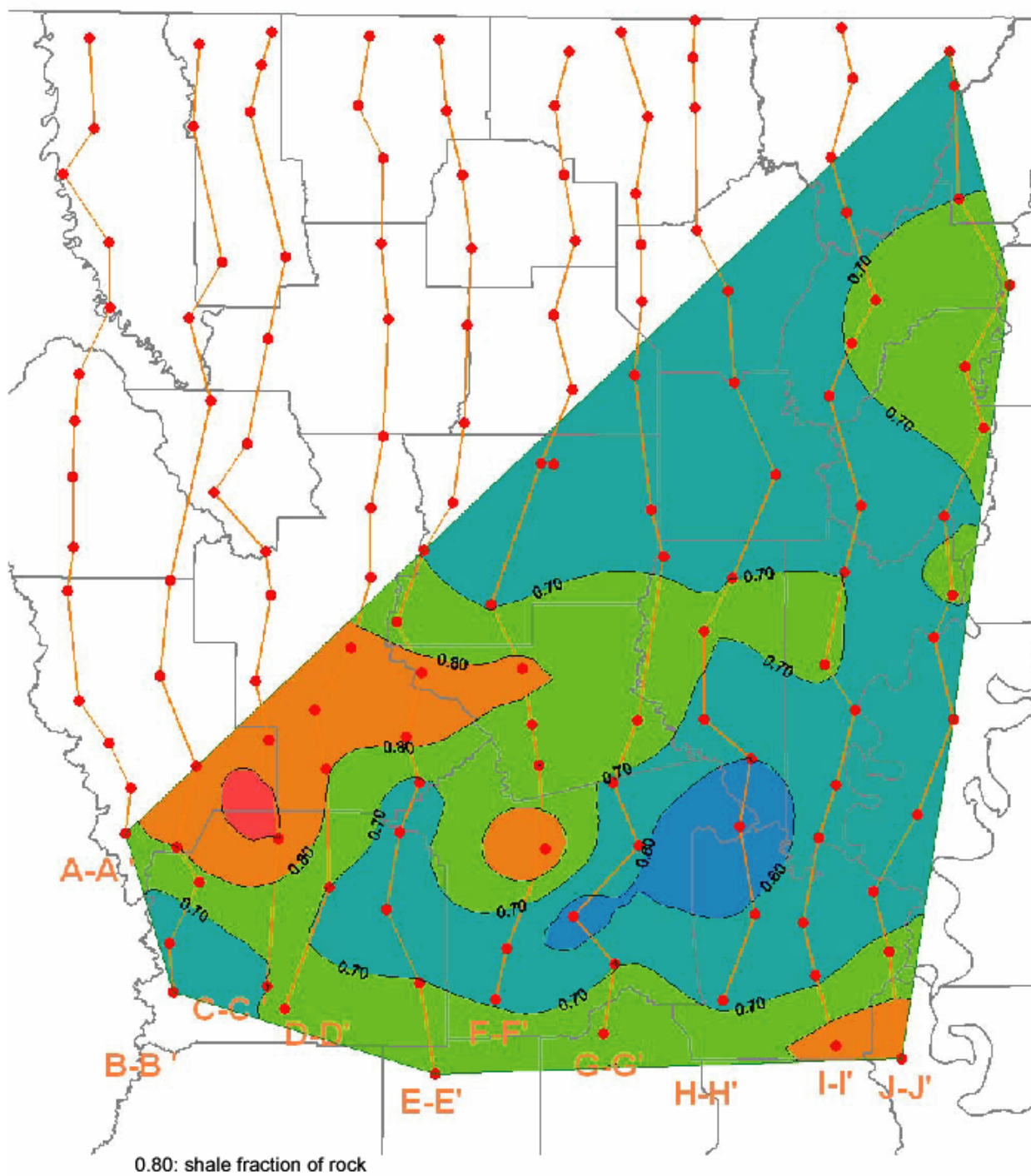
Figure 23. Lithology map of Cockfield. Prepared by Roger Barnaby.
