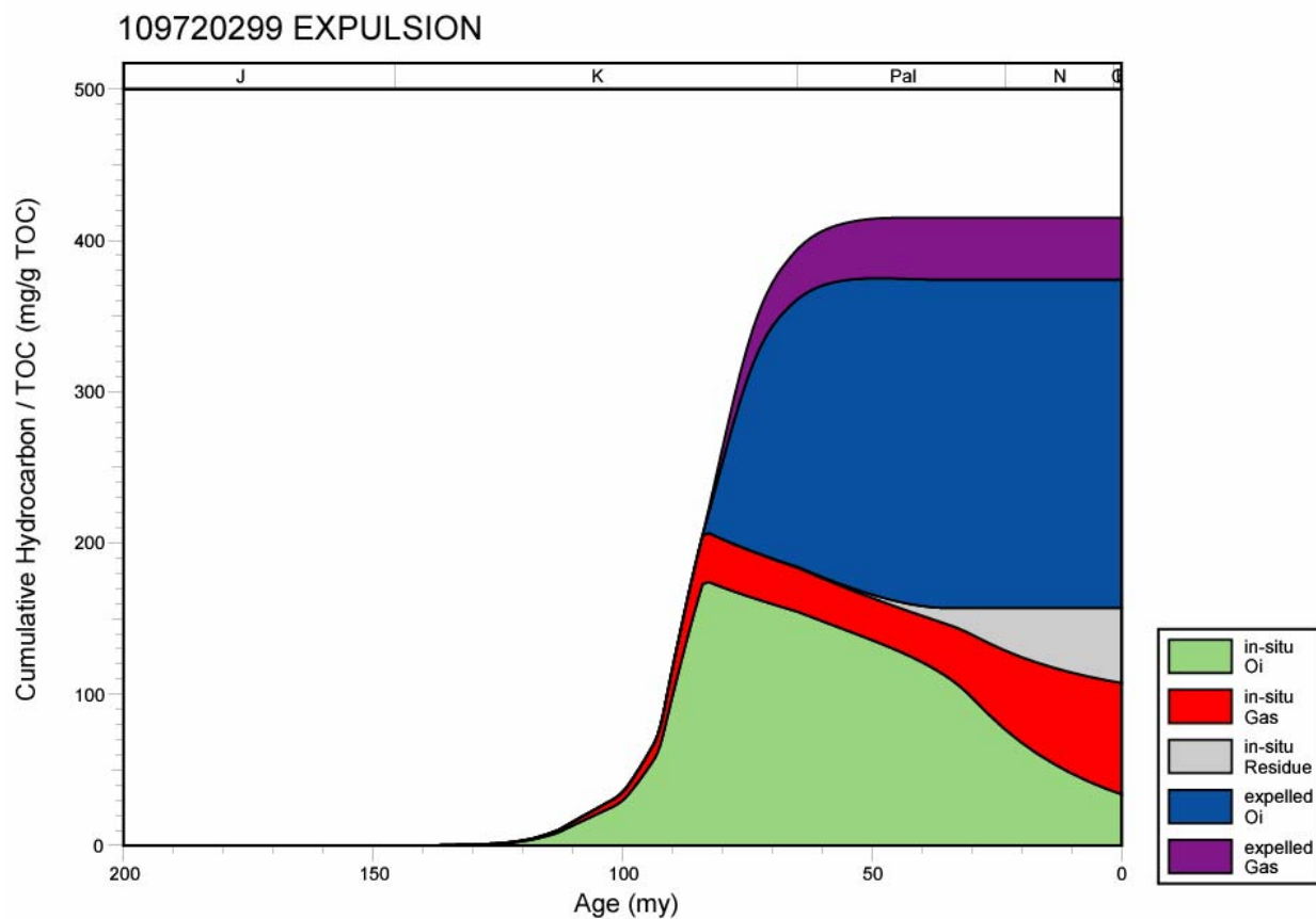
Figure 312. Hydrocarbon expulsion plot for well 109720299, Mississippi Interior Salt Basin.
