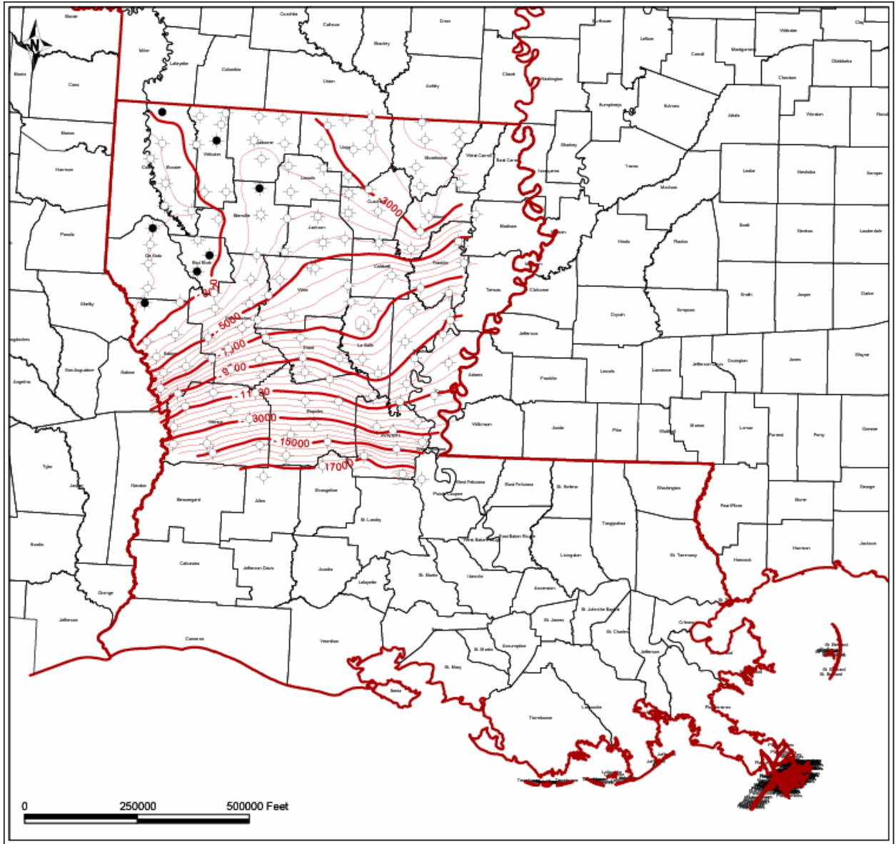
Figure 15. Structure map on the top of the Lower Cretaceous.
