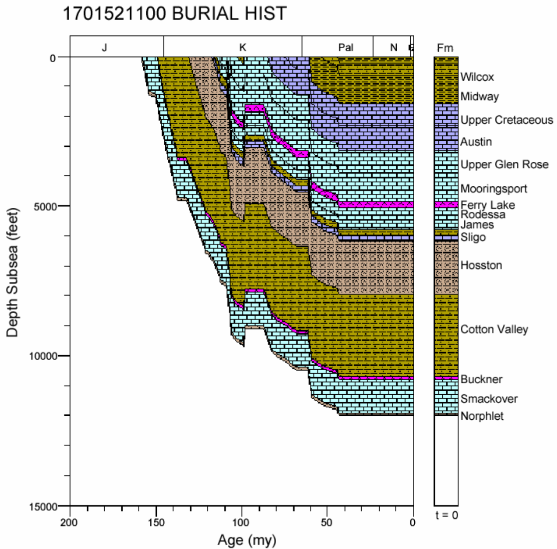
Figure 41. Burial history for well 1701521100, North Louisiana Salt Basin.
