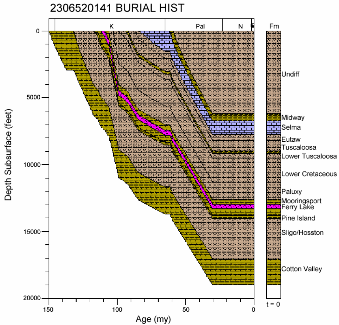
Figure 205. Burial history for well 2306520141, Mississippi Interior Salt Basin.
