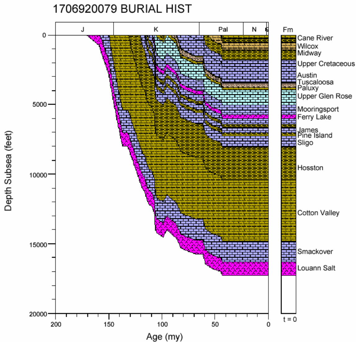
Figure 66. Burial history for well 1706920079, North Louisiana Salt Basin.
