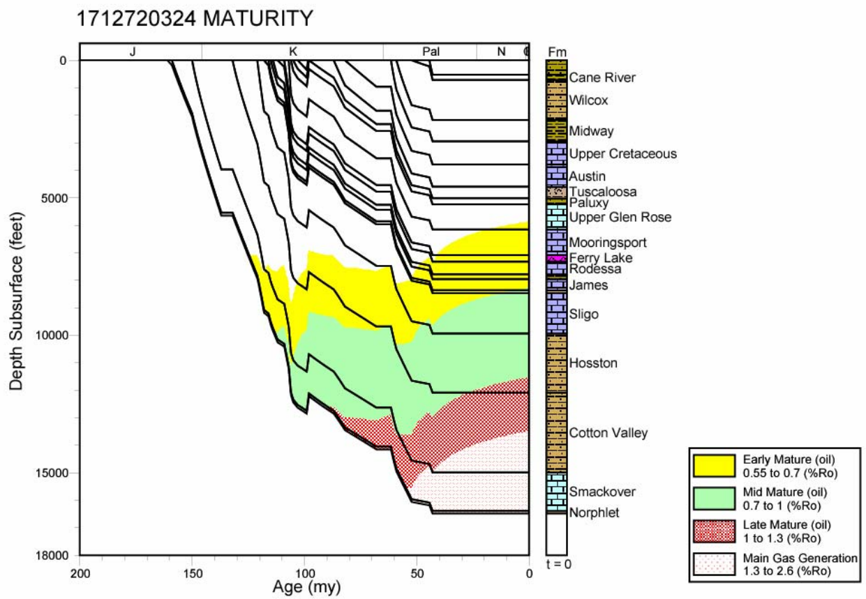
Figure 121. Thermal maturation profile for well 1712720324, North Louisiana Salt Basin.
