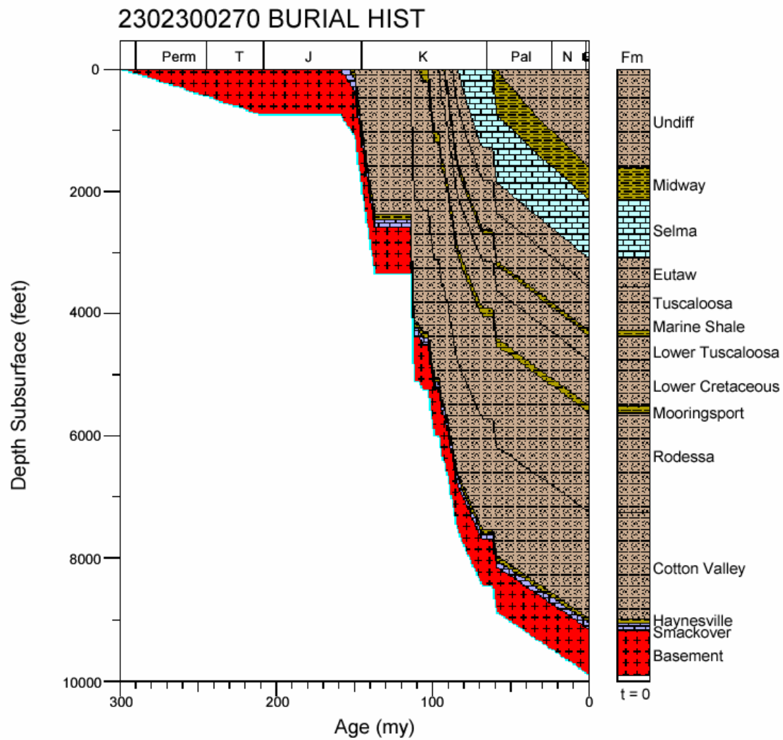
Figure 206. Burial history for well 2302300270, Mississippi Interior Salt Basin.
