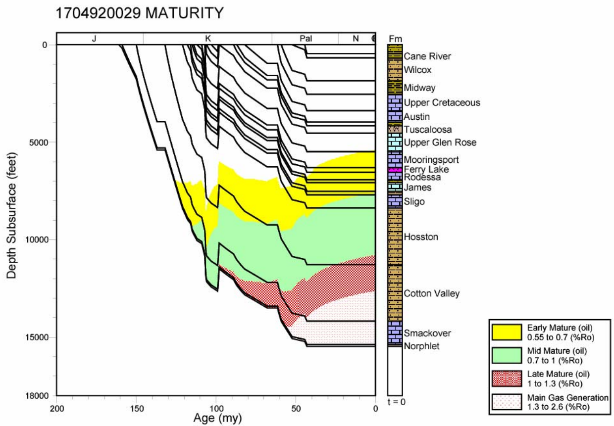
Figure 120. Thermal maturation profile for well 1704920029, North Louisiana Salt Basin.
