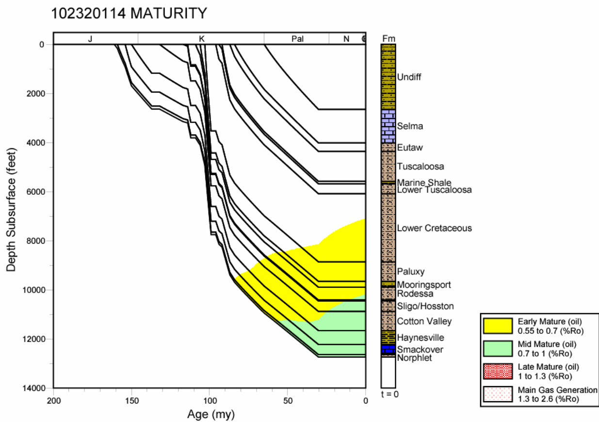
Figure 262. Thermal maturation profile for well 102320114, Mississippi Interior Salt Basin.
