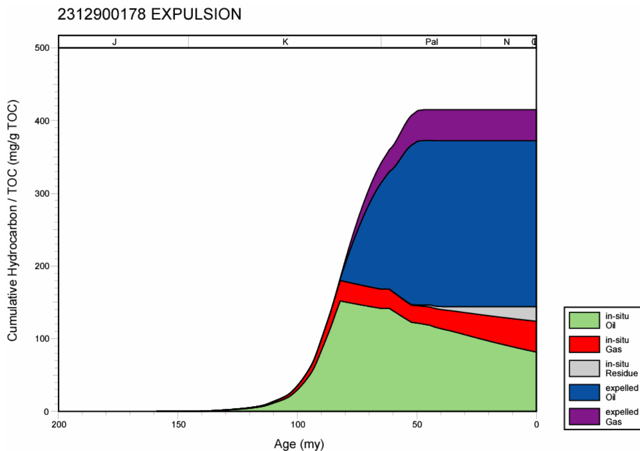
Figure 274. Hydrocarbon expulsion plot for well 2312900178, Mississippi Interior Salt Basin.
