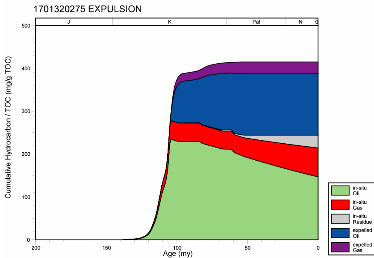
Figure 144. Hydrocarbon expulsion plot for well 1701320275, North Louisiana Salt Basin.
