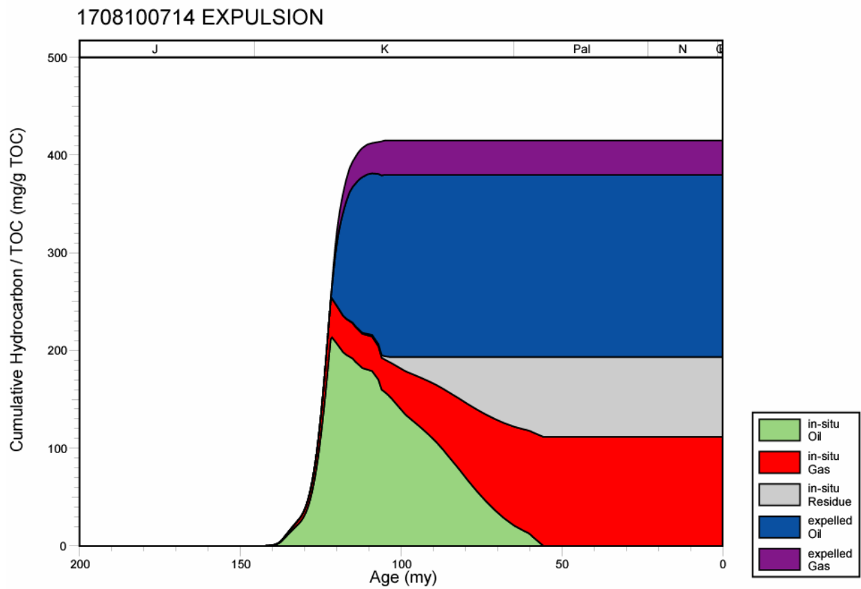
Figure 147. Hydrocarbon expulsion plot for well 1708100714, North Louisiana Salt Basin.
