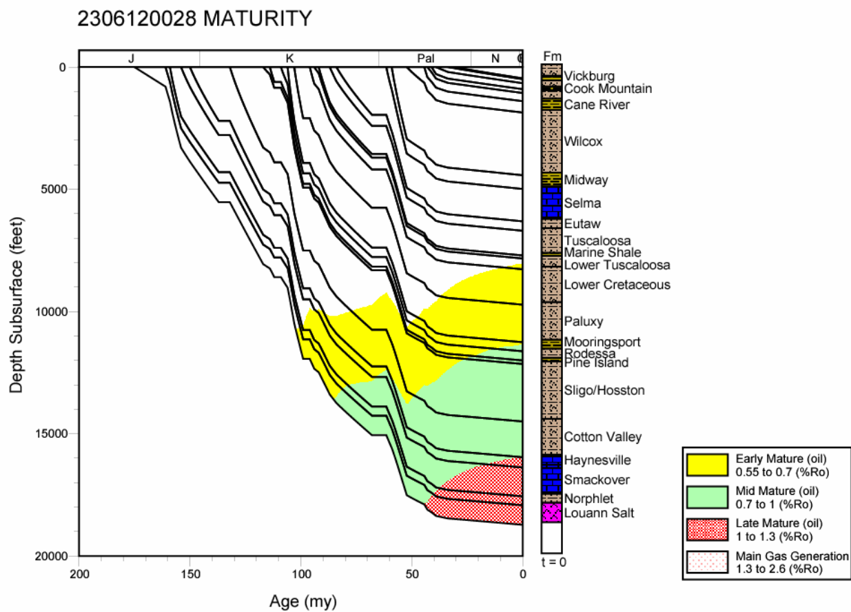
Figure 230. Thermal maturation profile for well 2306120028, Mississippi Interior Salt Basin.
