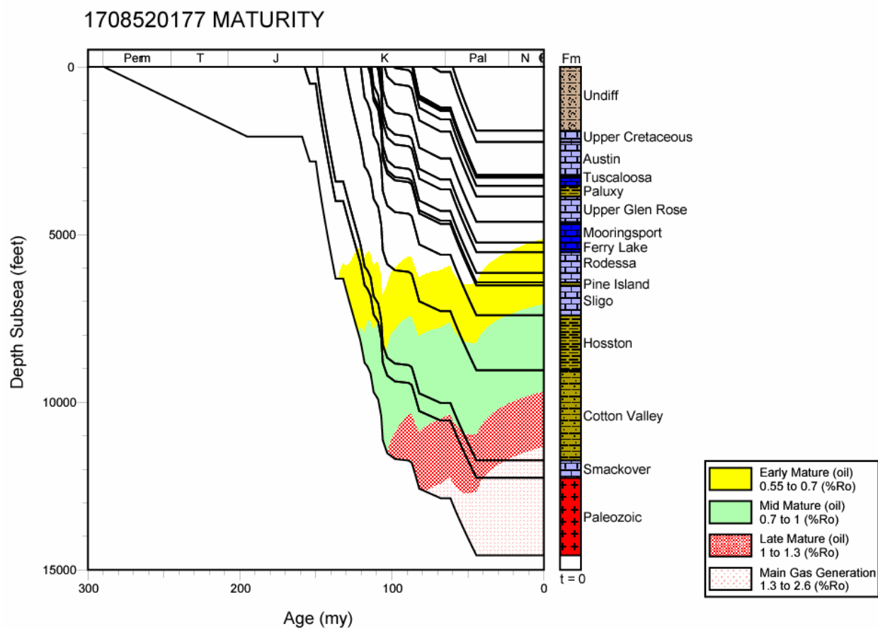
Figure 97. Thermal maturation profile for well 1708520177, North Louisiana Salt Basin.
