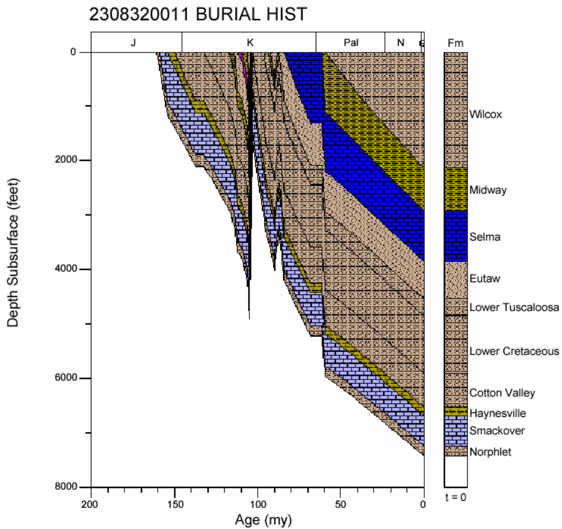
Figure 191. Burial history for well 2308320011, Mississippi Interior Salt Basin.
