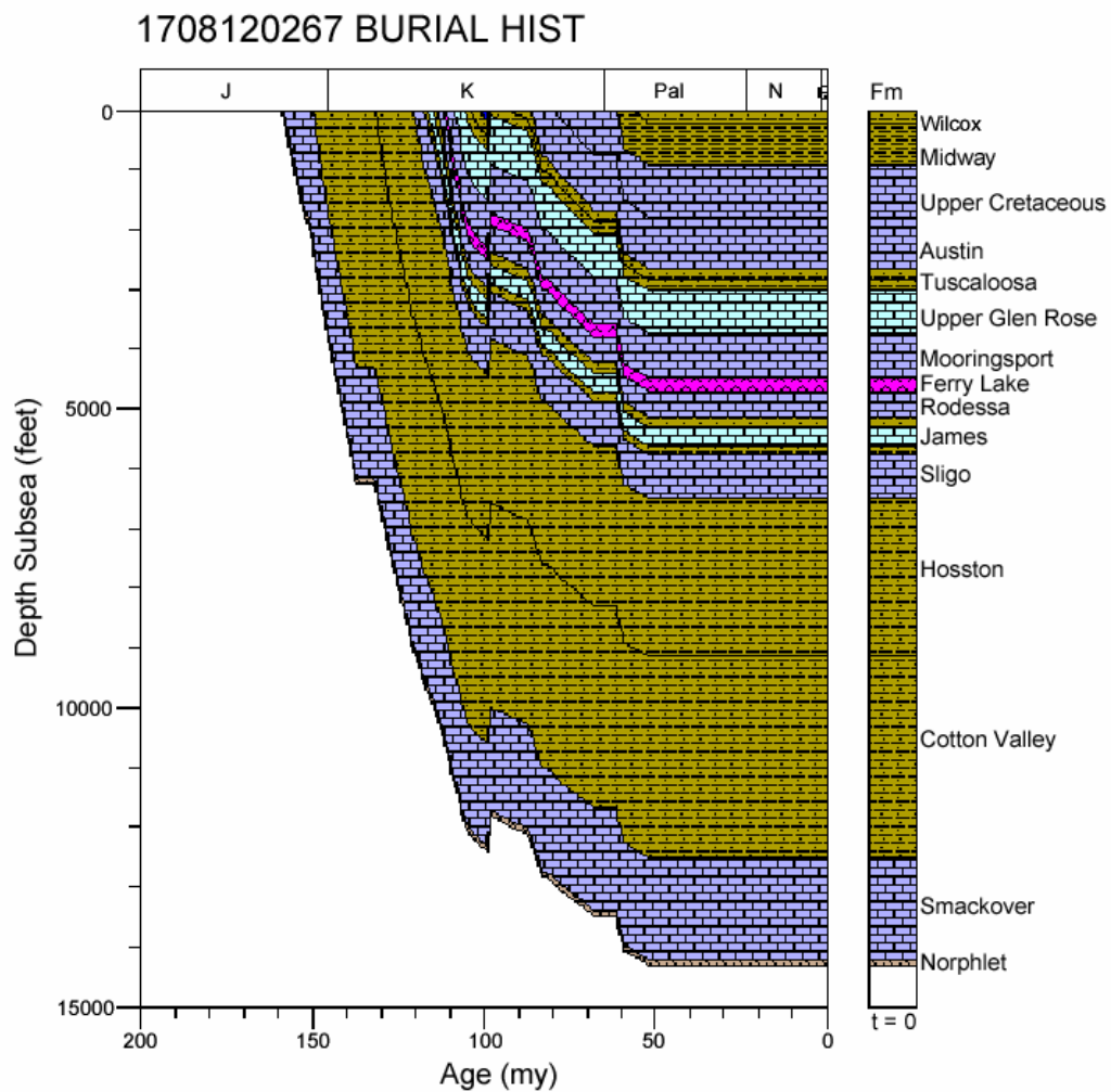
Figure 58. Burial history for well 1708120267, North Louisiana Salt Basin.
