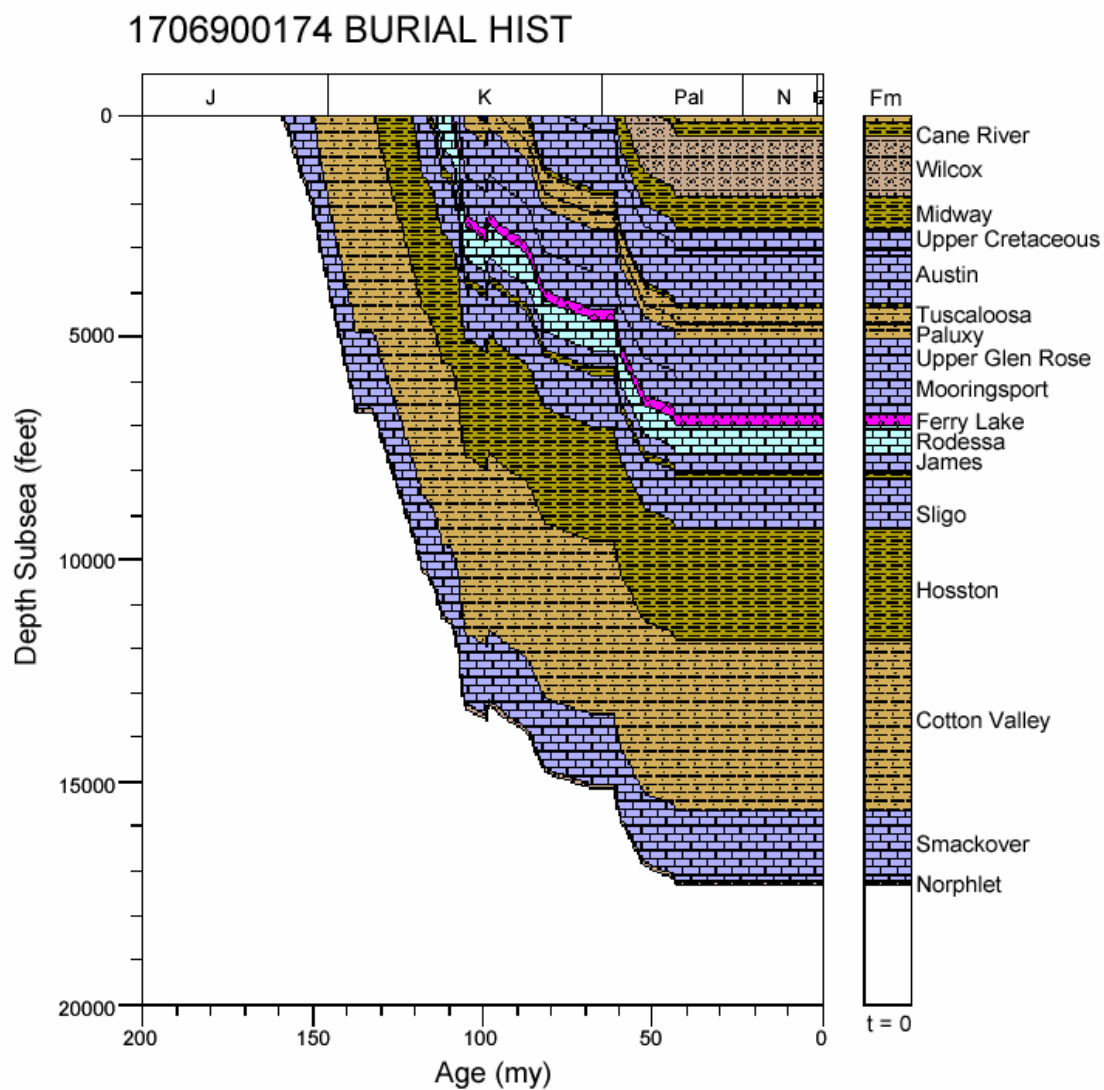
Figure 68. Burial history for well 1706900174, North Louisiana Salt Basin.
