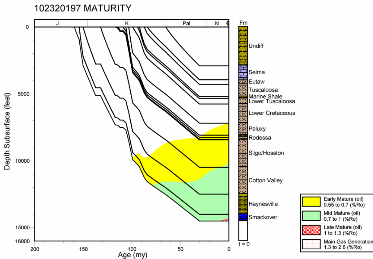
Figure 263. Thermal maturation profile for well 102320197, Mississippi Interior Salt Basin.
