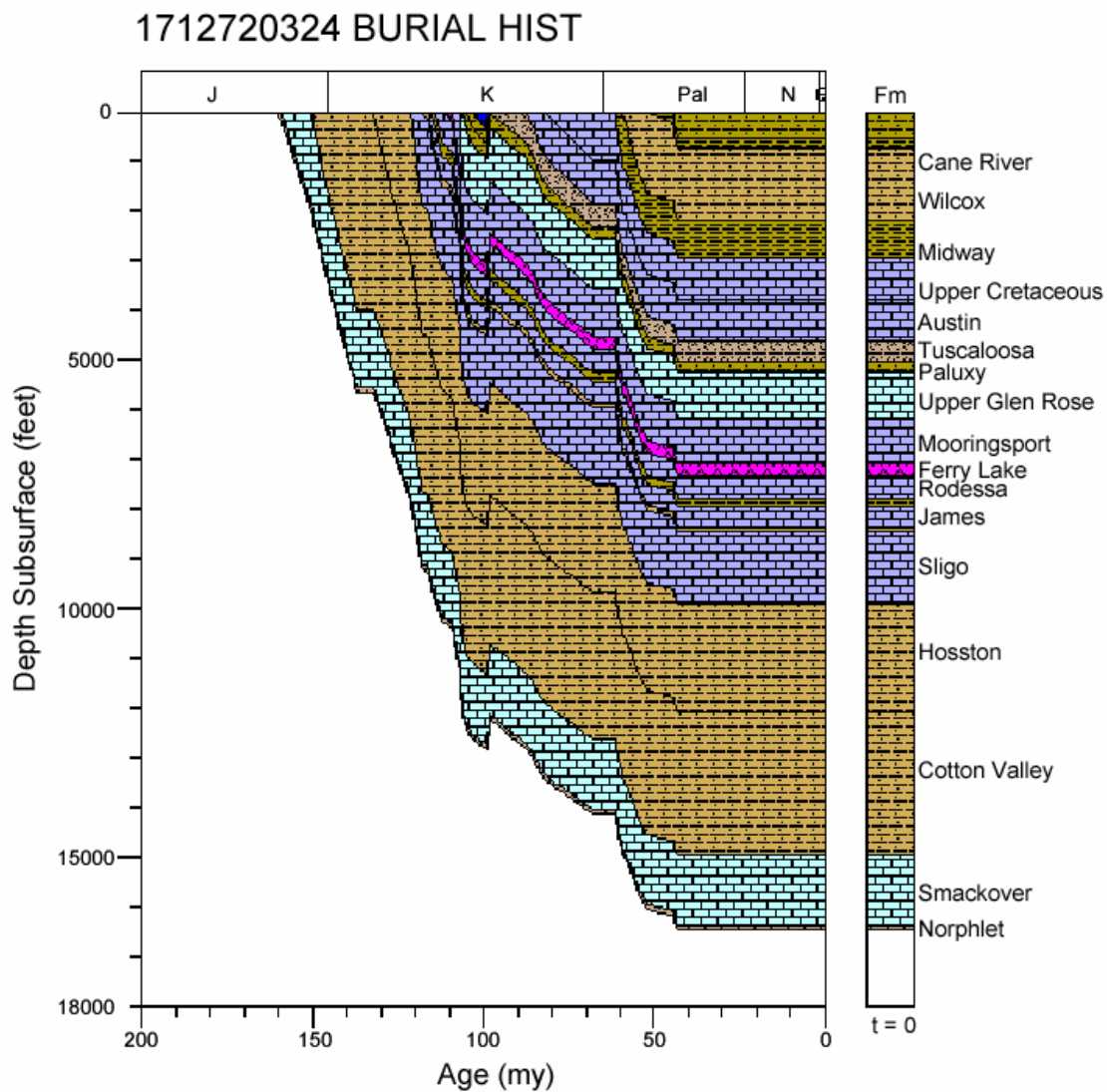
Figure 75. Burial history for well 1712720324, North Louisiana Salt Basin.
