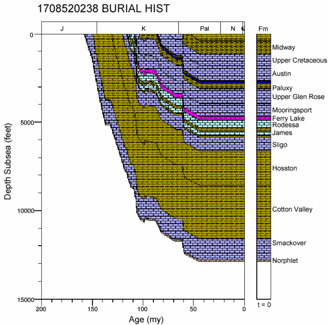
Figure 50. Burial history for well 1708520238, North Louisiana Salt Basin.
