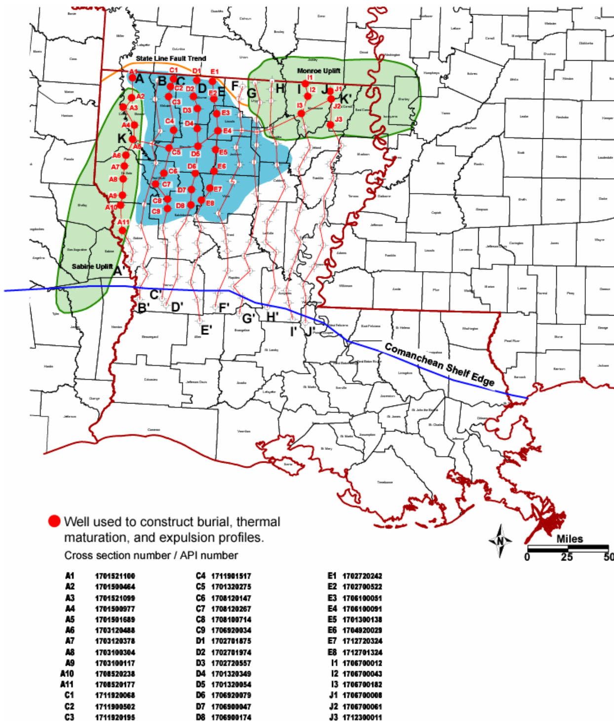
Figure 2. Index map showing line of cross sections and location of selected wells for the North Louisiana Salt Basin.
