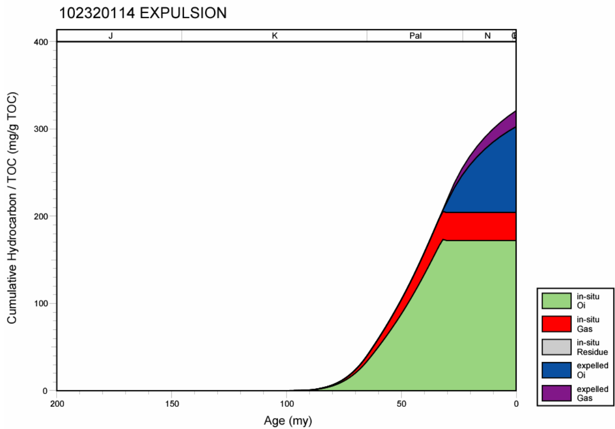
Figure 307. Hydrocarbon expulsion plot for well 102320114, Mississippi Interior Salt Basin.
