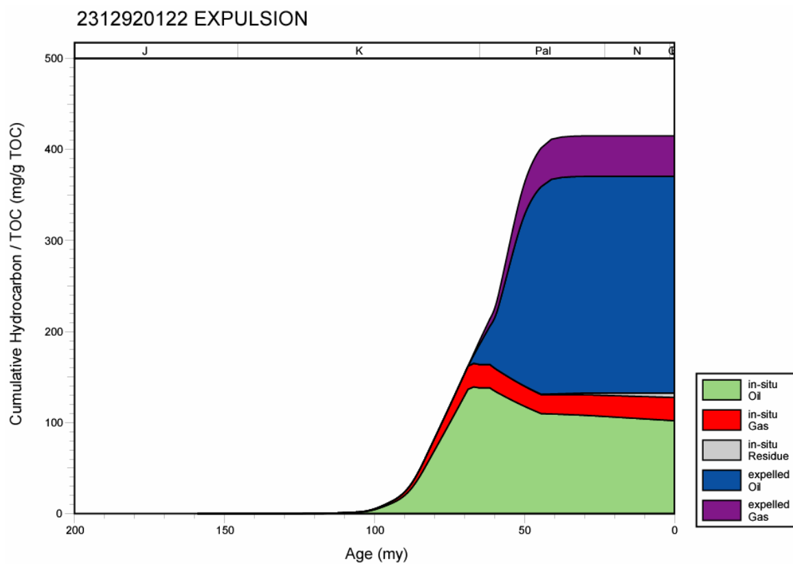
Figure 297. Hydrocarbon expulsion plot for well 2312920122, Mississippi Interior Salt Basin.
