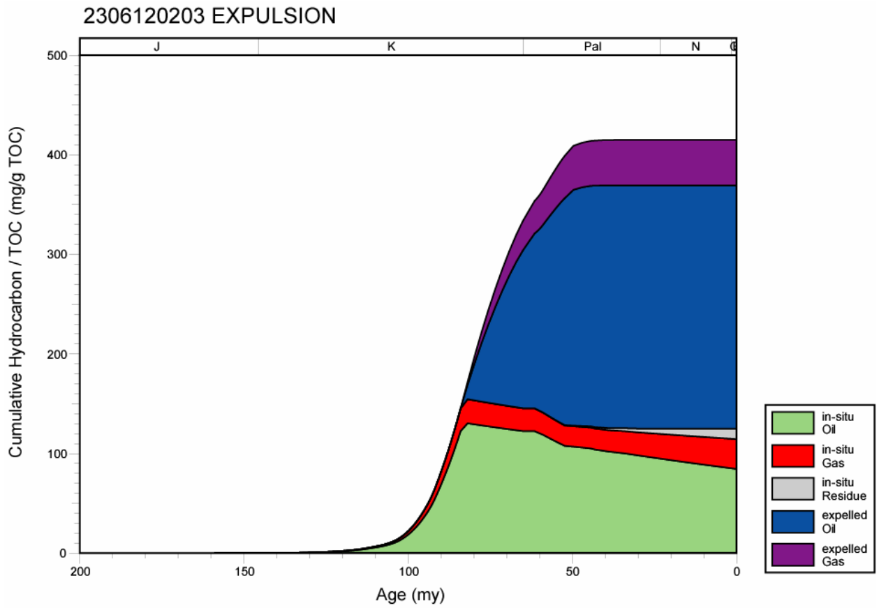
Figure 277. Hydrocarbon expulsion plot for well 2306120203, Mississippi Interior Salt Basin.
