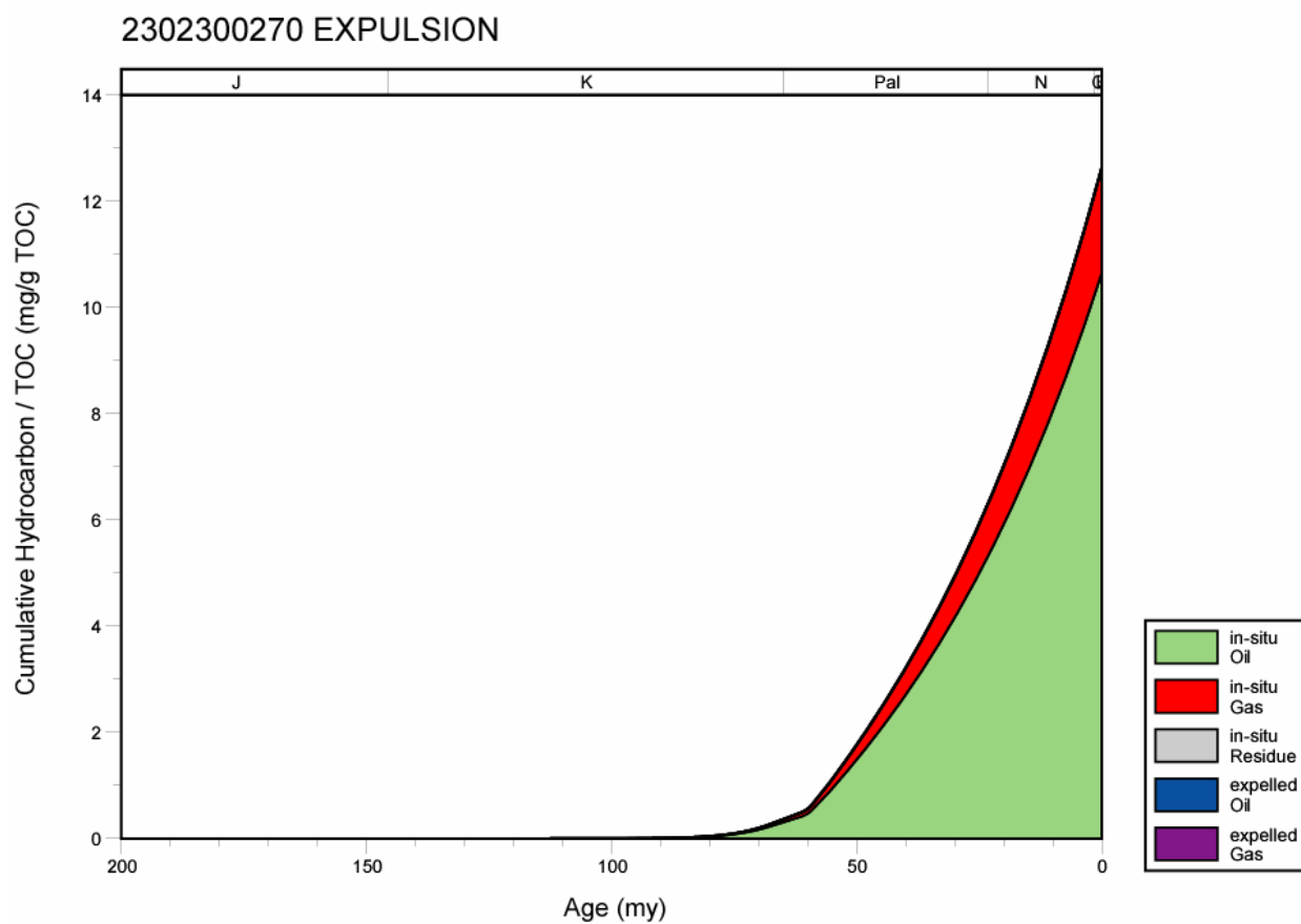
Figure 299. Hydrocarbon expulsion plot for well 2302300270, Mississippi Interior Salt Basin.
