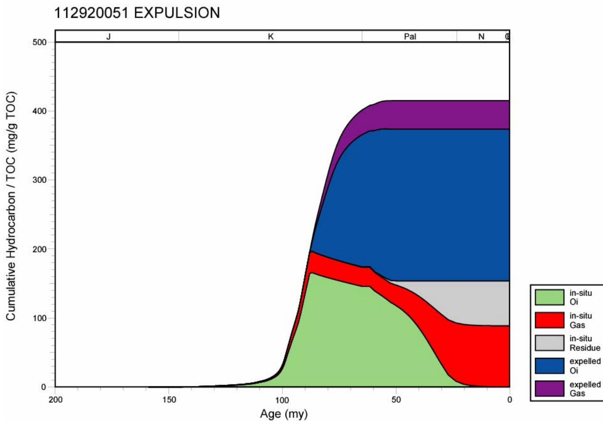
Figure 309. Hydrocarbon expulsion plot for well 112920051, Mississippi Interior Salt Basin.
