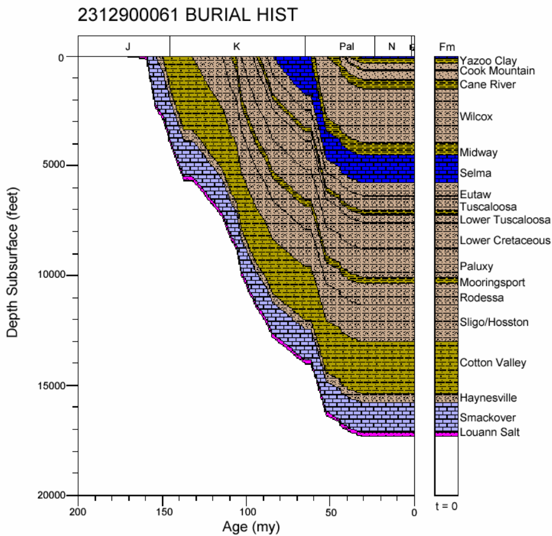
Figure 180. Burial history for well 2312900061, Mississippi Interior Salt Basin.
