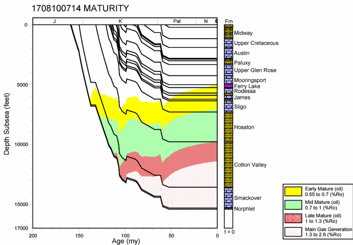
Figure 105. Thermal maturation profile for well 1708100714, North Louisiana Salt Basin.
