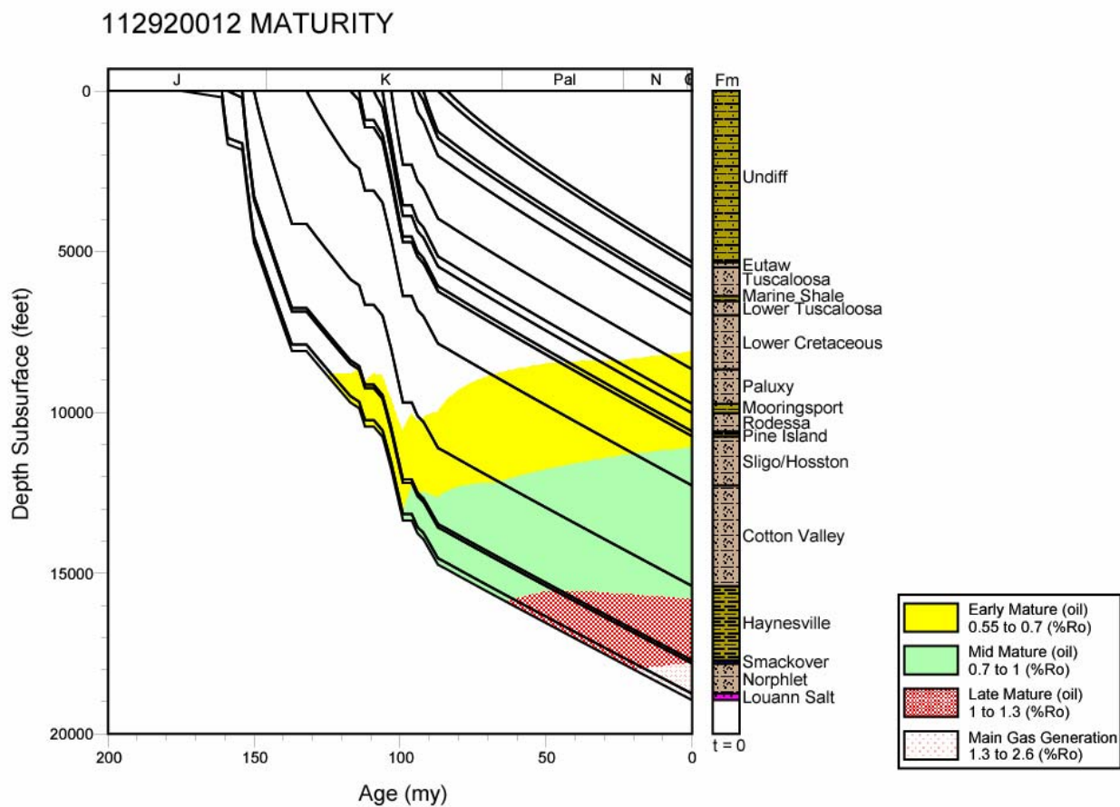
Figure 238. Thermal maturation profile for well 112920012, Mississippi Interior Salt Basin.
