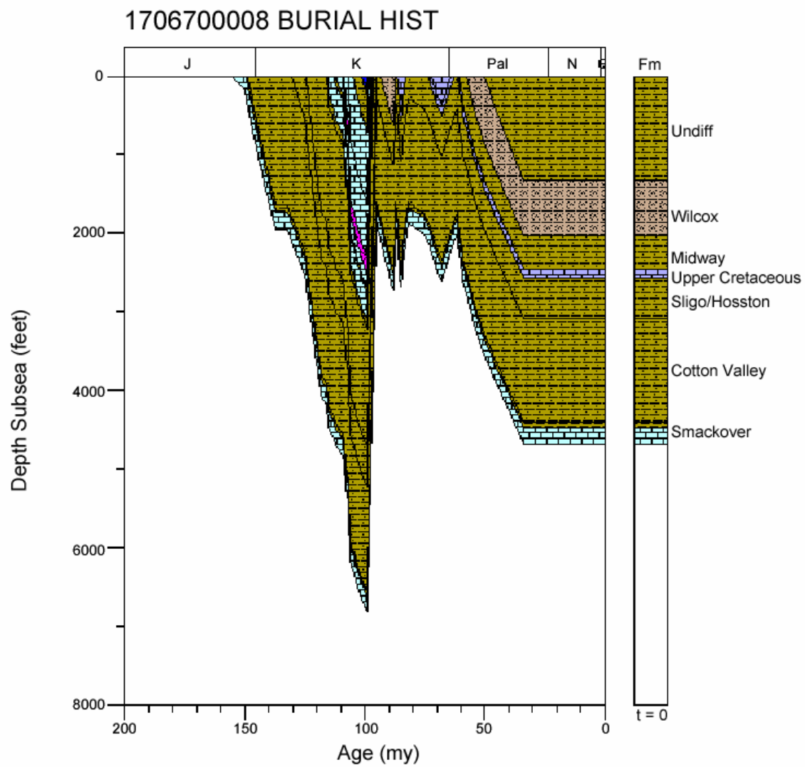
Figure 80. Burial history for well 1706700008, North Louisiana Salt Basin.
