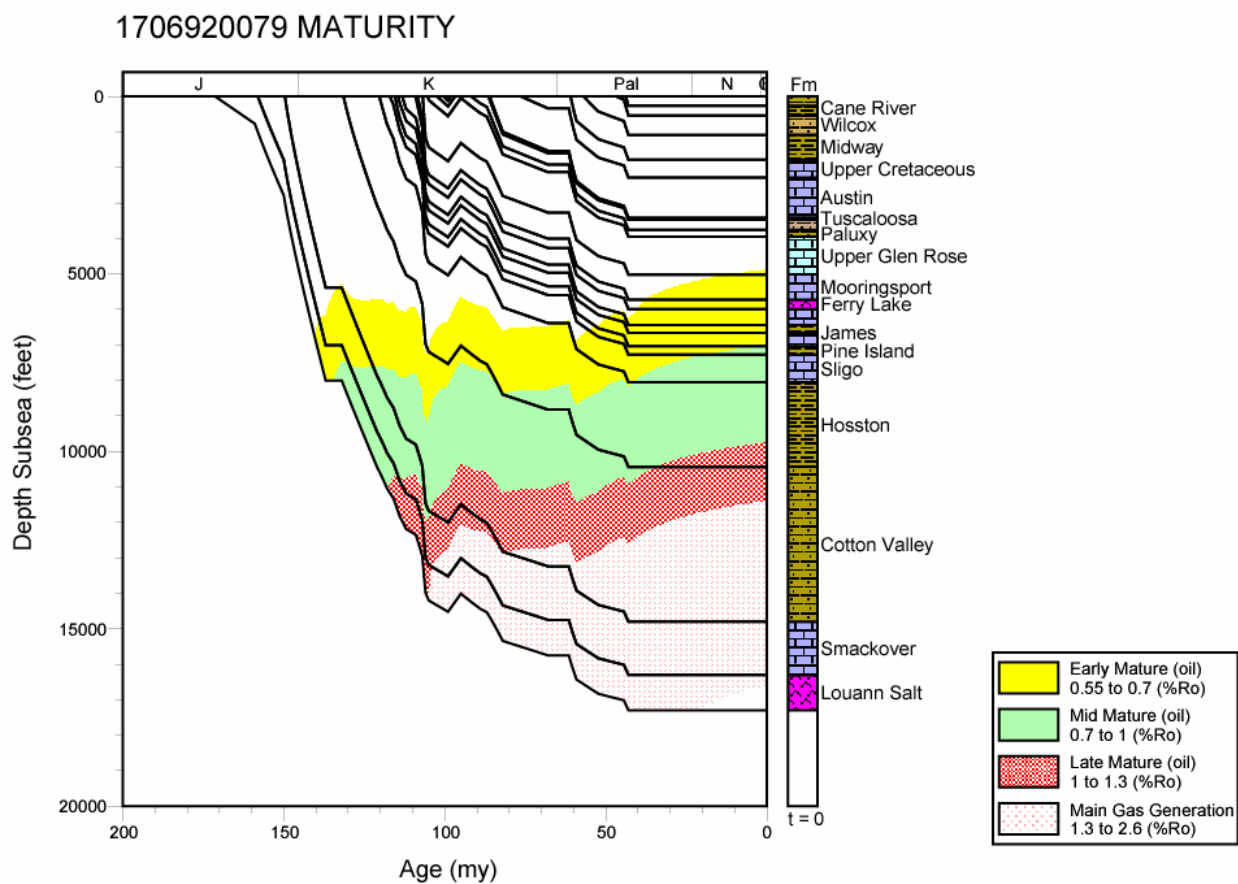
Figure 112. Thermal maturation profile for well 1706920079, North Louisiana Salt Basin.
