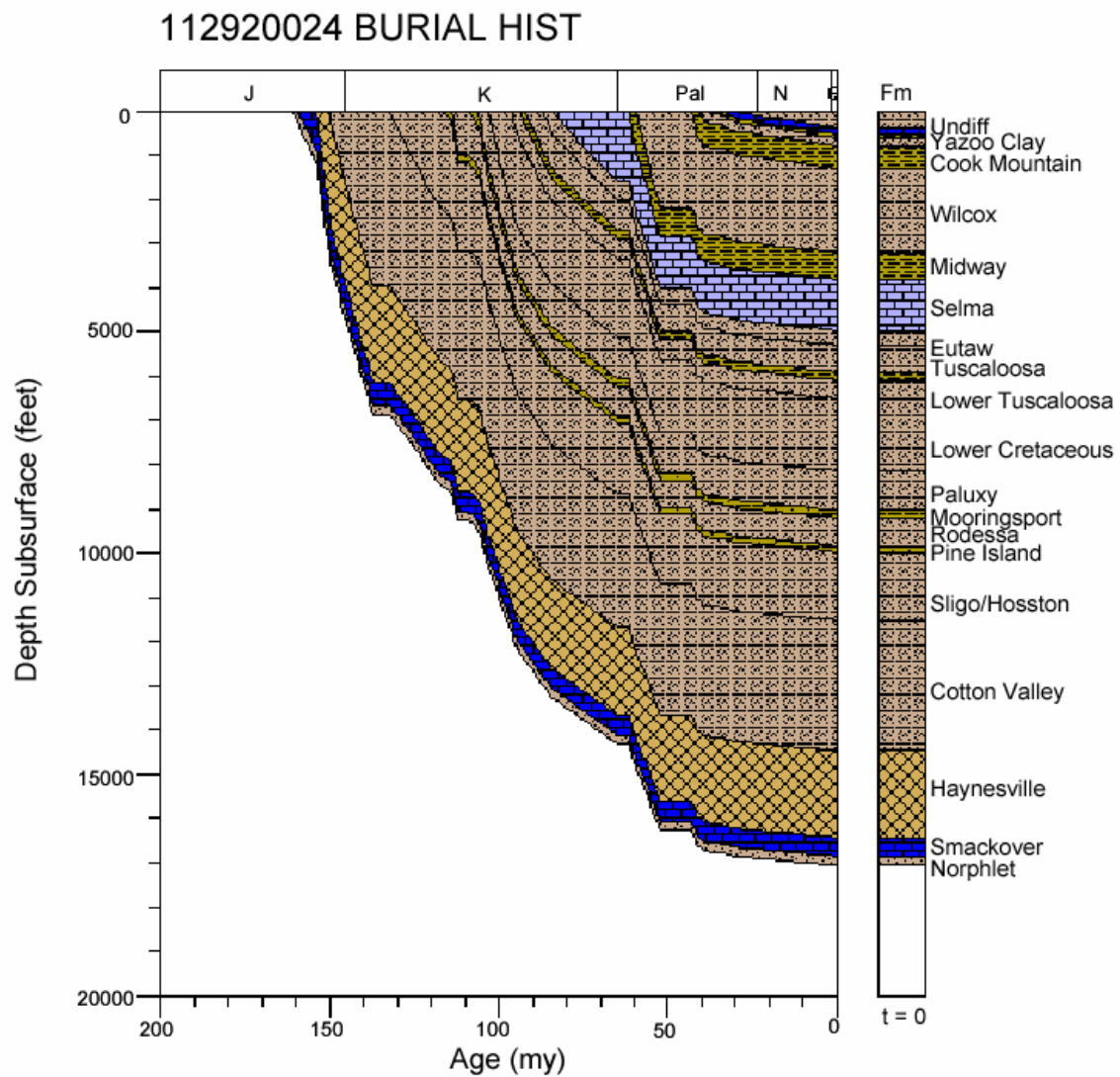
Figure 189. Burial history for well 112920024, Mississippi Interior Salt Basin.
