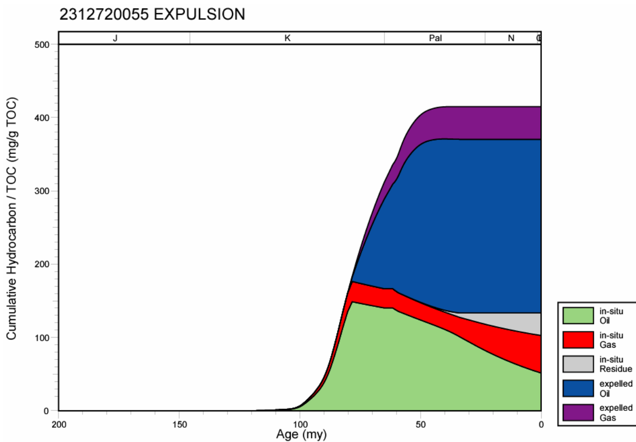
Figure 298. Hydrocarbon expulsion plot for well 2312720055, Mississippi Interior Salt Basin.
