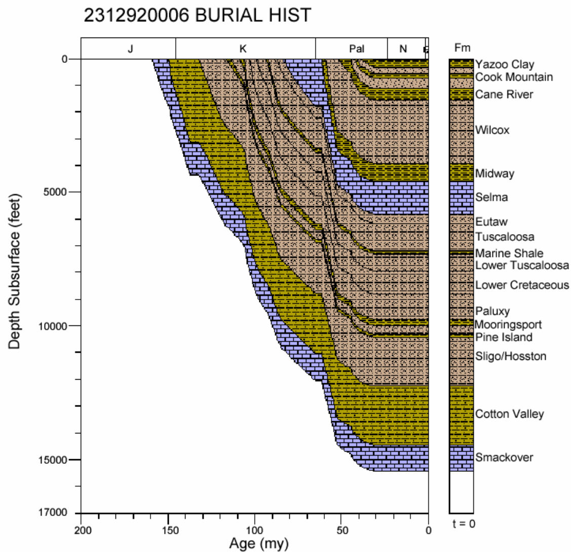
Figure 179. Burial history for well 2312920006, Mississippi Interior Salt Basin.
