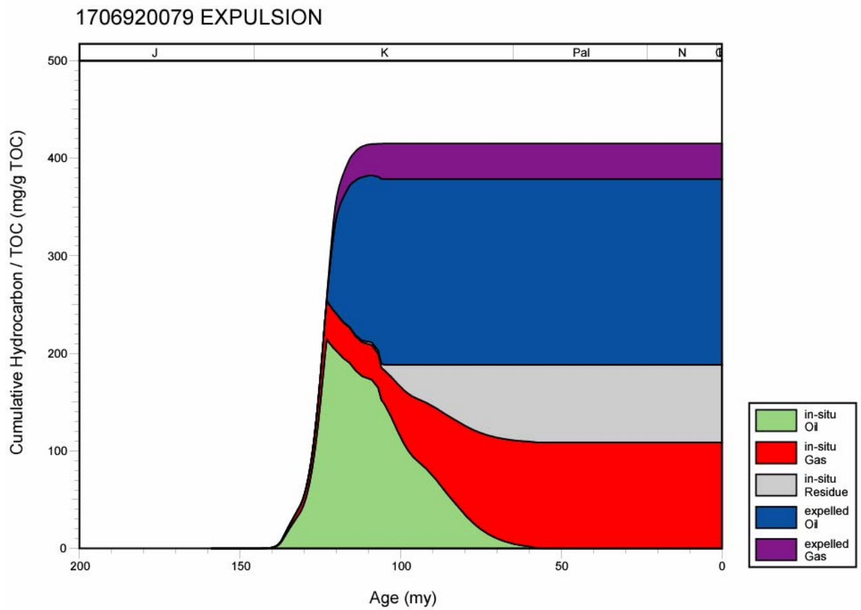
Figure 154. Hydrocarbon expulsion plot for well 1706920079, North Louisiana Salt Basin.
