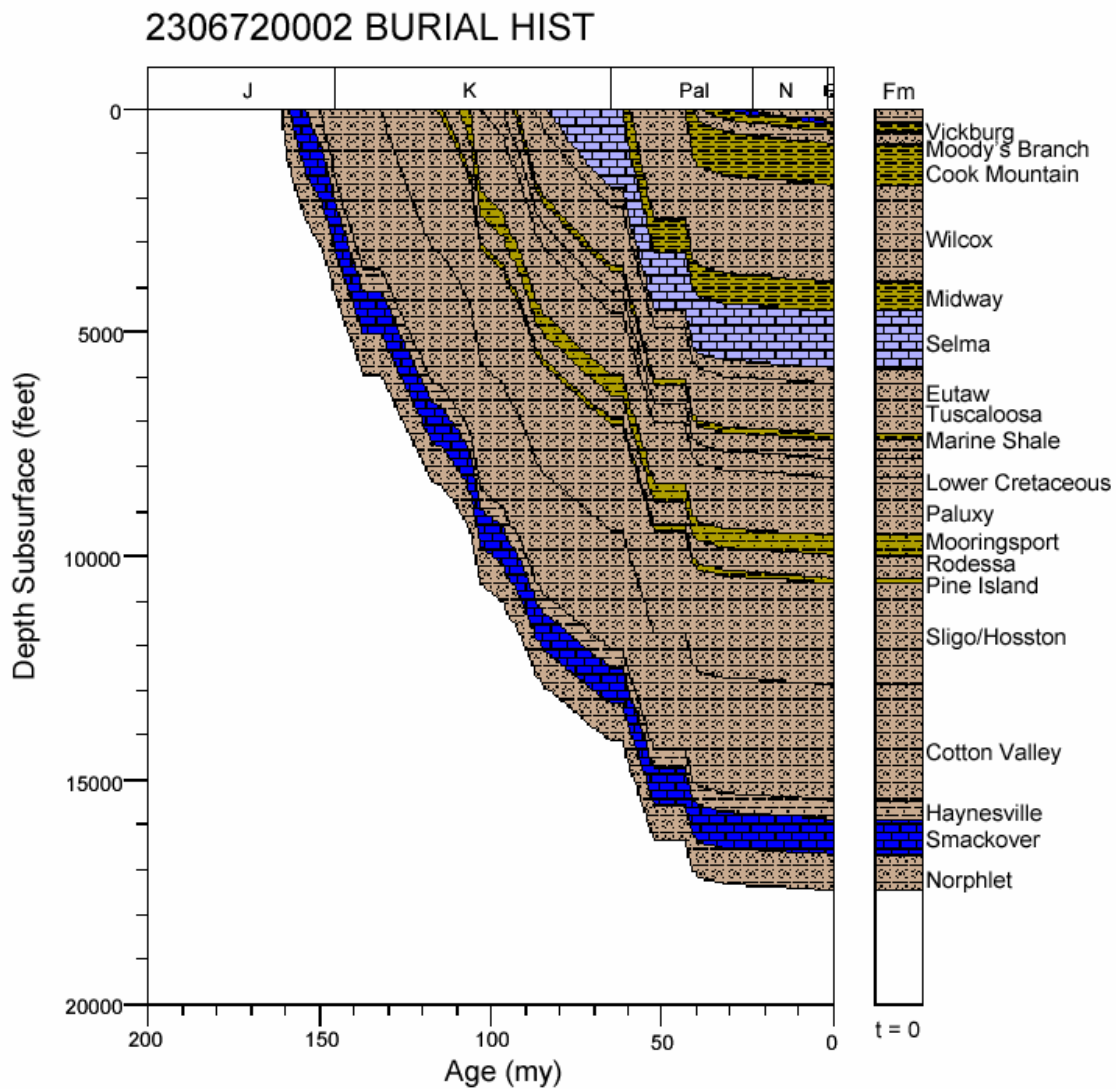
Figure 184. Burial history for well 2306720002, Mississippi Interior Salt Basin.
