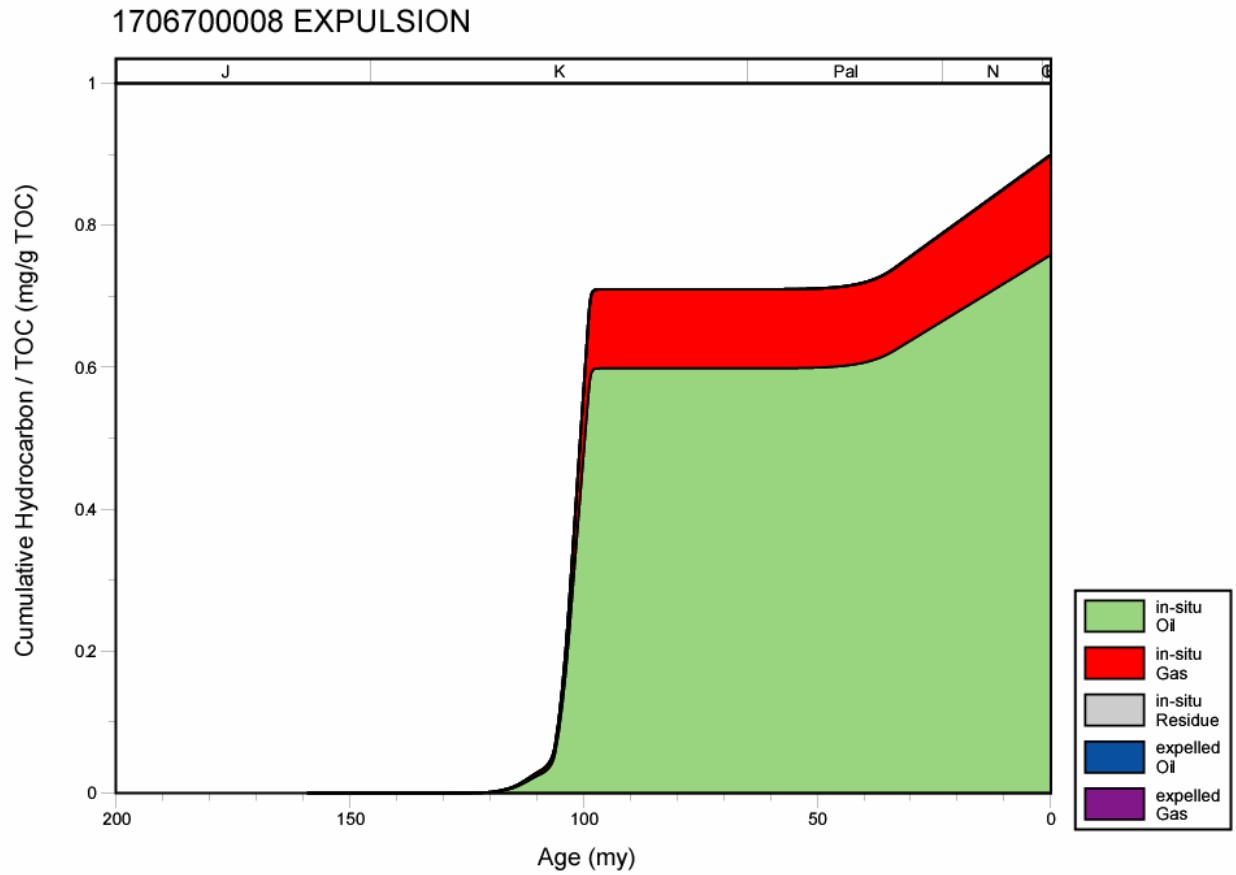
Figure 168. Hydrocarbon expulsion plot for well 1706700008, North Louisiana Salt Basin.
