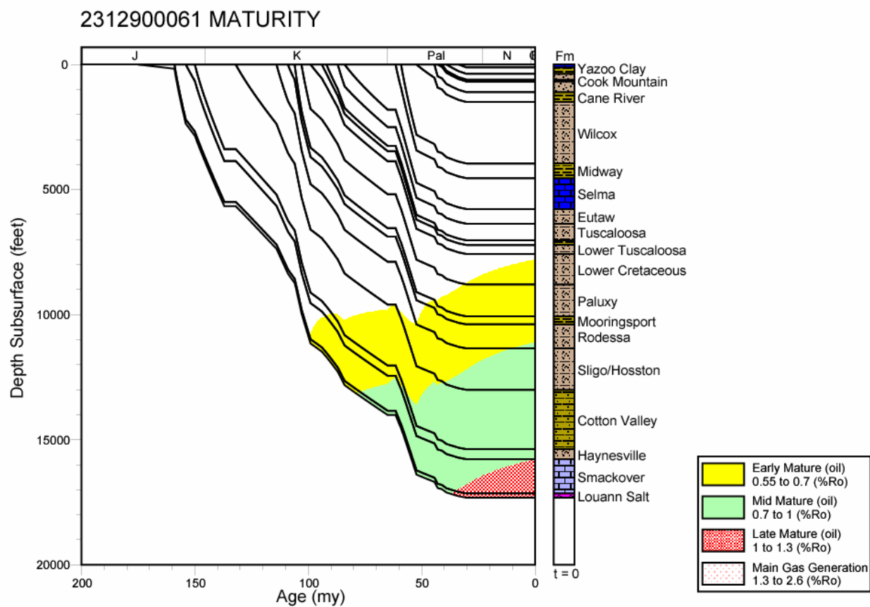
Figure 228. Thermal maturation profile for well 2312900061, Mississippi Interior Salt Basin.
