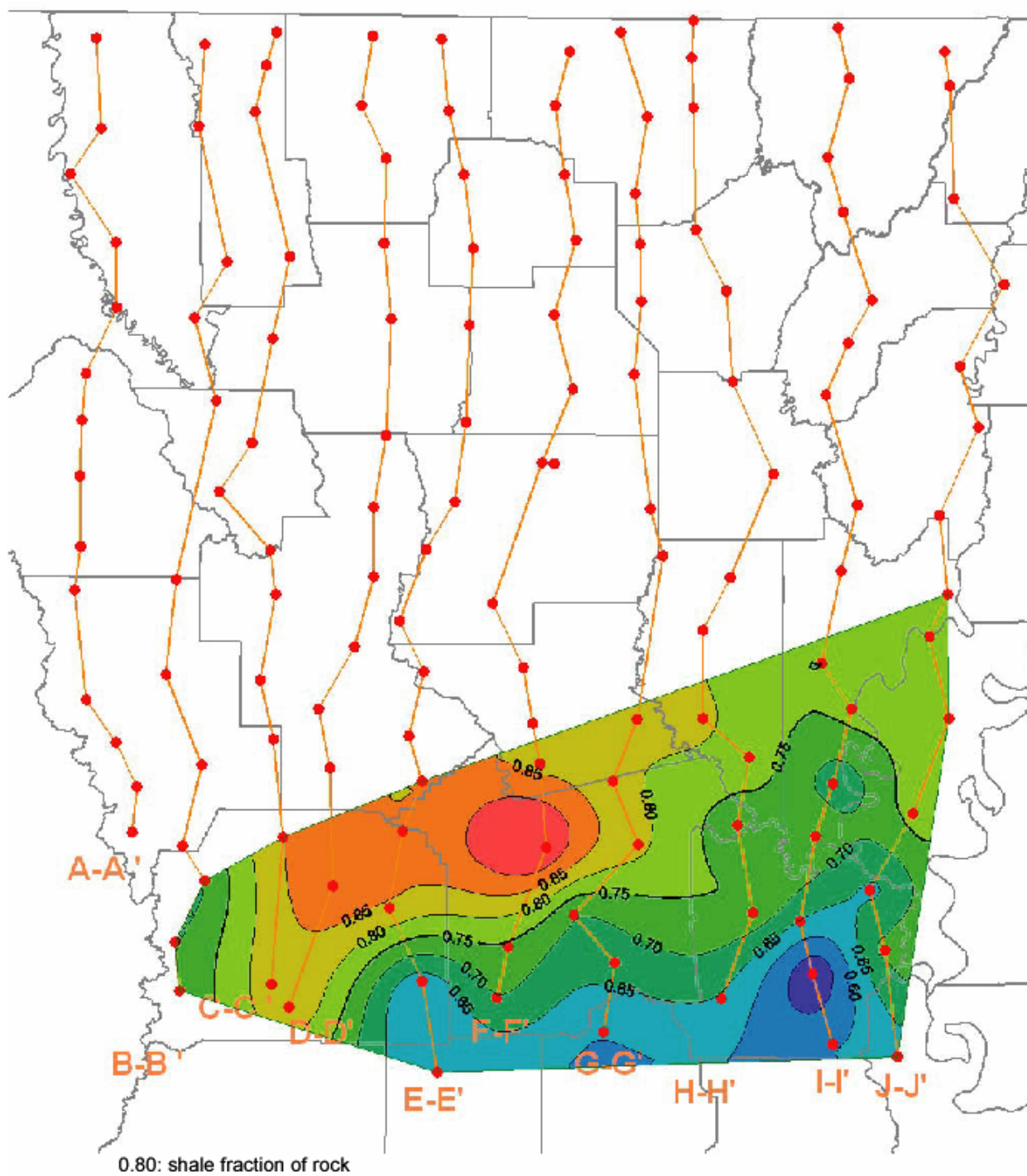
Figure 22. Lithology map of Oligocene strata. Prepared by Roger Barnaby.
