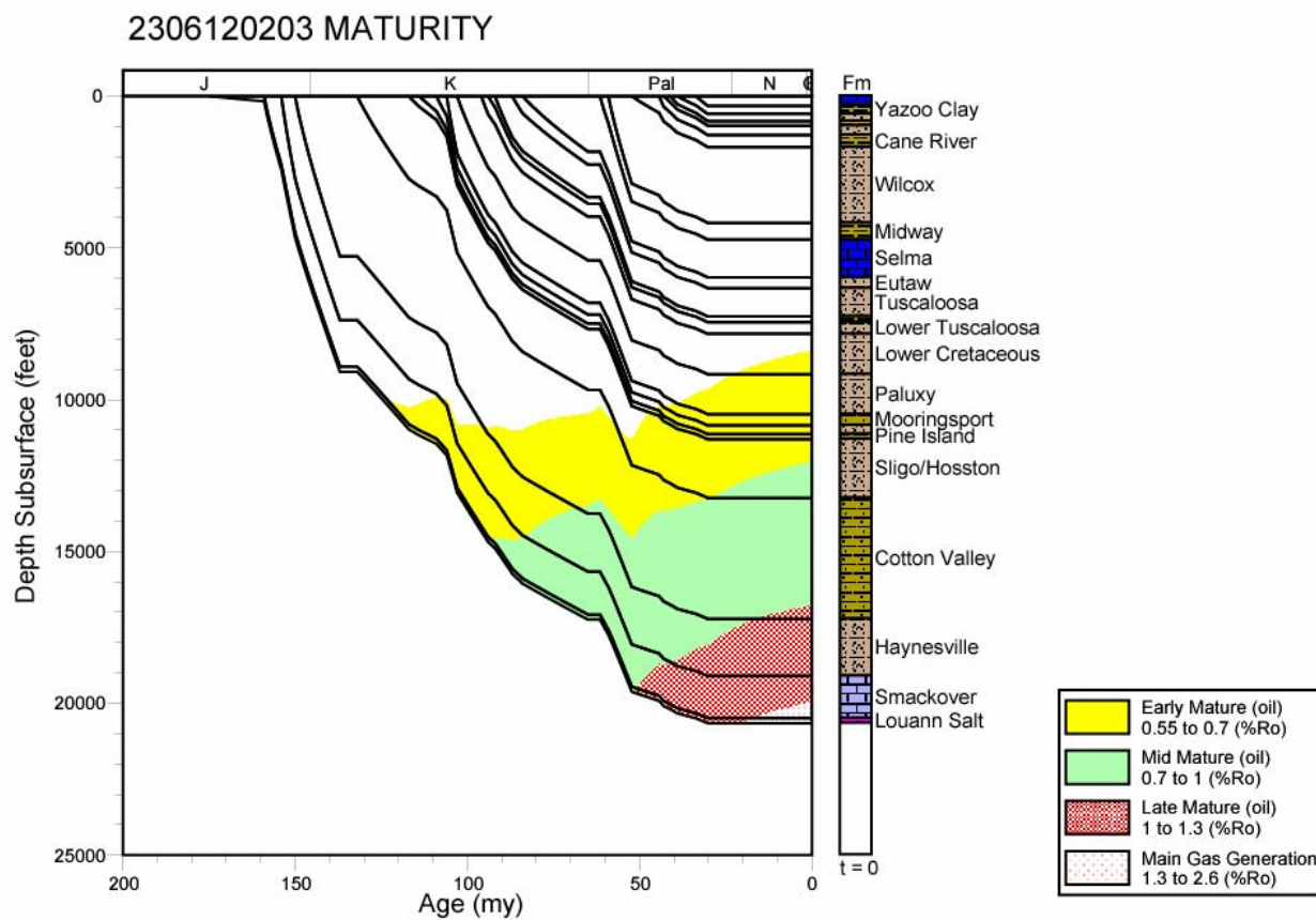
Figure 229. Thermal maturation profile for well 2306120203, Mississippi Interior Salt Basin.
