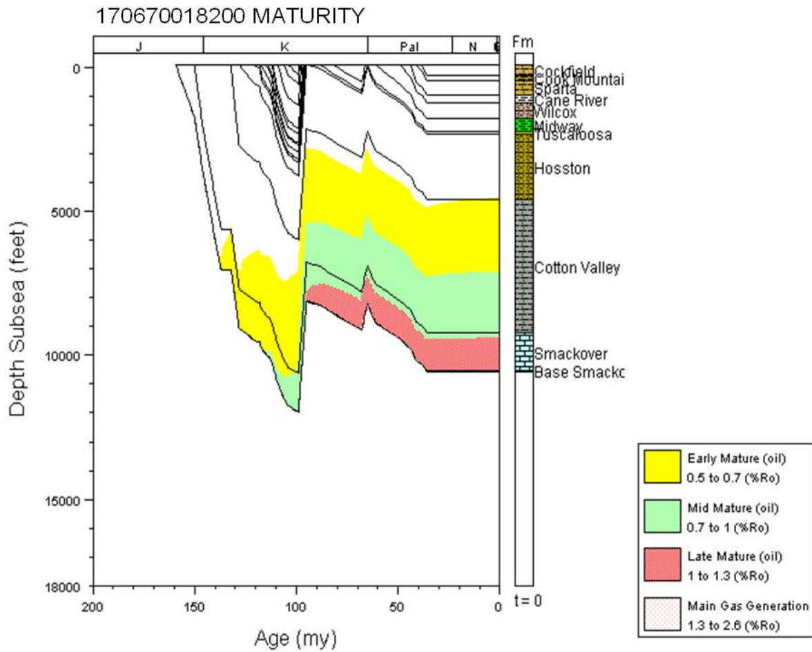
Figure 319. Thermal maturation profile for well 170670018200. Monroe Uplift. Prepared by Roger Barnaby.
