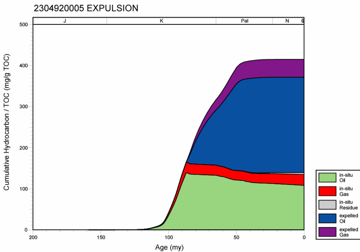
Figure 272. Hydrocarbon expulsion plot for well 2304920005, Mississippi Interior Salt Basin.
