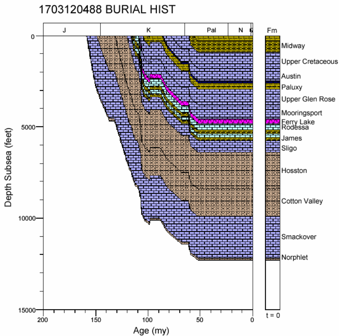
Figure 46. Burial history for well 1703120488, North Louisiana Salt Basin.
