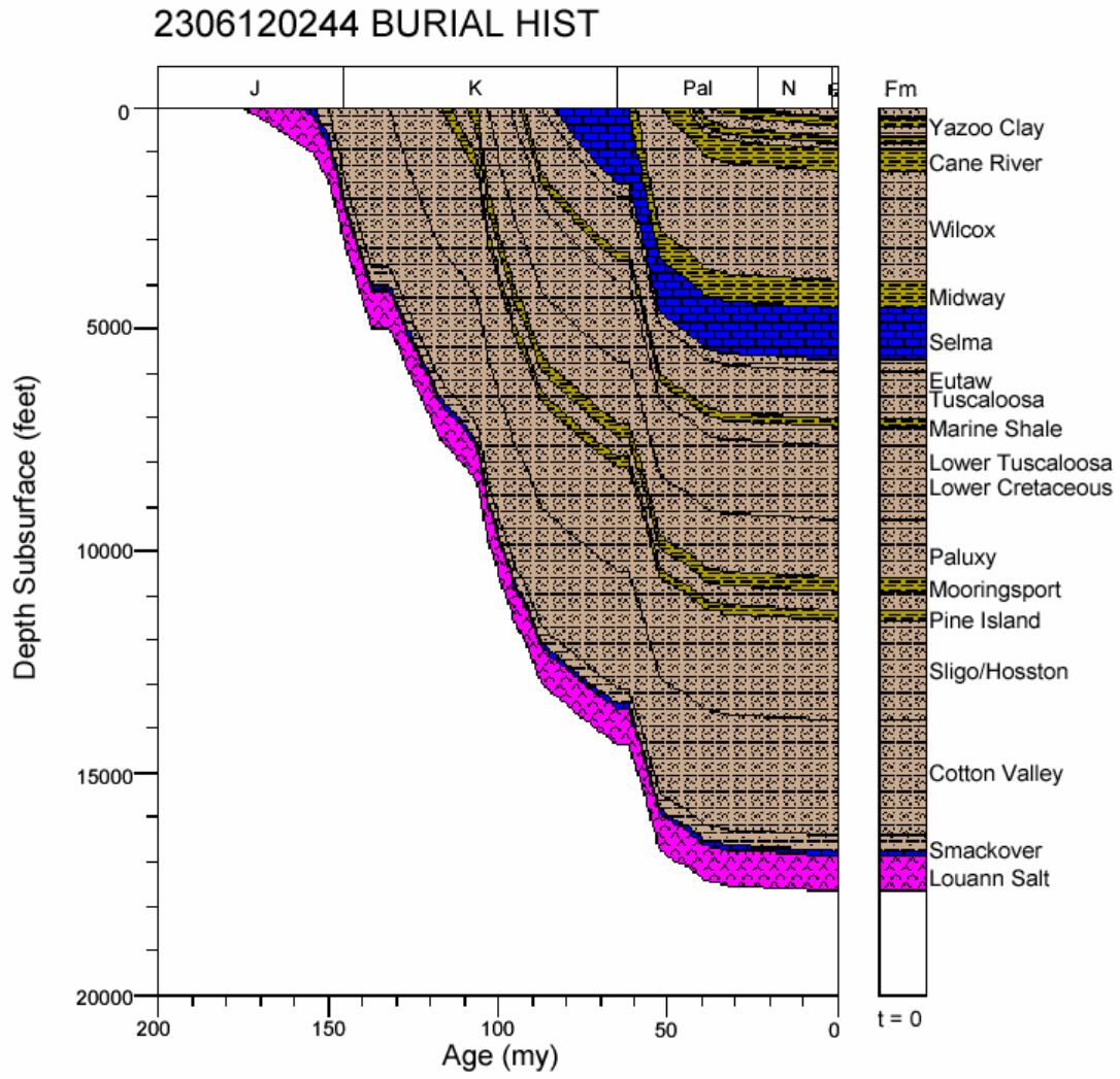
Figure 183. Burial history for well 2306120244, Mississippi Interior Salt Basin.
