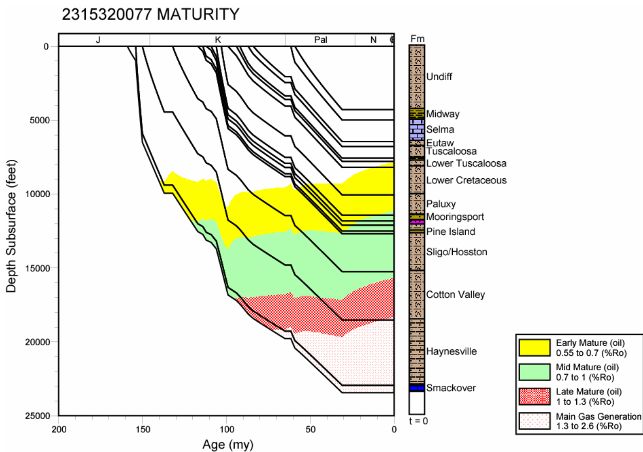
Figure 259. Thermal maturation profile for well 2315320077, Mississippi Interior Salt Basin.
