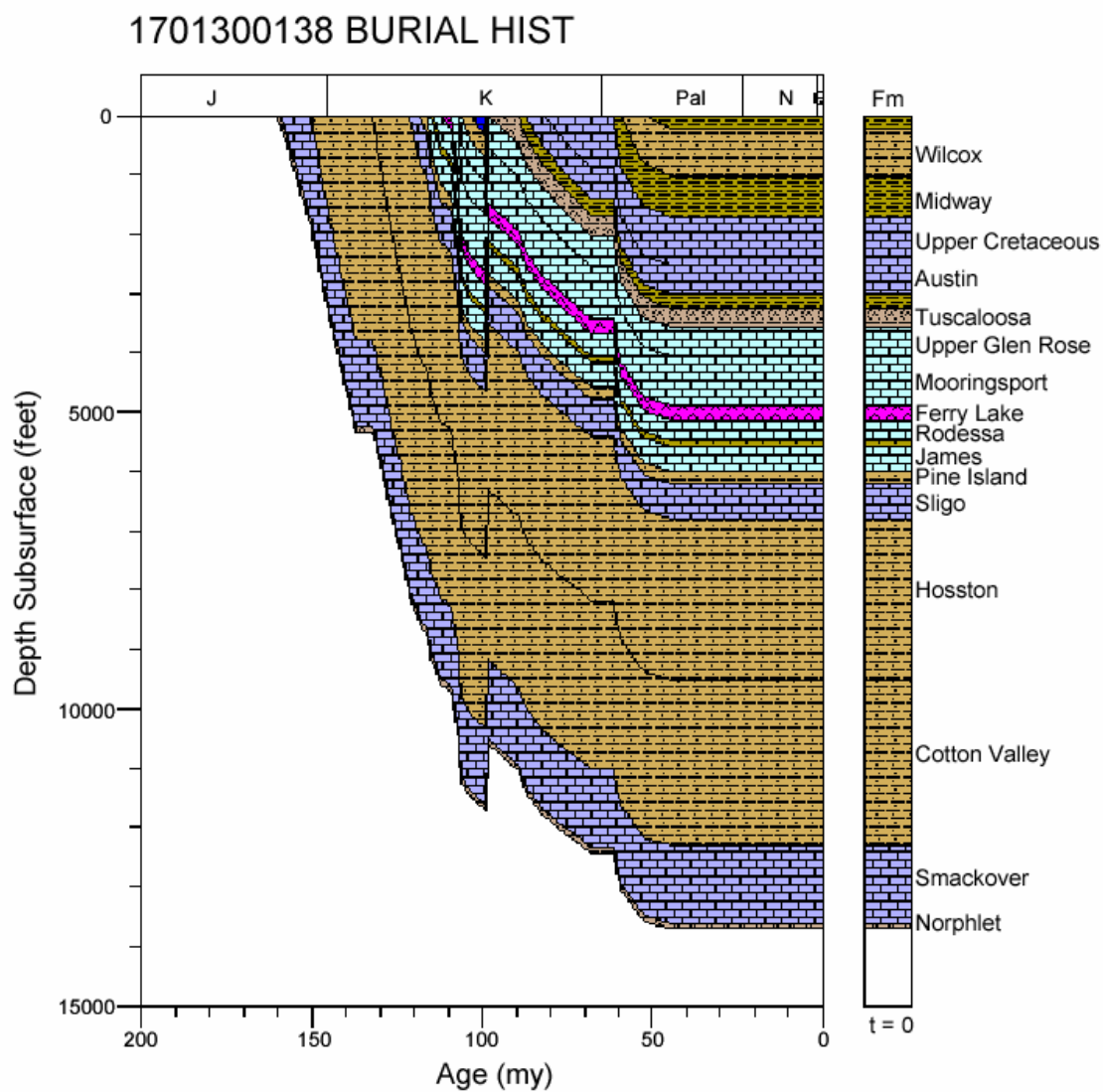
Figure 73. Burial history for well 1701300138, North Louisiana Salt Basin.
