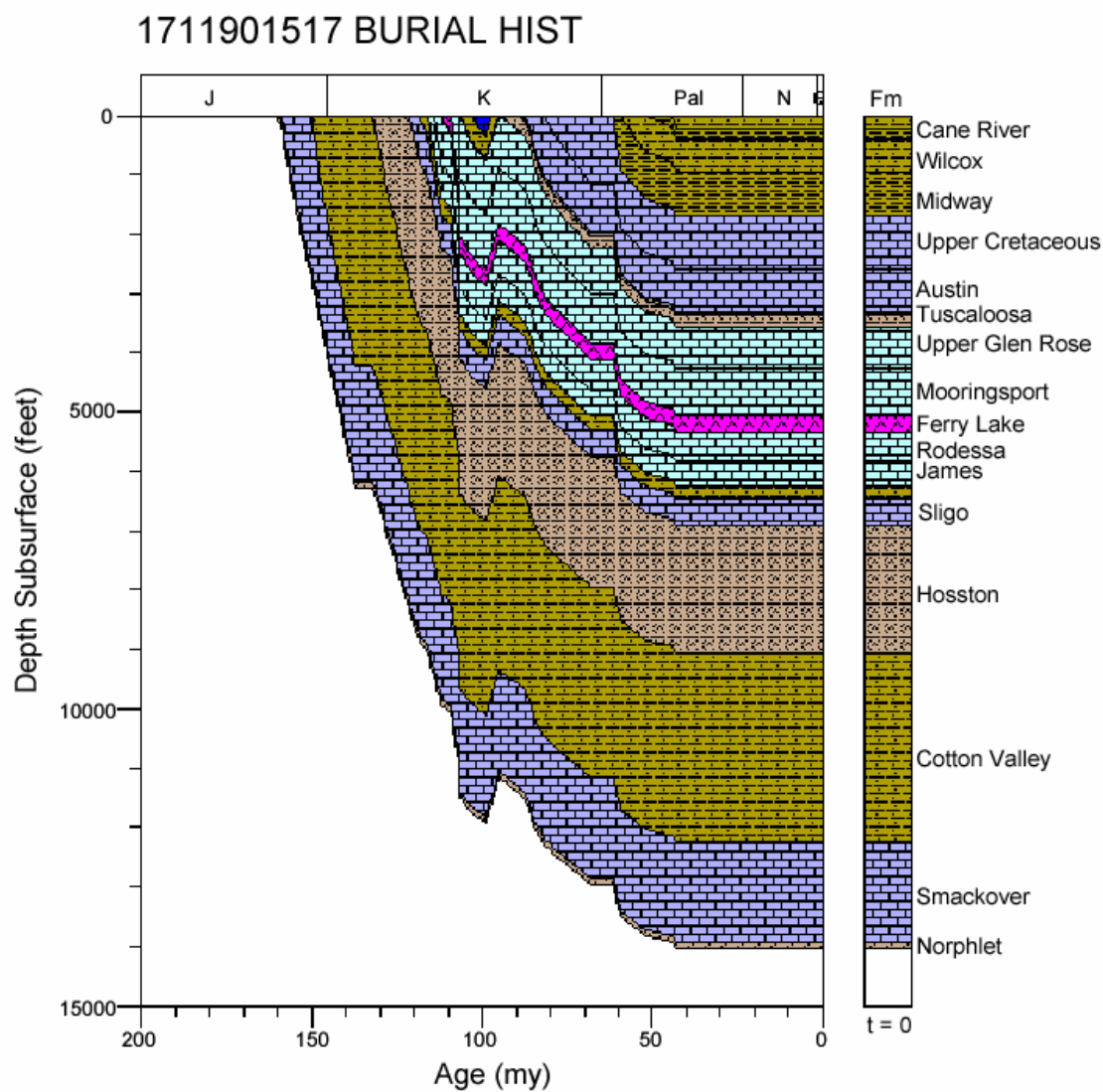
Figure 55. Burial history for well 1711901517, North Louisiana Salt Basin.
