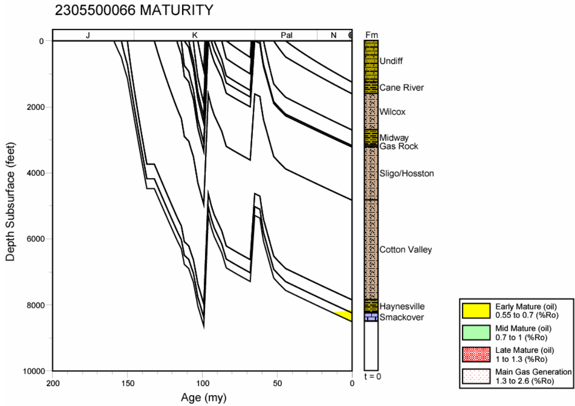
Figure 221. Thermal maturation profile for well 2305500066, Mississippi Interior Salt Basin.
