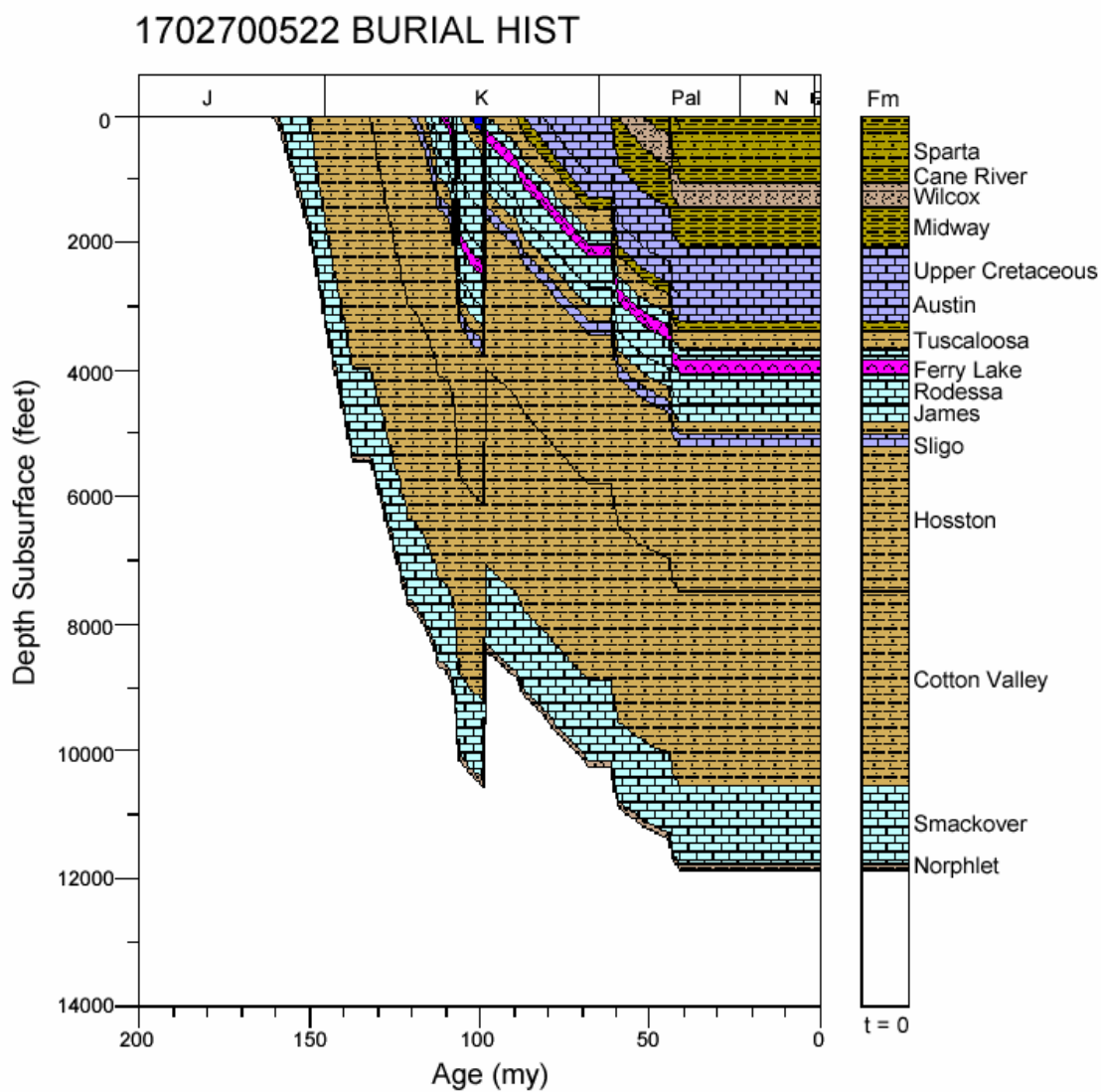
Figure 70. Burial history for well 1702700522, North Louisiana Salt Basin.
