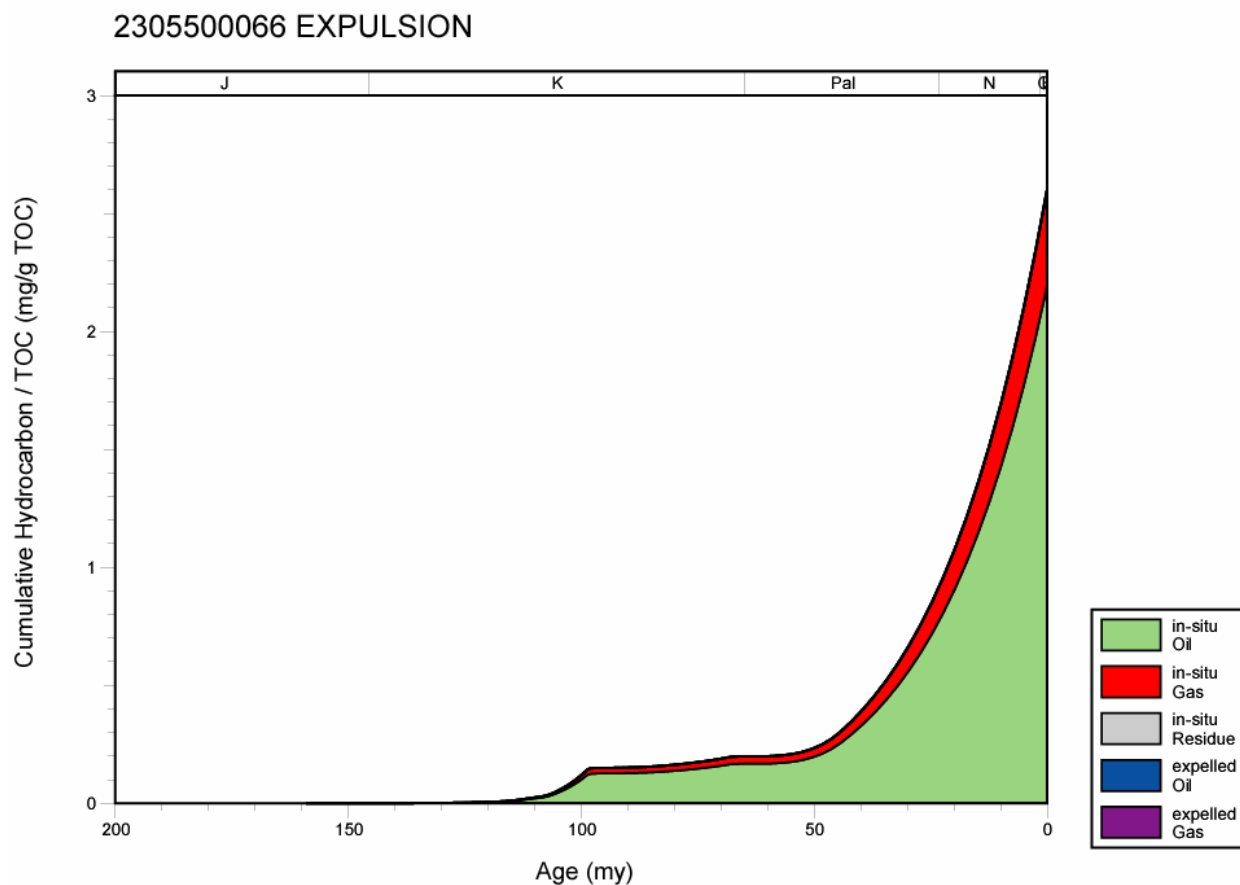
Figure 269. Hydrocarbon expulsion plot for well 2305500066, Mississippi Interior Salt Basin.
