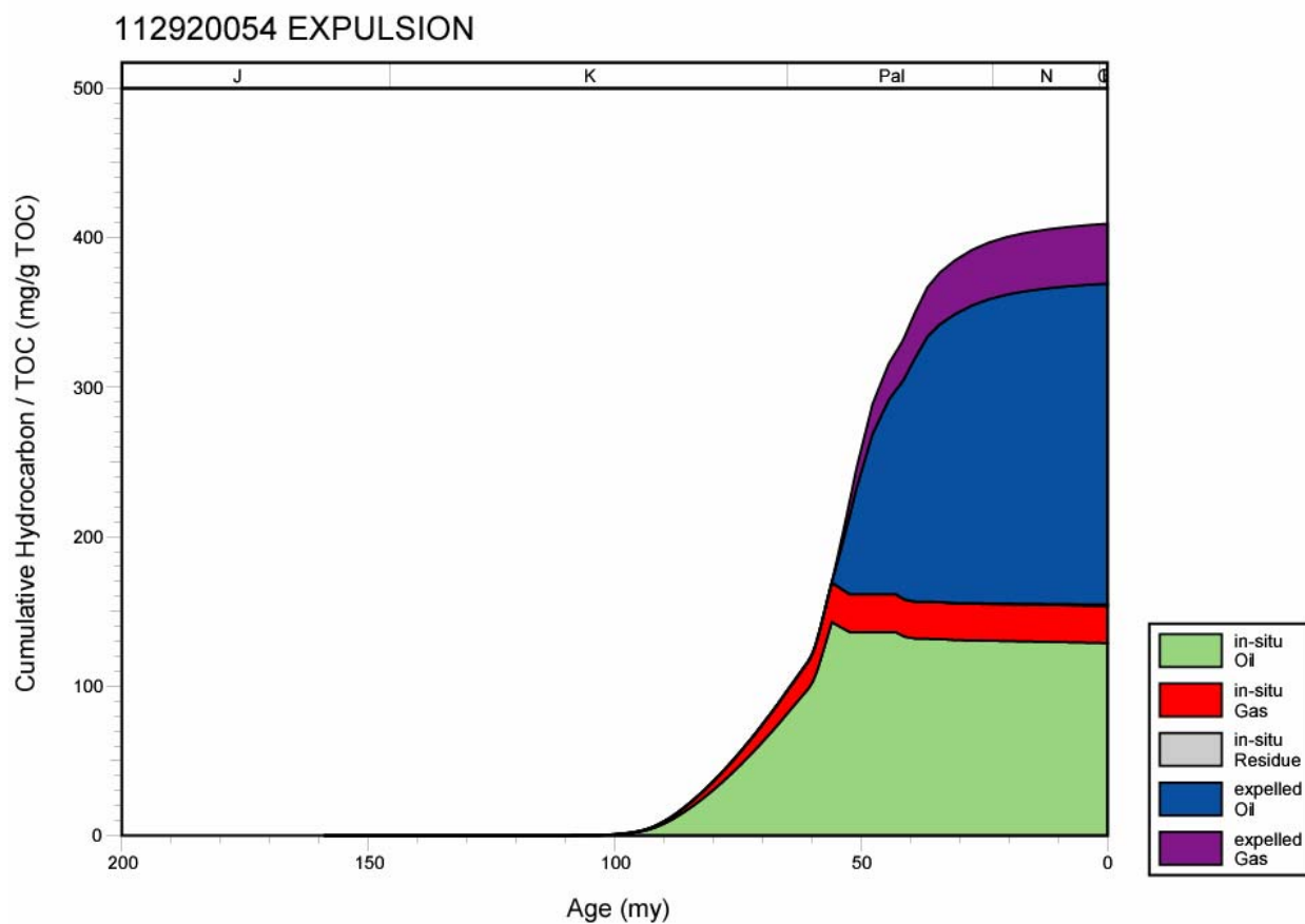
Figure 284. Hydrocarbon expulsion plot for well 112920054, Mississippi Interior Salt Basin.
