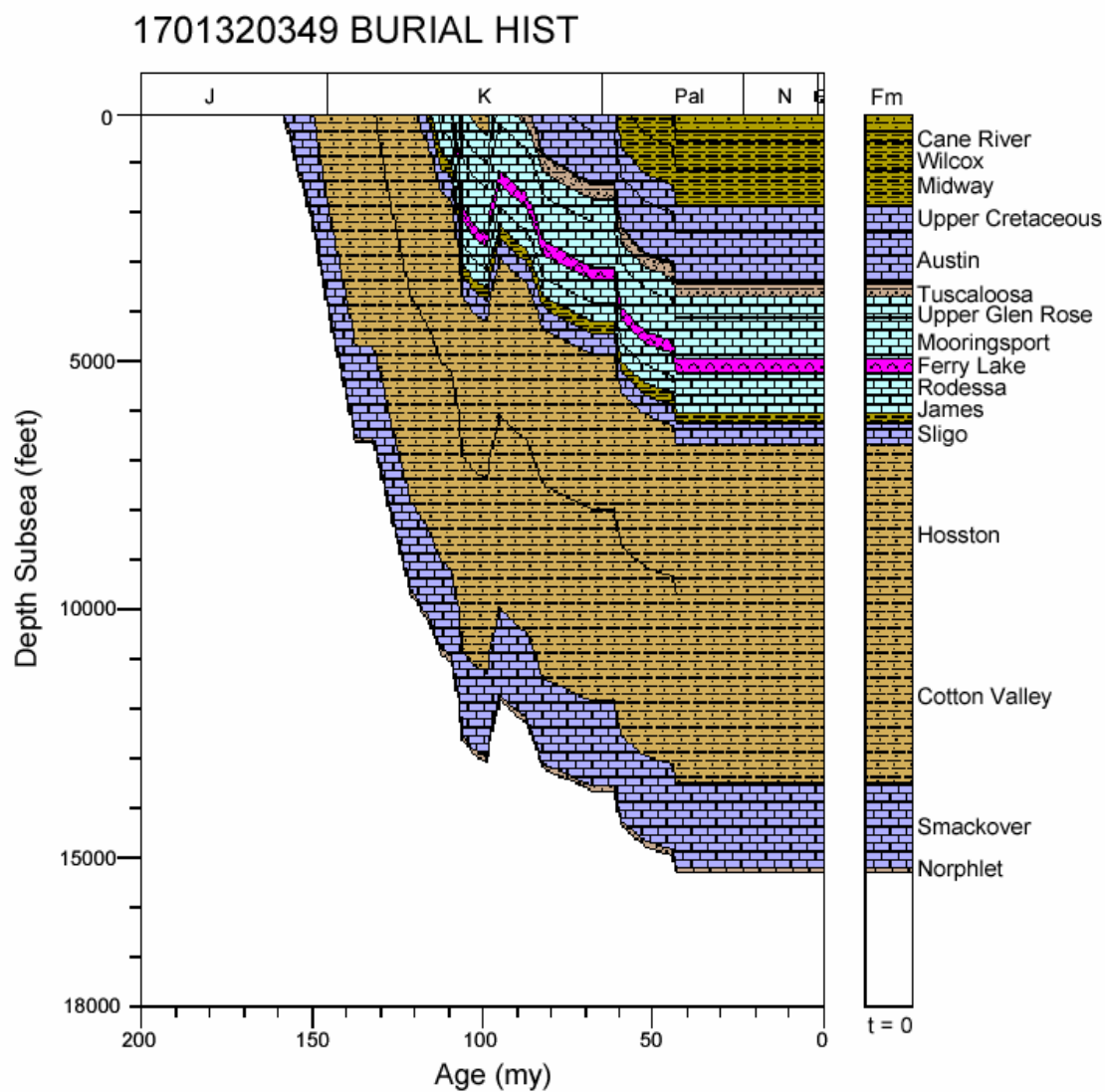
Figure 64. Burial history for well 1701320349, North Louisiana Salt Basin.
