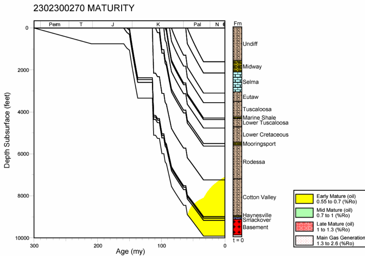
Figure 254. Thermal maturation profile for well 2302300270, Mississippi Interior Salt Basin.
