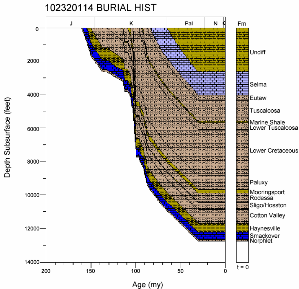
Figure 214. Burial history for well 102320114, Mississippi Interior Salt Basin.
