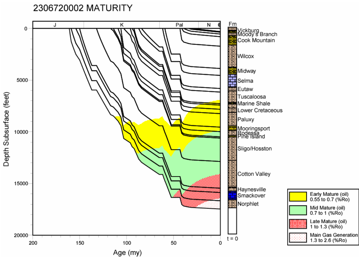
Figure 232. Thermal maturation profile for well 2306720002, Mississippi Interior Salt Basin.
