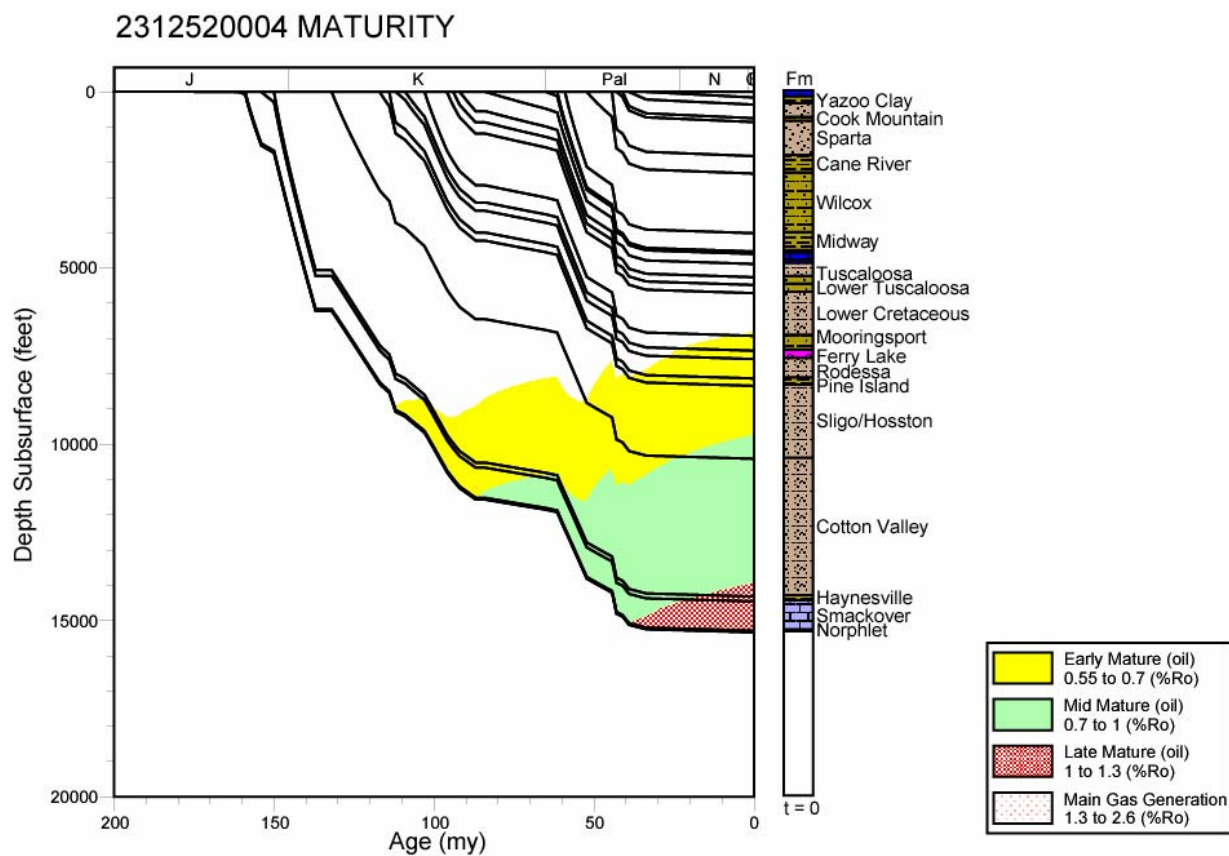
Figure 222. Thermal maturation profile for well 2312520004, Mississippi Interior Salt Basin.
