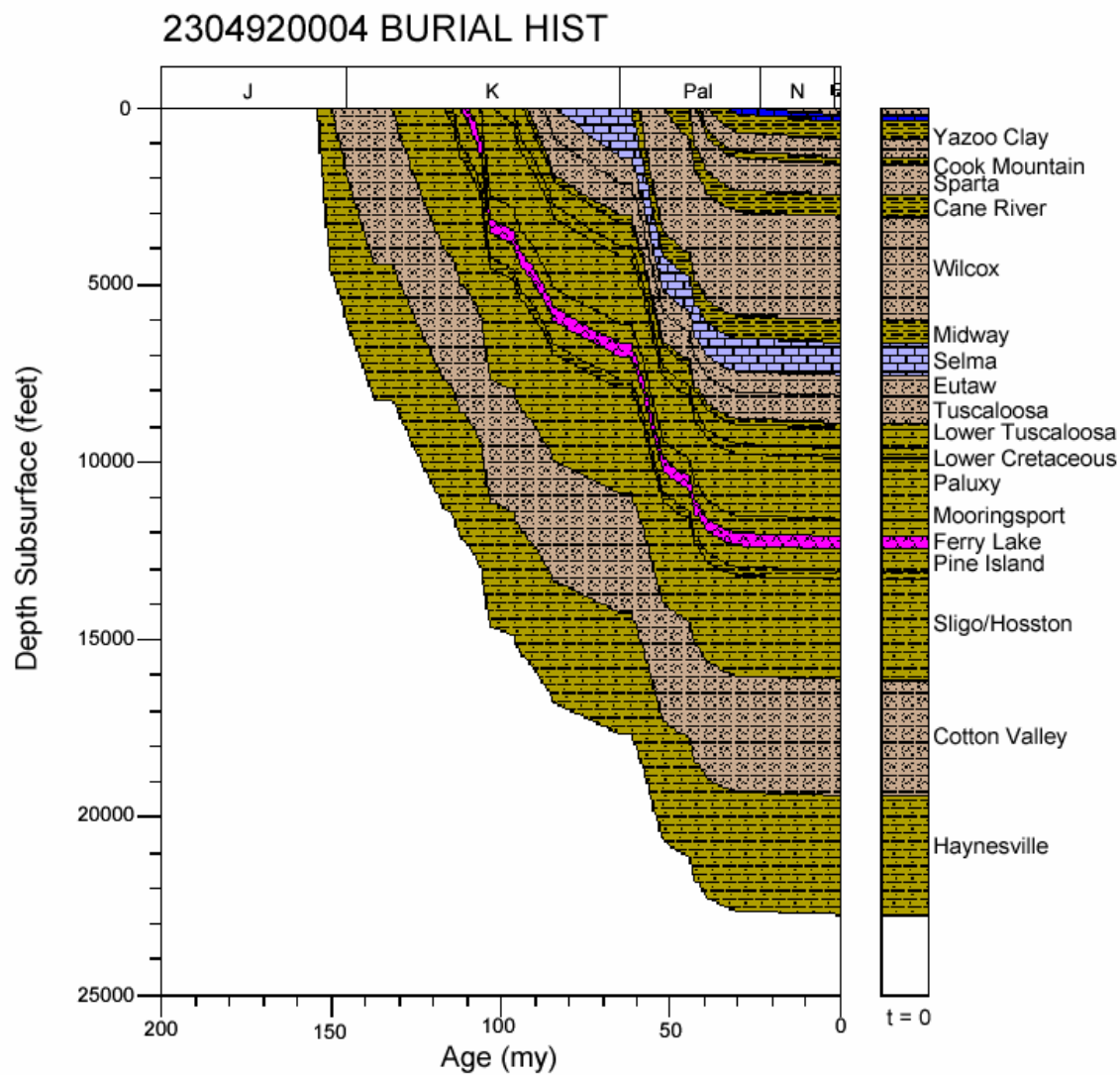
Figure 197. Burial history for well 2304920004, Mississippi Interior Salt Basin.
