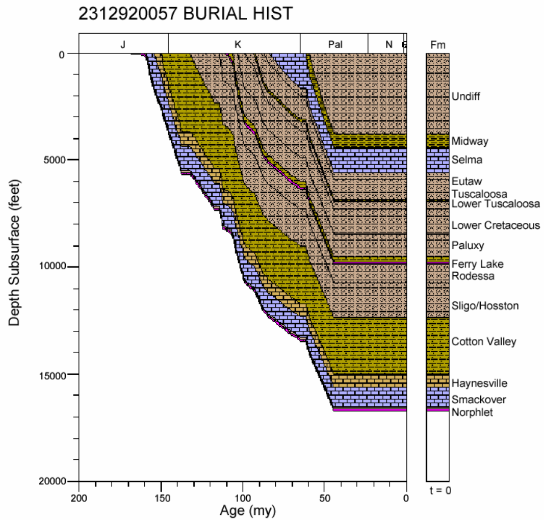
Figure 202. Burial history for well 2312920057, Mississippi Interior Salt Basin.
