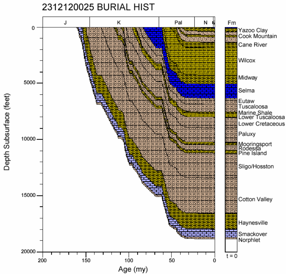
Figure 177. Burial history for well 2312120025, Mississippi Interior Salt Basin.
