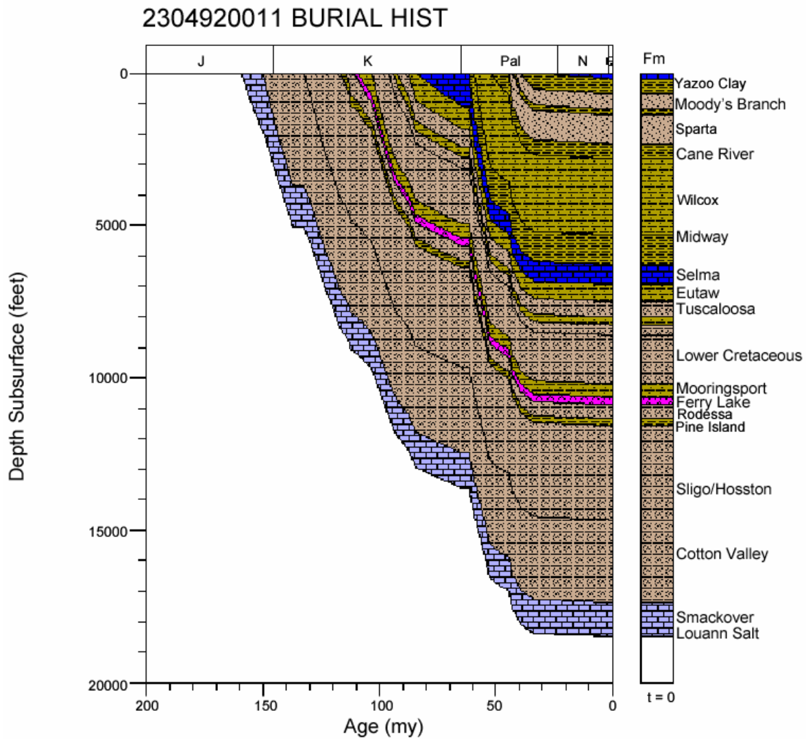
Figure 175. Burial history for well 2304920011, Mississippi Interior Salt Basin.
