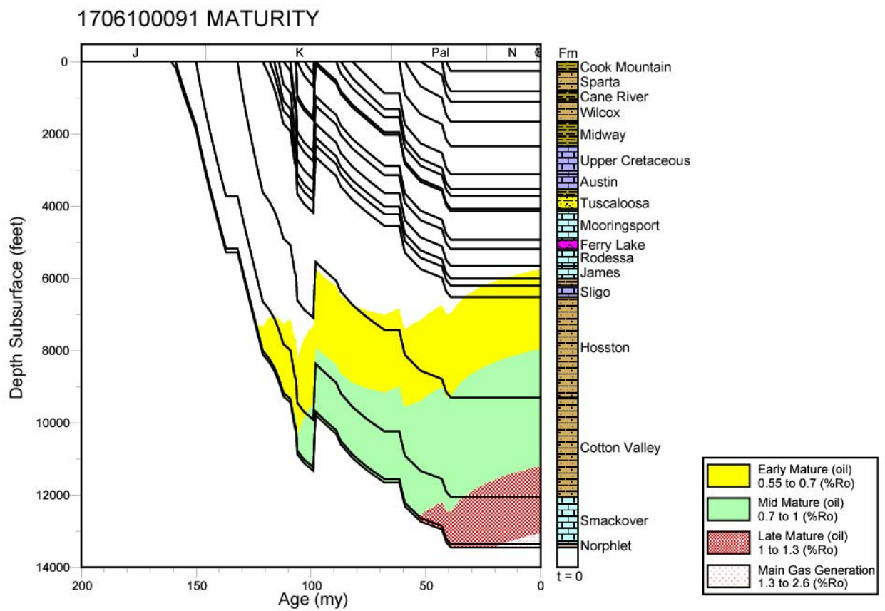
Figure 118. Thermal maturation profile for well 1706100091, North Louisiana Salt Basin.
