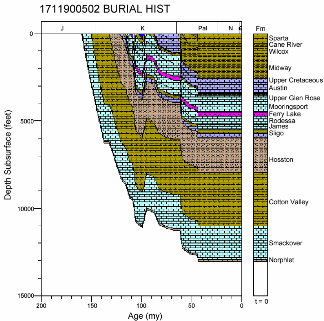
Figure 53. Burial history for well 1711900502, North Louisiana Salt Basin.
