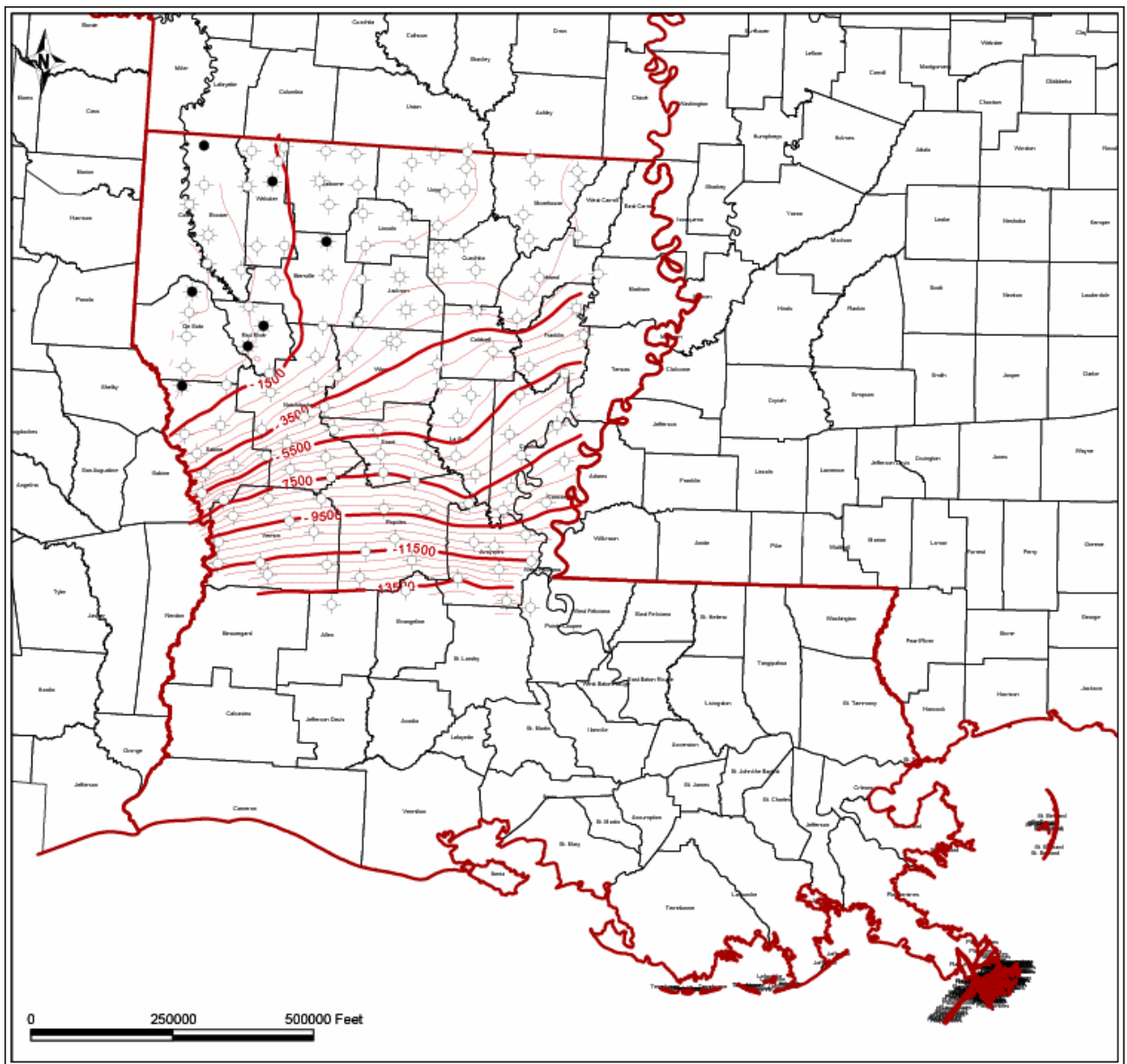
Figure 16. Structure map on the top of the Upper Cretaceous.
