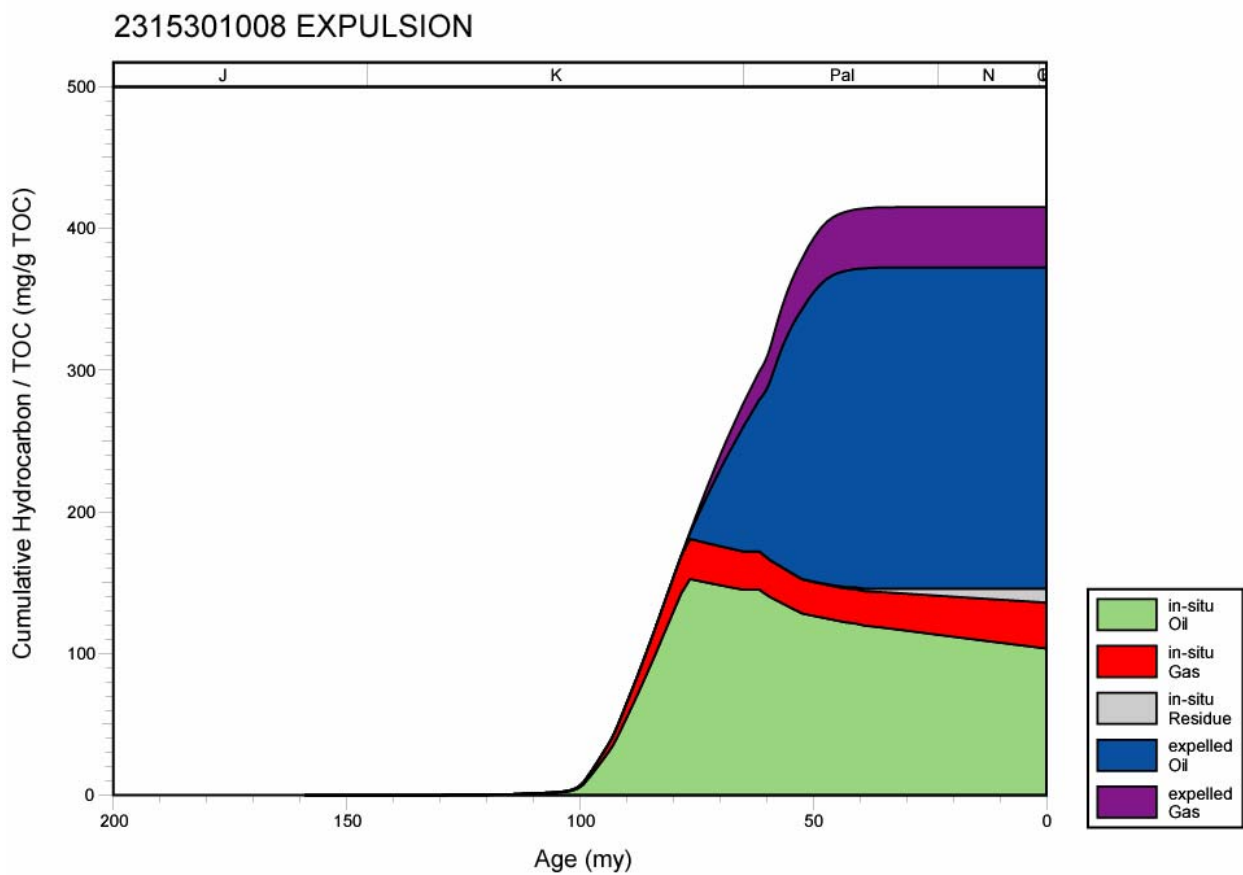
Figure 281. Hydrocarbon expulsion plot for well 2315301008, Mississippi Interior Salt Basin.
