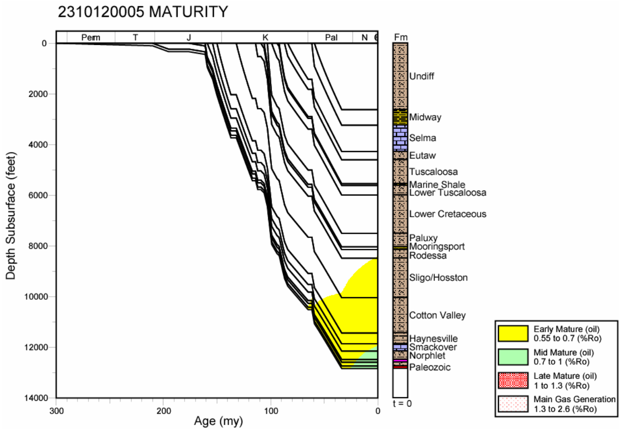
Figure 248. Thermal maturation profile for well 2310120005, Mississippi Interior Salt Basin.
