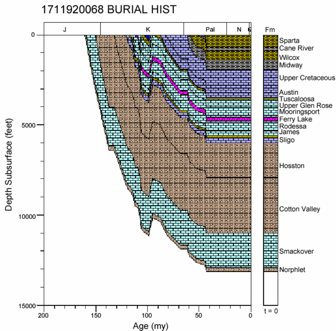
Figure 52. Burial history for well 1711920068, North Louisiana Salt Basin.
