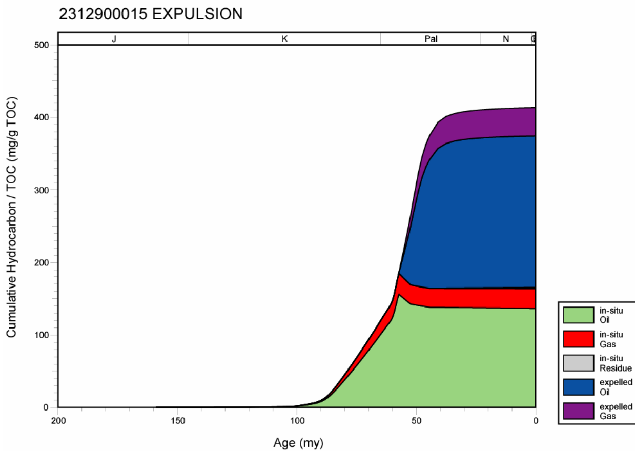
Figure 295. Hydrocarbon expulsion plot for well 2312900015, Mississippi Interior Salt Basin.
