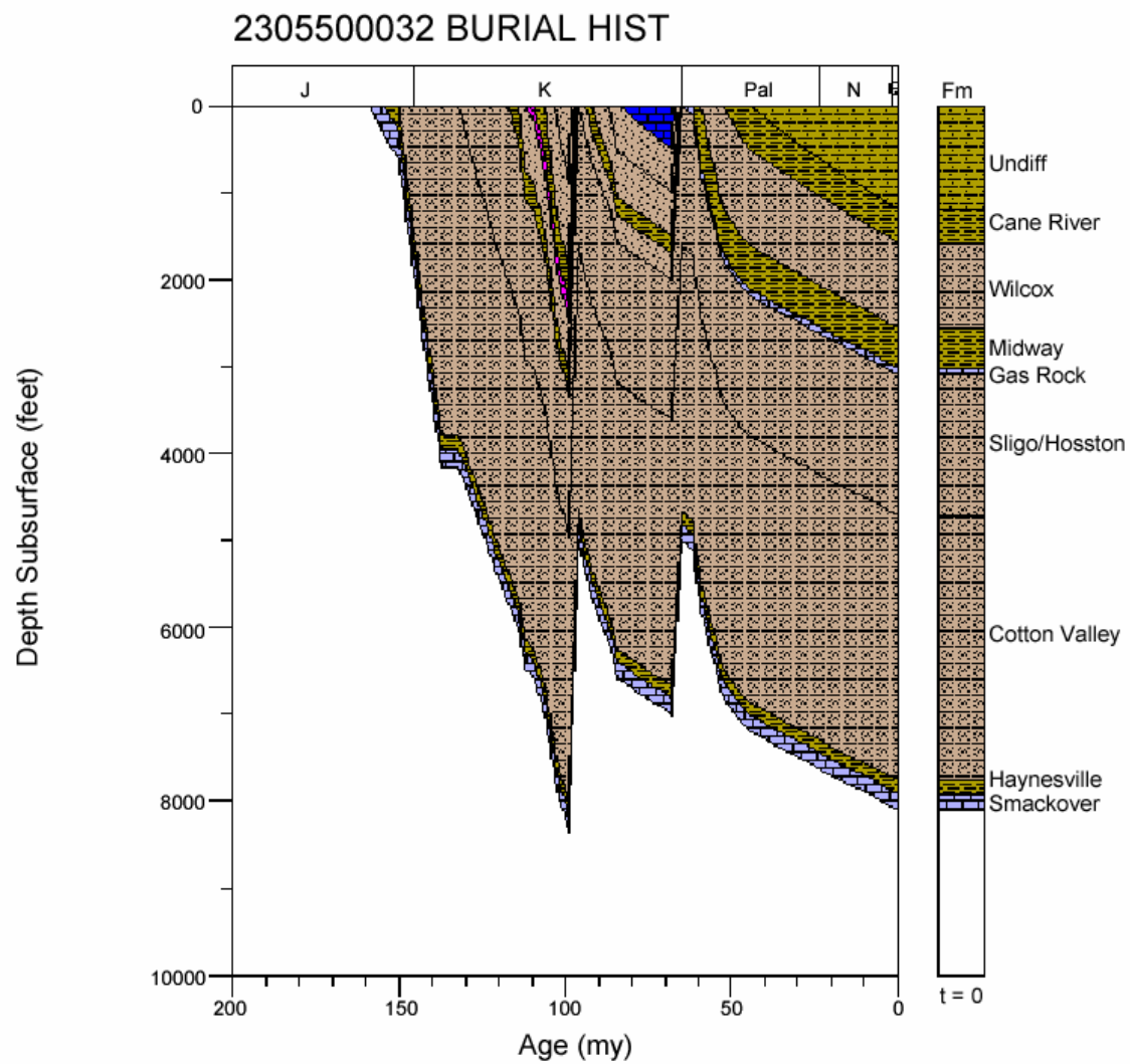
Figure 172. Burial history for well 2305500032, Mississippi Interior Salt Basin.
