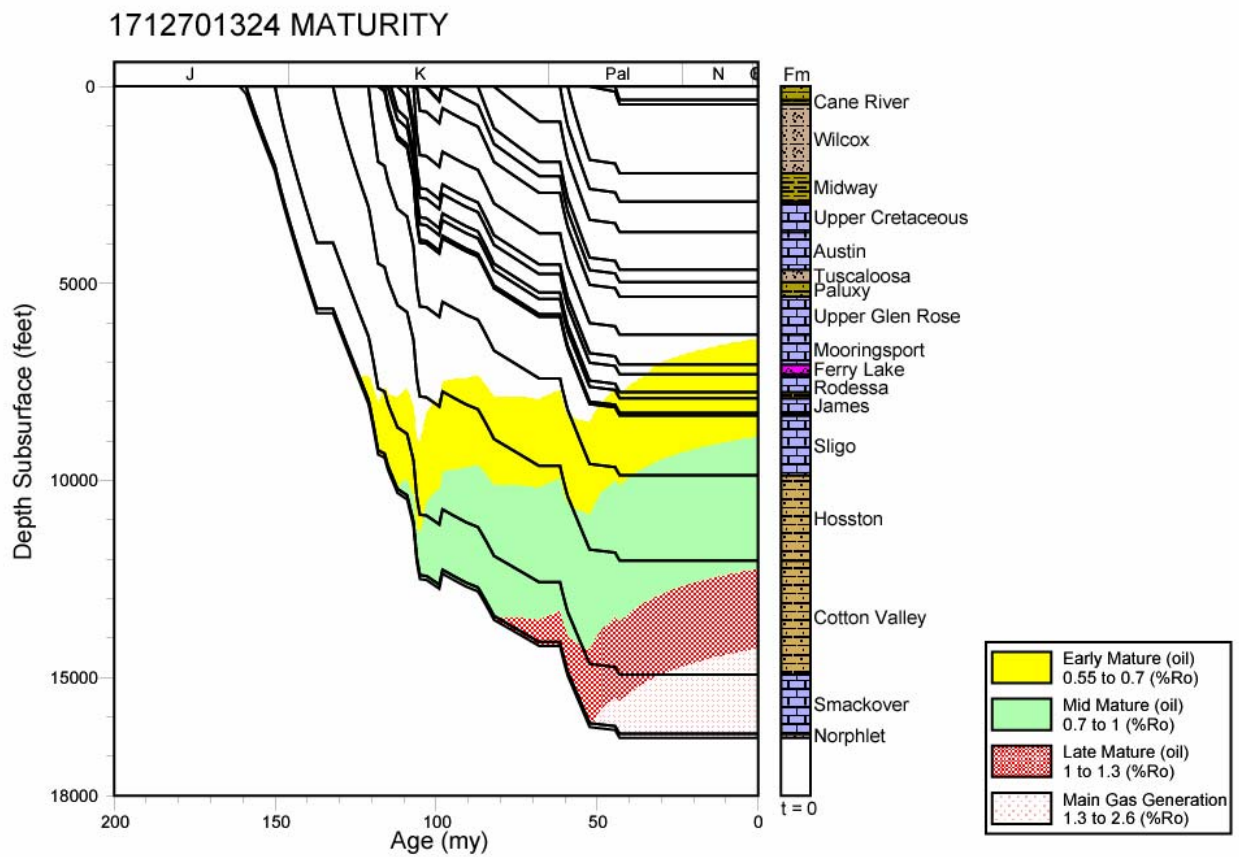
Figure 122. Thermal maturation profile for well 1712701324, North Louisiana Salt Basin.
