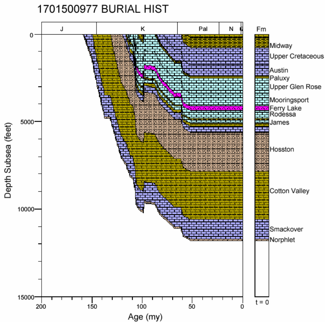
Figure 44. Burial history for well 1701500977, North Louisiana Salt Basin.
