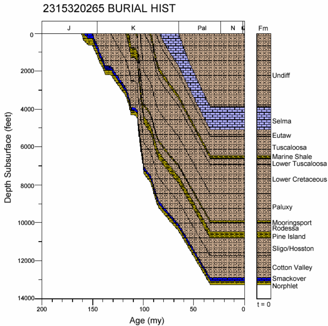
Figure 209. Burial history for well 2315320265, Mississippi Interior Salt Basin.
