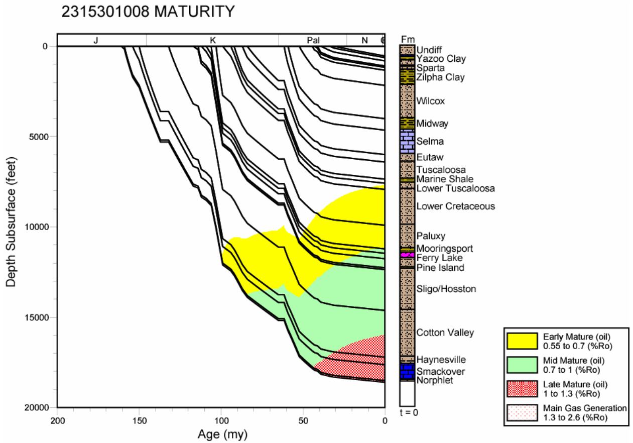
Figure 233. Thermal maturation profile for well 2315301008, Mississippi Interior Salt Basin.
