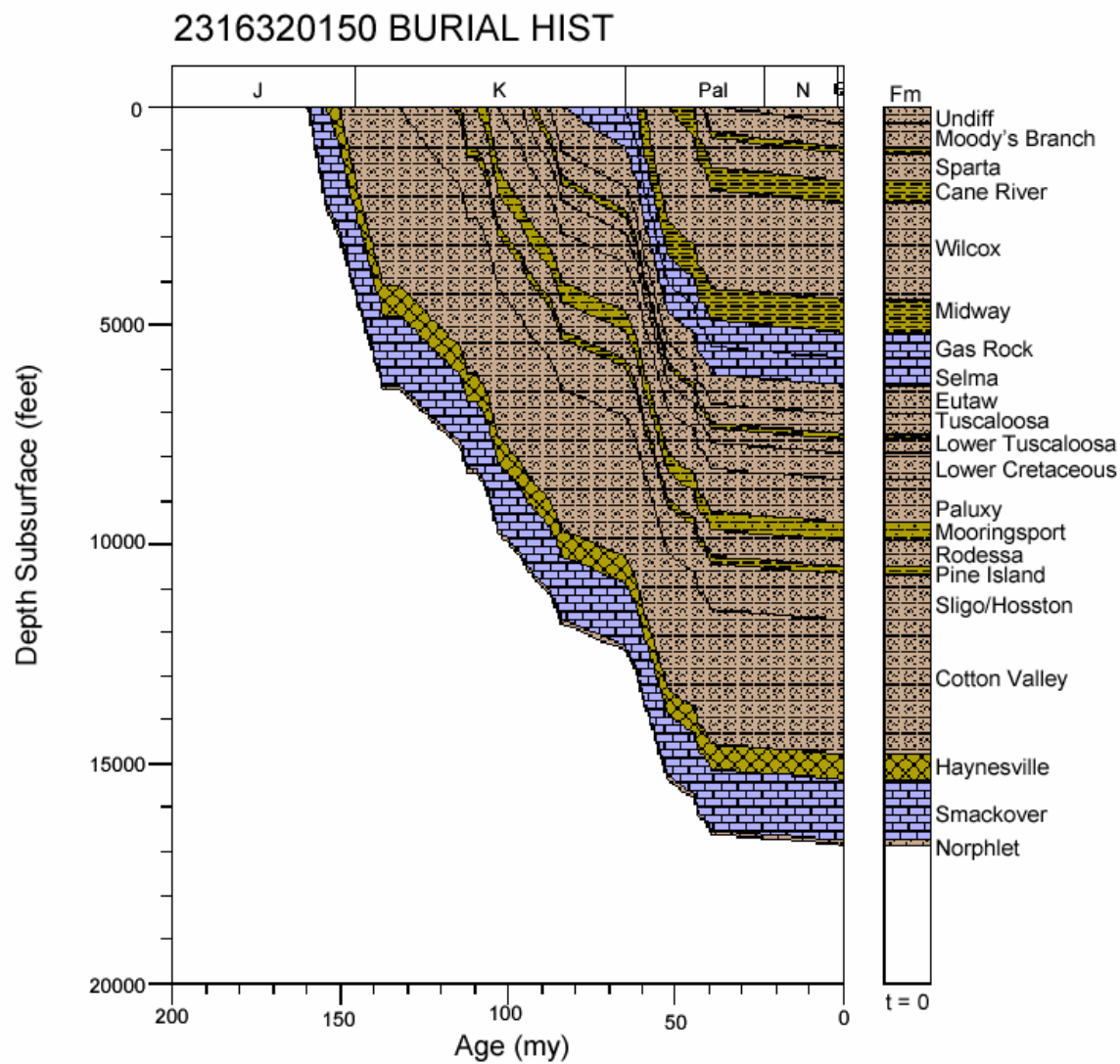
Figure 195. Burial history for well 2316320150, Mississippi Interior Salt Basin.
