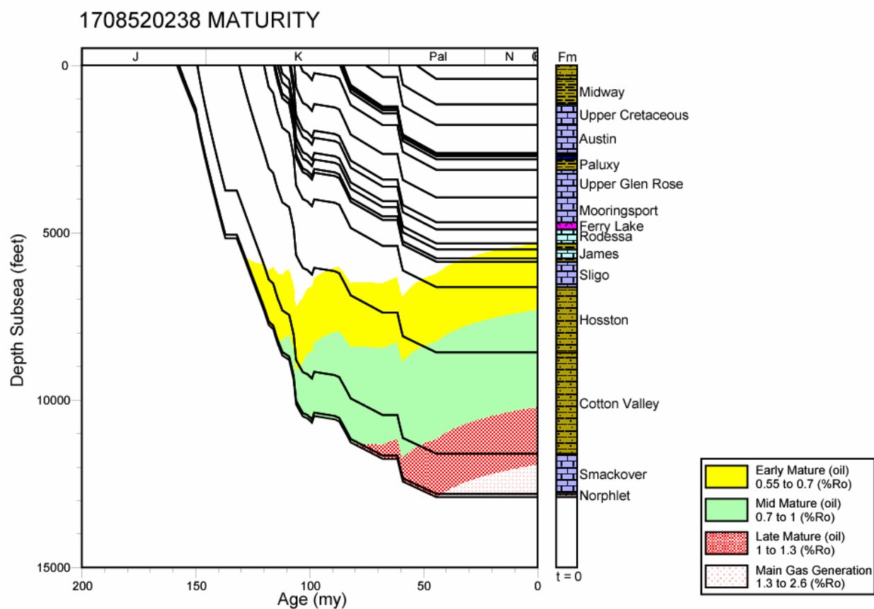
Figure 96. Thermal maturation profile for well 1708520238, North Louisiana Salt Basin.
