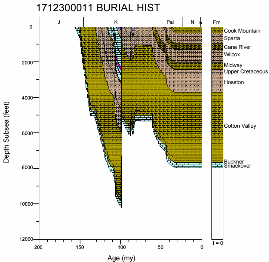
Figure 82. Burial history for well 1712300011, North Louisiana Salt Basin.
