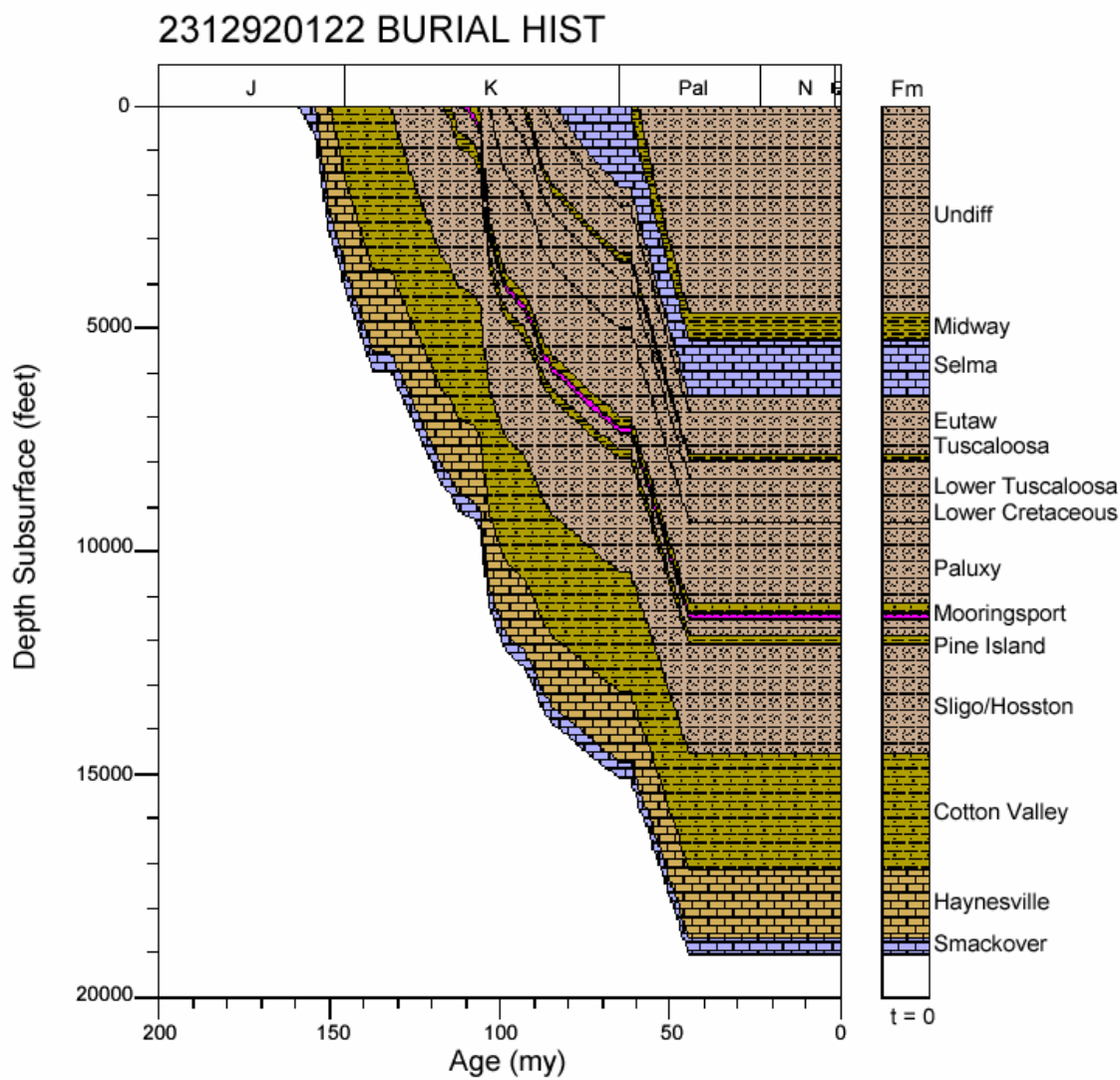
Figure 203. Burial history for well 2312920122, Mississippi Interior Salt Basin.
