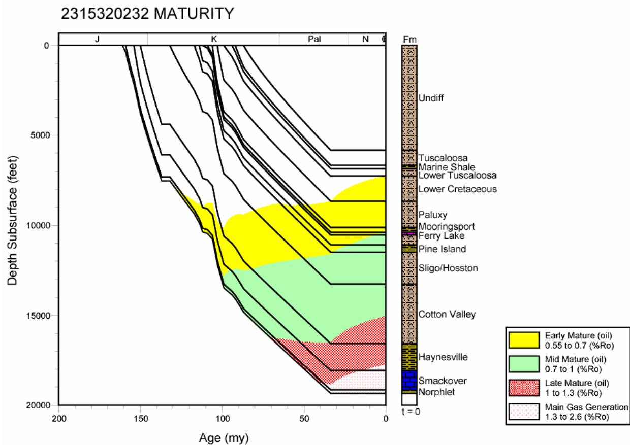
Figure 258. Thermal maturation profile for well 2315320232, Mississippi Interior Salt Basin.
