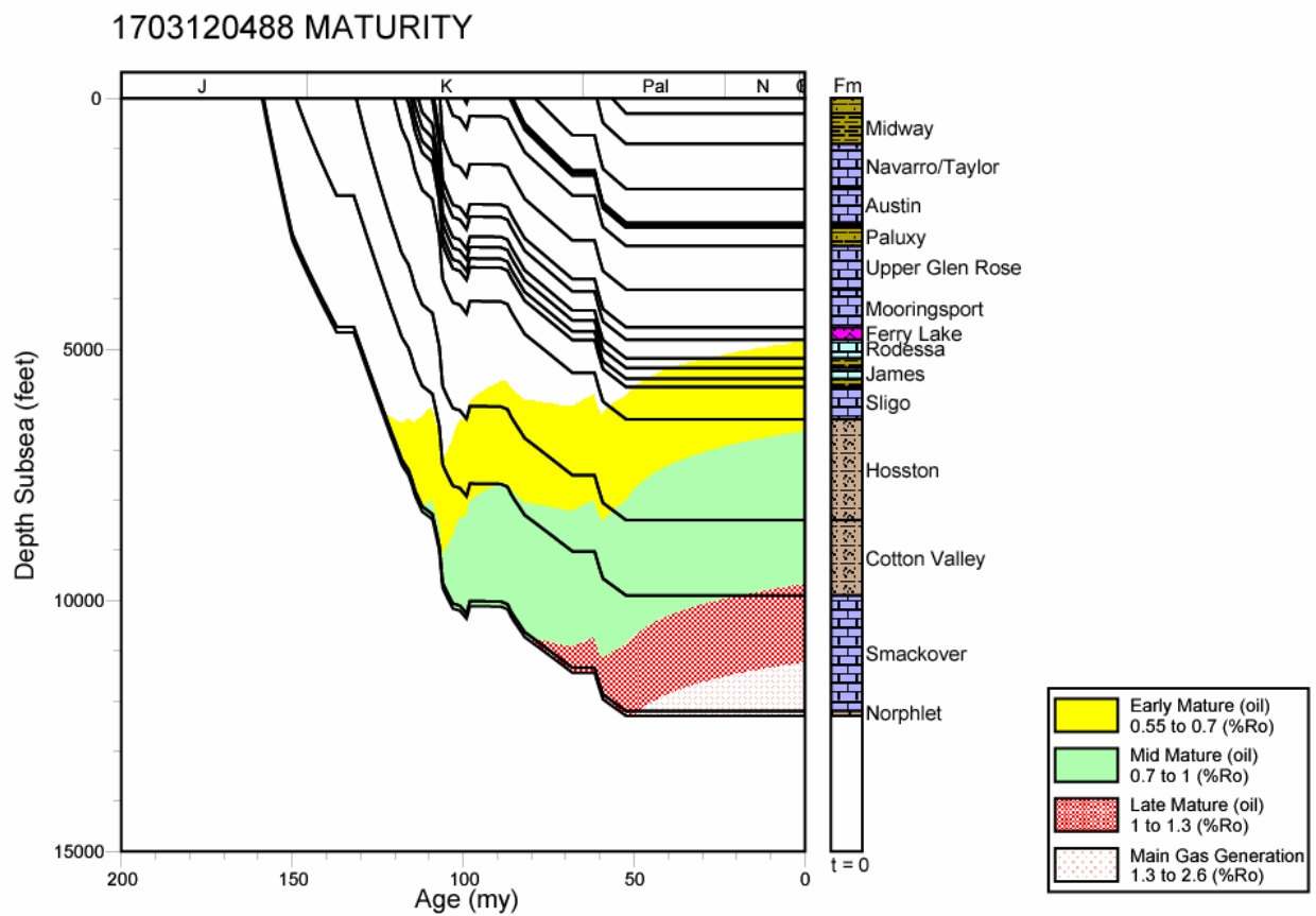
Figure 92. Thermal maturation profile for well 1703120488, North Louisiana Salt Basin.
