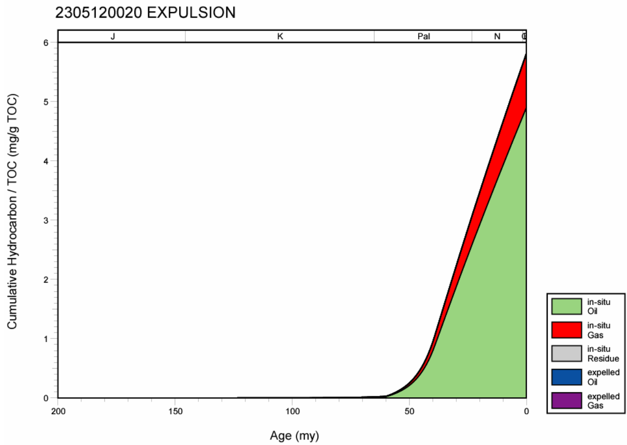
Figure 288. Hydrocarbon expulsion plot for well 2305120020, Mississippi Interior Salt Basin.
