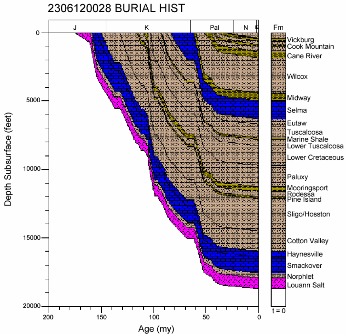
Figure 182. Burial history for well 2306120028, Mississippi Interior Salt Basin.
