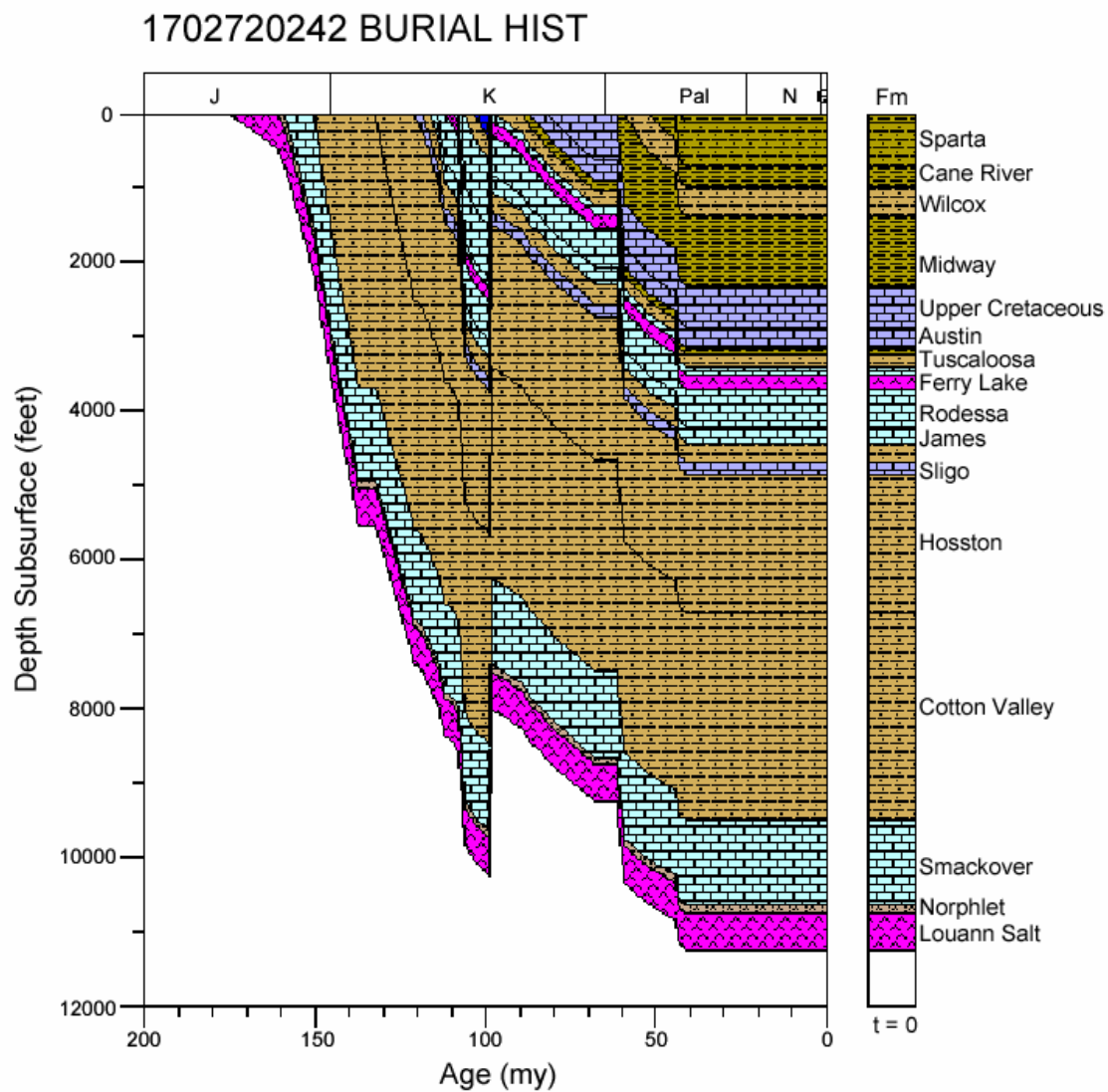
Figure 69. Burial history for well 1702720242, North Louisiana Salt Basin.
