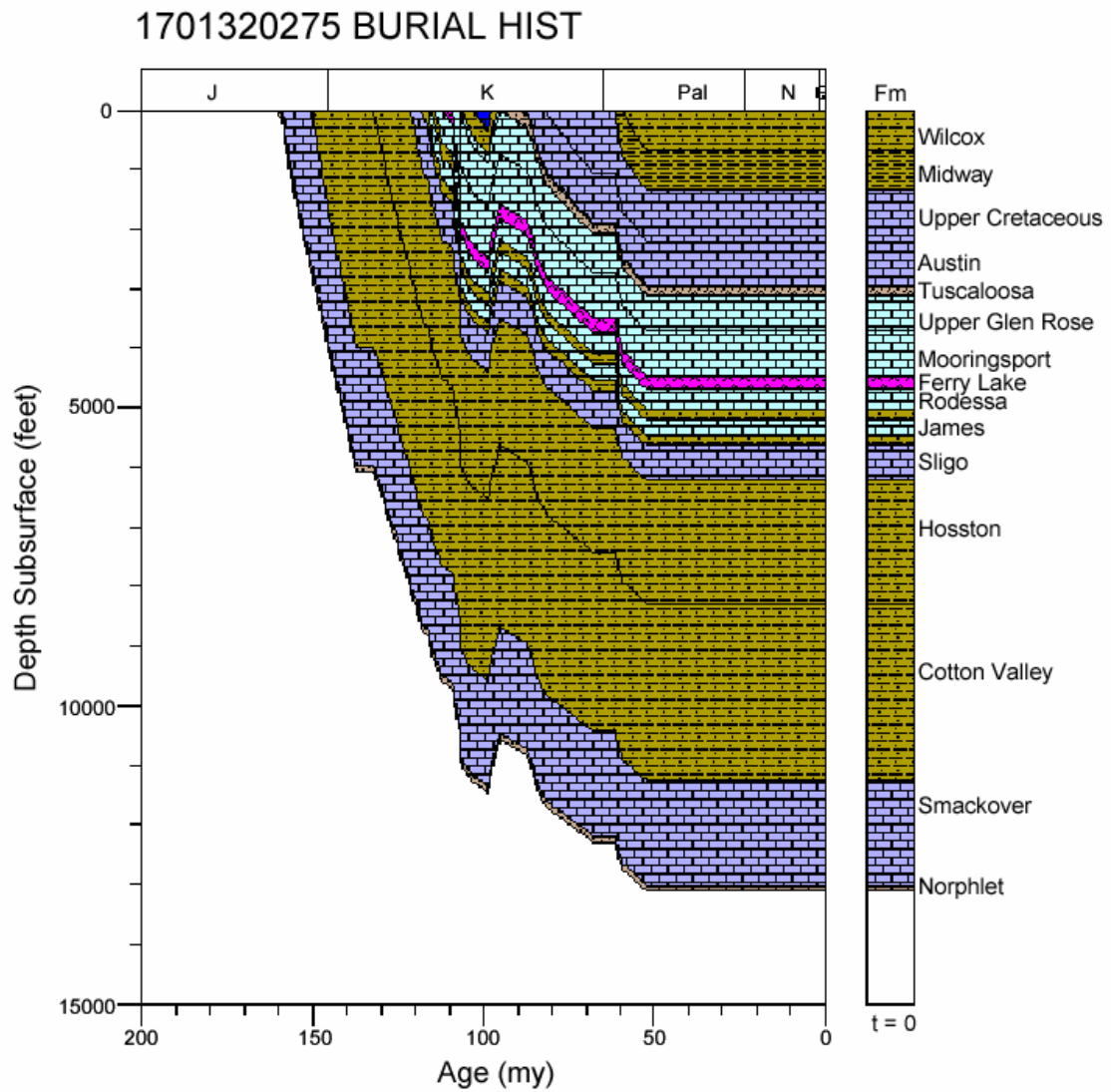
Figure 56. Burial history for well 1701320275, North Louisiana Salt Basin.
