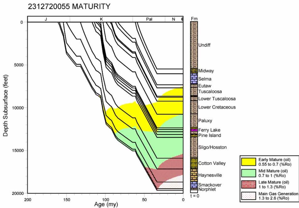
Figure 252. Thermal maturation profile for well 2312720055, Mississippi Interior Salt Basin.
