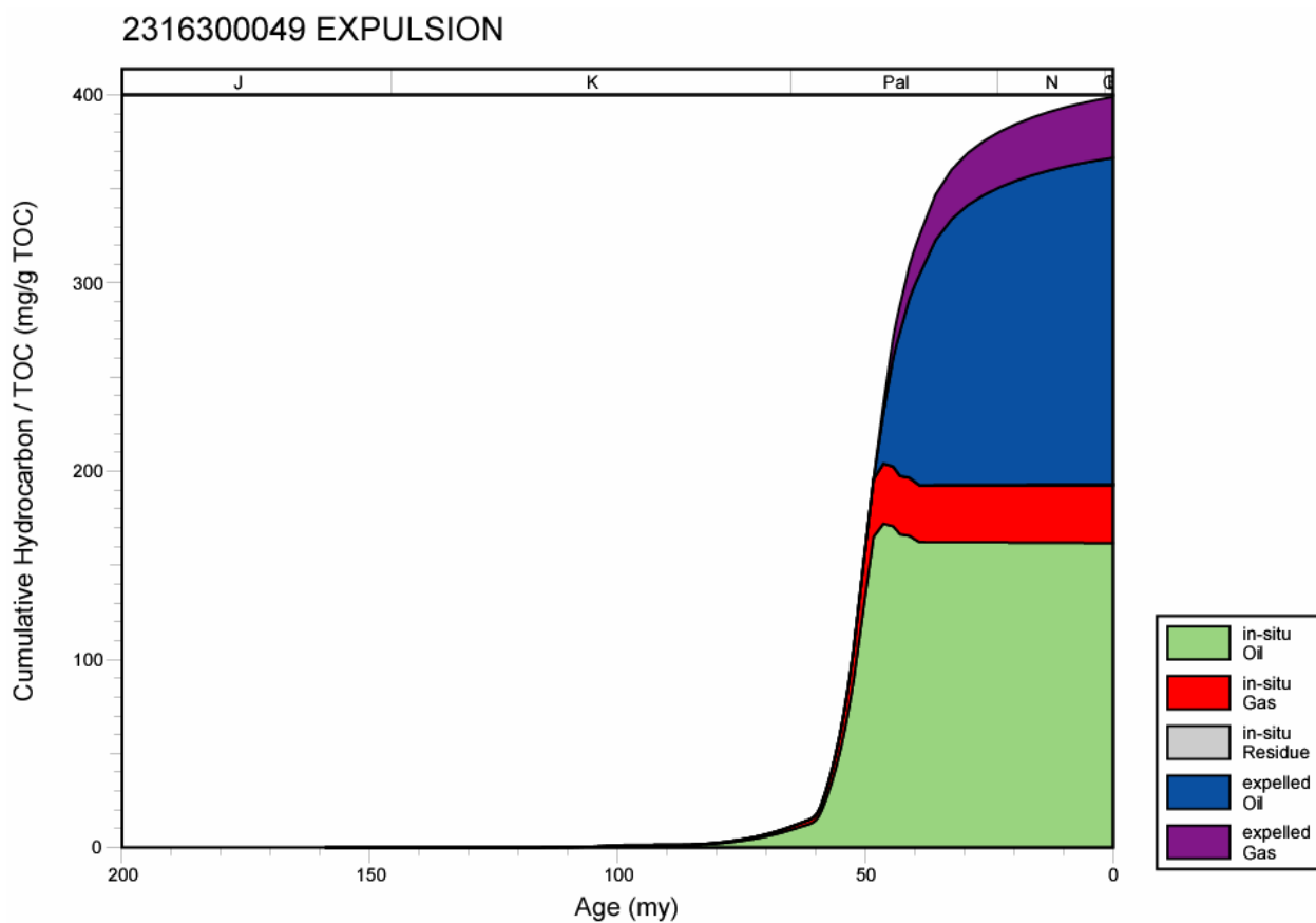
Figure 290. Hydrocarbon expulsion plot for well 2316300049, Mississippi Interior Salt Basin.
