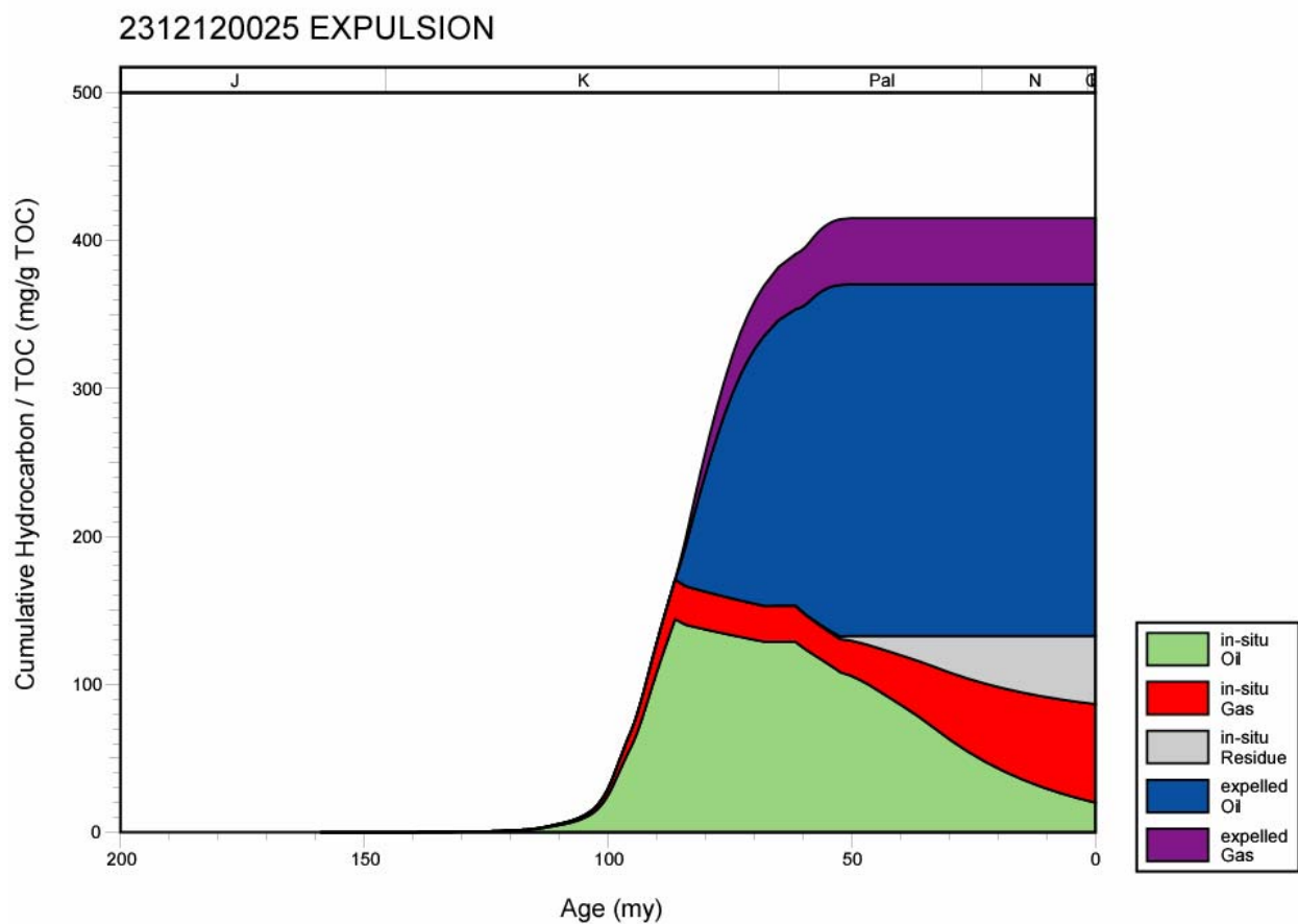
Figure 273. Hydrocarbon expulsion plot for well 2312120025, Mississippi Interior Salt Basin.
