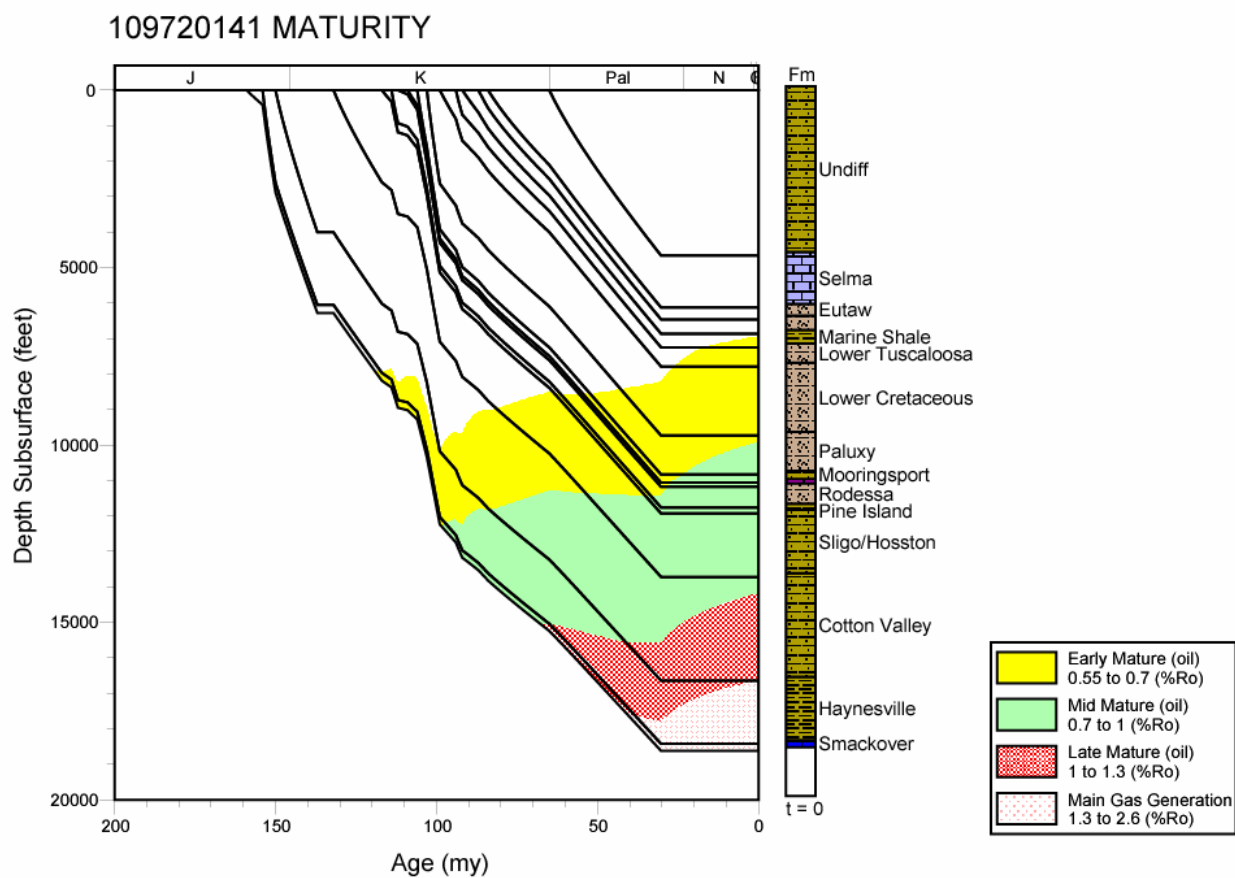
Figure 266. Thermal maturation profile for well 109720141, Mississippi Interior Salt Basin.
