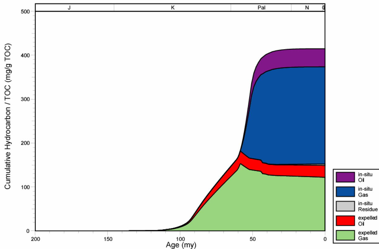
Figure 270. Hydrocarbon expulsion plot for well 2312520004, Mississippi Interior Salt Basin.
