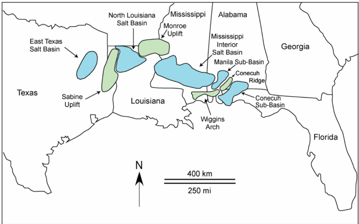
Figure 1. Location map of interior salt basins and subbasins in the north central and northeastern Gulf of Mexico area.
