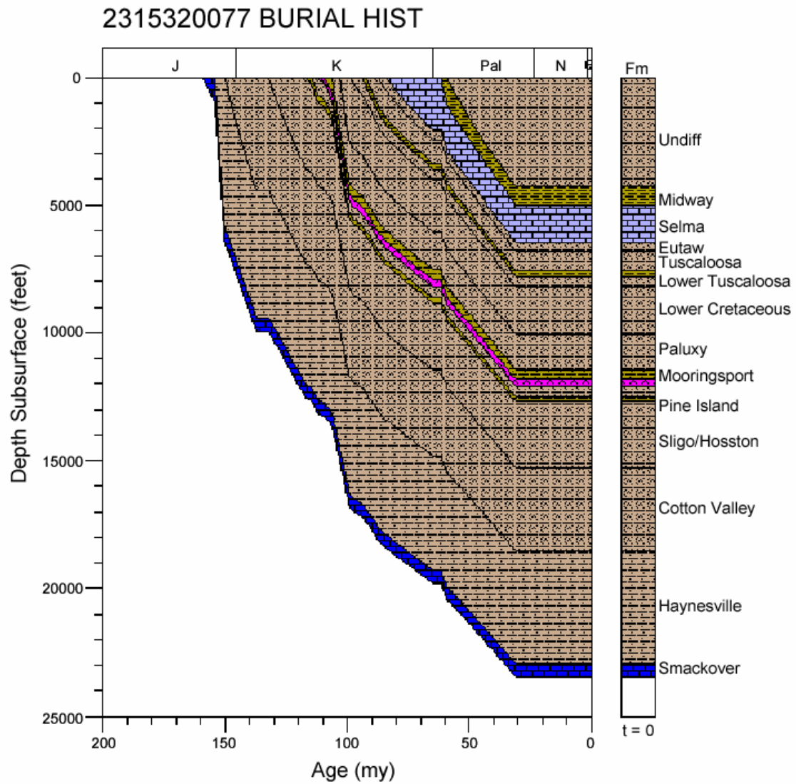
Figure 211. Burial history for well 2315320077, Mississippi Interior Salt Basin.
