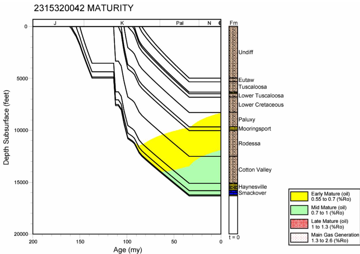
Figure 256. Thermal maturation profile for well 2315320042, Mississippi Interior Salt Basin.
