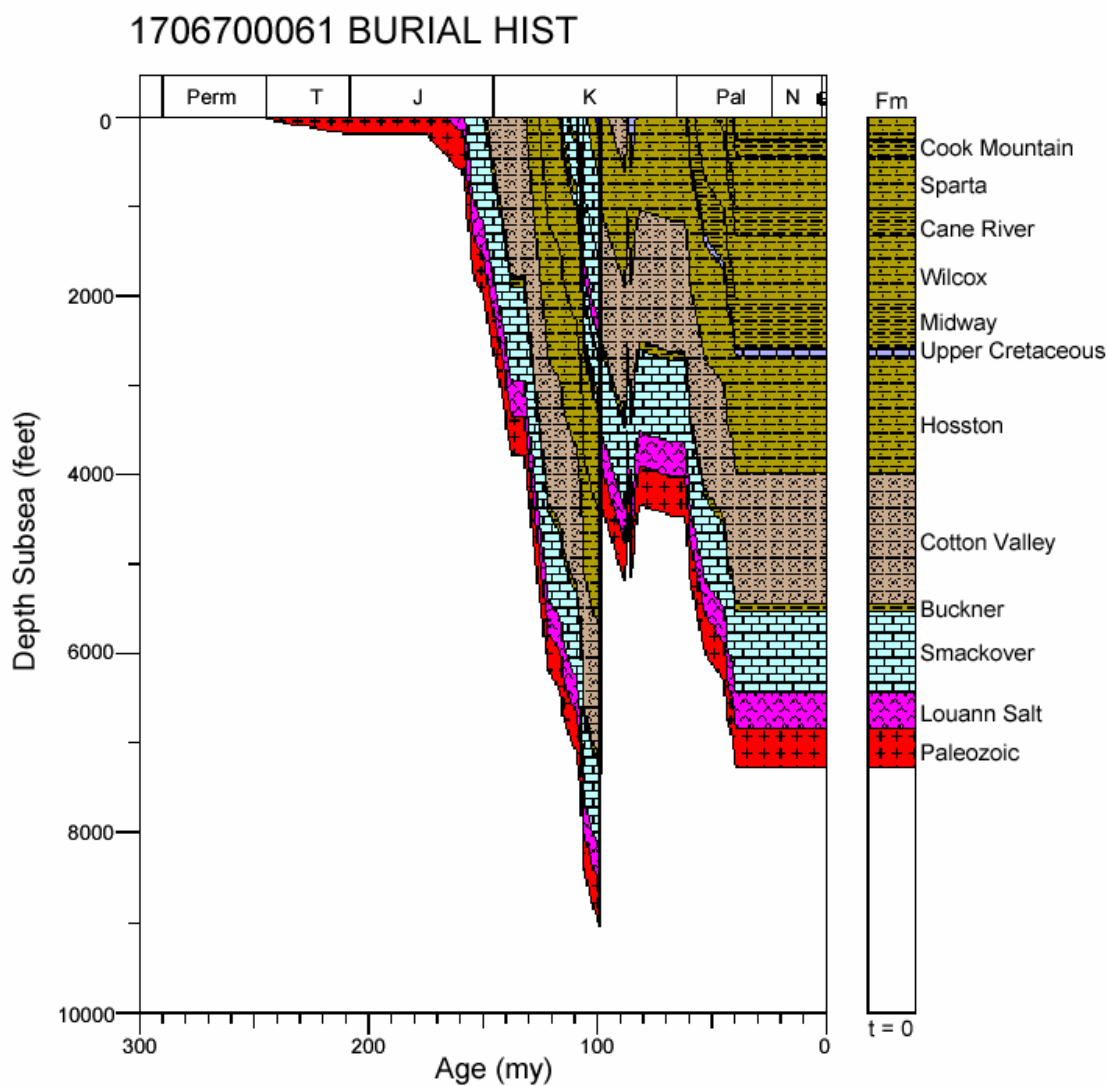
Figure 81. Burial history for well 1706700061, North Louisiana Salt Basin.
