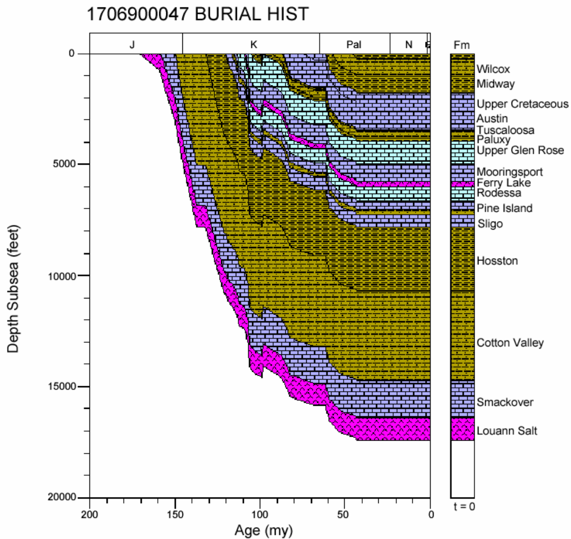
Figure 67. Burial history for well 1706900047, North Louisiana Salt Basin.
