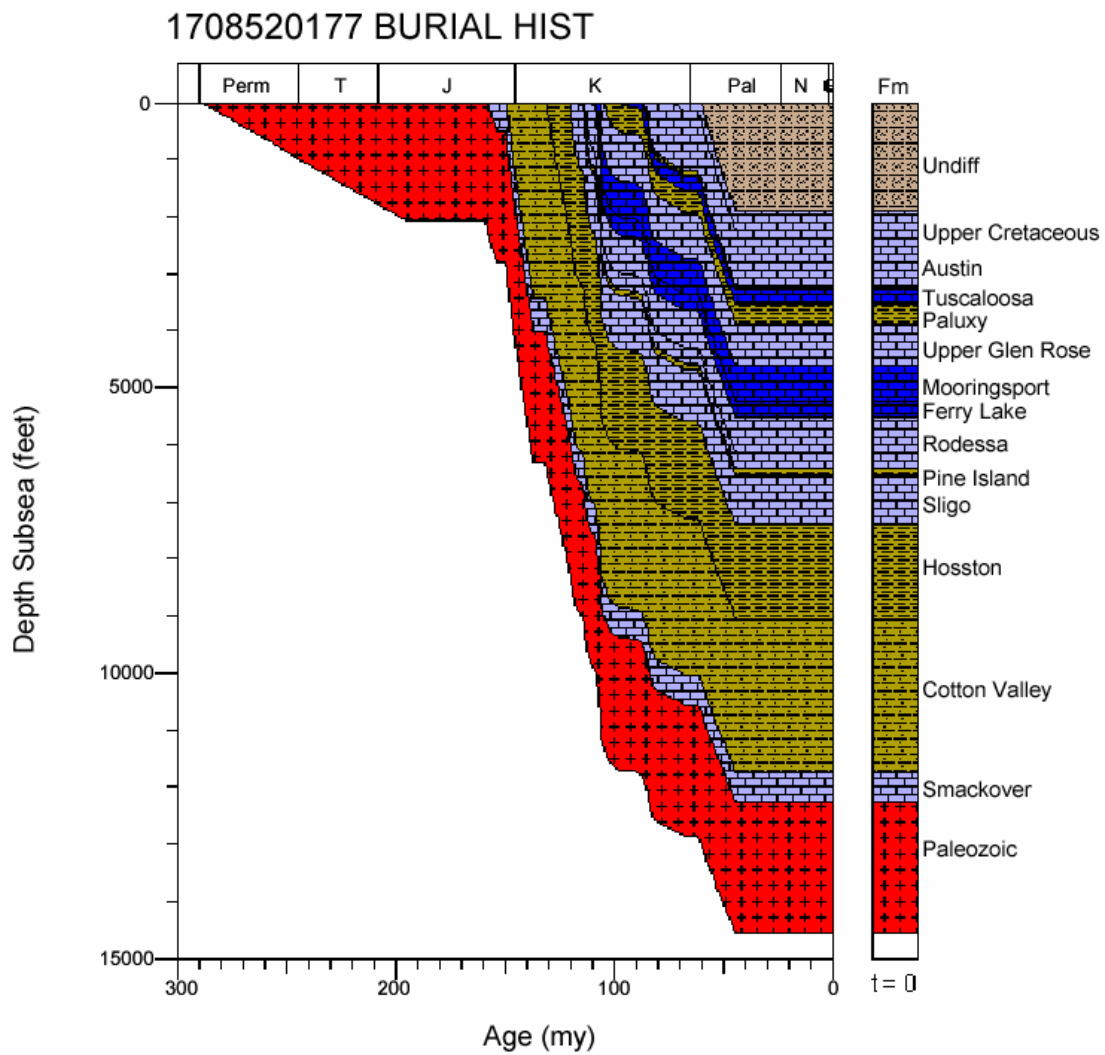
Figure 51. Burial history for well 1708520177, North Louisiana Salt Basin.
