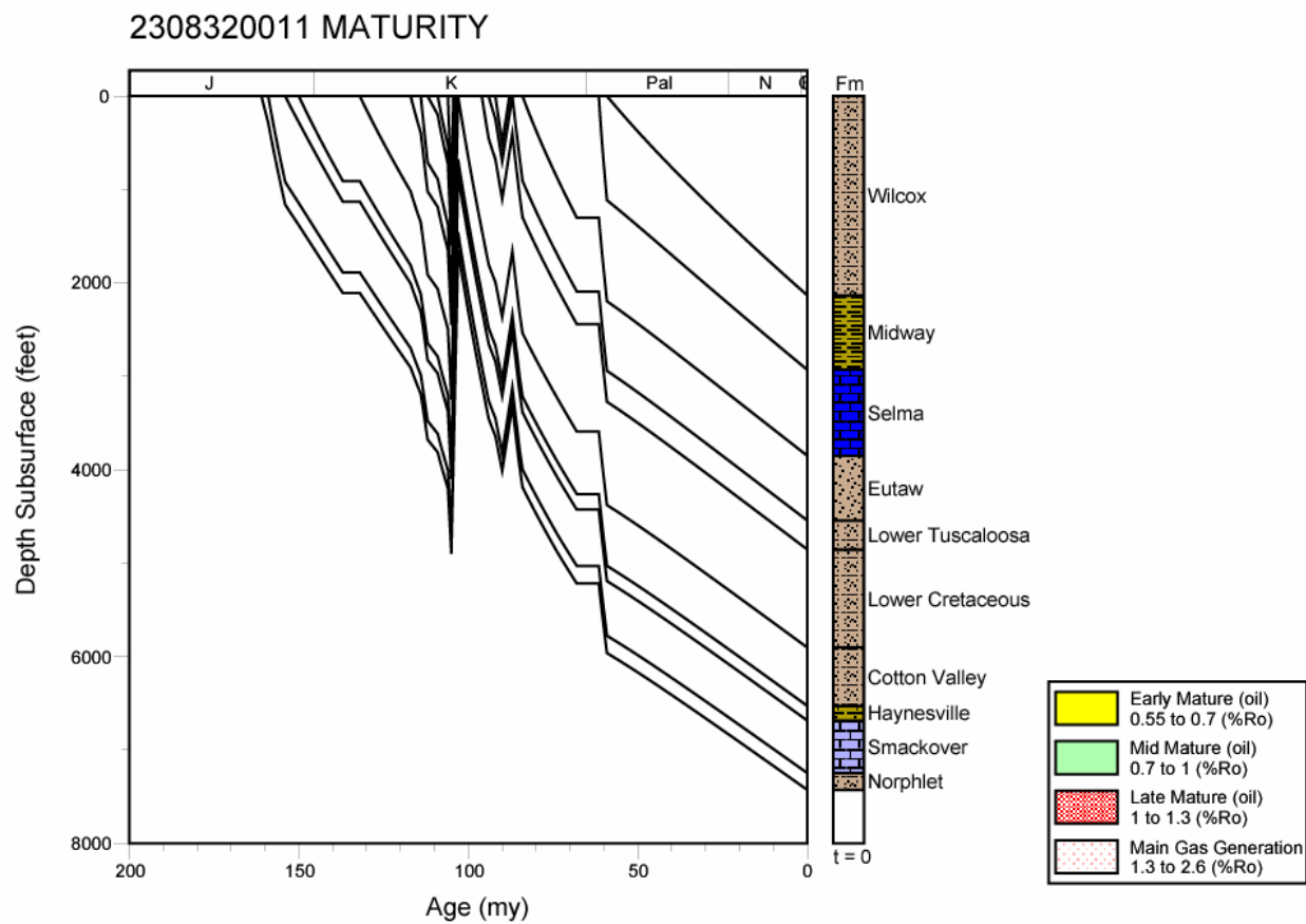
Figure 239. Thermal maturation profile for well 2308320011, Mississippi Interior Salt Basin.
