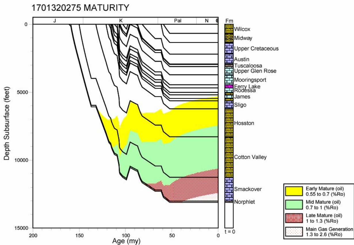
Figure 102. Thermal maturation profile for well 1701320275, North Louisiana Salt Basin.
