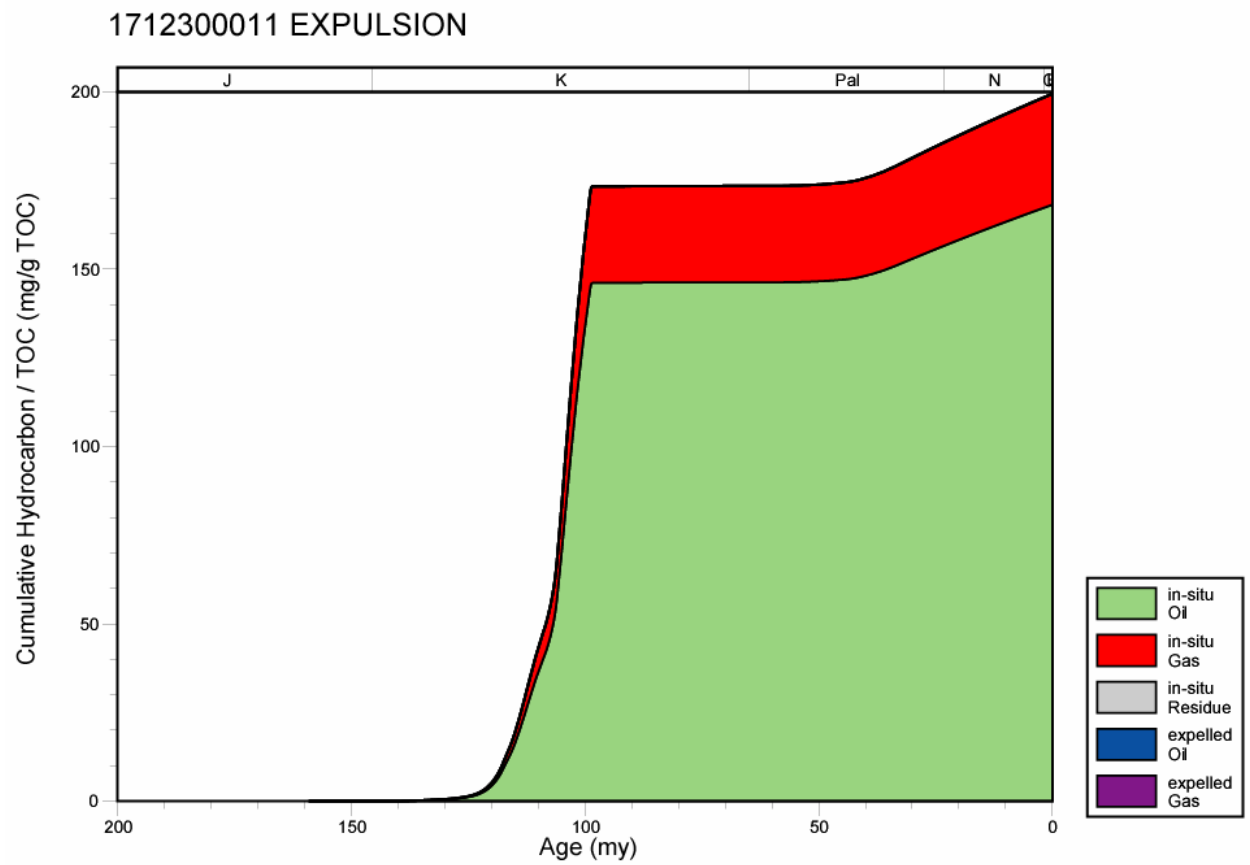
Figure 170. Hydrocarbon expulsion plot for well 1712300011, North Louisiana Salt Basin.
