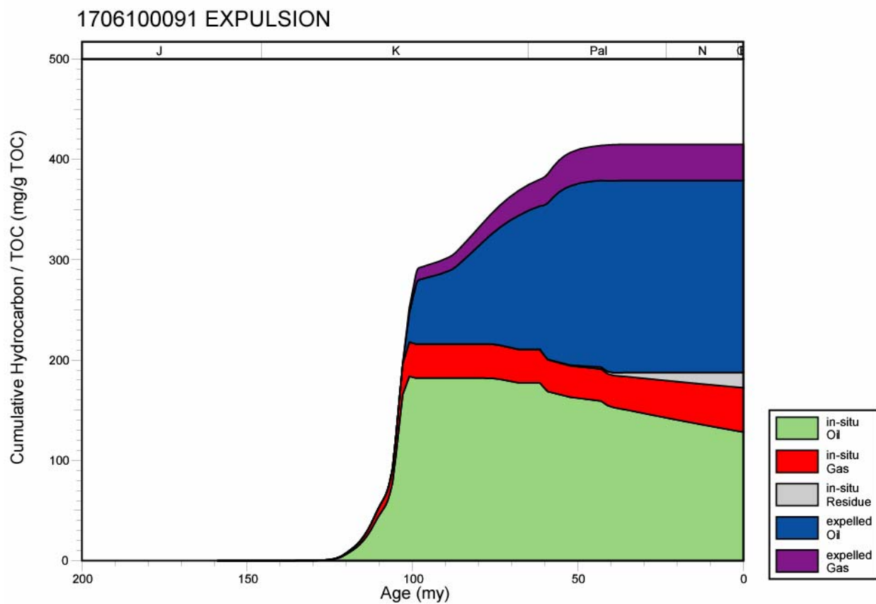
Figure 160. Hydrocarbon expulsion plot for well 1706100091, North Louisiana Salt Basin.
