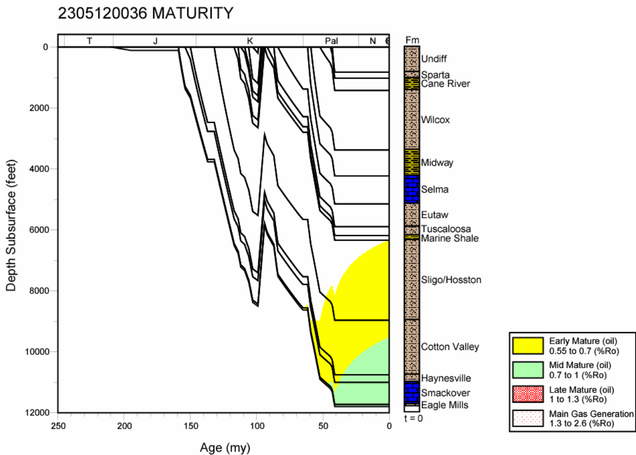
Figure 241. Thermal maturation profile for well 2305120036, Mississippi Interior Salt Basin.
