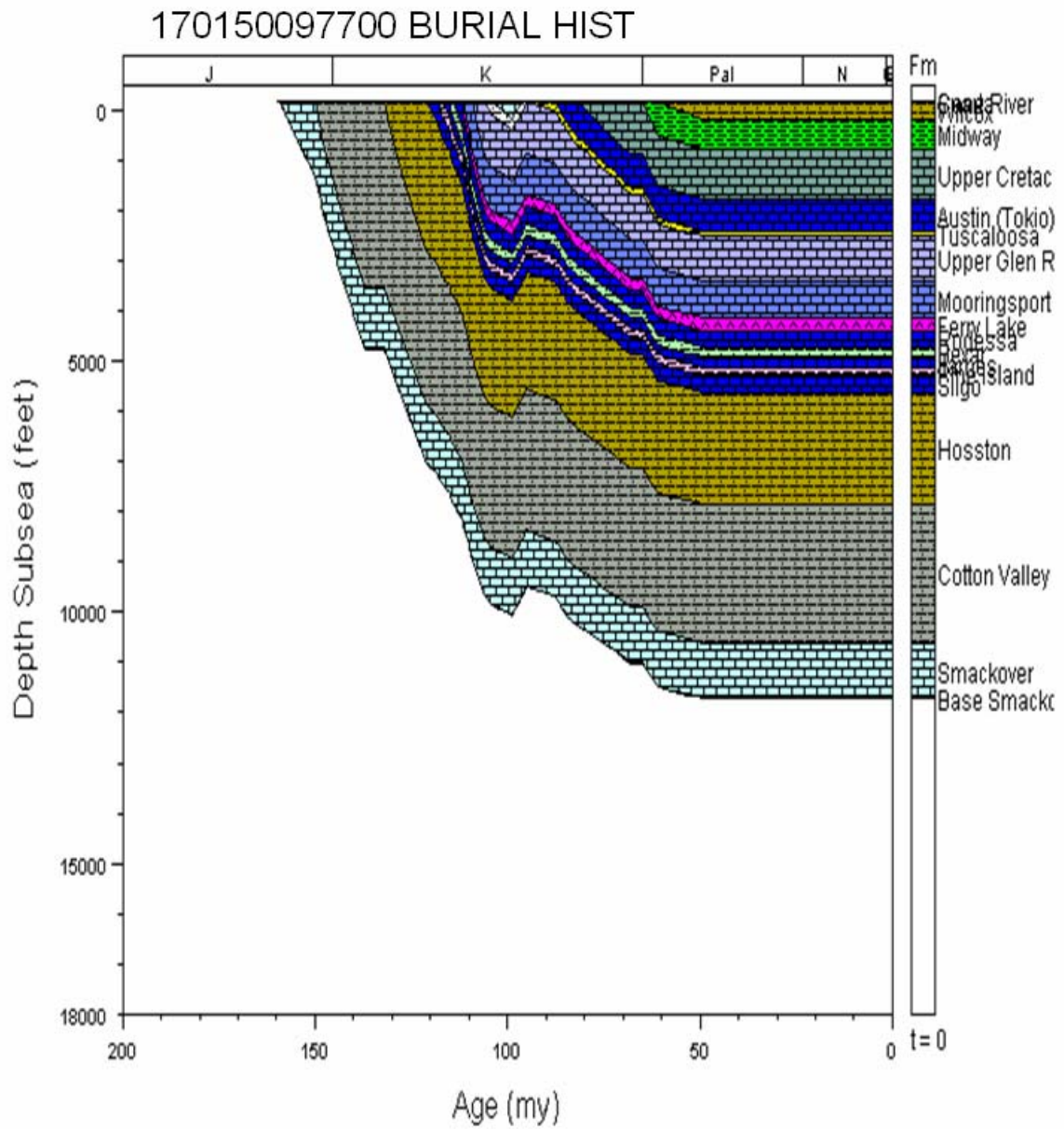
Figure 313. Burial history for well 170150097700. Sabine Uplift. Prepared by Roger Barnaby.
