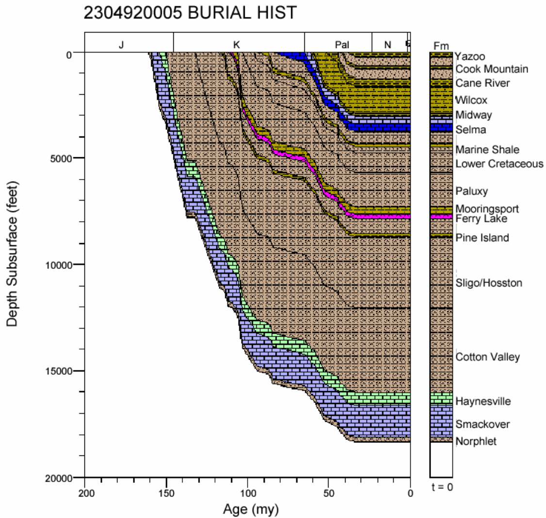
Figure 176. Burial history for well 2304920005, Mississippi Interior Salt Basin.
