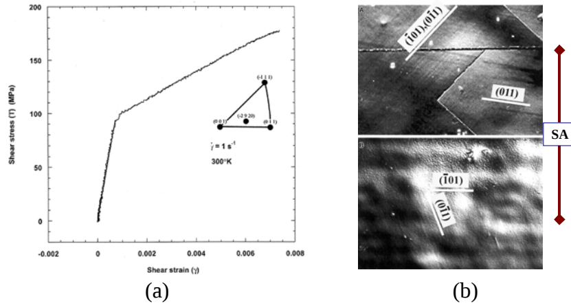
Fig. 1. (a) The stress-strain curve recorded from the uniaxial compression of a [\bar{2} \ 9 \ 20] -oriented Mo crystal; (b) The optical metallography taken from two surfaces of the tested crystal showing the anomalous slip.
