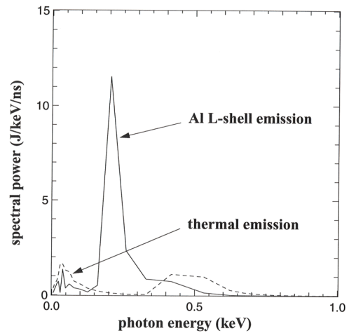
Figure 1. Simulated spectral power crossing the front face of the parylene-N for an intensity of 2 \times 10^{11} \text{ W/cm}^2 incident on a target of 15 \mu m parylene-N on 250 \mu m Fe, with (solid curve) and without (dashed curve) a 0.1- \mu m Al overcoat on the ablator.
