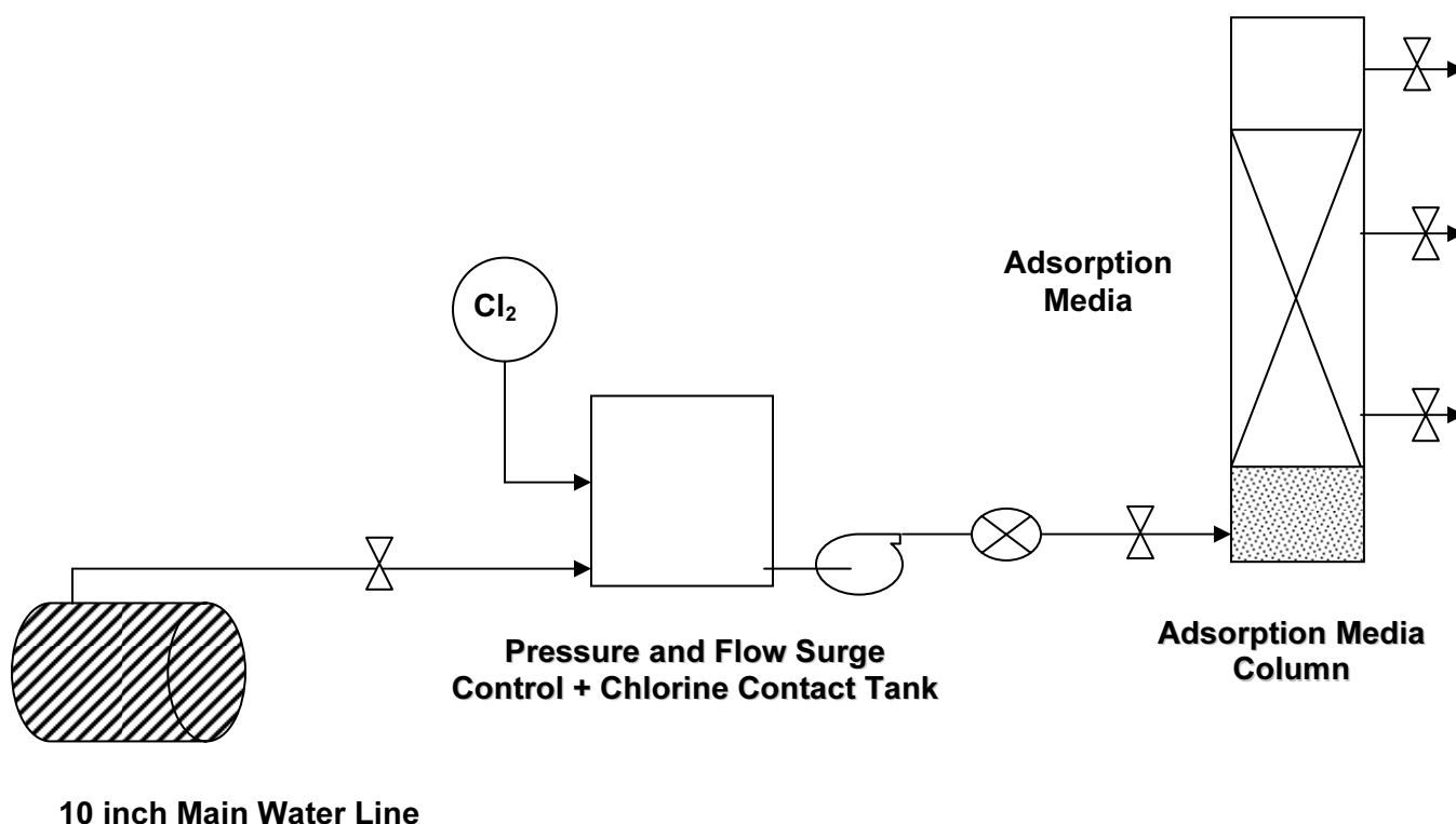
Figure 2-1. Process Flow Diagram of Field Trial Setup for Evaluation of Arsenic Sorption Media.
