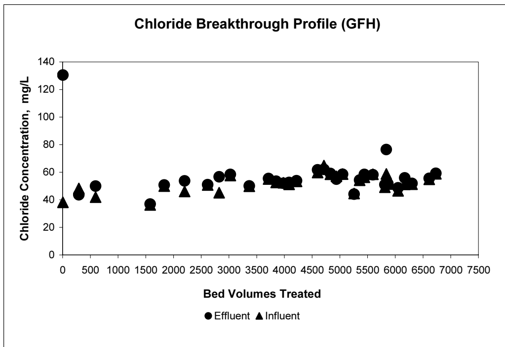
Figure 4-8. Chloride Breakthrough Profile of Granular Ferric Hydroxide (GFH) Packed Column.
