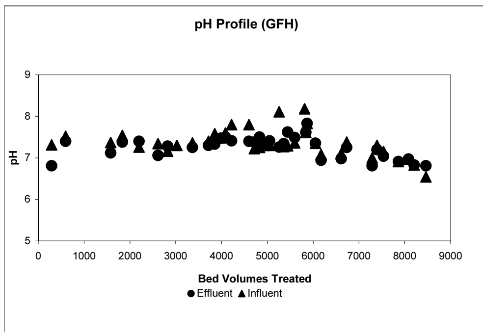
Figure 4-3. pH Profile of Granular Ferric Hydroxide (GFH) Packed Column.
