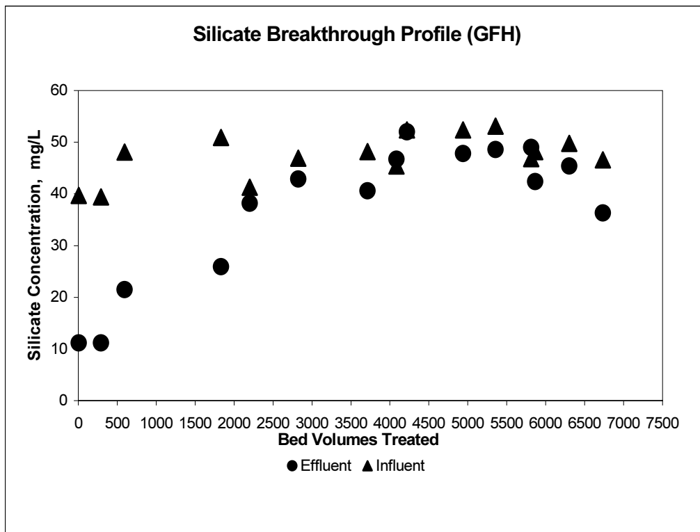
Figure 4-5. Silicates Breakthrough Profile of Granular Ferric Hydroxide (GFH) Packed Column.
