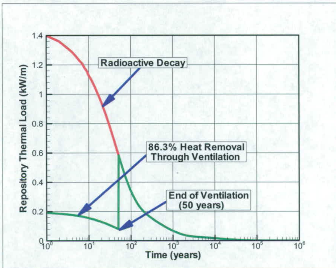
Figure 2. Radioactive heat decay curve for an initial thermal load of 1.45 kW/m. showing the thermal load when 86.3% of the heat is removed by ventilation during the first 50 years [26]
