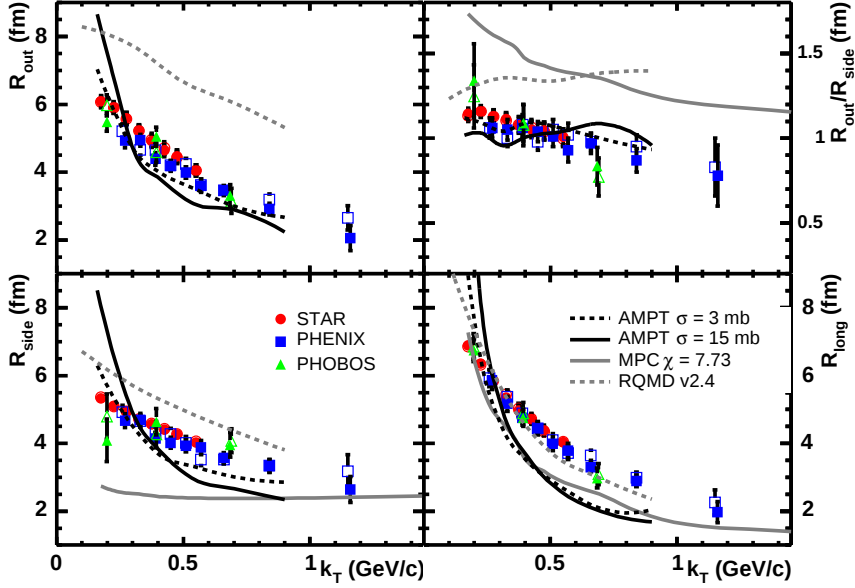
Figure 15: RHIC results are compared to three Boltzmann/cascade models, RQMD, MPC and AMPT with two different parton cross sections. Data are for 2\pi^- (open symbols) and 2\pi^+ (closed symbols) source radii.
