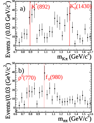
FIG. 3: a) shows the m_{K_S^0\pi} signal distribution of B^0 \rightarrow K^0\pi^+\pi^- candidates [17]. The one-dimensional distribution is obtained by merging m_{K\pi^+}^2 and m_{K\pi^-}^2 into one ( m_{K\pi}^2 ) by folding the Dalitz plane along the line corresponding to m_{K\pi^+}^2 = m_{K\pi^-}^2 in order to obtain the above m_{K\pi} mass distribution. b) shows the m_{\pi^+\pi^-} signal distribution of B^0 \rightarrow K^0\pi^+\pi^- candidates [17]. The dashed lines indicate the expected mass of the labeled resonances.
